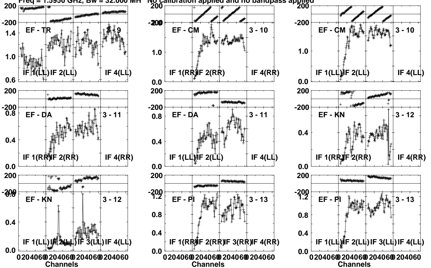
Lower frame: Milli Ampl Jy Top frame: Phas deg Vector averaged cross-power spectrum Several baselines displayed Timerange: 01/00:56:31 to 01/00:57:29
