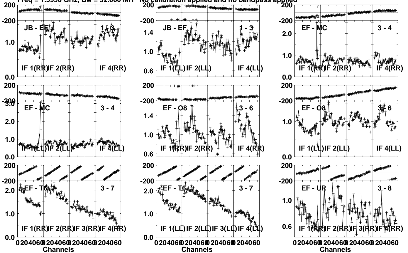
Lower frame: Milli Ampl Jy Top frame: Phas deg Vector averaged cross-power spectrum Several baselines displayed Timerange: 01/01:40:31 to 01/01:41:29
