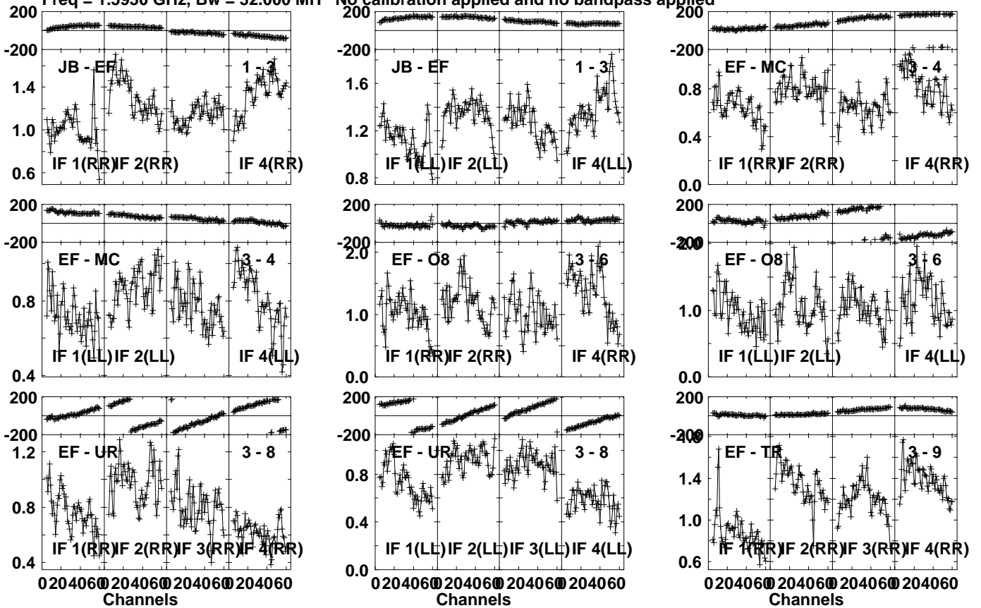
Lower frame: Milli Ampl Jy Top frame: Phas deg Vector averaged cross-power spectrum Several baselines displayed Timerange: 01/00:51:01 to 01/00:51:59
