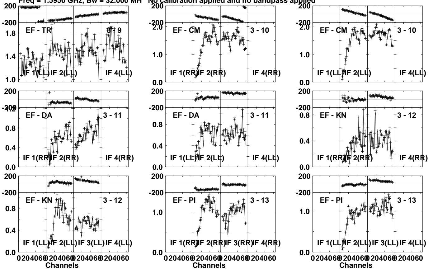
Lower frame: Milli Ampl Jy Top frame: Phas deg Vector averaged cross-power spectrum Several baselines displayed Timerange: 00/19:05:01 to 00/19:05:59
