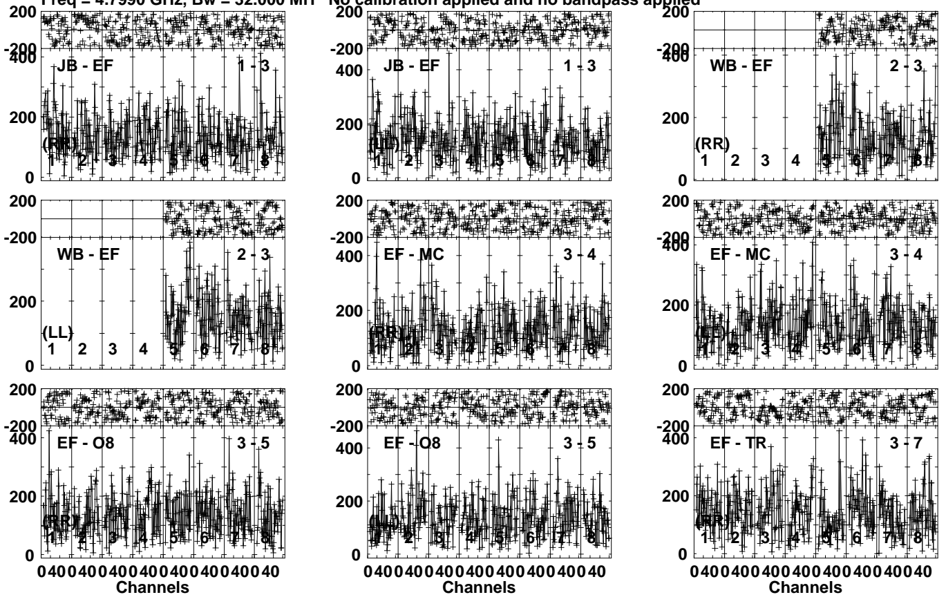
Lower frame: Micro Ampl Jy Top frame: Phas deg Vector averaged cross-power spectrum Several baselines displayed Timerange: 00/14:59:51 to 00/15:01:49
