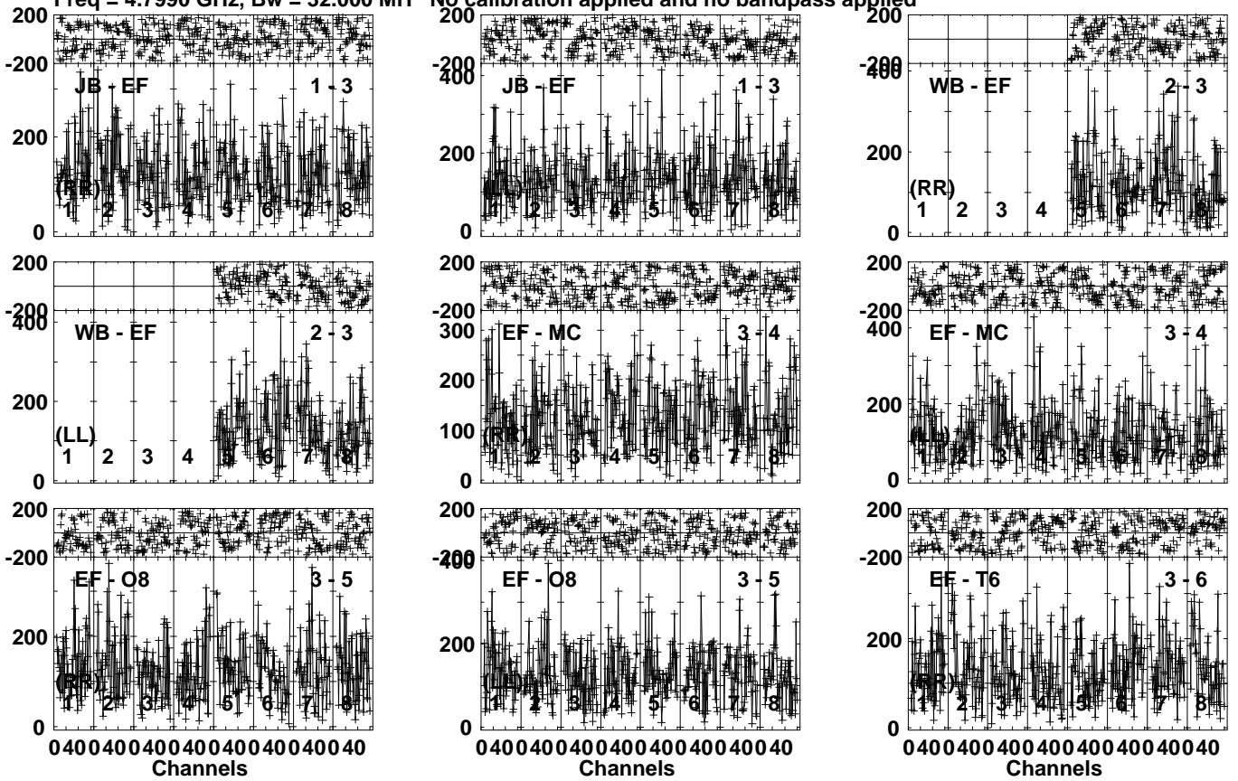
Lower frame: Micro Ampl Jy Top frame: Phas deg Vector averaged cross-power spectrum Several baselines displayed Timerange: 01/11:52:21 to 01/11:54:19
