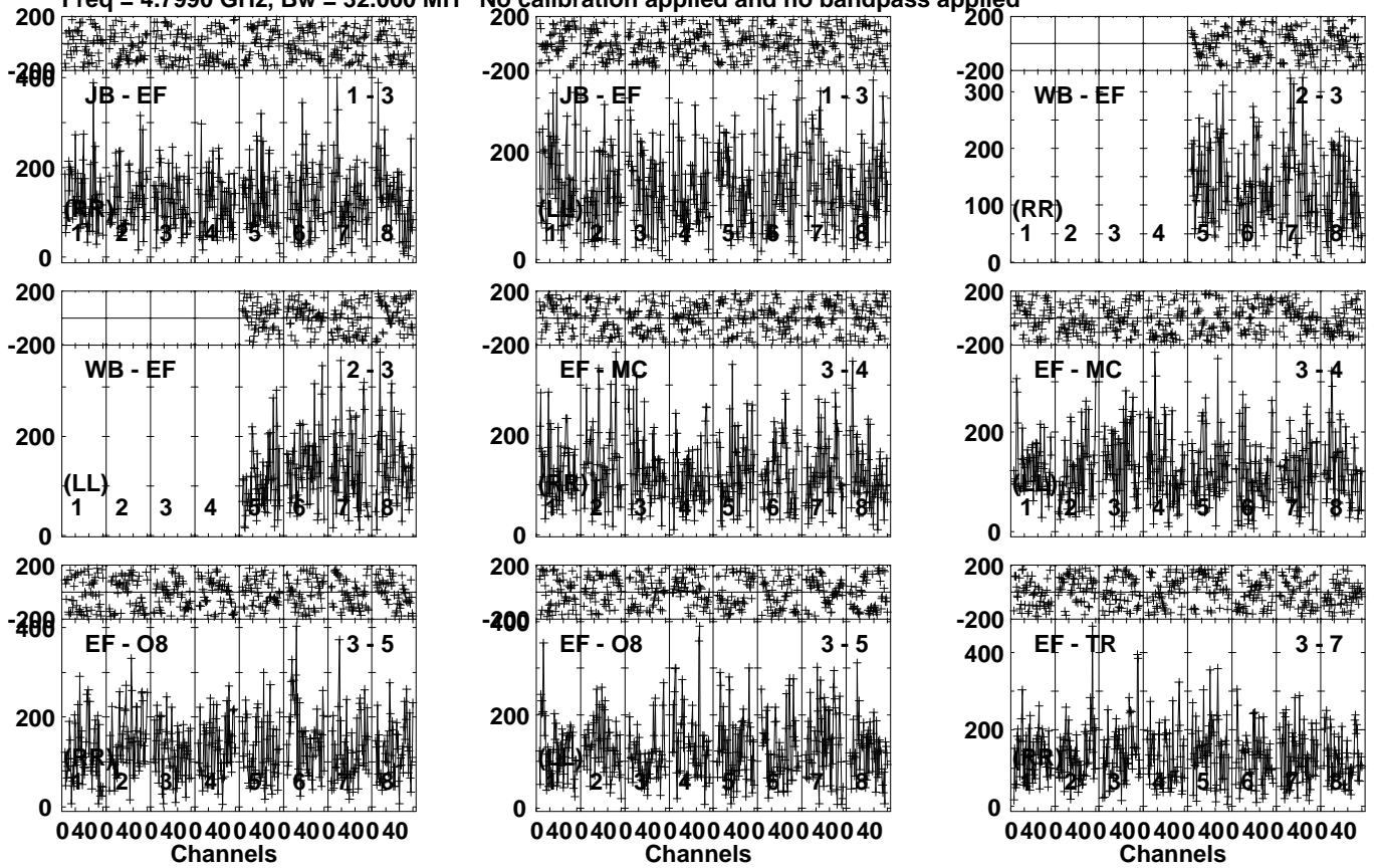
Lower frame: Micro Ampl Jy Top frame: Phas deg Vector averaged cross-power spectrum Several baselines displayed Timerange: 01/12:53:01 to 01/12:54:59
