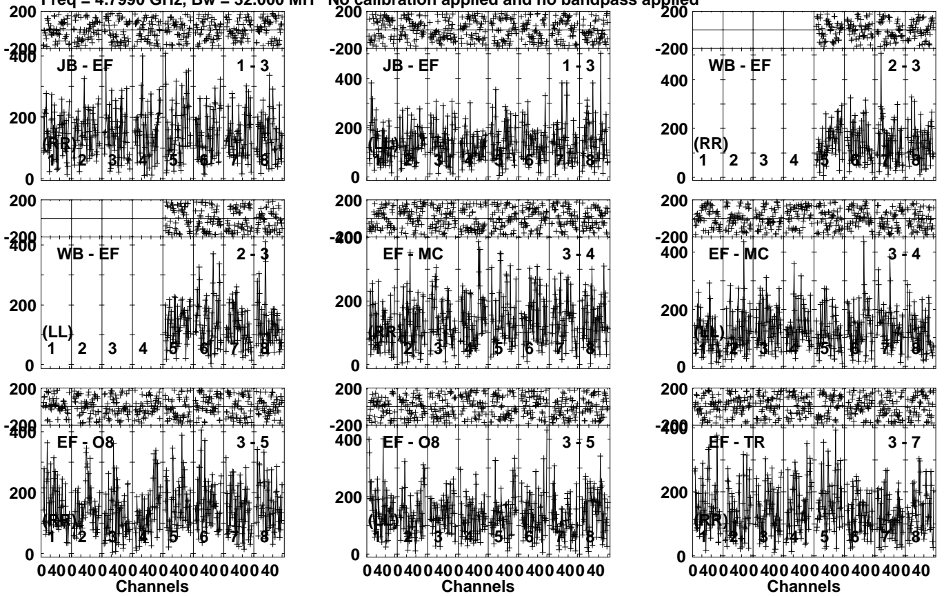
Lower frame: Micro Ampl Jy Top frame: Phas deg Vector averaged cross-power spectrum Several baselines displayed Timerange: 00/16:32:11 to 00/16:34:09
