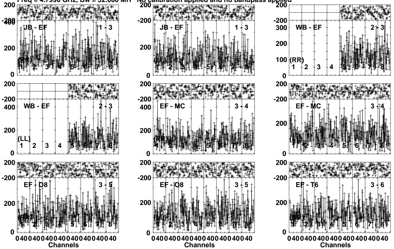
Lower frame: Micro Ampl Jy Top frame: Phas deg Vector averaged cross-power spectrum Several baselines displayed Timerange: 01/11:20:51 to 01/11:22:49
