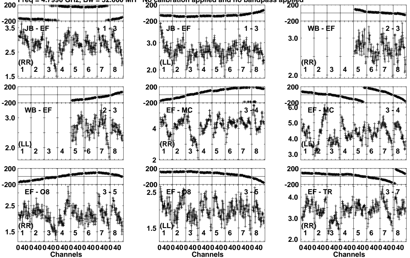
Lower frame: Milli Ampl Jy Top frame: Phas deg Vector averaged cross-power spectrum Several baselines displayed Timerange: 00/15:30:21 to 00/15:31:19
