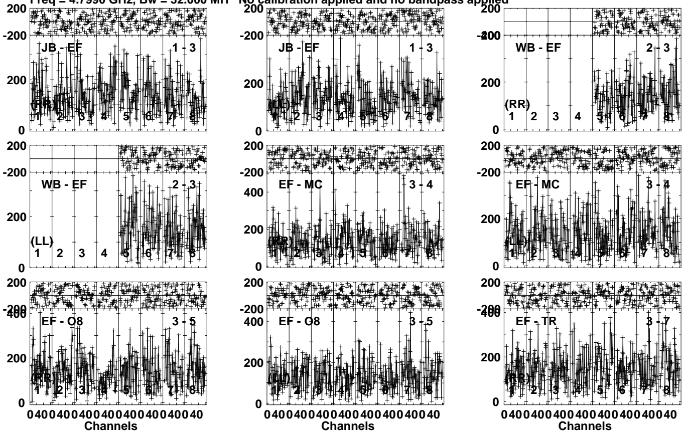
Lower frame: Micro Ampl Jy Top frame: Phas deg Vector averaged cross-power spectrum Several baselines displayed Timerange: 00/16:42:41 to 00/16:44:39
