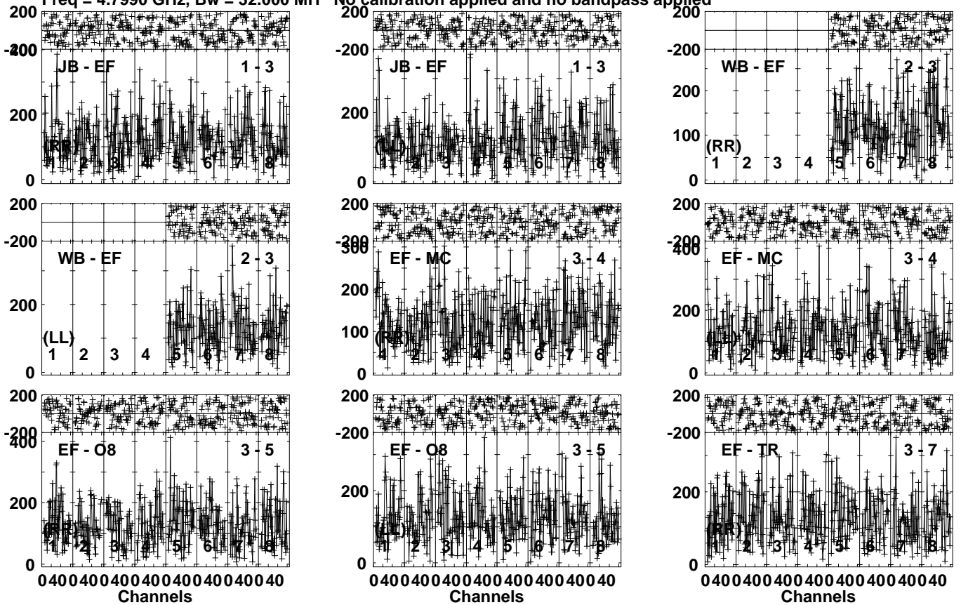
Lower frame: Micro Ampl Jy Top frame: Phas deg Vector averaged cross-power spectrum Several baselines displayed Timerange: 01/12:16:51 to 01/12:18:49
