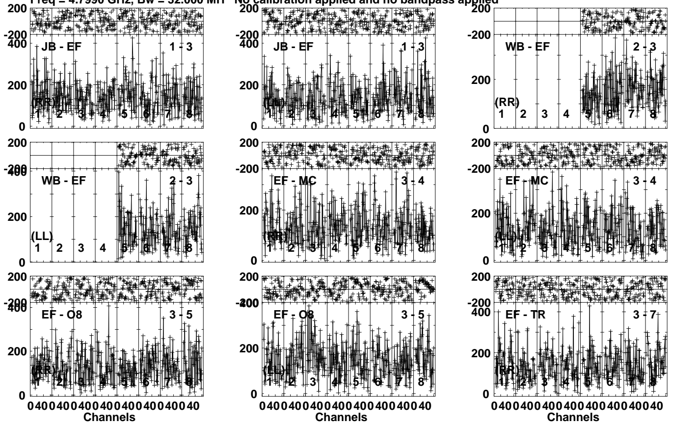
Lower frame: Micro Ampl Jy Top frame: Phas deg Vector averaged cross-power spectrum Several baselines displayed Timerange: 00/13:03:01 to 00/13:04:59
