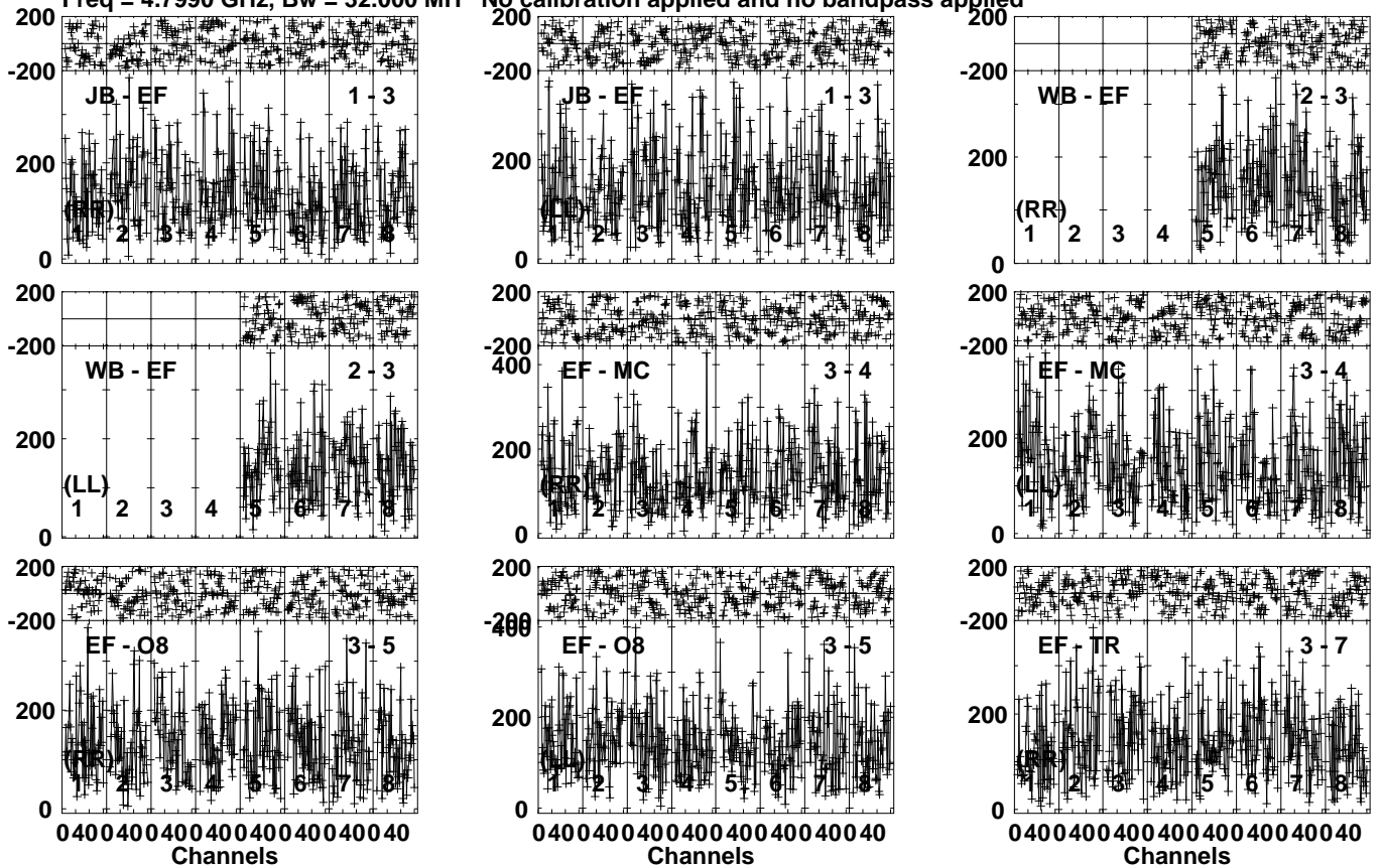
Lower frame: Micro Ampl Jy Top frame: Phas deg Vector averaged cross-power spectrum Several baselines displayed Timerange: 00/13:24:01 to 00/13:25:59
