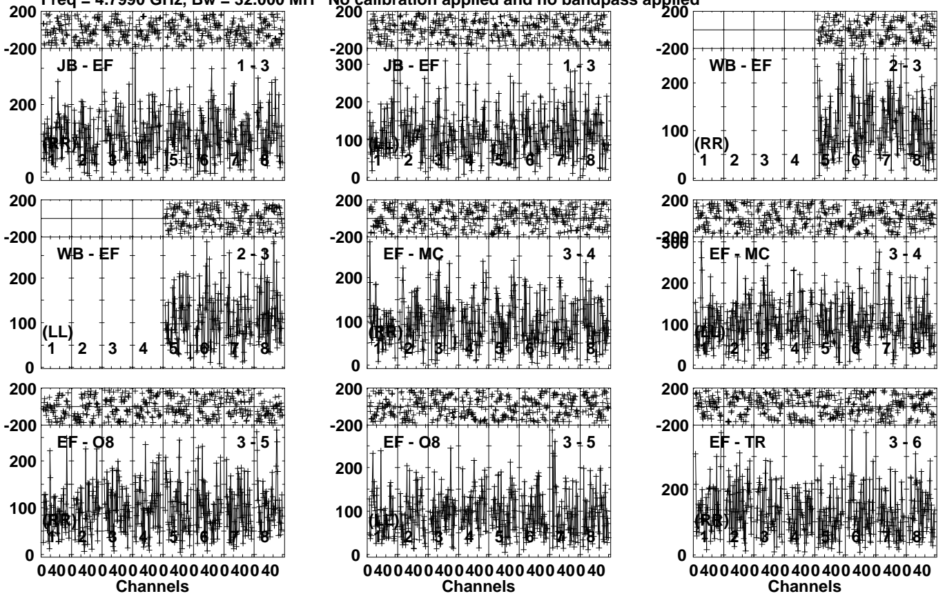
Lower frame: Micro Ampl Jy Top frame: Phas deg Vector averaged cross-power spectrum Several baselines displayed Timerange: 00/12:47:41 to 00/12:49:39
