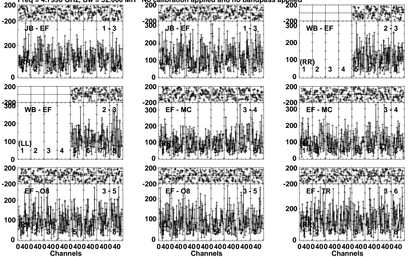
Lower frame: Micro Ampl Jy Top frame: Phas deg Vector averaged cross-power spectrum Several baselines displayed Timerange: 00/11:58:41 to 00/12:00:39
