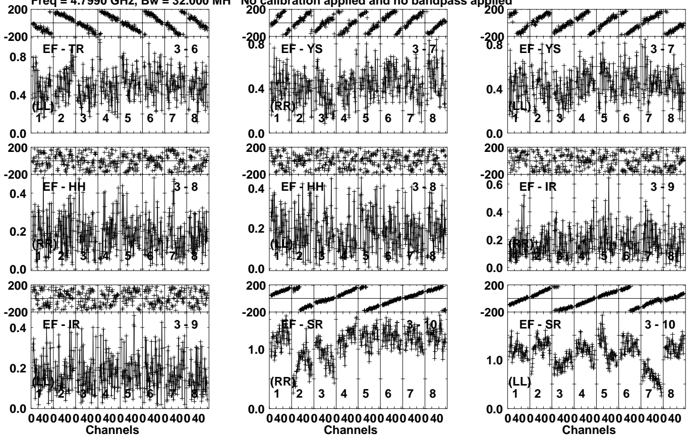
Lower frame: Milli Ampl Jy Top frame: Phas deg Vector averaged cross-power spectrum Several baselines displayed Timerange: 00/10:13:31 to 00/10:14:29
