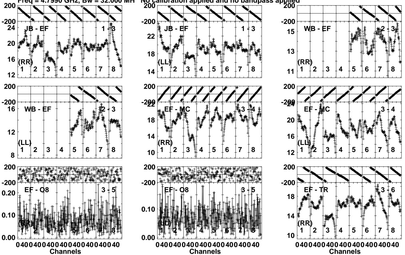
Lower frame: Milli Ampl Jy Top frame: Phas deg Vector averaged cross-power spectrum Several baselines displayed Timerange: 00/10:19:31 to 00/10:23:29
