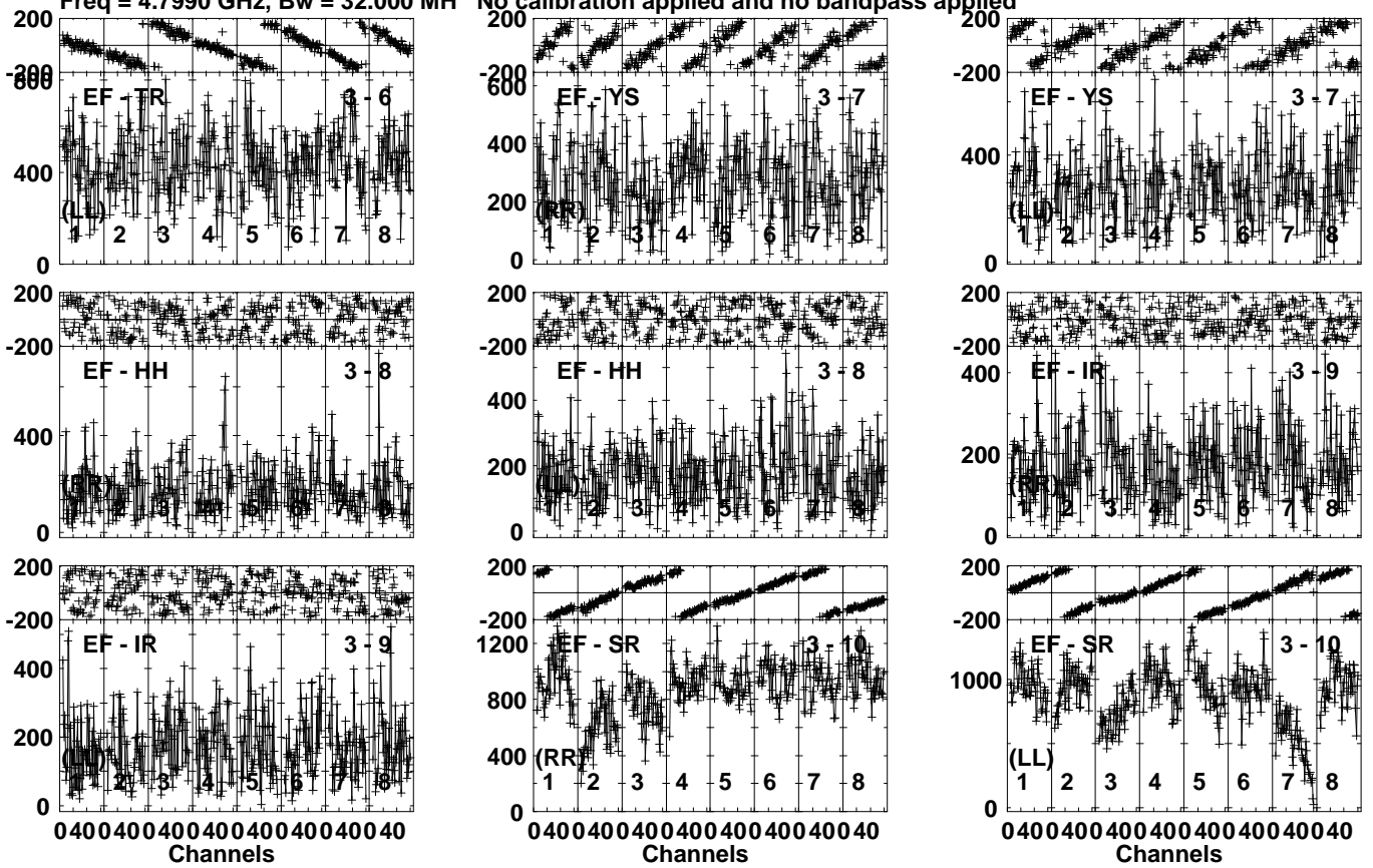
Lower frame: Micro Ampl Jy Top frame: Phas deg Vector averaged cross-power spectrum Several baselines displayed Timerange: 00/08:27:41 to 00/08:28:39
