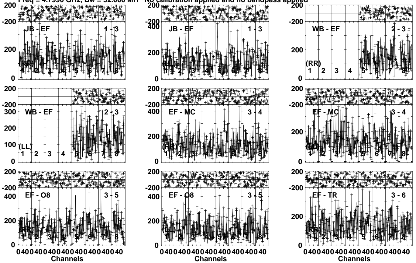
Lower frame: Micro Ampl Jy Top frame: Phas deg Vector averaged cross-power spectrum Several baselines displayed Timerange: 00/08:39:11 to 00/08:41:09
