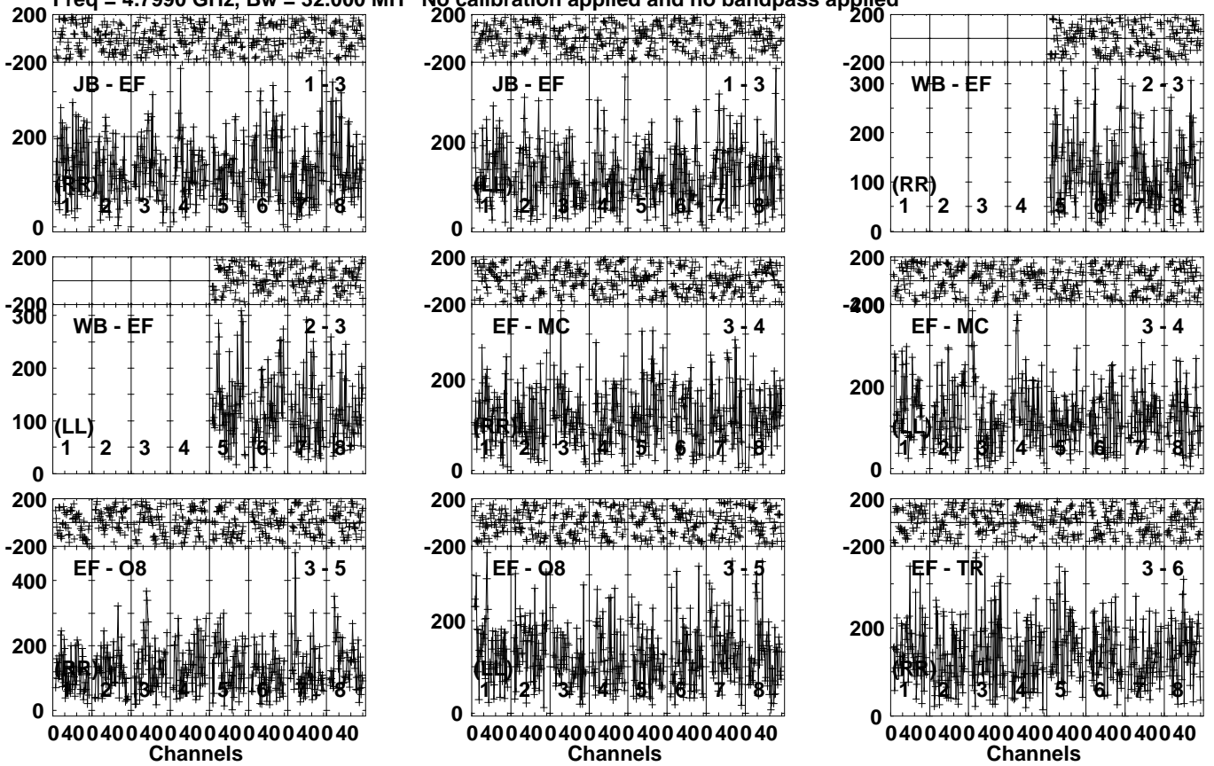
Lower frame: Micro Ampl Jy Top frame: Phas deg Vector averaged cross-power spectrum Several baselines displayed Timerange: 00/08:14:41 to 00/08:16:39
