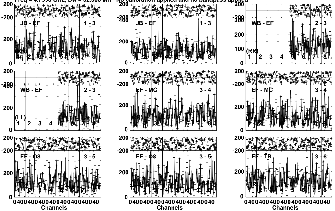
Lower frame: Micro Ampl Jy Top frame: Phas deg Vector averaged cross-power spectrum Several baselines displayed Timerange: 00/10:26:21 to 00/10:28:19
