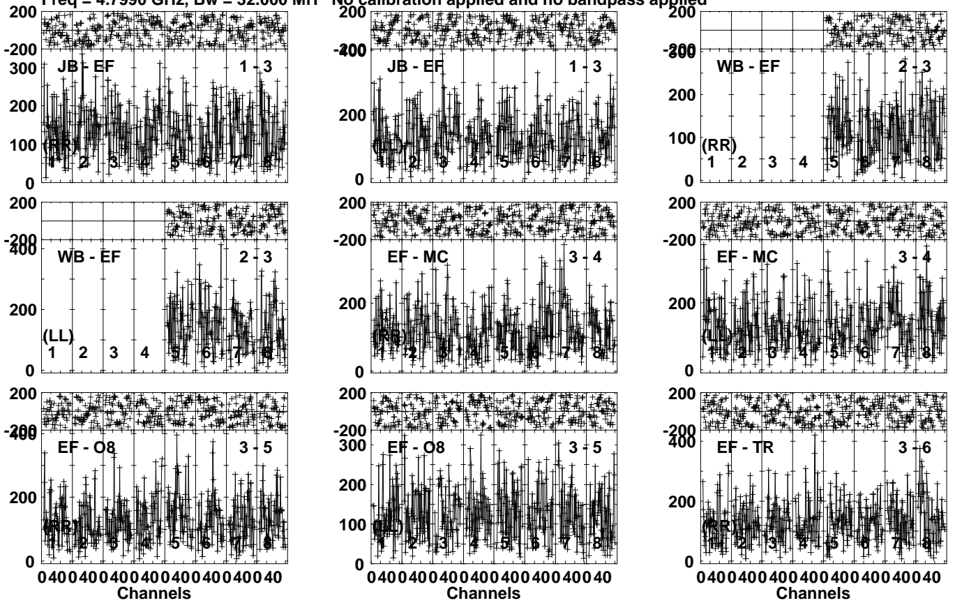
Lower frame: Micro Ampl Jy Top frame: Phas deg Vector averaged cross-power spectrum Several baselines displayed Timerange: 00/08:11:11 to 00/08:13:09
