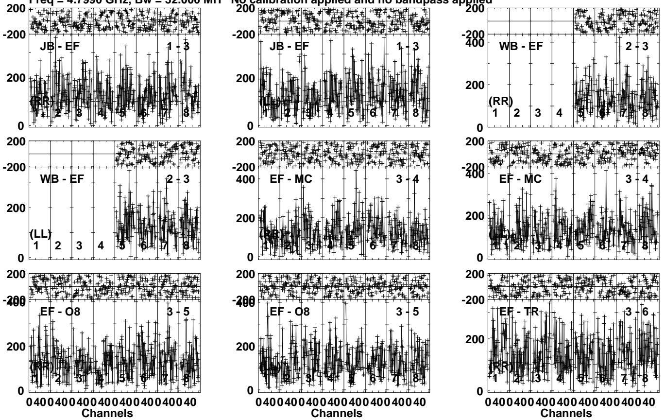
Lower frame: Micro Ampl Jy Top frame: Phas deg Vector averaged cross-power spectrum Several baselines displayed Timerange: 00/07:43:11 to 00/07:45:09
