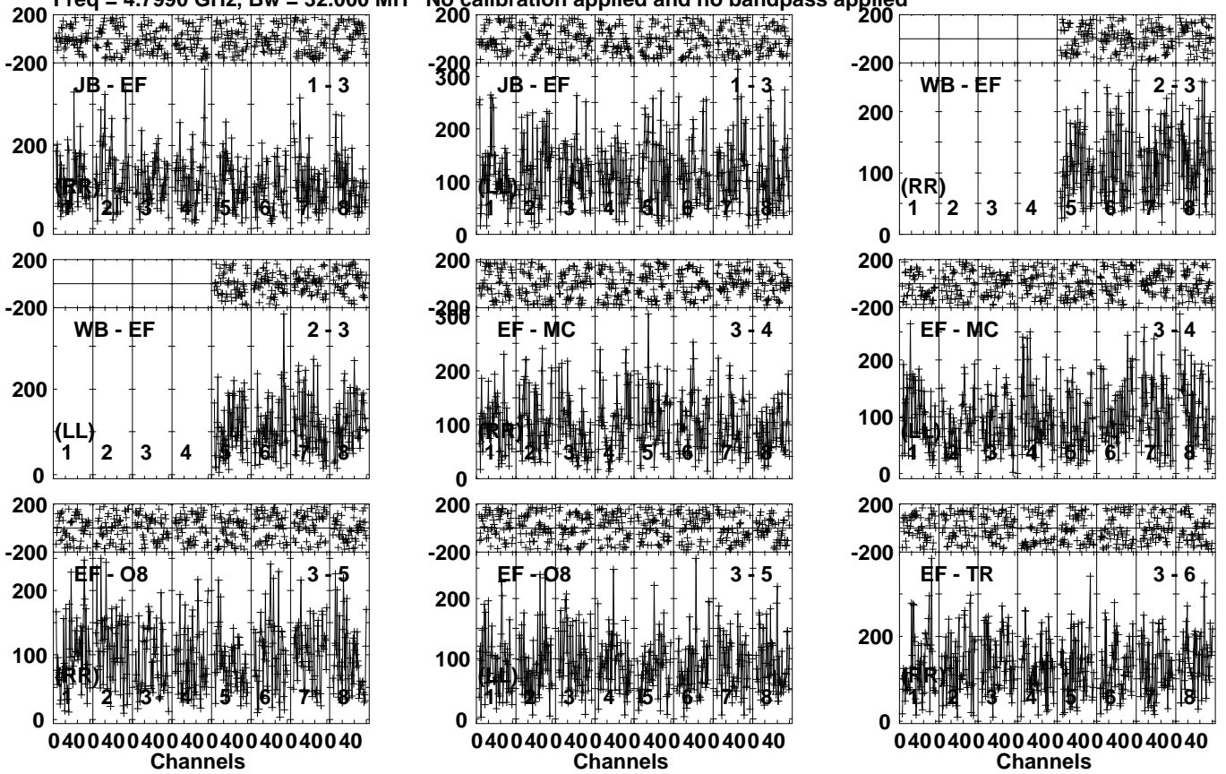
Lower frame: Micro Ampl Jy Top frame: Phas deg Vector averaged cross-power spectrum Several baselines displayed Timerange: 00/11:55:11 to 00/11:57:09
