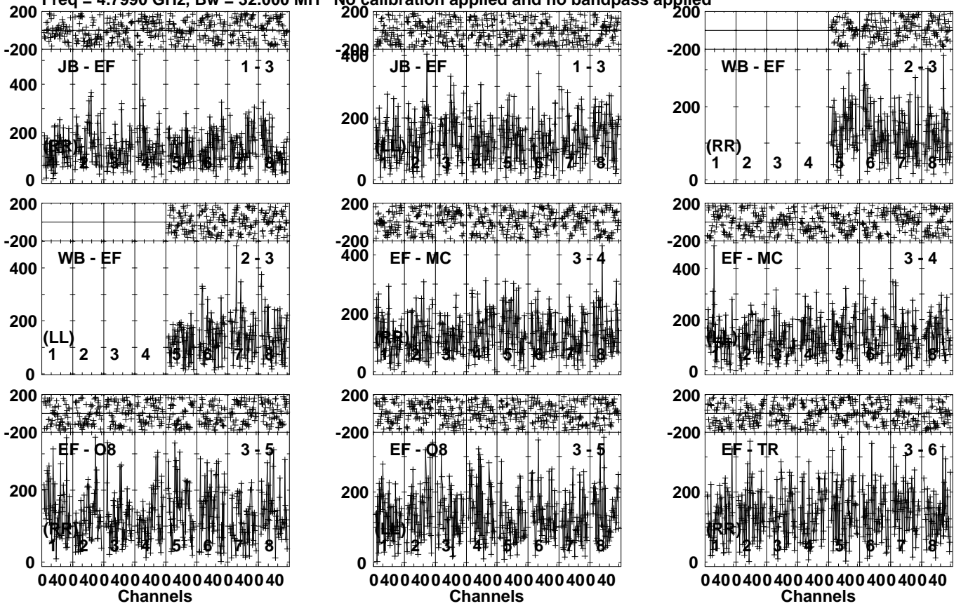
Lower frame: Micro Ampl Jy Top frame: Phas deg Vector averaged cross-power spectrum Several baselines displayed Timerange: 00/07:27:51 to 00/07:29:49
