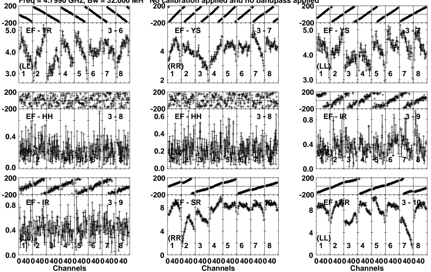
Lower frame: Milli Ampl Jy Top frame: Phas deg Vector averaged cross-power spectrum Several baselines displayed Timerange: 00/11:00:21 to 00/11:01:19
