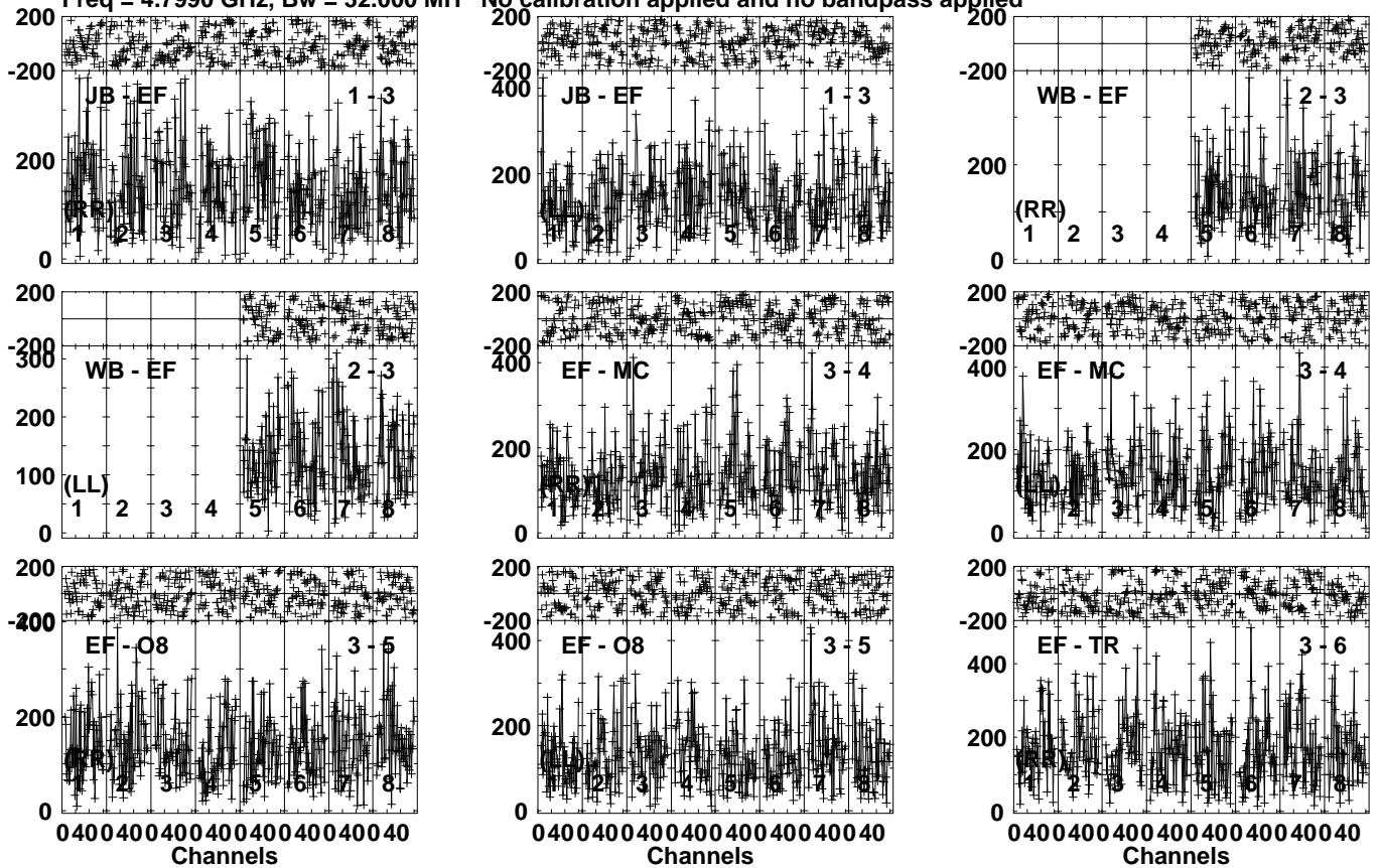
Lower frame: Micro Ampl Jy Top frame: Phas deg Vector averaged cross-power spectrum Several baselines displayed Timerange: 00/12:46:41 to 00/12:47:39
