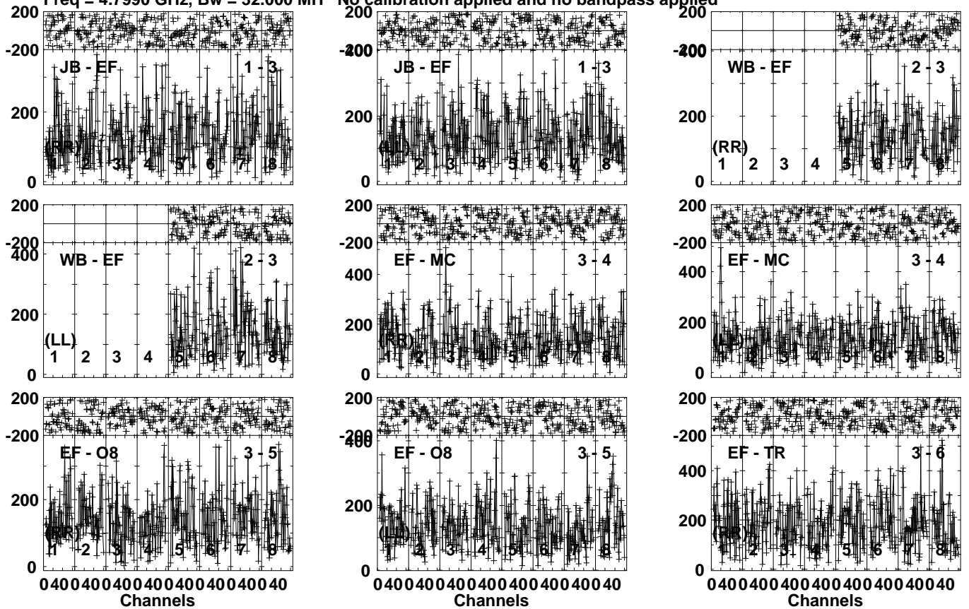
Lower frame: Micro Ampl Jy Top frame: Phas deg Vector averaged cross-power spectrum Several baselines displayed Timerange: 00/11:21:21 to 00/11:22:19
