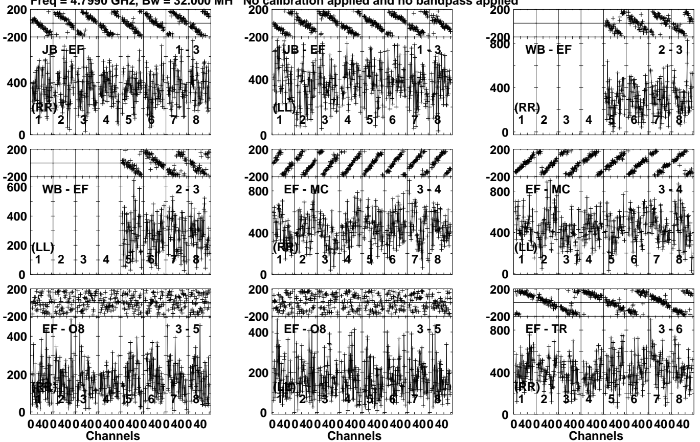
Lower frame: Micro Ampl Jy Top frame: Phas deg Vector averaged cross-power spectrum Several baselines displayed Timerange: 00/07:23:21 to 00/07:24:19
