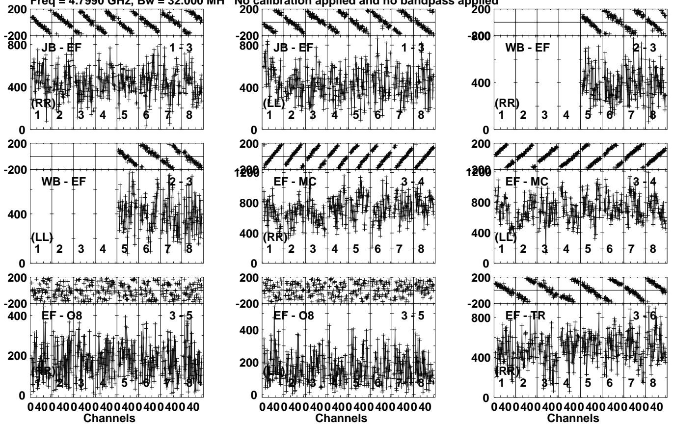
Lower frame: Micro Ampl Jy Top frame: Phas deg Vector averaged cross-power spectrum Several baselines displayed Timerange: 00/09:31:31 to 00/09:32:29
