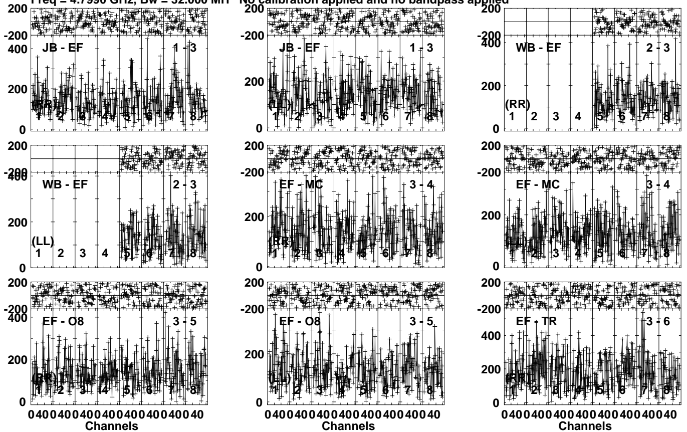
Lower frame: Micro Ampl Jy Top frame: Phas deg Vector averaged cross-power spectrum Several baselines displayed Timerange: 00/12:01:11 to 00/12:02:09
