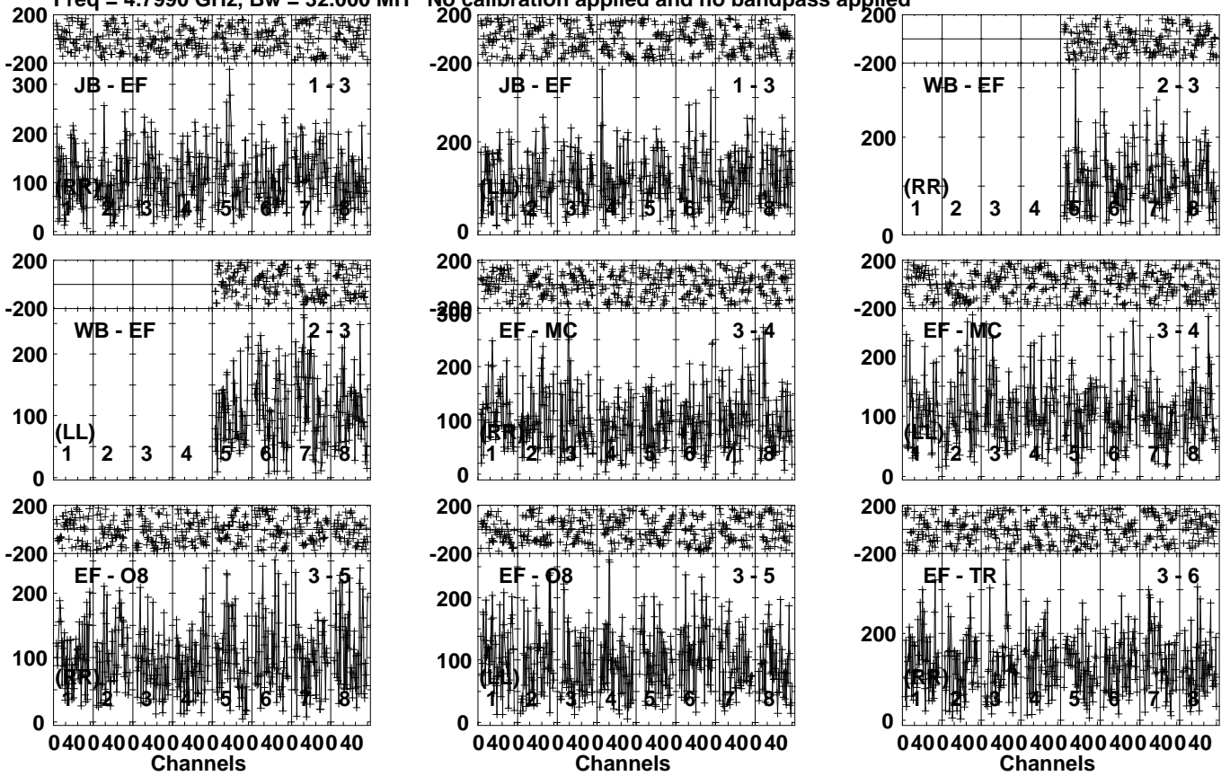
Lower frame: Micro Ampl Jy Top frame: Phas deg Vector averaged cross-power spectrum Several baselines displayed Timerange: 00/11:04:51 to 00/11:06:49
