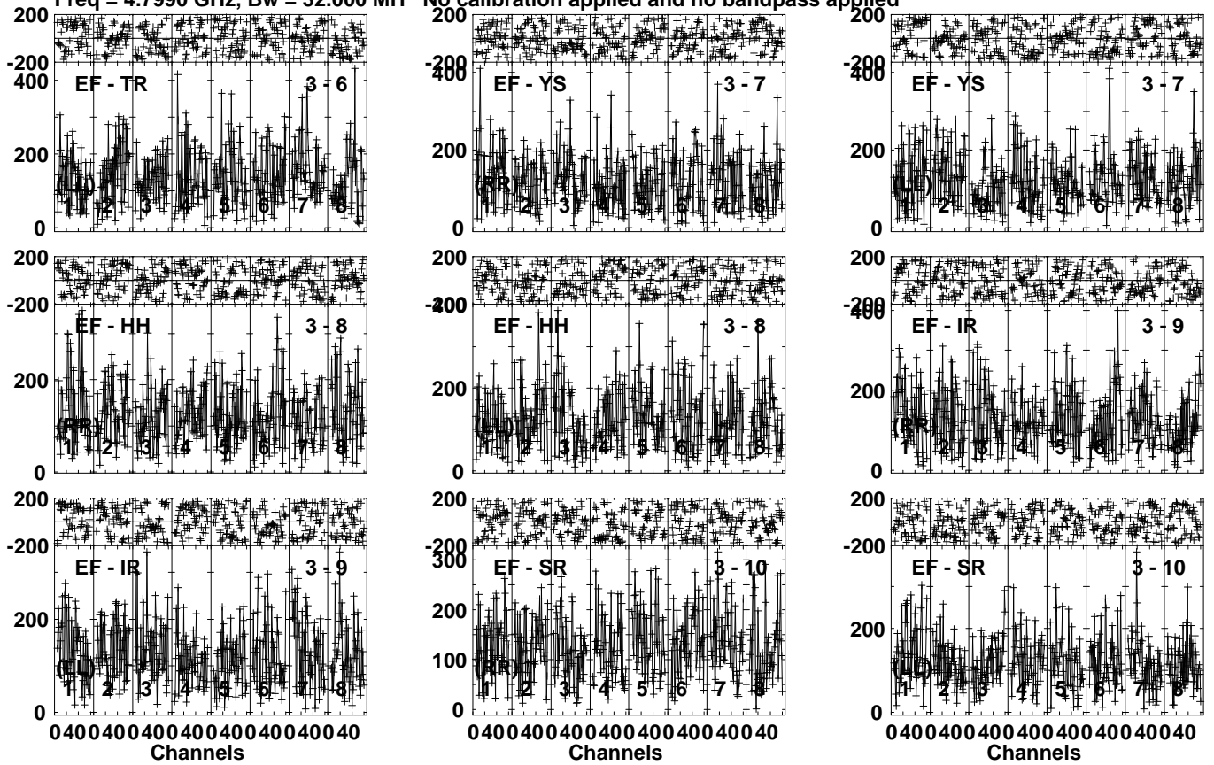
Lower frame: Micro Ampl Jy Top frame: Phas deg Vector averaged cross-power spectrum Several baselines displayed Timerange: 00/08:42:41 to 00/08:44:39
