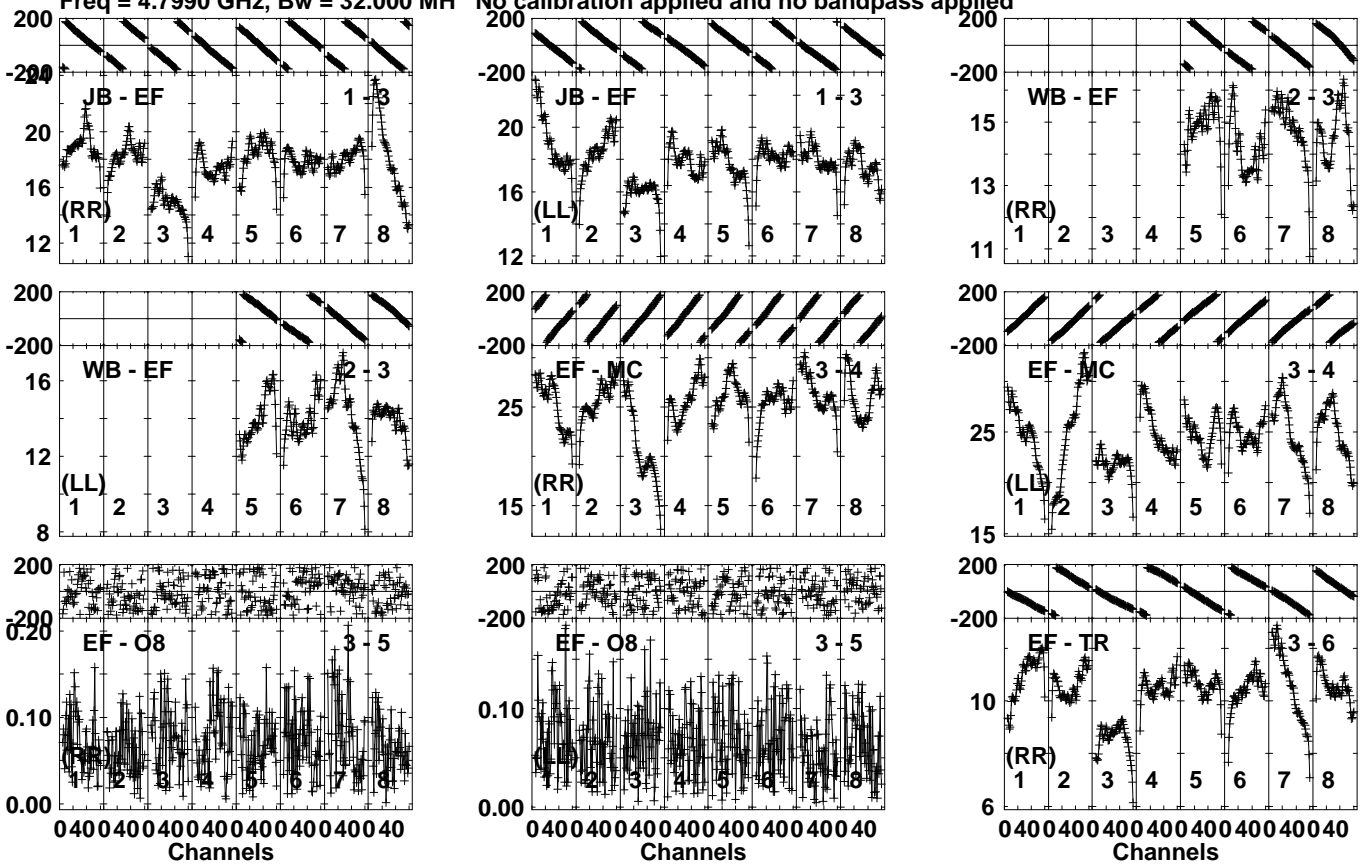
Lower frame: Milli Ampl Jy Top frame: Phas deg Vector averaged cross-power spectrum Several baselines displayed Timerange: 00/09:01:17 to 00/09:05:09
