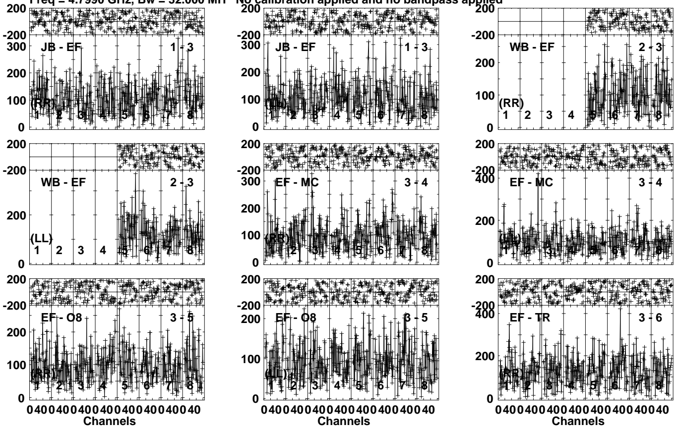
Lower frame: Micro Ampl Jy Top frame: Phas deg Vector averaged cross-power spectrum Several baselines displayed Timerange: 00/12:23:11 to 00/12:25:09
