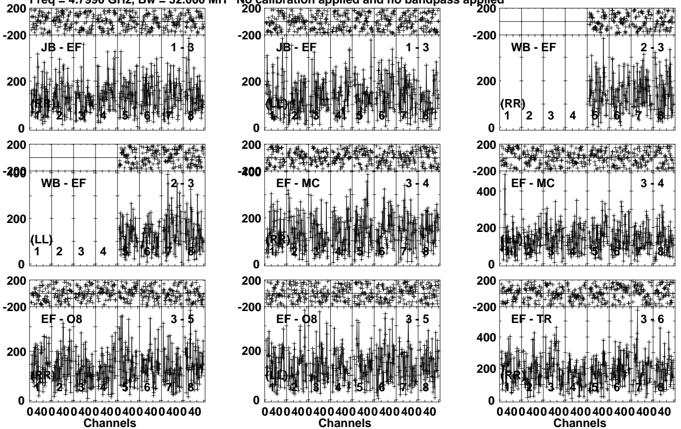
Lower frame: Micro Ampl Jy Top frame: Phas deg Vector averaged cross-power spectrum Several baselines displayed Timerange: 00/12:15:11 to 00/12:16:09
