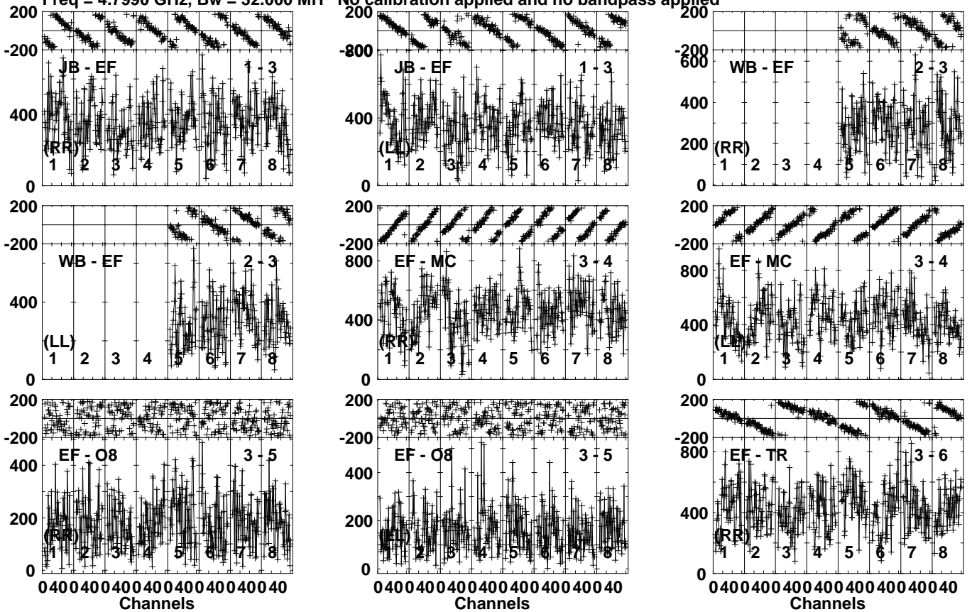
Lower frame: Micro Ampl Jy Top frame: Phas deg Vector averaged cross-power spectrum Several baselines displayed Timerange: 00/07:30:21 to 00/07:31:19
