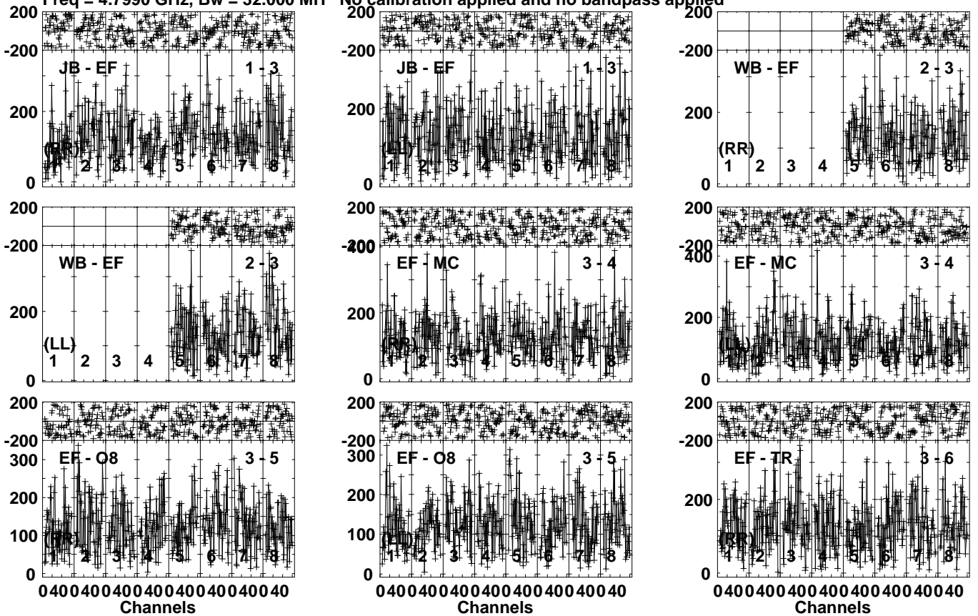
Lower frame: Micro Ampl Jy Top frame: Phas deg Vector averaged cross-power spectrum Several baselines displayed Timerange: 00/08:28:41 to 00/08:30:39
