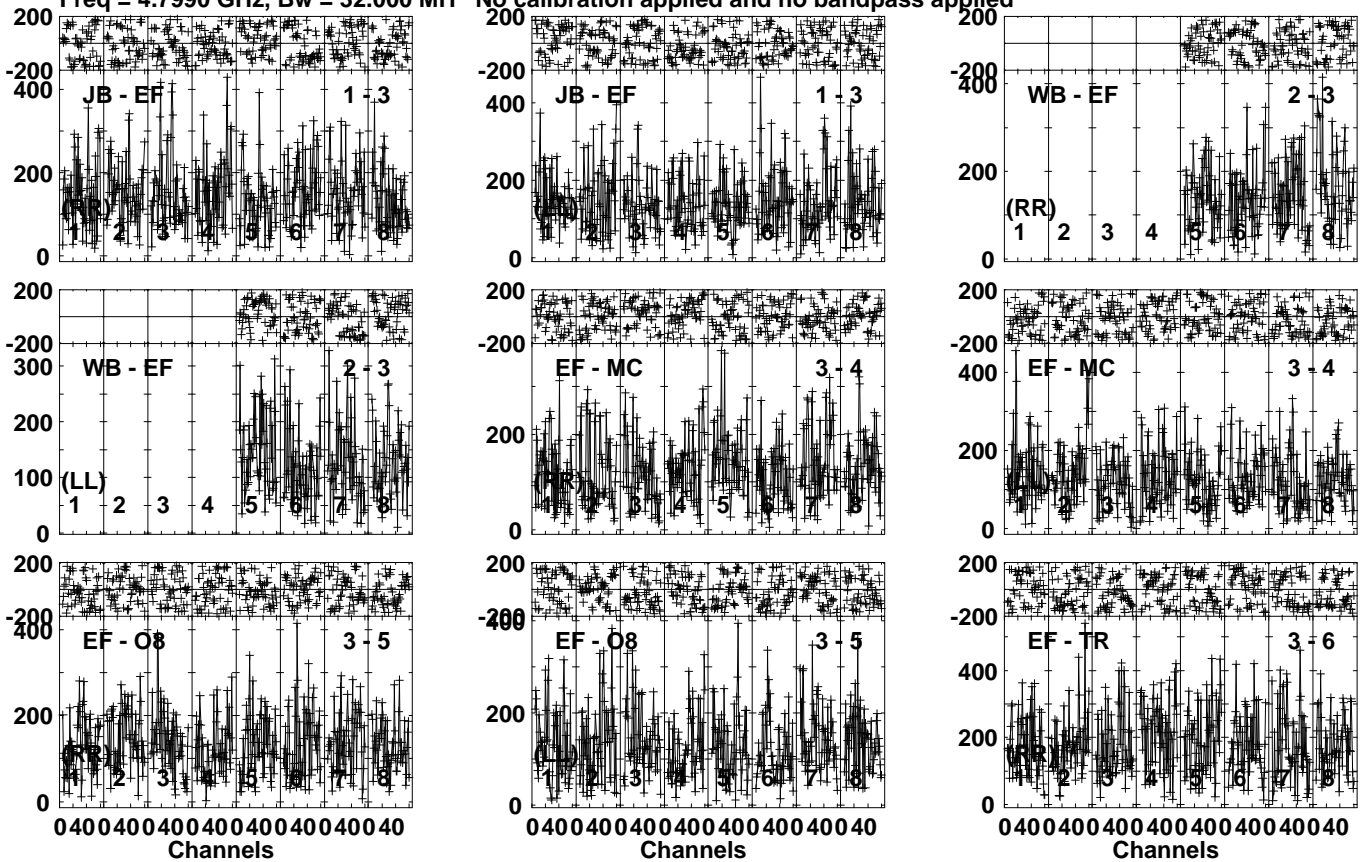
Lower frame: Micro Ampl Jy Top frame: Phas deg Vector averaged cross-power spectrum Several baselines displayed Timerange: 00/12:29:11 to 00/12:30:09
