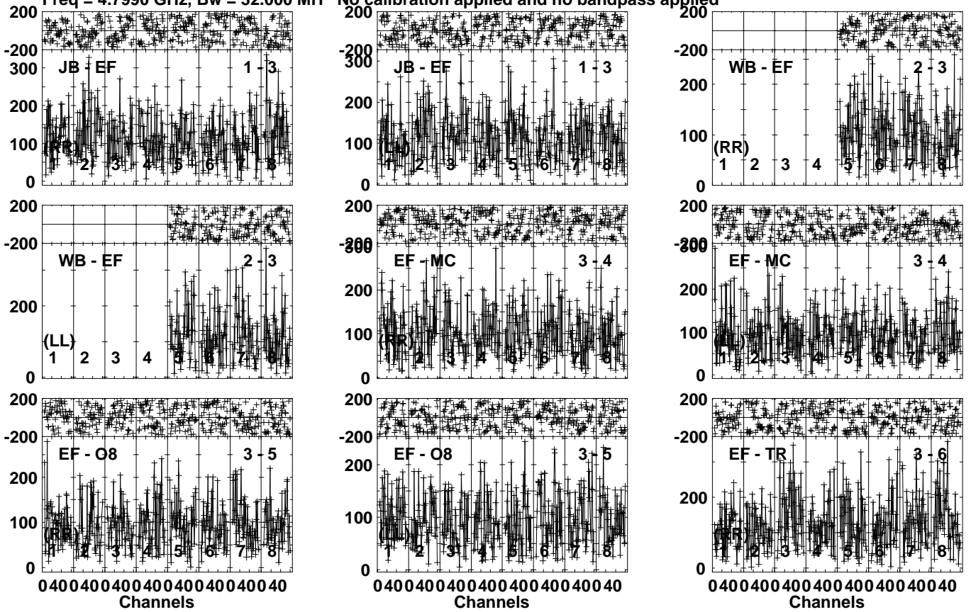
Lower frame: Micro Ampl Jy Top frame: Phas deg Vector averaged cross-power spectrum Several baselines displayed Timerange: 00/12:12:41 to 00/12:14:39
