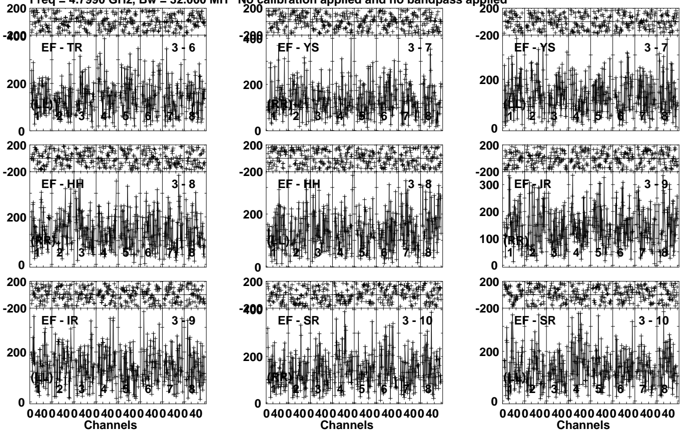
Lower frame: Micro Ampl Jy Top frame: Phas deg Vector averaged cross-power spectrum Several baselines displayed Timerange: 00/10:36:51 to 00/10:38:49
