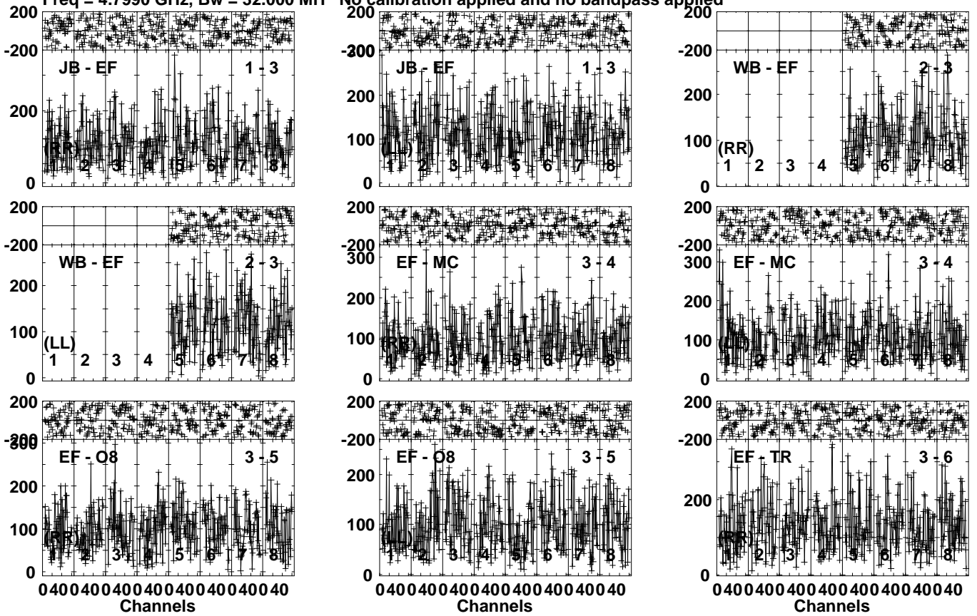
Lower frame: Micro Ampl Jy Top frame: Phas deg Vector averaged cross-power spectrum Several baselines displayed Timerange: 00/07:03:21 to 00/07:05:19
