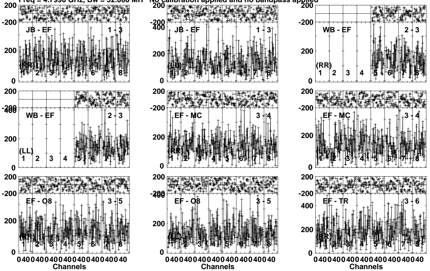
Lower frame: Micro Ampl Jy Top frame: Phas deg Vector averaged cross-power spectrum Several baselines displayed Timerange: 00/11:28:21 to 00/11:29:19
