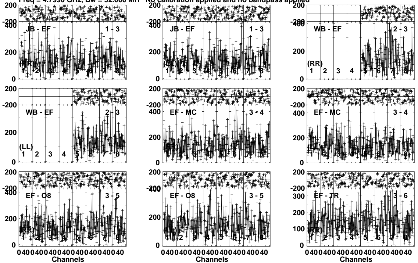
Lower frame: Micro Ampl Jy Top frame: Phas deg Vector averaged cross-power spectrum Several baselines displayed Timerange: 00/09:50:01 to 00/09:51:59
