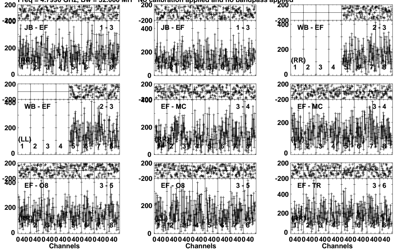
Lower frame: Micro Ampl Jy Top frame: Phas deg Vector averaged cross-power spectrum Several baselines displayed Timerange: 00/12:11:41 to 00/12:12:39
