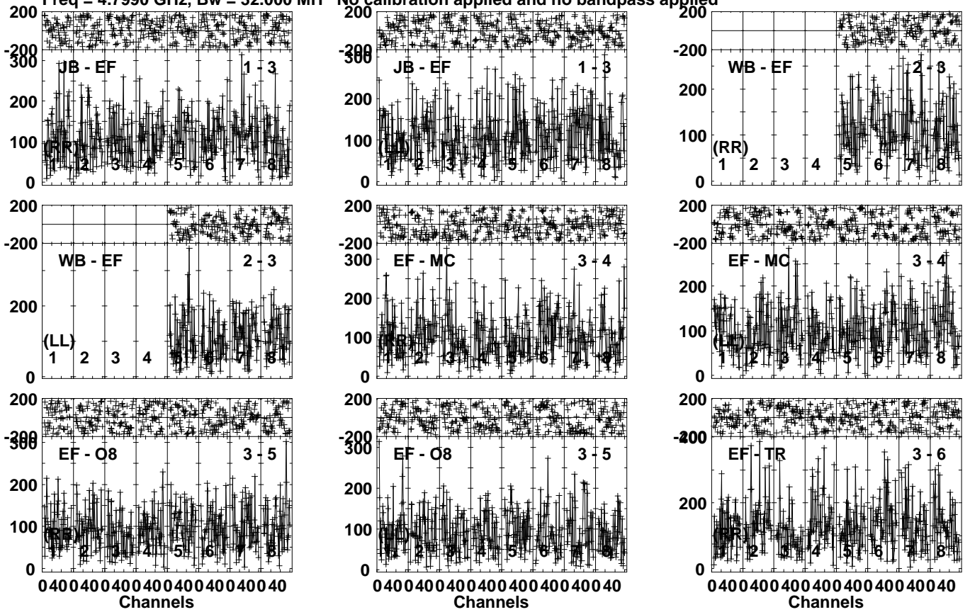
Lower frame: Micro Ampl Jy Top frame: Phas deg Vector averaged cross-power spectrum Several baselines displayed Timerange: 00/12:16:11 to 00/12:18:09
