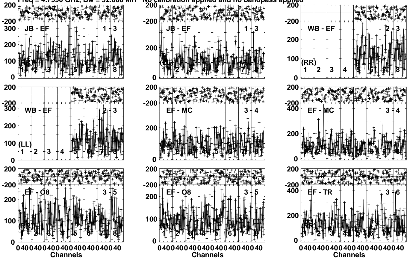
Lower frame: Micro Ampl Jy Top frame: Phas deg Vector averaged cross-power spectrum Several baselines displayed Timerange: 00/11:08:21 to 00/11:10:19
