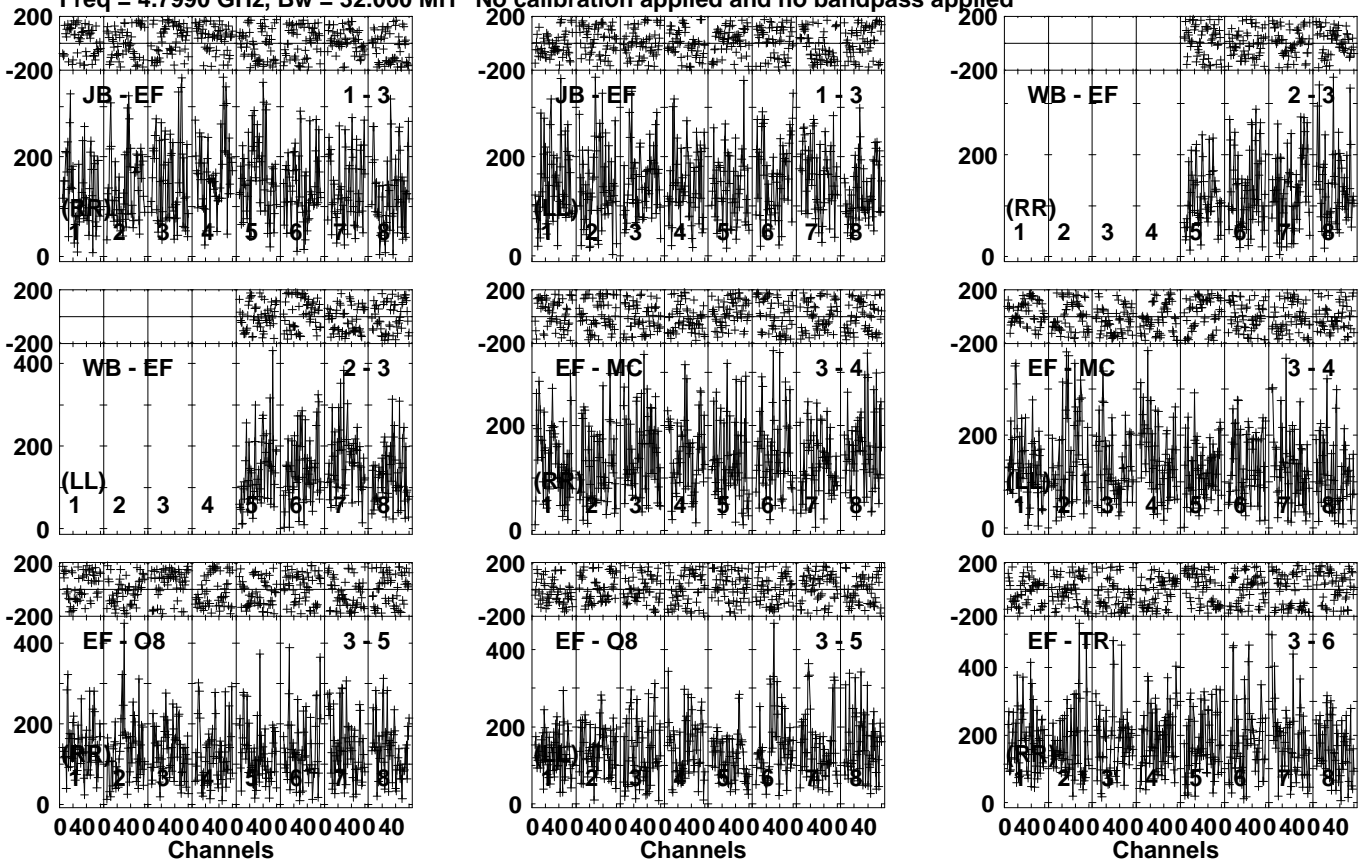
Lower frame: Micro Ampl Jy Top frame: Phas deg Vector averaged cross-power spectrum Several baselines displayed Timerange: 00/11:50:41 to 00/11:51:39
