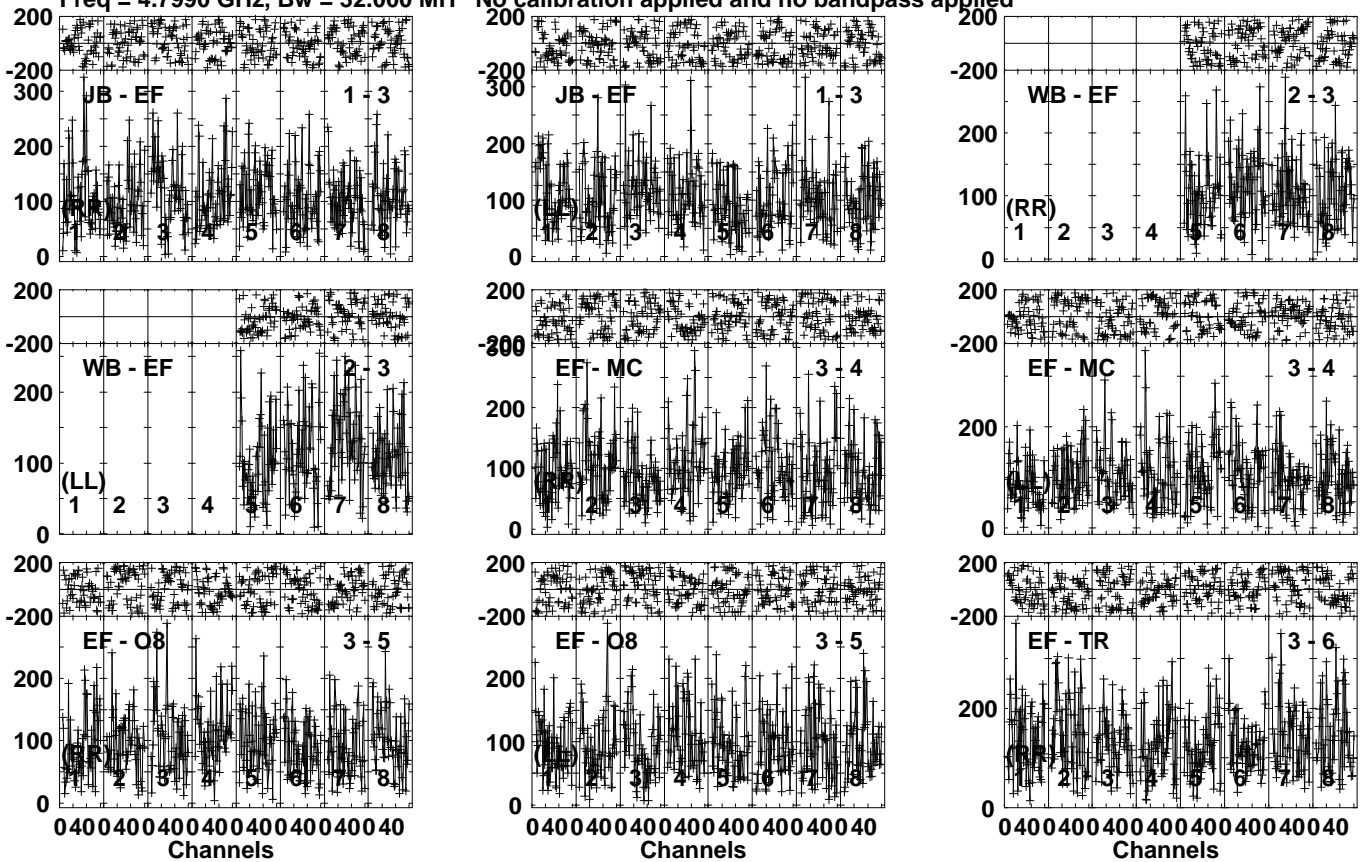
Lower frame: Micro Ampl Jy Top frame: Phas deg Vector averaged cross-power spectrum Several baselines displayed Timerange: 00/11:18:51 to 00/11:20:49
