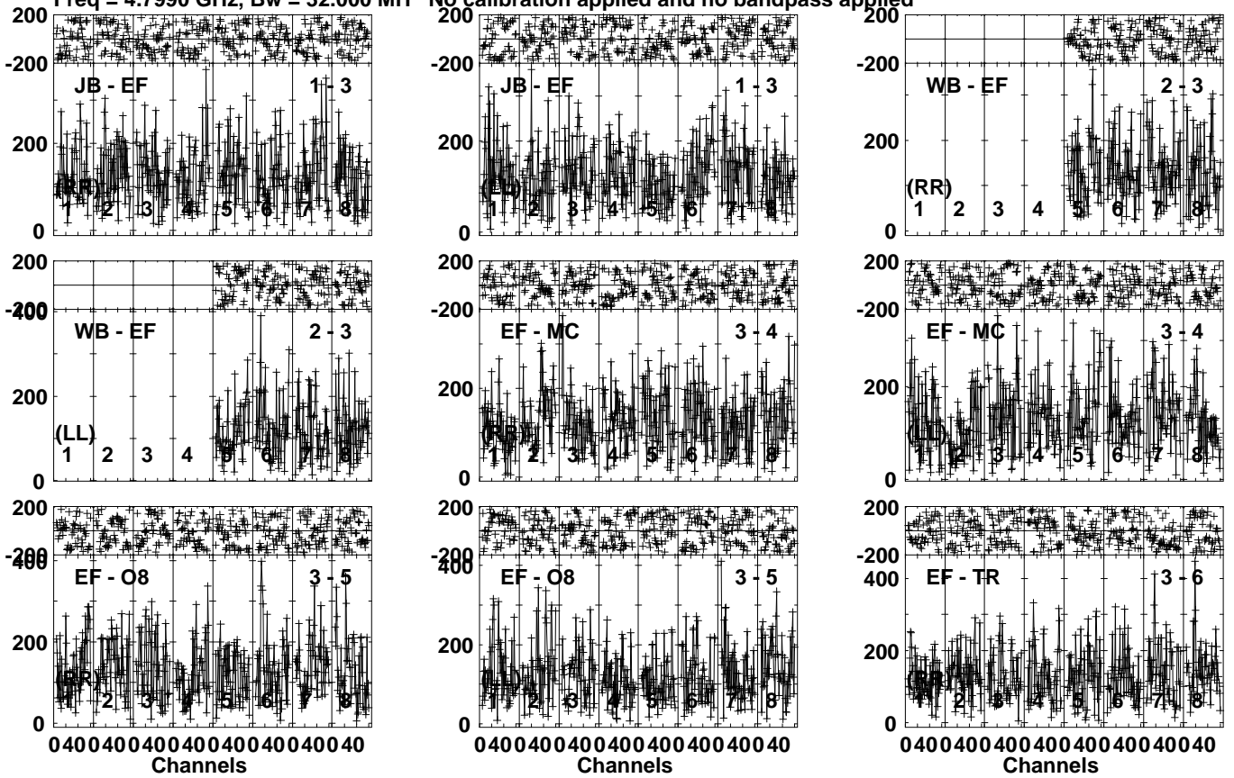
Lower frame: Micro Ampl Jy Top frame: Phas deg Vector averaged cross-power spectrum Several baselines displayed Timerange: 00/07:10:21 to 00/07:12:19
