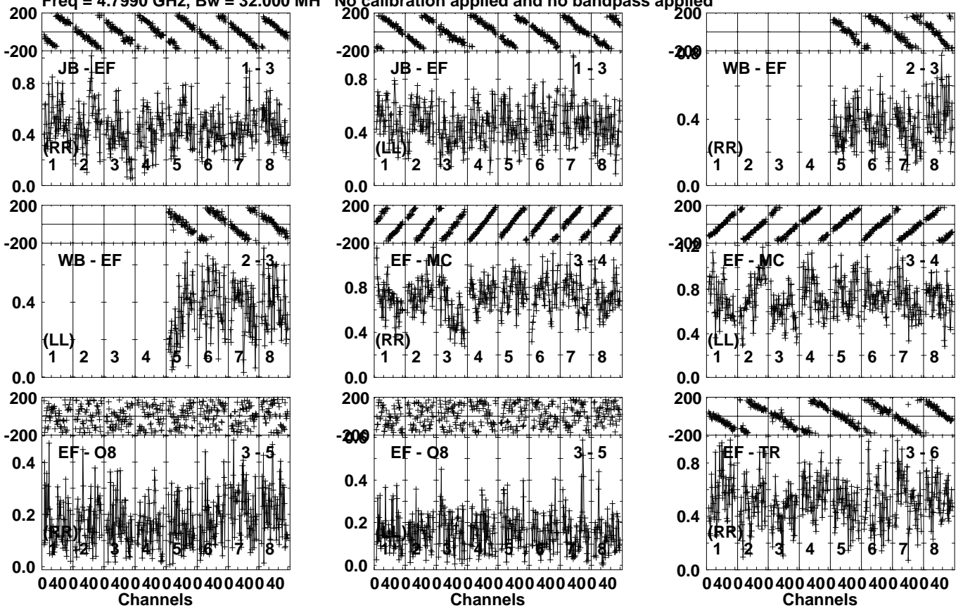
Lower frame: Milli Ampl Jy Top frame: Phas deg Vector averaged cross-power spectrum Several baselines displayed Timerange: 00/09:17:31 to 00/09:18:29
