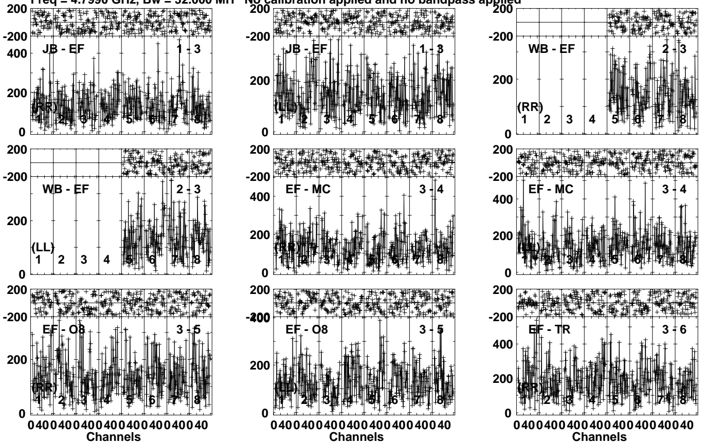
Lower frame: Micro Ampl Jy Top frame: Phas deg Vector averaged cross-power spectrum Several baselines displayed Timerange: 00/12:50:11 to 00/12:51:09
