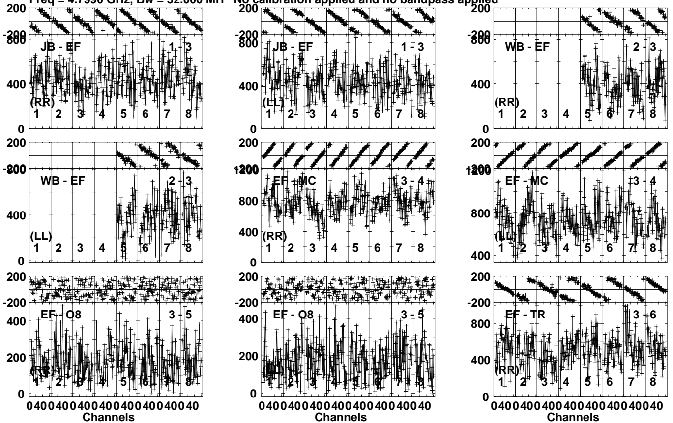
Lower frame: Micro Ampl Jy Top frame: Phas deg Vector averaged cross-power spectrum Several baselines displayed Timerange: 00/09:38:31 to 00/09:39:29
