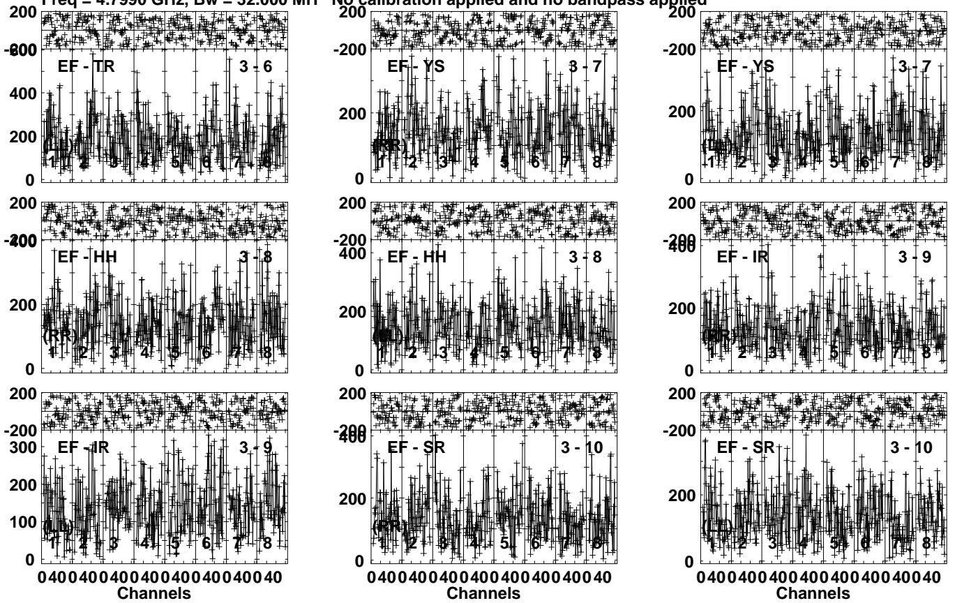
Lower frame: Micro Ampl Jy Top frame: Phas deg Vector averaged cross-power spectrum Several baselines displayed Timerange: 00/11:31:51 to 00/11:32:49
