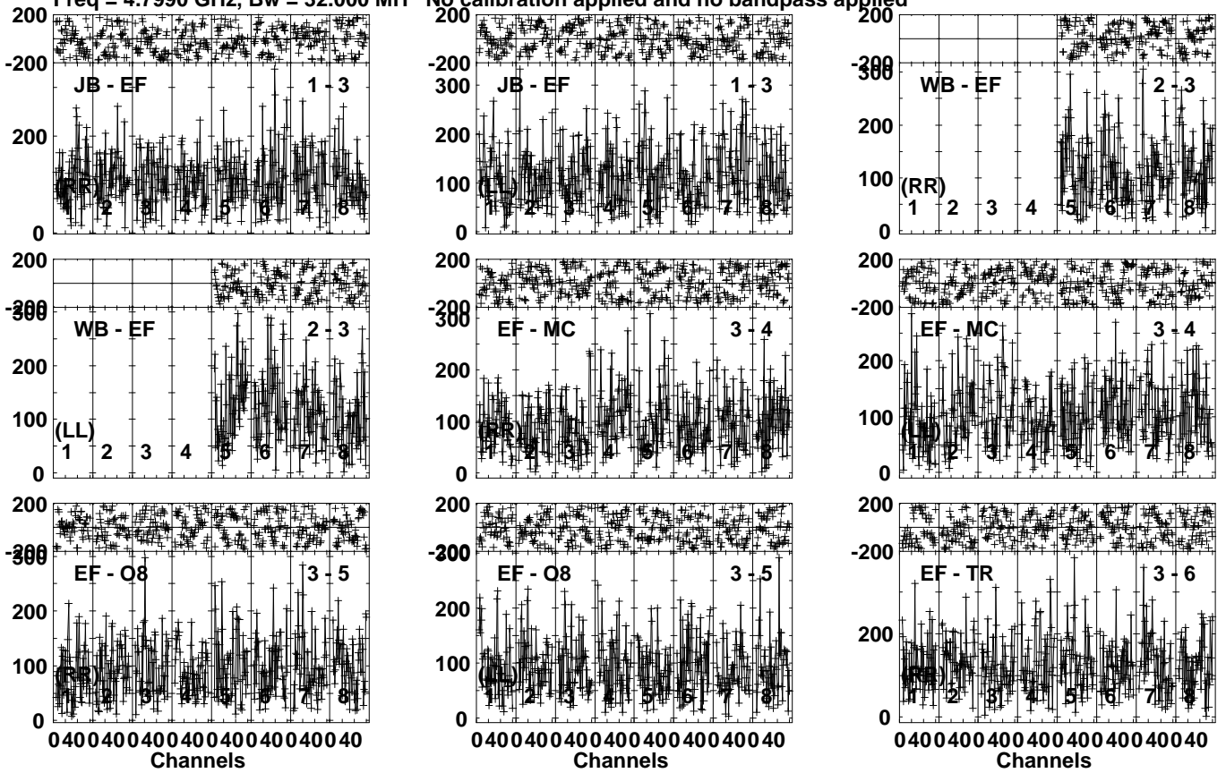
Lower frame: Micro Ampl Jy Top frame: Phas deg Vector averaged cross-power spectrum Several baselines displayed Timerange: 00/12:33:41 to 00/12:35:39
