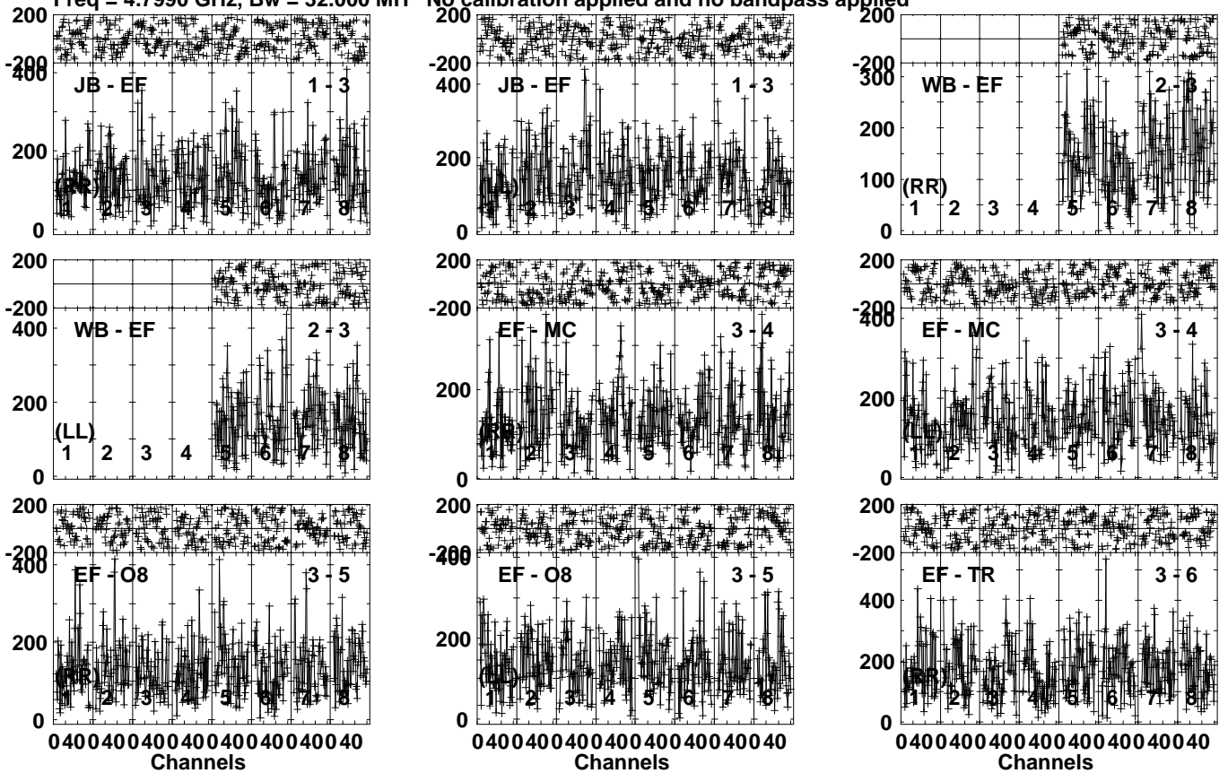
Lower frame: Micro Ampl Jy Top frame: Phas deg Vector averaged cross-power spectrum Several baselines displayed Timerange: 00/11:17:51 to 00/11:18:49
