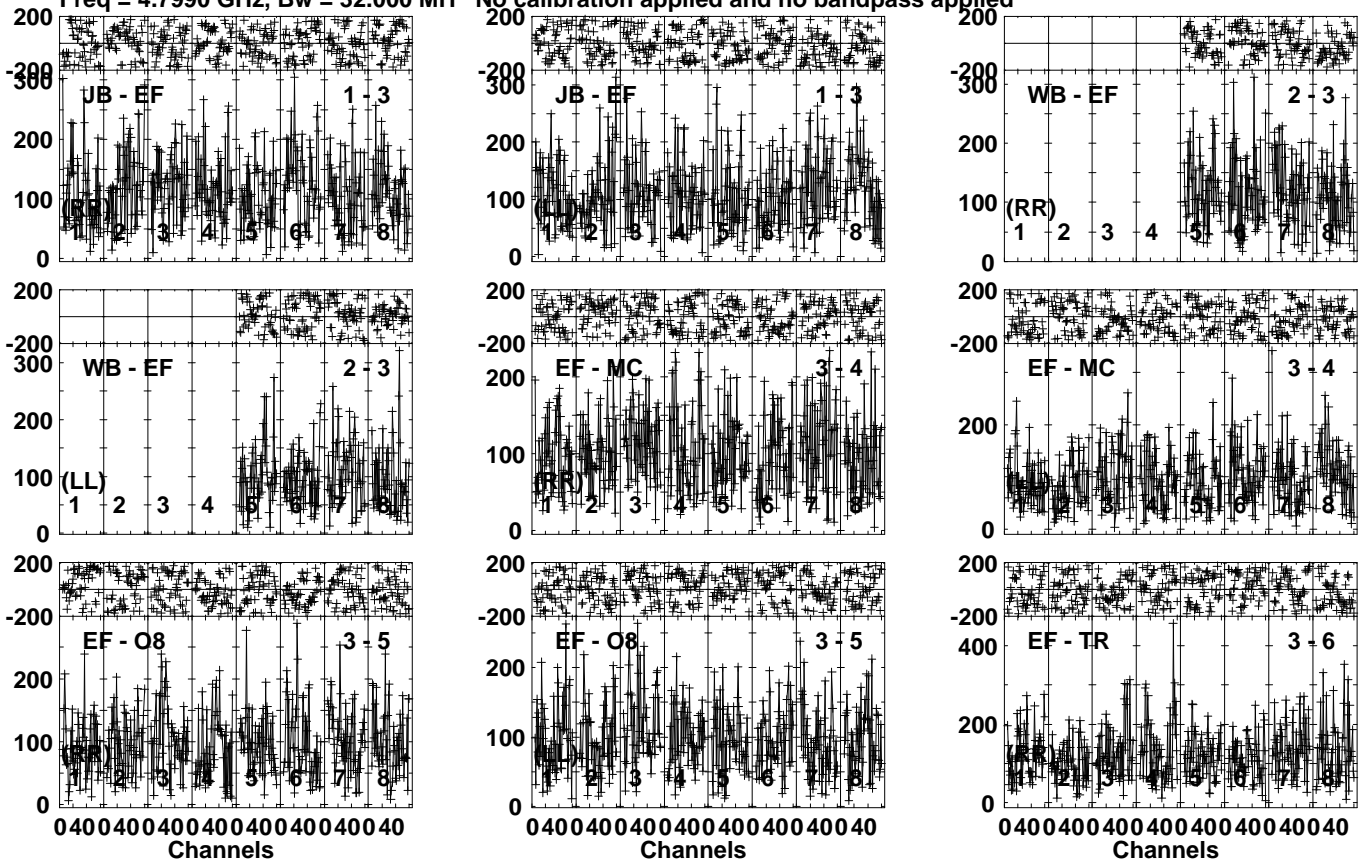
Lower frame: Micro Ampl Jy Top frame: Phas deg Vector averaged cross-power spectrum Several baselines displayed Timerange: 00/12:05:41 to 00/12:07:39
