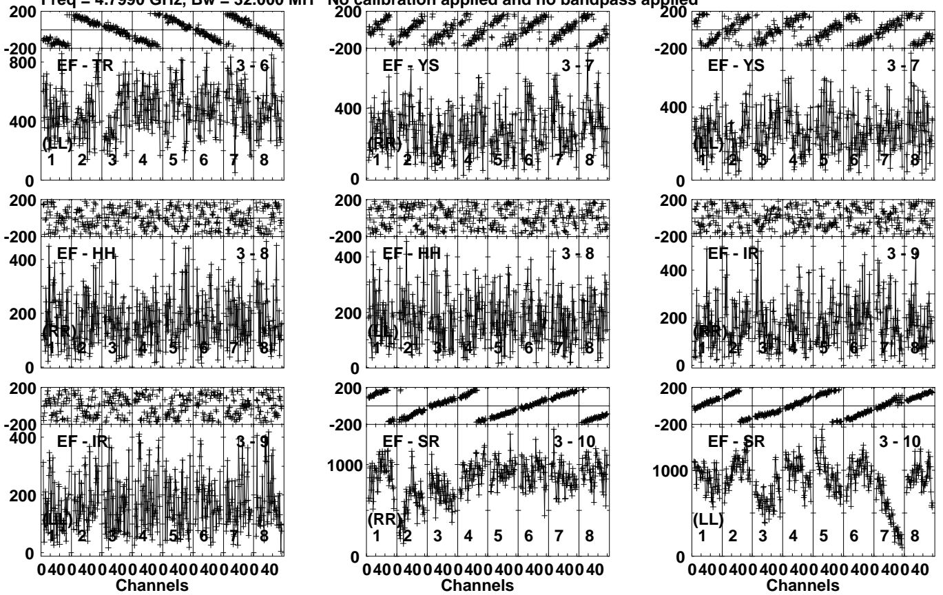
Lower frame: Micro Ampl Jy Top frame: Phas deg Vector averaged cross-power spectrum Several baselines displayed Timerange: 00/08:13:41 to 00/08:14:39
