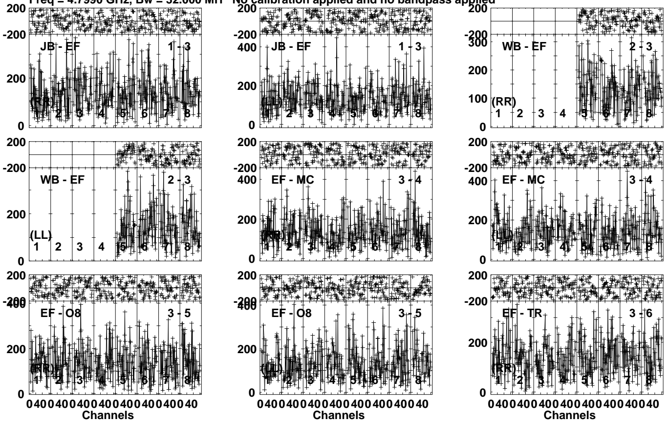
Lower frame: Micro Ampl Jy Top frame: Phas deg Vector averaged cross-power spectrum Several baselines displayed Timerange: 00/10:11:01 to 00/10:12:59
