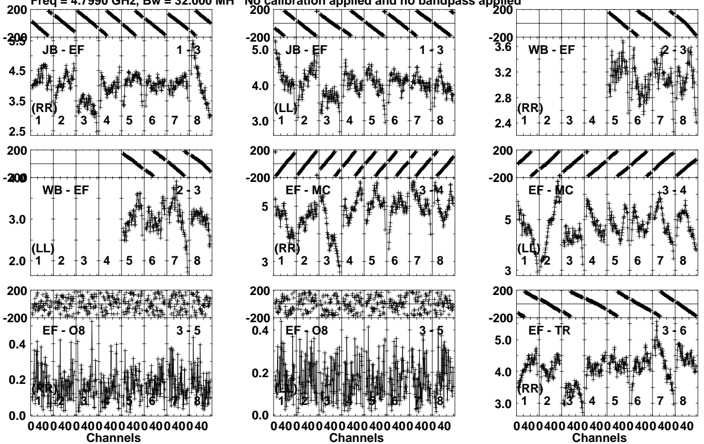
Lower frame: Milli Ampl Jy Top frame: Phas deg Vector averaged cross-power spectrum Several baselines displayed Timerange: 00/09:06:41 to 00/09:07:59
