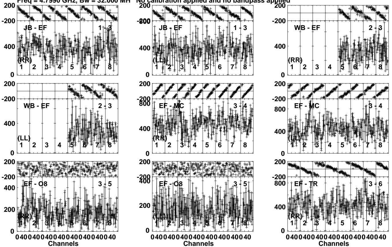
Lower frame: Micro Ampl Jy Top frame: Phas deg Vector averaged cross-power spectrum Several baselines displayed Timerange: 00/07:45:41 to 00/07:46:39
