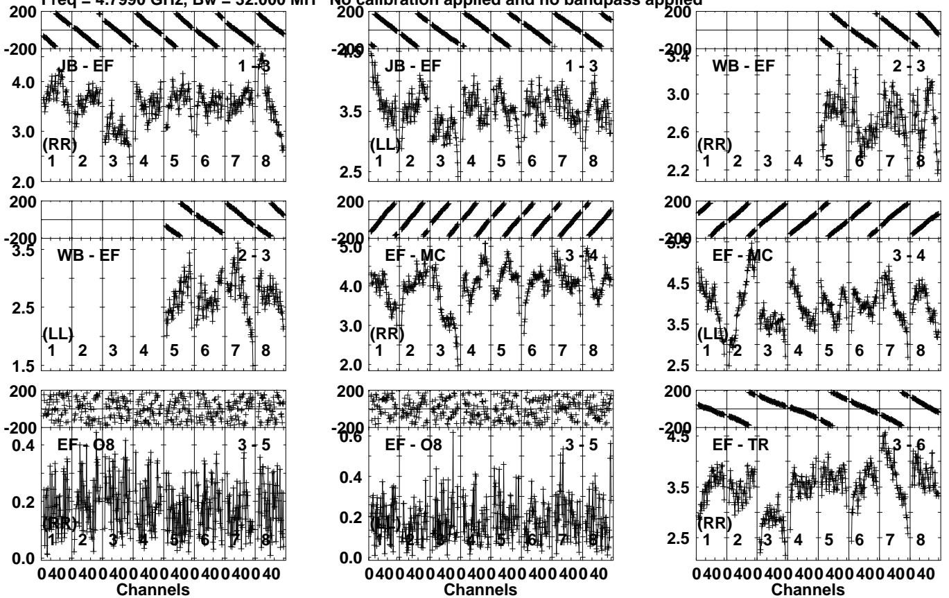
Lower frame: Milli Ampl Jy Top frame: Phas deg Vector averaged cross-power spectrum Several baselines displayed Timerange: 00/07:26:51 to 00/07:27:49
