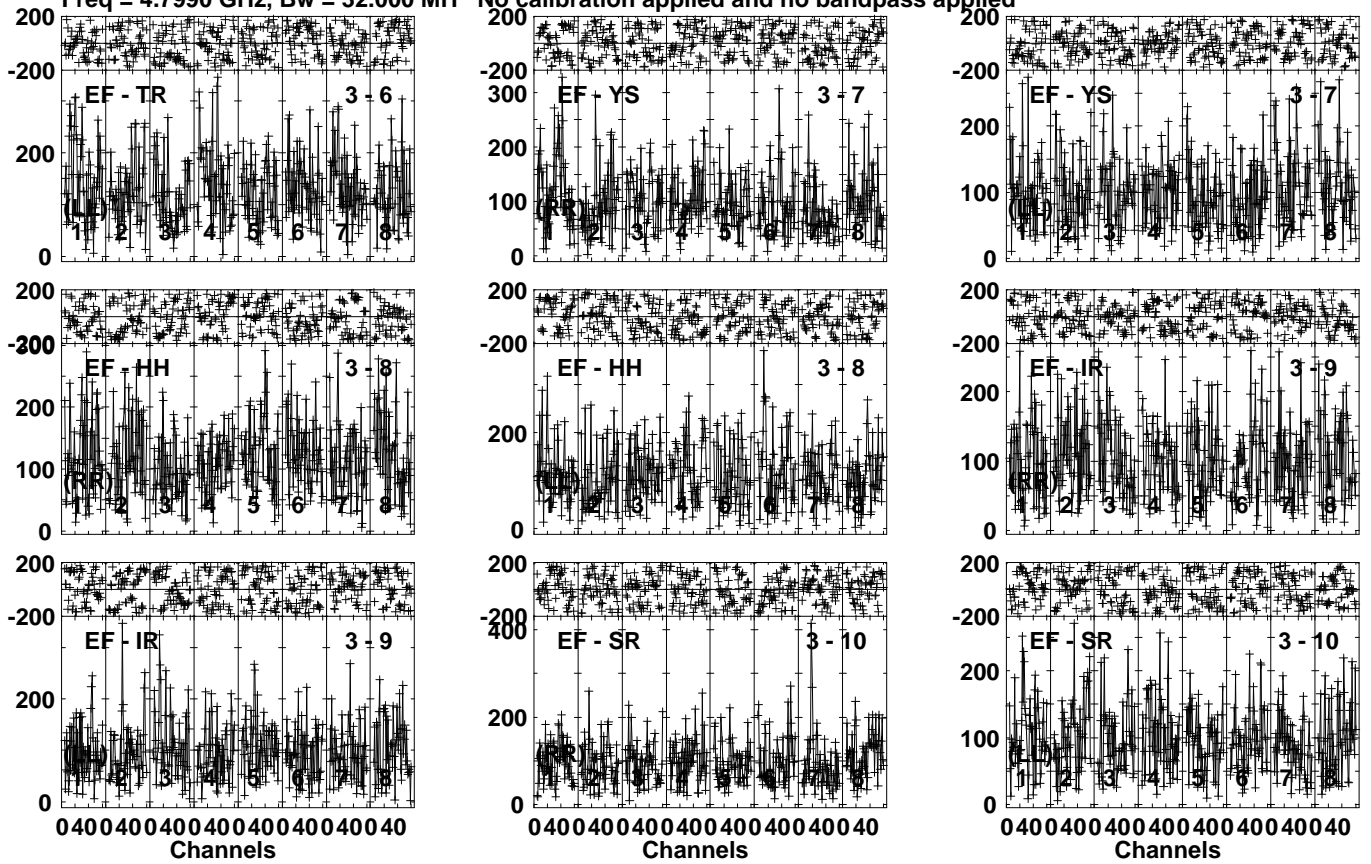
Lower frame: Micro Ampl Jy Top frame: Phas deg Vector averaged cross-power spectrum Several baselines displayed Timerange: 00/11:25:51 to 00/11:27:49
