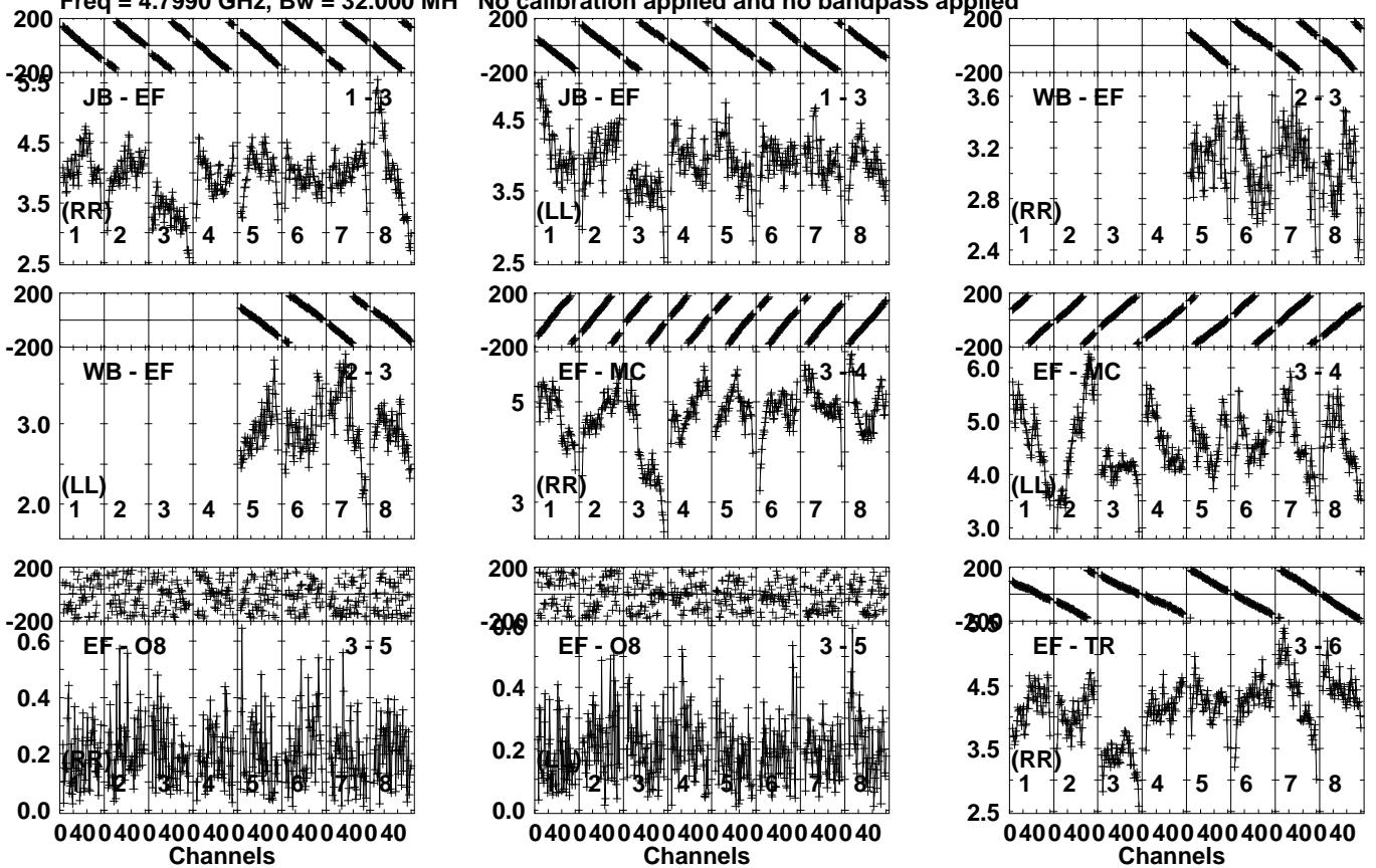
Lower frame: Milli Ampl Jy Top frame: Phas deg Vector averaged cross-power spectrum Several baselines displayed Timerange: 00/08:31:11 to 00/08:32:09
