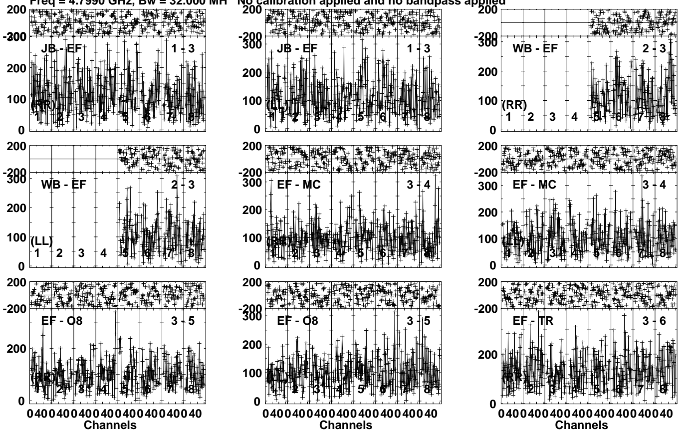
Lower frame: Micro Ampl Jy Top frame: Phas deg Vector averaged cross-power spectrum Several baselines displayed Timerange: 00/12:09:11 to 00/12:11:09
