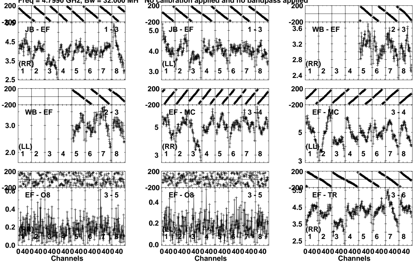
Lower frame: Milli Ampl Jy Top frame: Phas deg Vector averaged cross-power spectrum Several baselines displayed Timerange: 00/10:03:01 to 00/10:03:59
