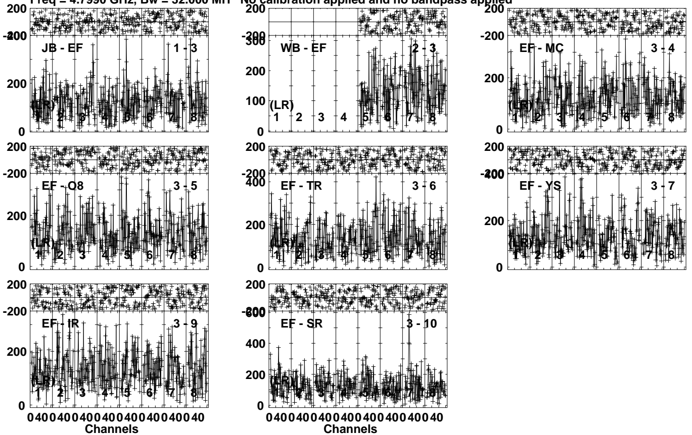
Lower frame: Micro Ampl Jy Top frame: Phas deg Vector averaged cross-power spectrum Several baselines displayed Timerange: 00/04:51:21 to 00/04:53:19
