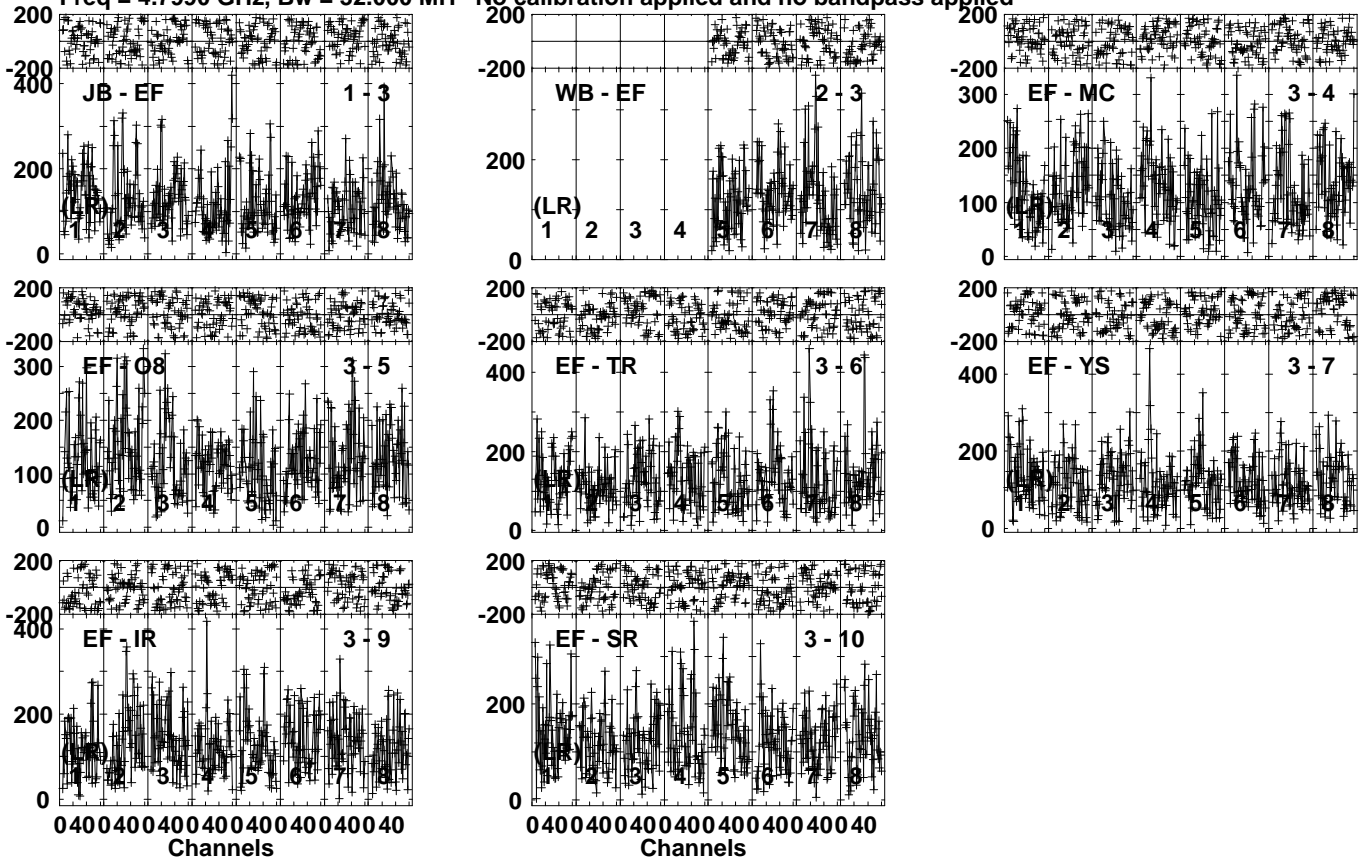
Lower frame: Micro Ampl Jy Top frame: Phas deg Vector averaged cross-power spectrum Several baselines displayed Timerange: 00/06:09:11 to 00/06:11:09
