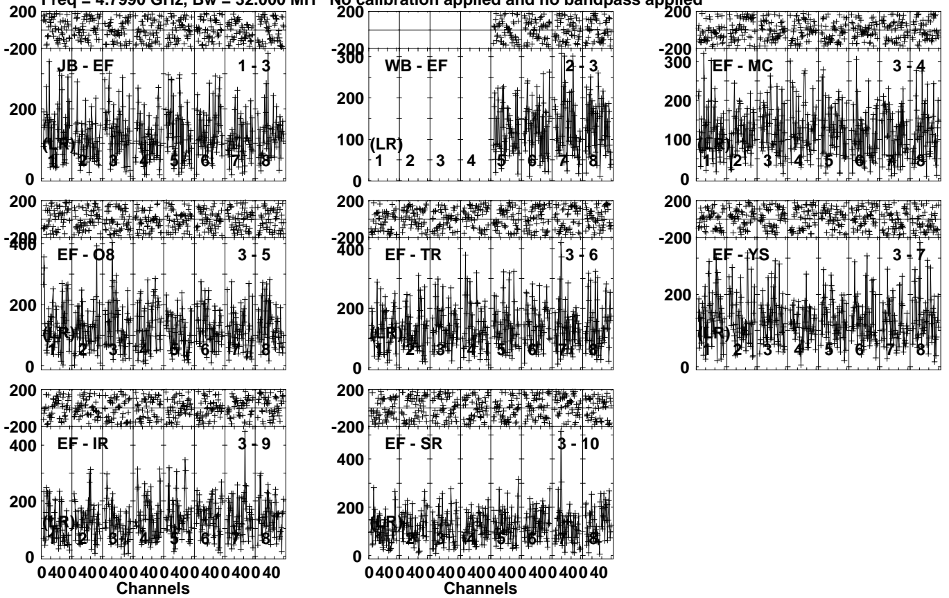
Lower frame: Micro Ampl Jy Top frame: Phas deg Vector averaged cross-power spectrum Several baselines displayed Timerange: 00/05:19:21 to 00/05:21:19
