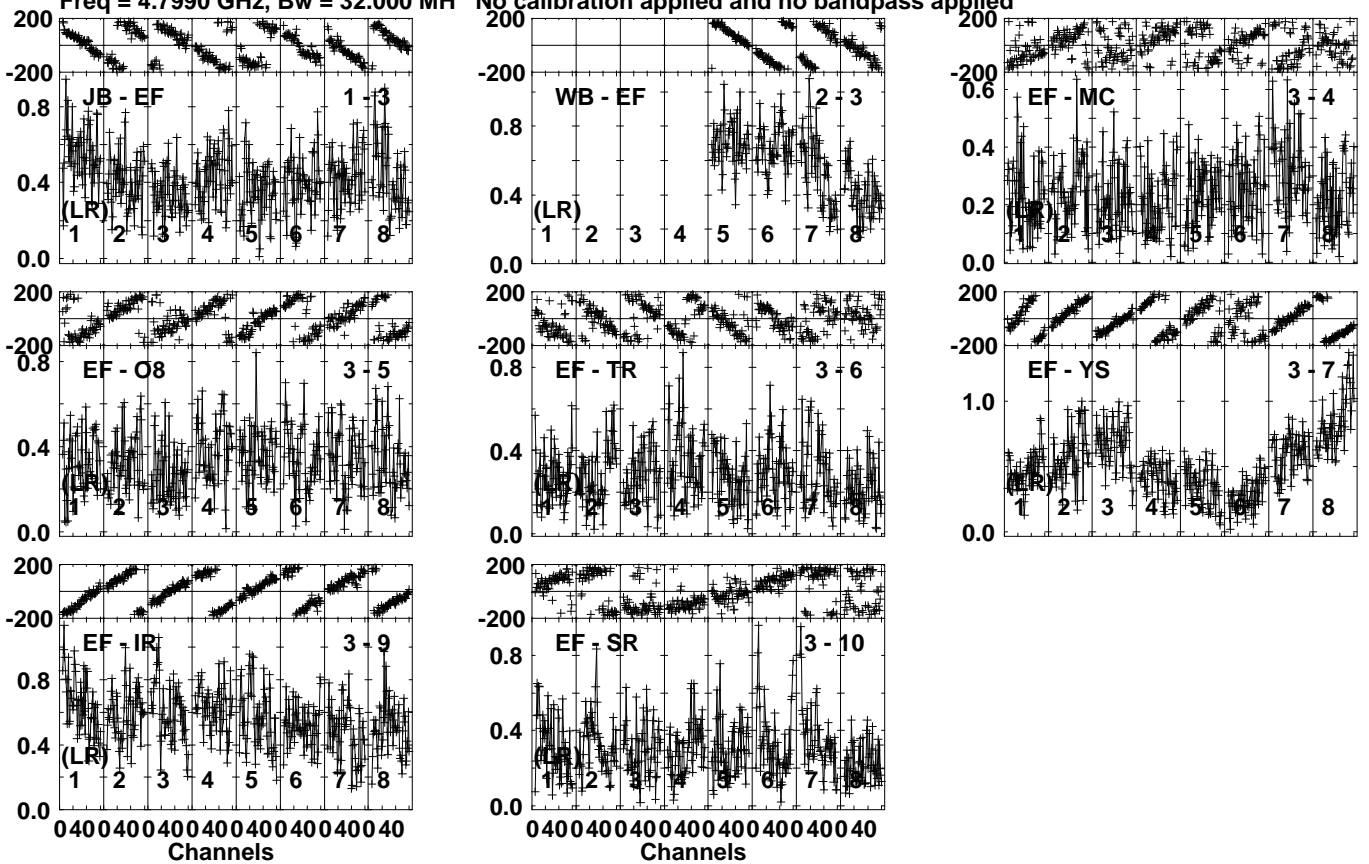
Lower frame: Milli Ampl Jy Top frame: Phas deg Vector averaged cross-power spectrum Several baselines displayed Timerange: 00/07:14:41 to 00/07:15:39
