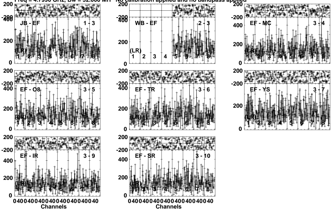
Lower frame: Micro Ampl Jy Top frame: Phas deg Vector averaged cross-power spectrum Several baselines displayed Timerange: 00/04:40:51 to 00/04:42:49
