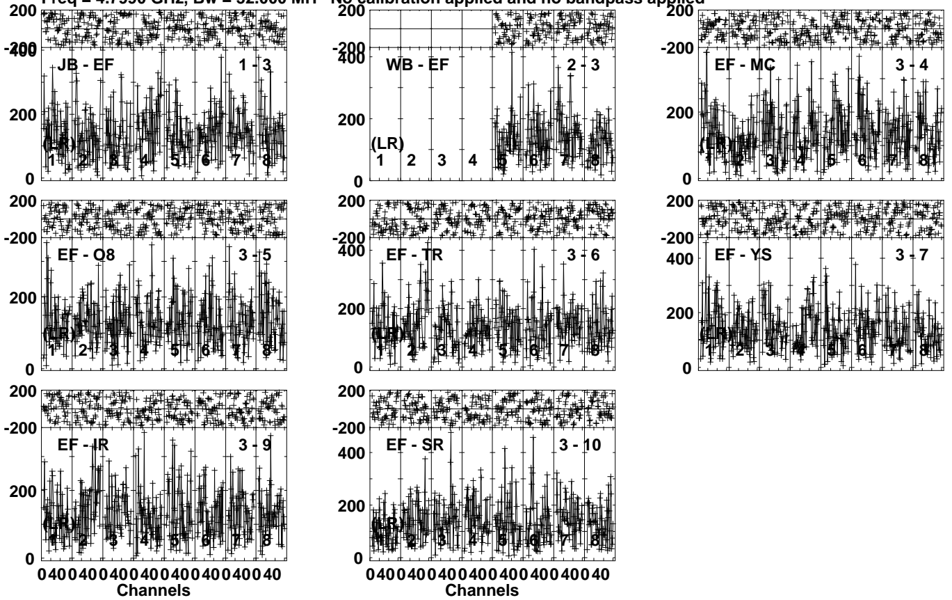
Lower frame: Micro Ampl Jy Top frame: Phas deg Vector averaged cross-power spectrum Several baselines displayed Timerange: 00/08:09:31 to 00/08:11:29
