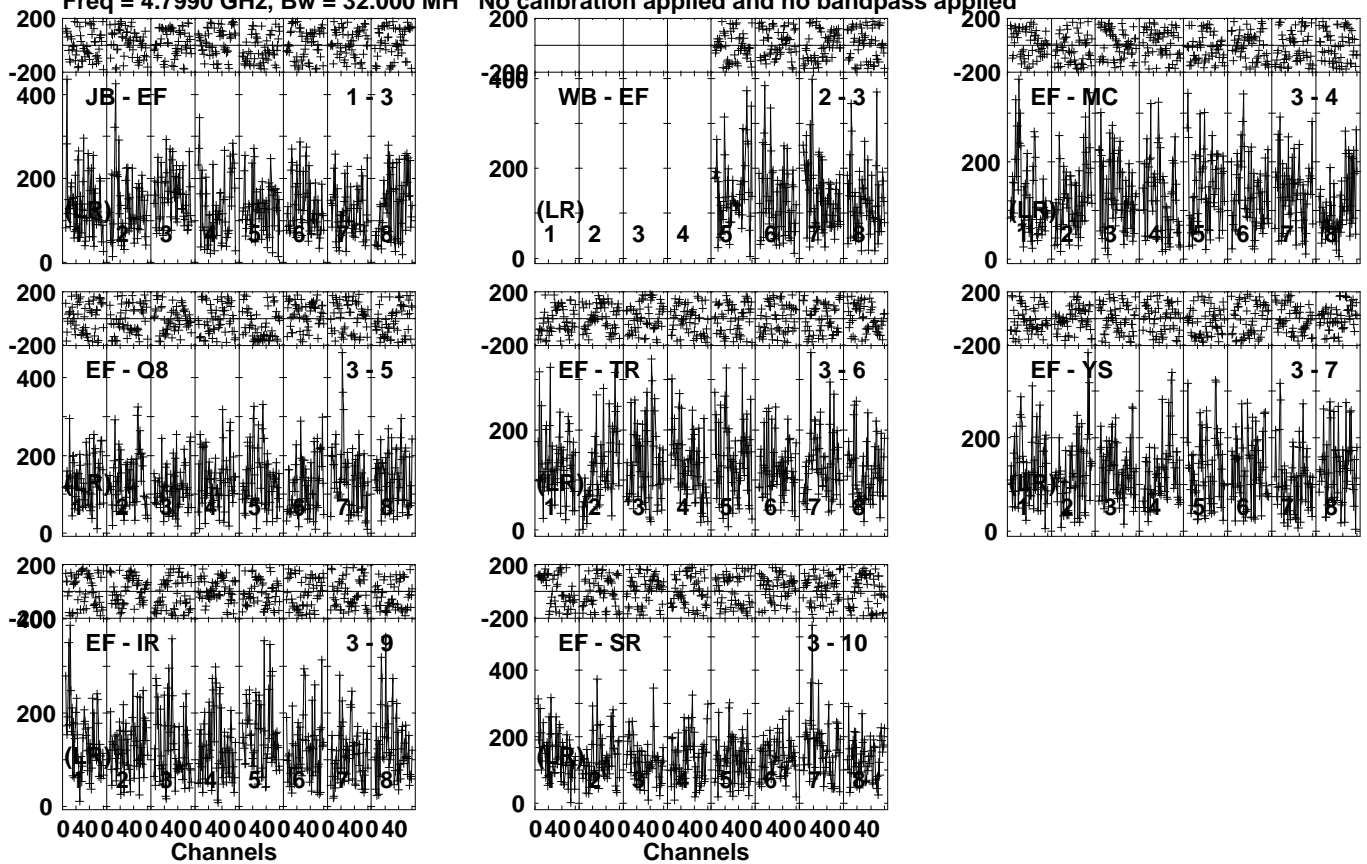
Lower frame: Micro Ampl Jy Top frame: Phas deg Vector averaged cross-power spectrum Several baselines displayed Timerange: 00/08:16:31 to 00/08:18:29
