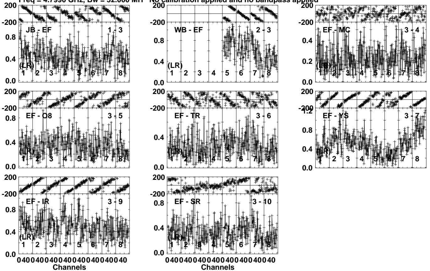
Lower frame: Milli Ampl Jy Top frame: Phas deg Vector averaged cross-power spectrum Several baselines displayed Timerange: 00/07:37:01 to 00/07:37:59
