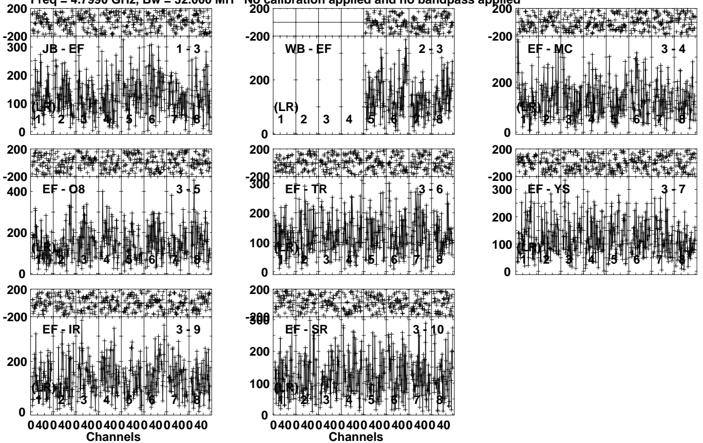
Lower frame: Micro Ampl Jy Top frame: Phas deg Vector averaged cross-power spectrum Several baselines displayed Timerange: 00/03:47:01 to 00/03:48:59
