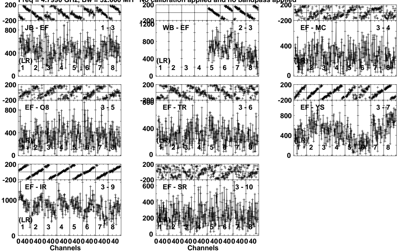
Lower frame: Micro Ampl Jy Top frame: Phas deg Vector averaged cross-power spectrum Several baselines displayed Timerange: 00/04:18:51 to 00/04:19:49
