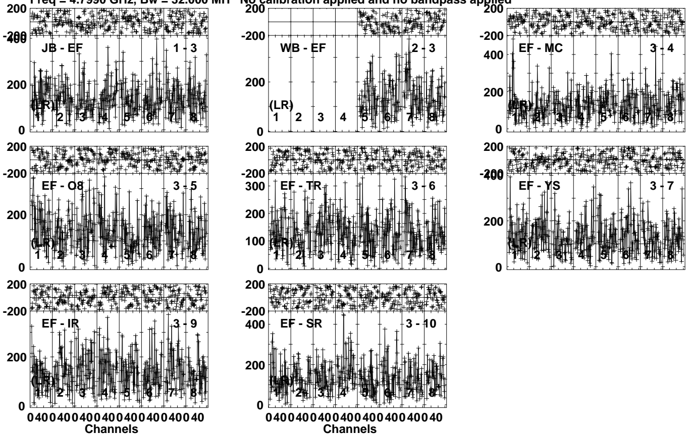
Lower frame: Micro Ampl Jy Top frame: Phas deg Vector averaged cross-power spectrum Several baselines displayed Timerange: 00/08:23:31 to 00/08:25:29
