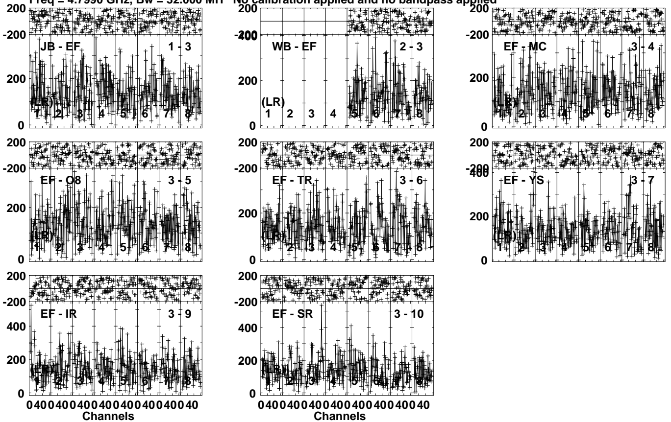
Lower frame: Micro Ampl Jy Top frame: Phas deg Vector averaged cross-power spectrum Several baselines displayed Timerange: 00/06:30:11 to 00/06:32:09
