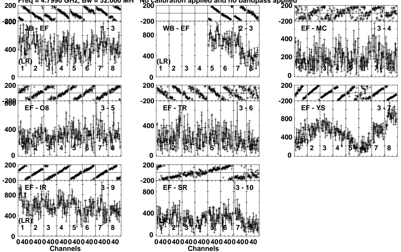
Lower frame: Micro Ampl Jy Top frame: Phas deg Vector averaged cross-power spectrum Several baselines displayed Timerange: 00/07:22:41 to 00/07:23:59
