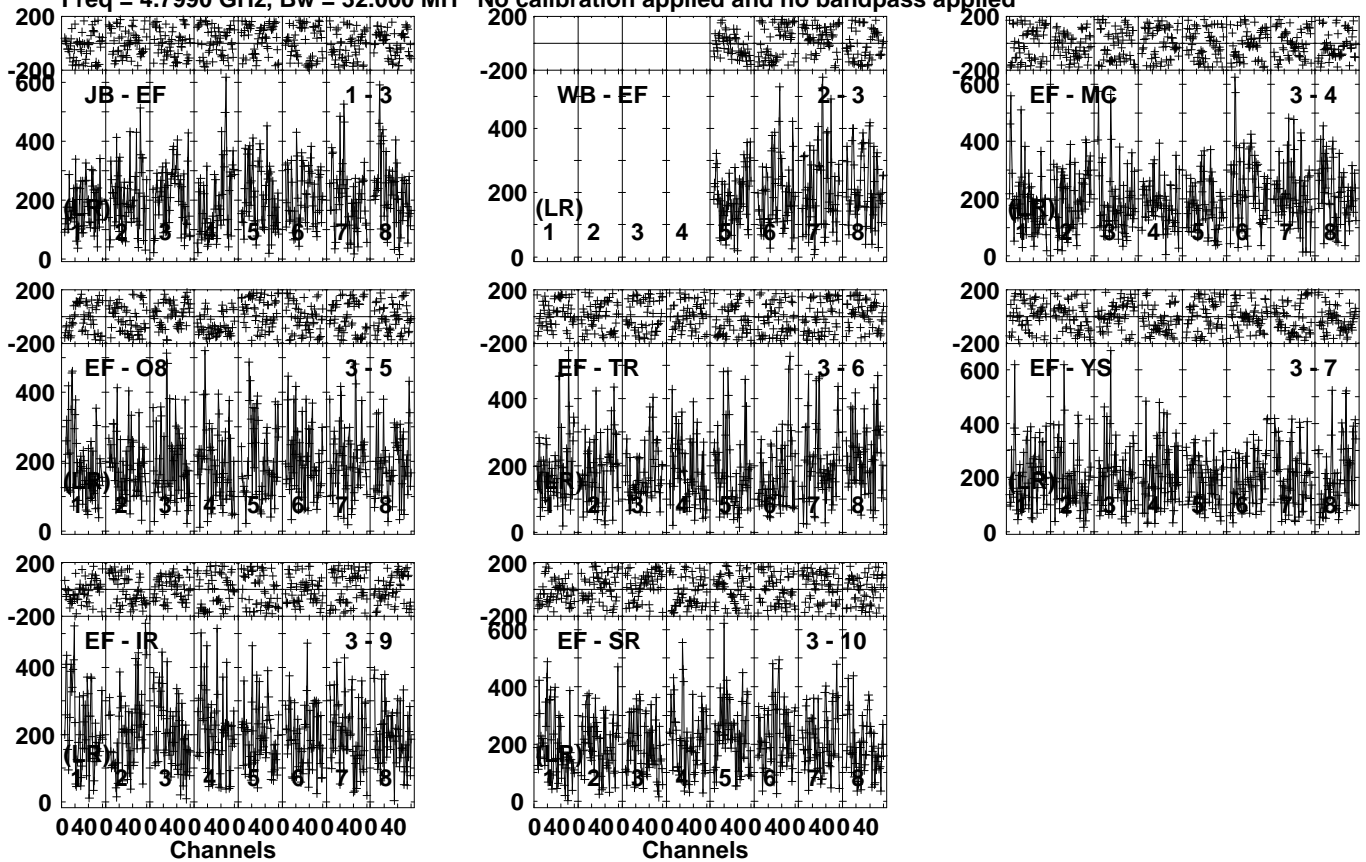
Lower frame: Micro Ampl Jy Top frame: Phas deg Vector averaged cross-power spectrum Several baselines displayed Timerange: 00/06:50:11 to 00/06:51:09
