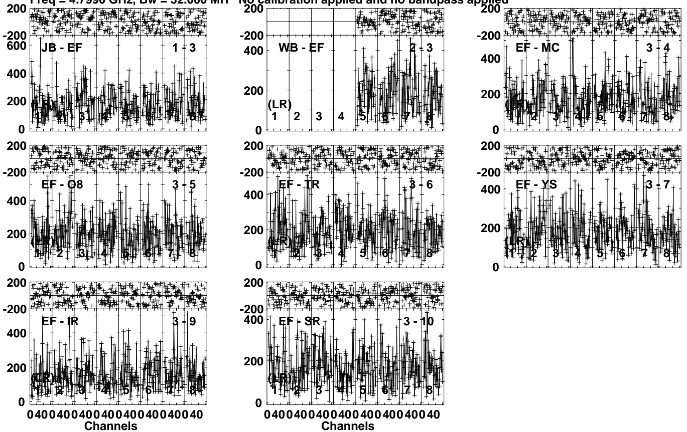
Lower frame: Micro Ampl Jy Top frame: Phas deg Vector averaged cross-power spectrum Several baselines displayed Timerange: 00/03:18:01 to 00/03:18:59
