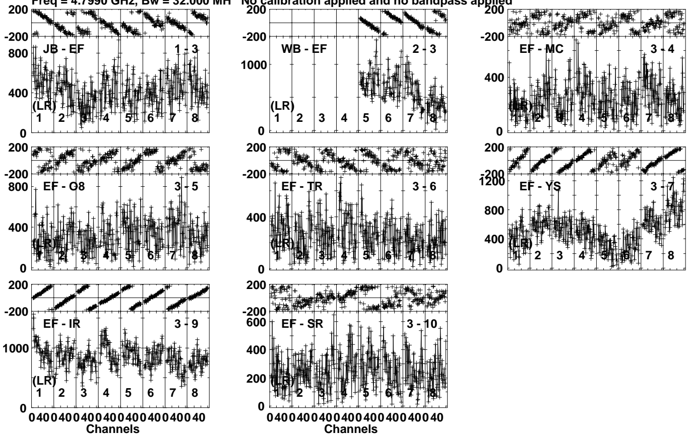
Lower frame: Micro Ampl Jy Top frame: Phas deg Vector averaged cross-power spectrum Several baselines displayed Timerange: 00/05:21:51 to 00/05:22:49
