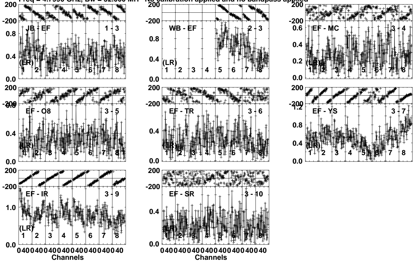
Lower frame: Milli Ampl Jy Top frame: Phas deg Vector averaged cross-power spectrum Several baselines displayed Timerange: 00/04:46:51 to 00/04:47:49
