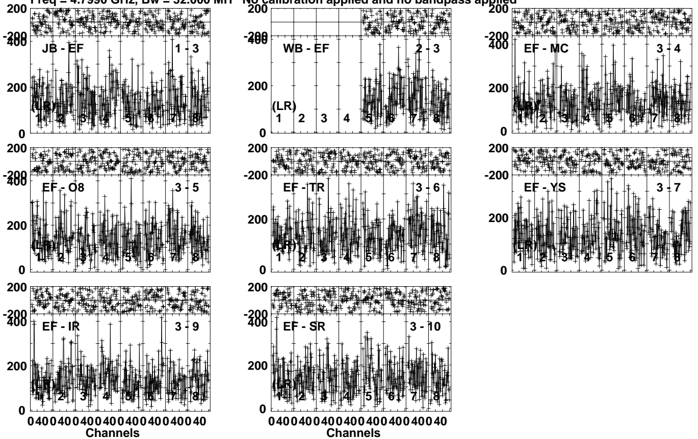
Lower frame: Micro Ampl Jy Top frame: Phas deg Vector averaged cross-power spectrum Several baselines displayed Timerange: 00/06:05:41 to 00/06:07:39
