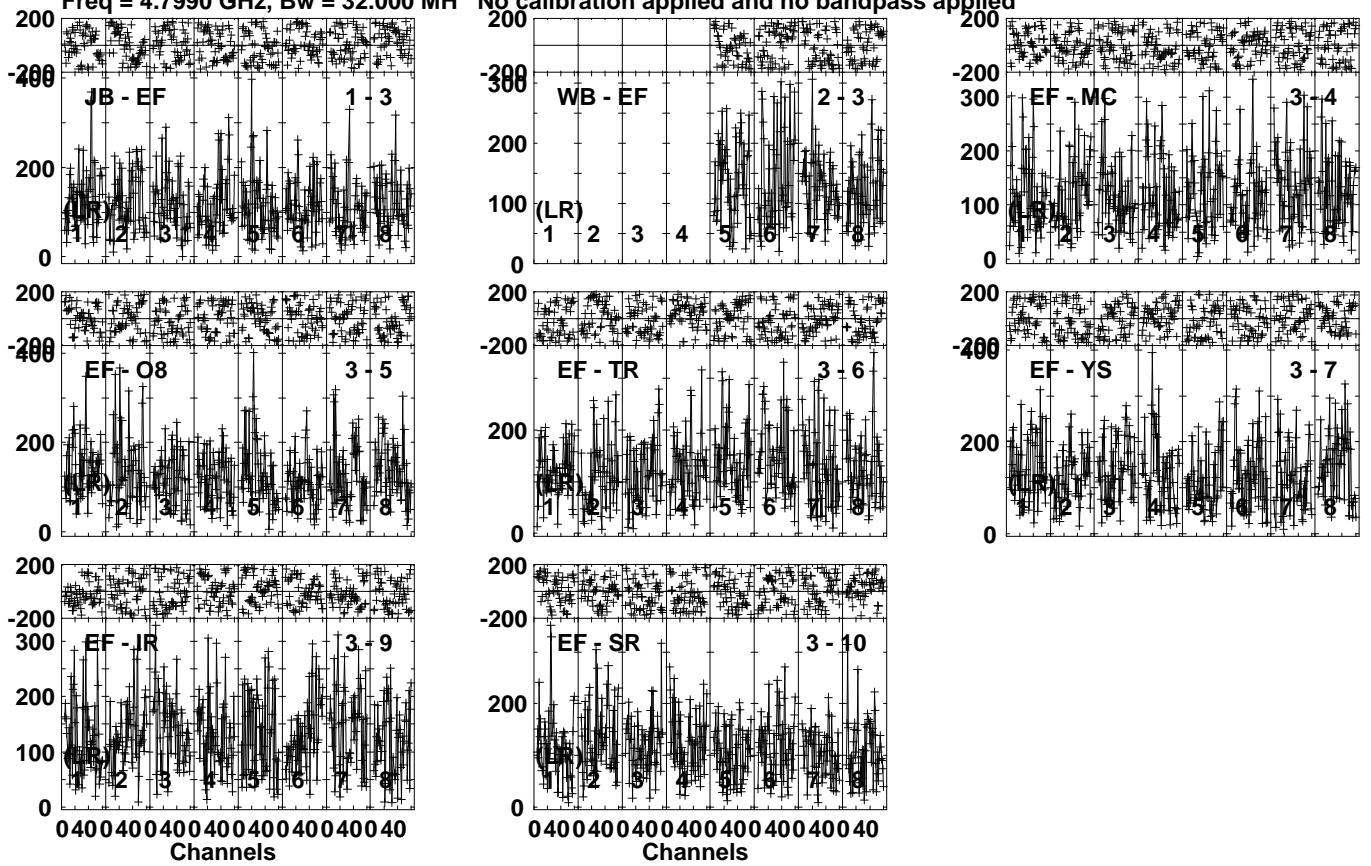
Lower frame: Micro Ampl Jy Top frame: Phas deg Vector averaged cross-power spectrum Several baselines displayed Timerange: 00/05:05:21 to 00/05:07:19
