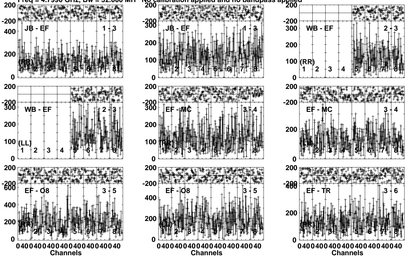
Lower frame: Micro Ampl Jy Top frame: Phas deg Vector averaged cross-power spectrum Several baselines displayed Timerange: 00/03:26:01 to 00/03:27:59
