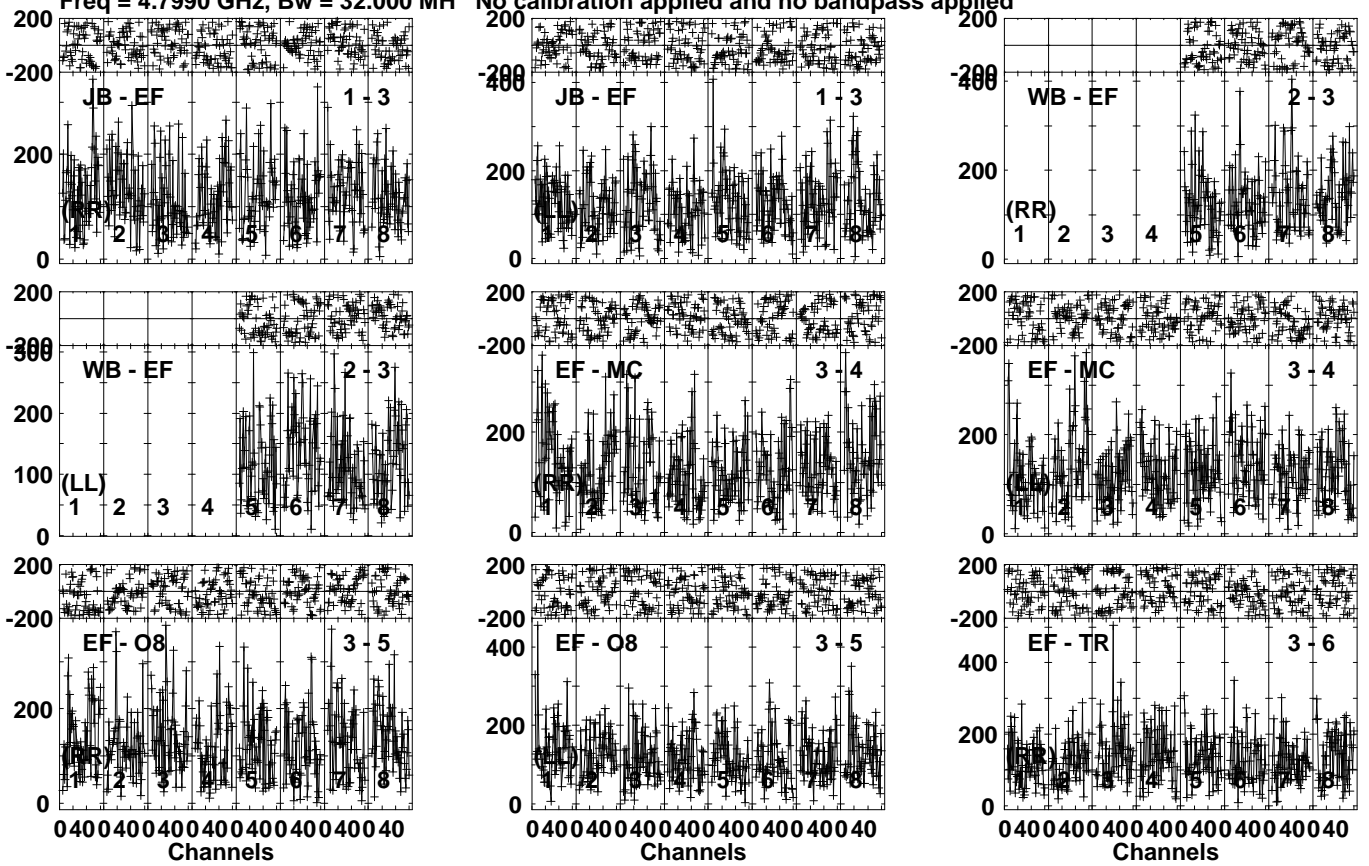
Lower frame: Micro Ampl Jy Top frame: Phas deg Vector averaged cross-power spectrum Several baselines displayed Timerange: 00/04:44:21 to 00/04:46:19
