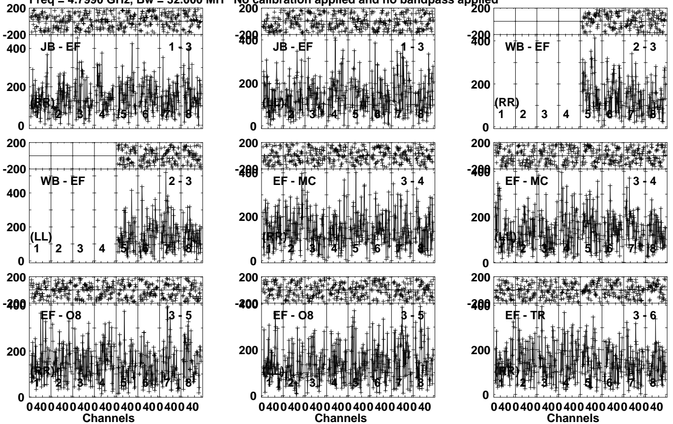
Lower frame: Micro Ampl Jy Top frame: Phas deg Vector averaged cross-power spectrum Several baselines displayed Timerange: 00/08:34:01 to 00/08:35:59
