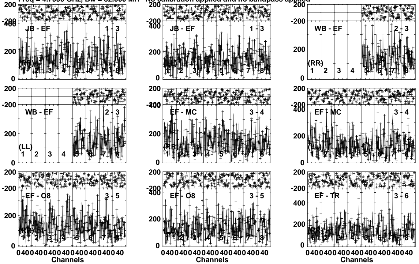
Lower frame: Micro Ampl Jy Top frame: Phas deg Vector averaged cross-power spectrum Several baselines displayed Timerange: 00/05:29:51 to 00/05:31:49
