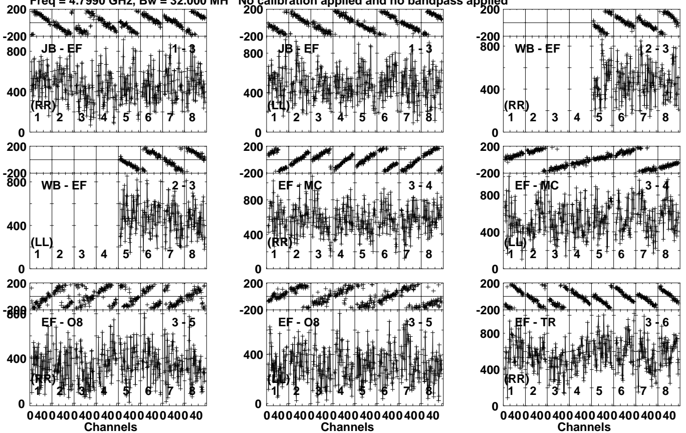
Lower frame: Micro Ampl Jy Top frame: Phas deg Vector averaged cross-power spectrum Several baselines displayed Timerange: 00/07:47:31 to 00/07:48:29
