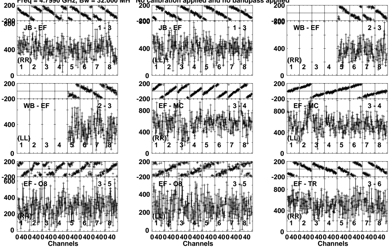
Lower frame: Micro Ampl Jy Top frame: Phas deg Vector averaged cross-power spectrum Several baselines displayed Timerange: 00/04:29:21 to 00/04:30:19
