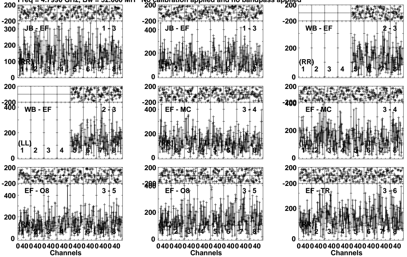
Lower frame: Micro Ampl Jy Top frame: Phas deg Vector averaged cross-power spectrum Several baselines displayed Timerange: 00/05:08:51 to 00/05:10:49
