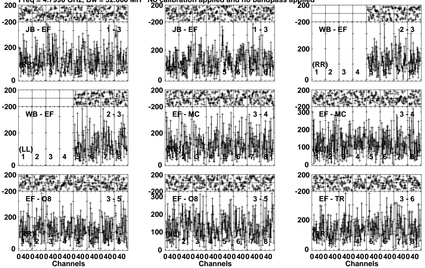
Lower frame: Micro Ampl Jy Top frame: Phas deg Vector averaged cross-power spectrum Several baselines displayed Timerange: 00/06:47:41 to 00/06:49:39
