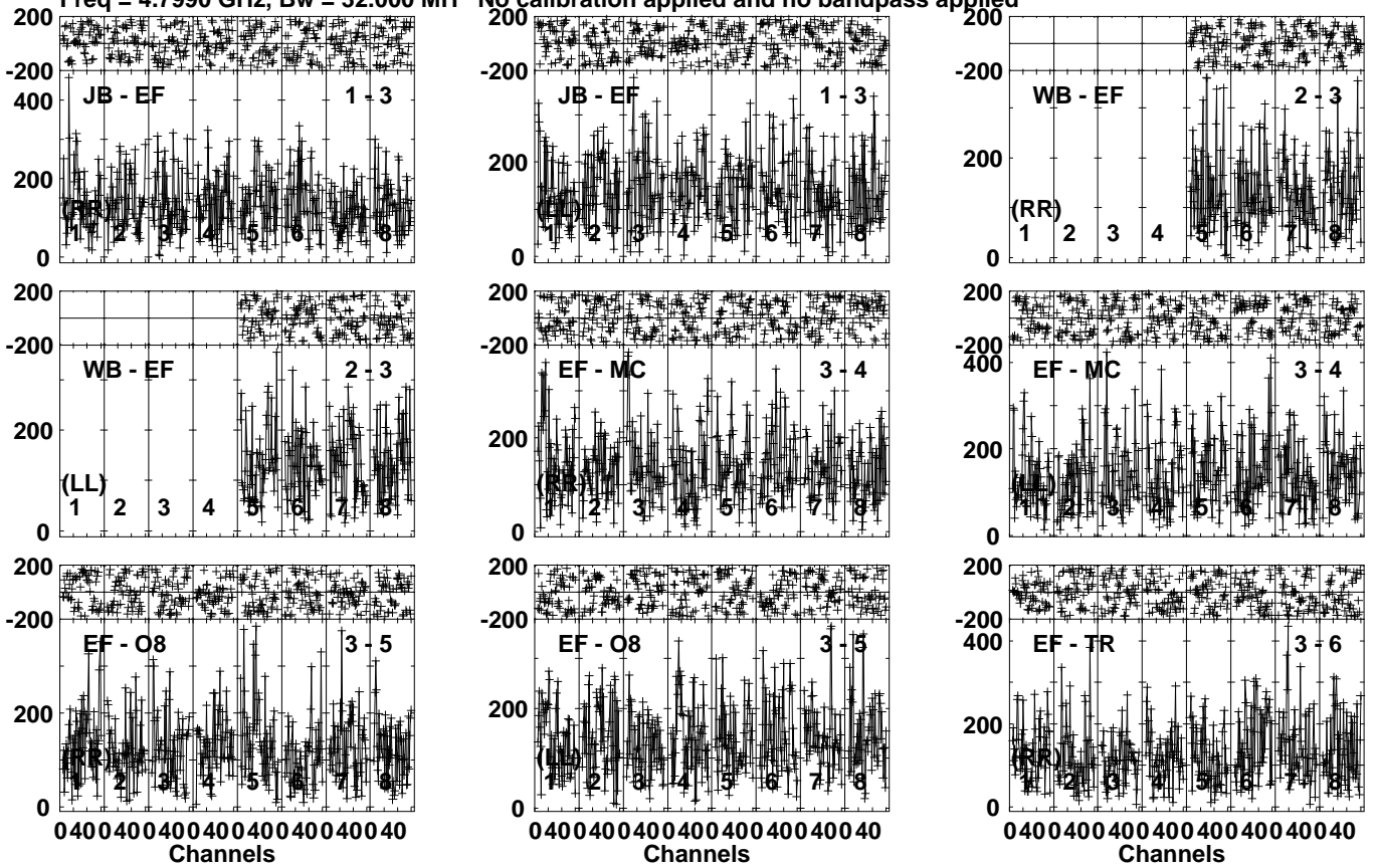
Lower frame: Micro Ampl Jy Top frame: Phas deg Vector averaged cross-power spectrum Several baselines displayed Timerange: 00/06:51:11 to 00/06:53:09
