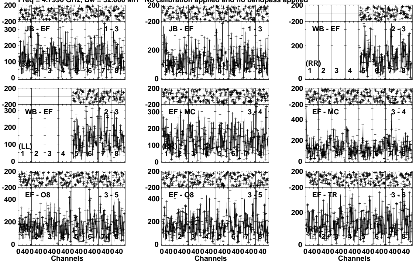
Lower frame: Micro Ampl Jy Top frame: Phas deg Vector averaged cross-power spectrum Several baselines displayed Timerange: 00/03:33:01 to 00/03:34:59
