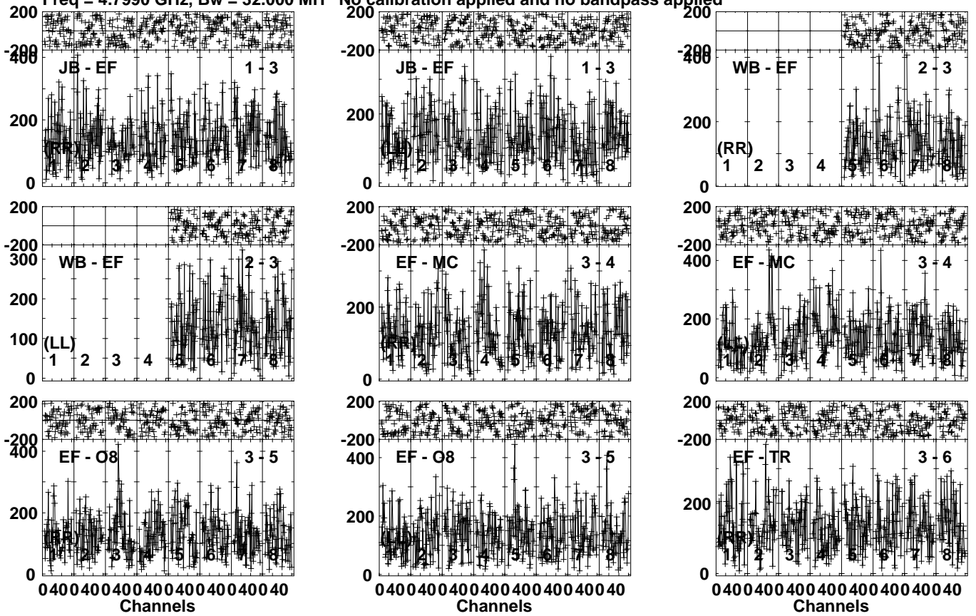
Lower frame: Micro Ampl Jy Top frame: Phas deg Vector averaged cross-power spectrum Several baselines displayed Timerange: 00/07:05:11 to 00/07:07:09
