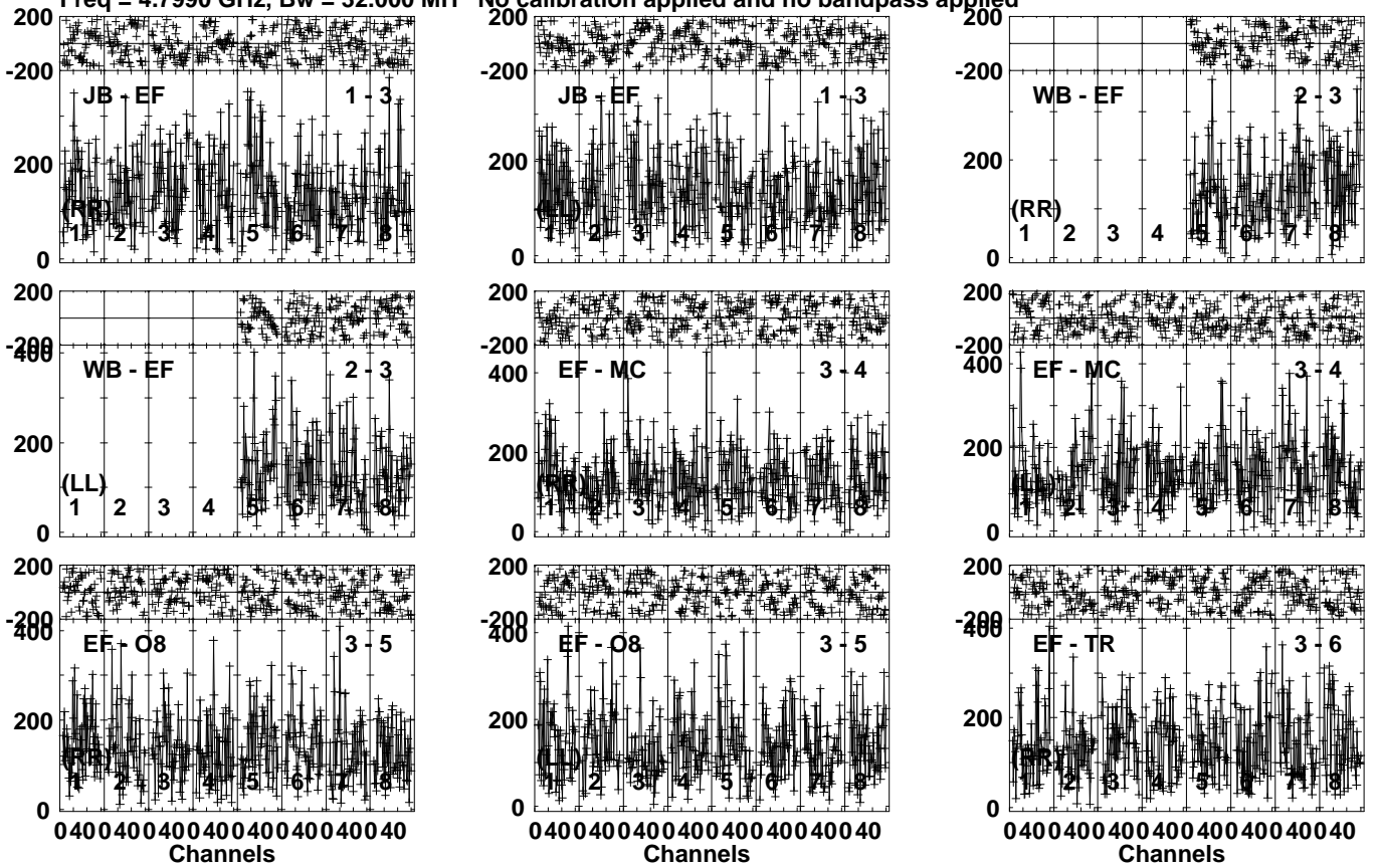
Lower frame: Micro Ampl Jy Top frame: Phas deg Vector averaged cross-power spectrum Several baselines displayed Timerange: 00/08:20:01 to 00/08:21:59
