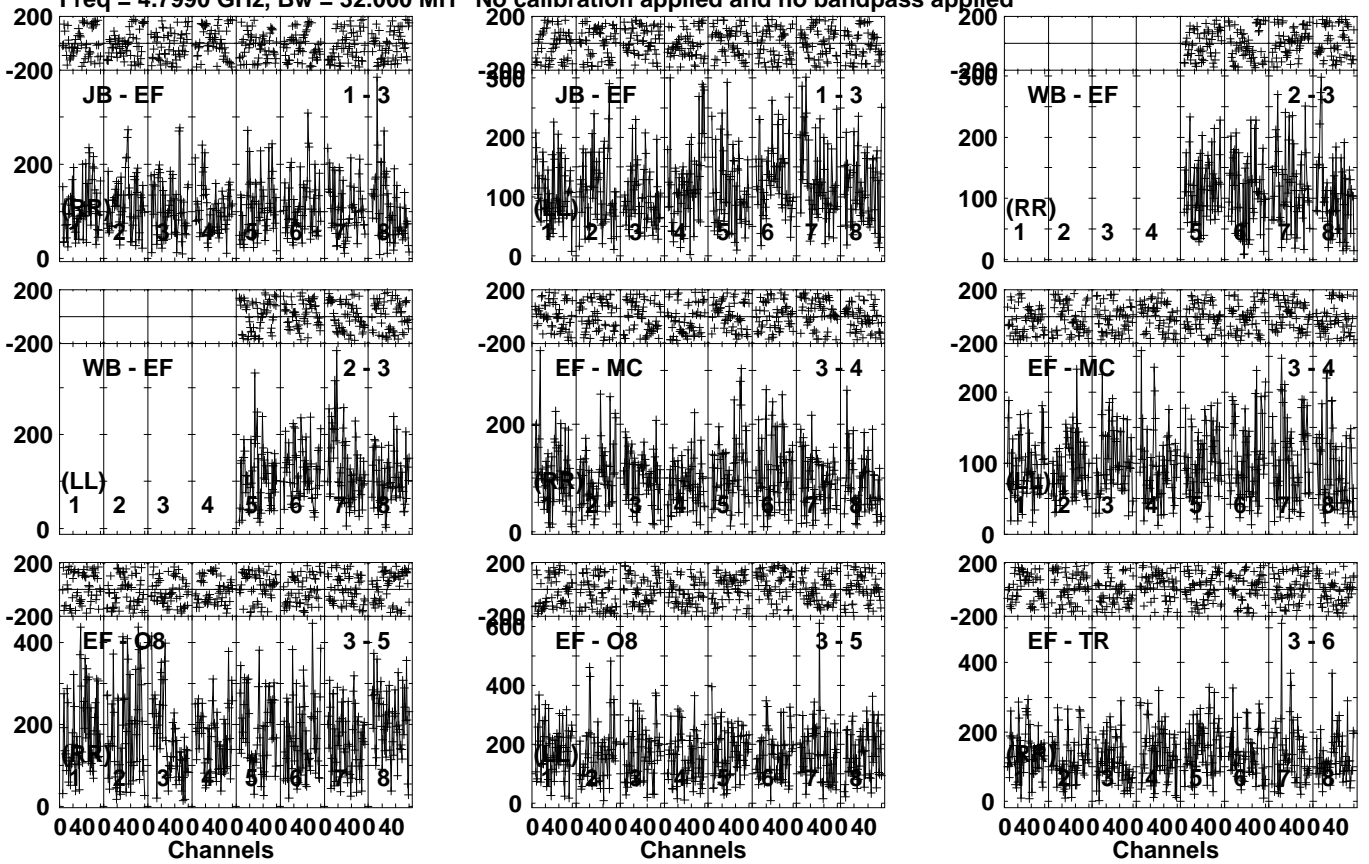
Lower frame: Micro Ampl Jy Top frame: Phas deg Vector averaged cross-power spectrum Several baselines displayed Timerange: 00/02:58:01 to 00/02:59:59
