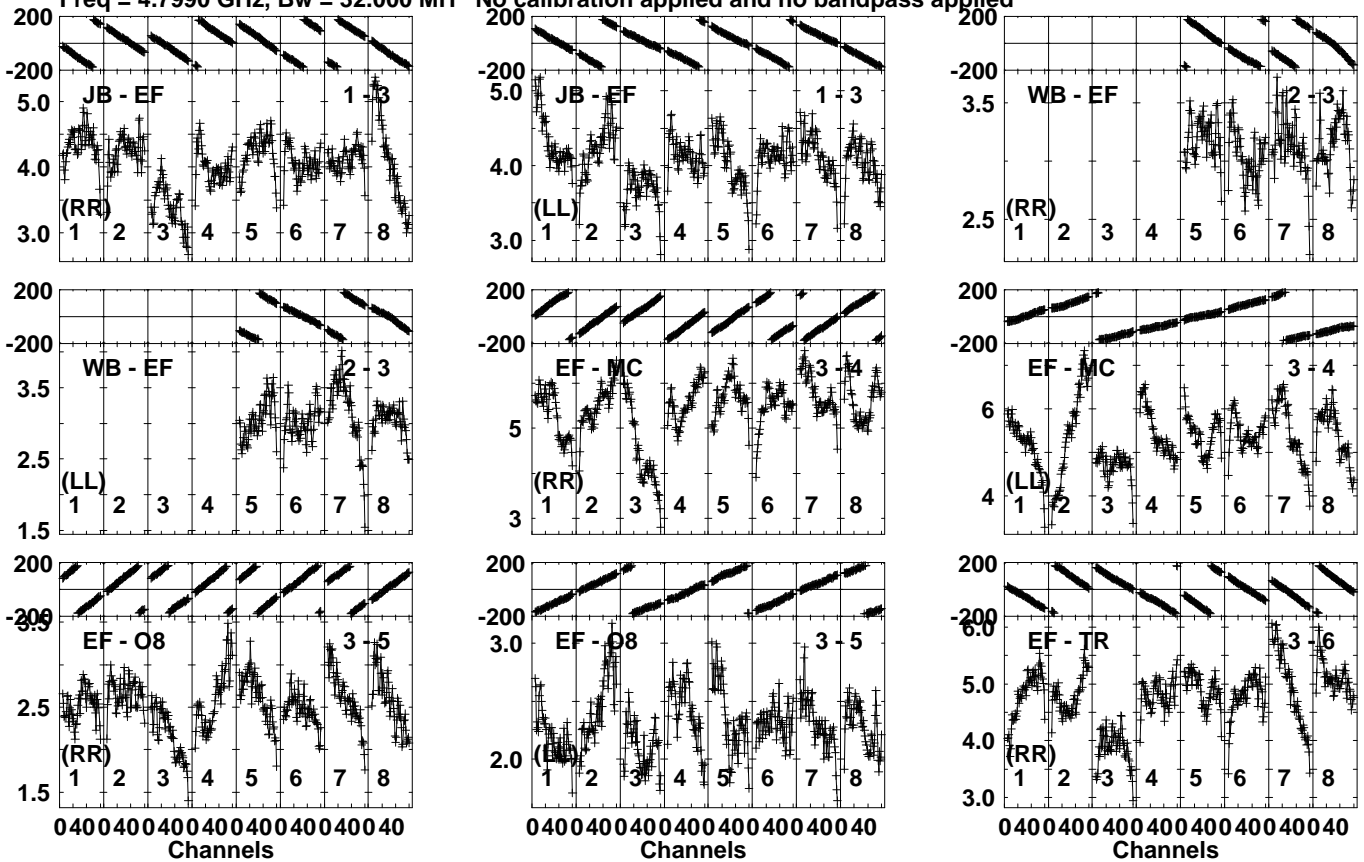
Lower frame: Milli Ampl Jy Top frame: Phas deg Vector averaged cross-power spectrum Several baselines displayed Timerange: 00/06:25:41 to 00/06:26:39
