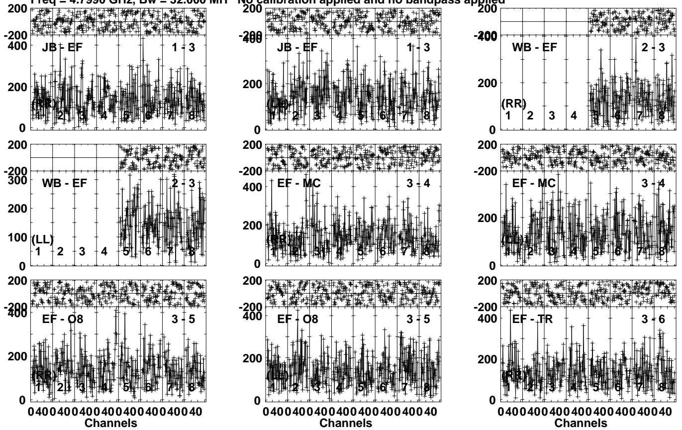
Lower frame: Micro Ampl Jy Top frame: Phas deg Vector averaged cross-power spectrum Several baselines displayed Timerange: 00/07:27:31 to 00/07:29:29
