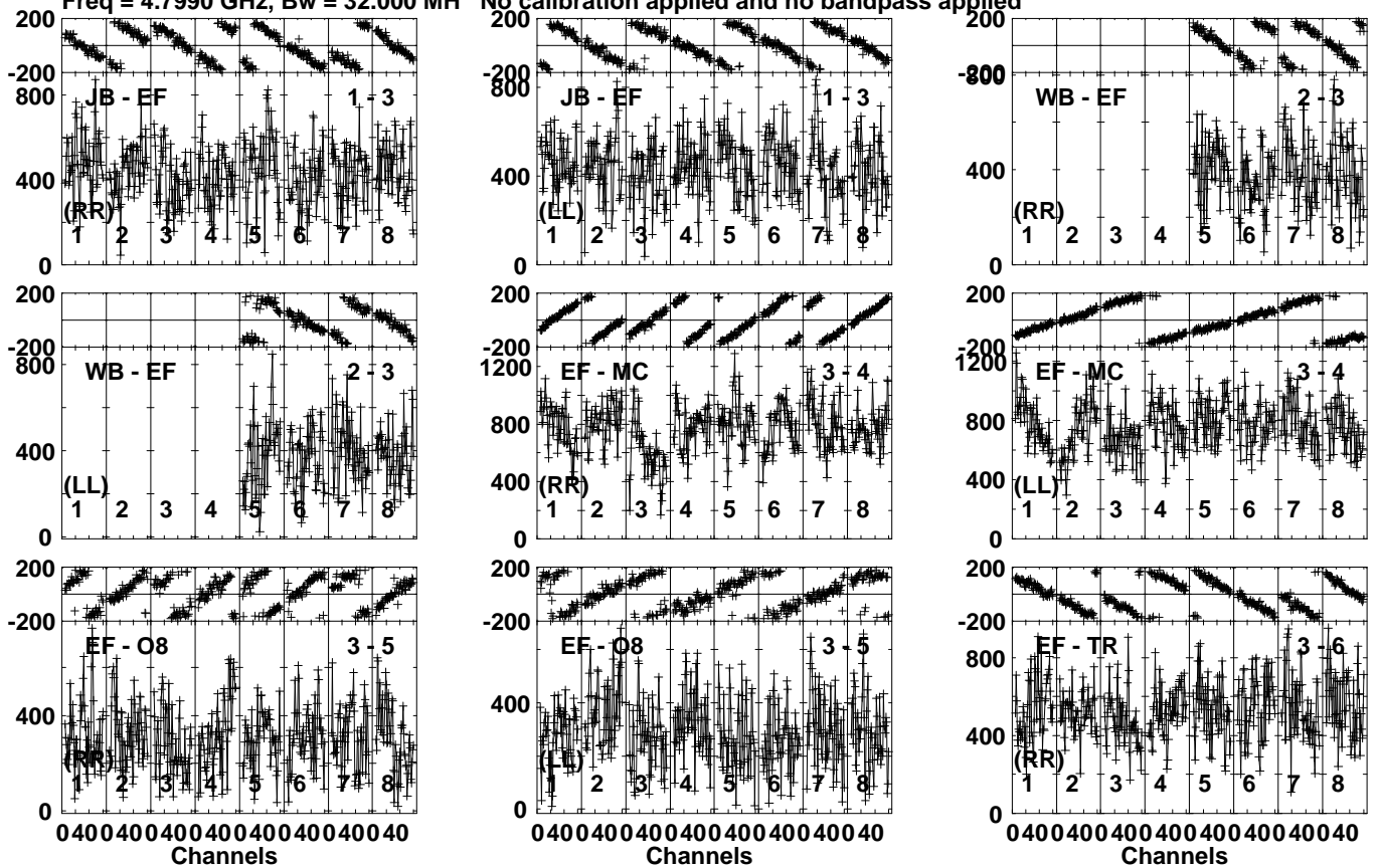
Lower frame: Micro Ampl Jy Top frame: Phas deg Vector averaged cross-power spectrum Several baselines displayed Timerange: 00/05:25:21 to 00/05:26:19
