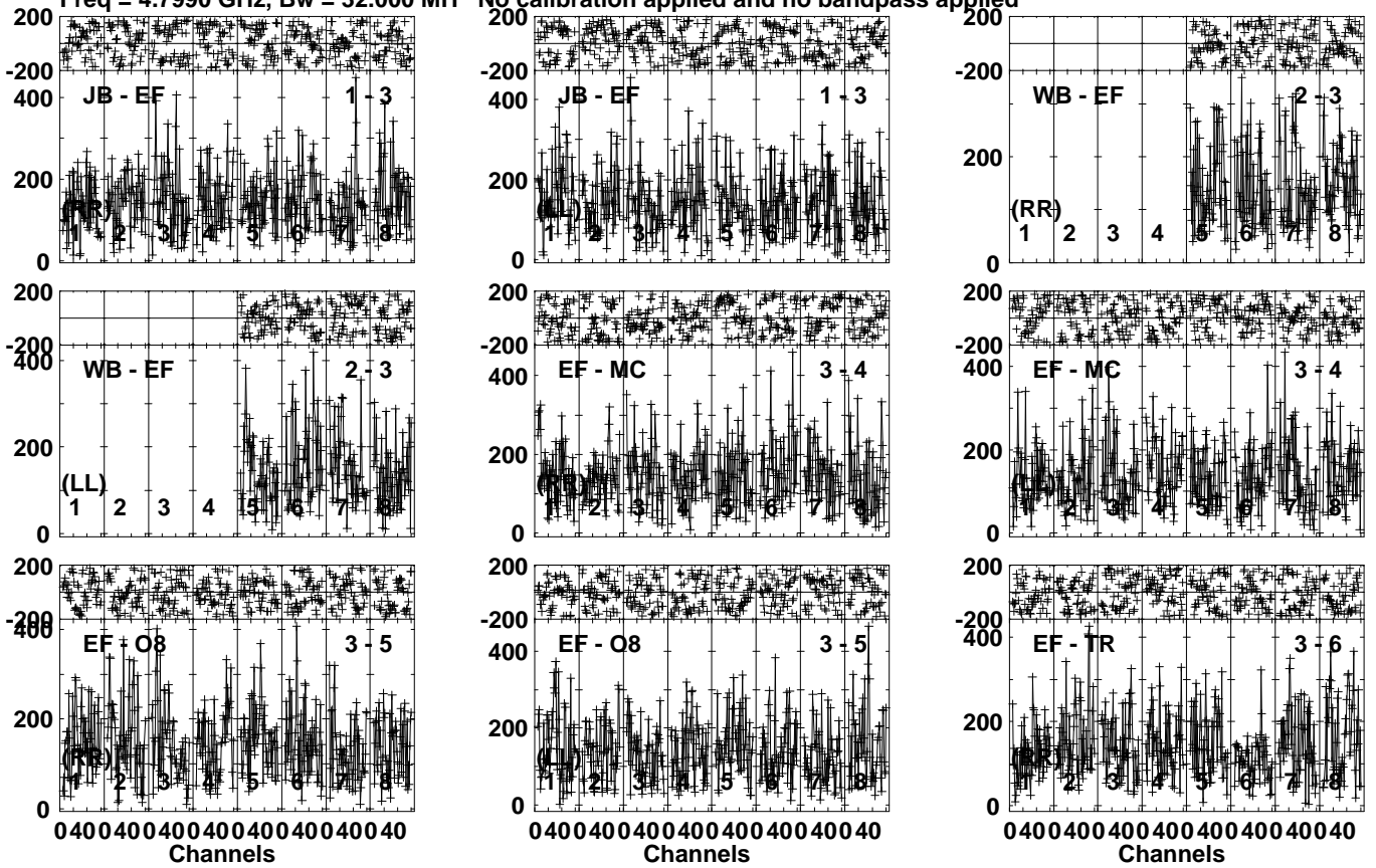
Lower frame: Micro Ampl Jy Top frame: Phas deg Vector averaged cross-power spectrum Several baselines displayed Timerange: 00/08:06:01 to 00/08:07:59
