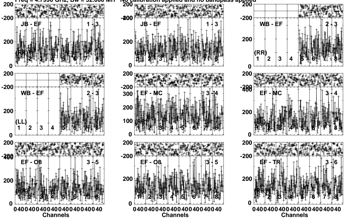
Lower frame: Micro Ampl Jy Top frame: Phas deg Vector averaged cross-power spectrum Several baselines displayed Timerange: 00/07:12:11 to 00/07:14:09
