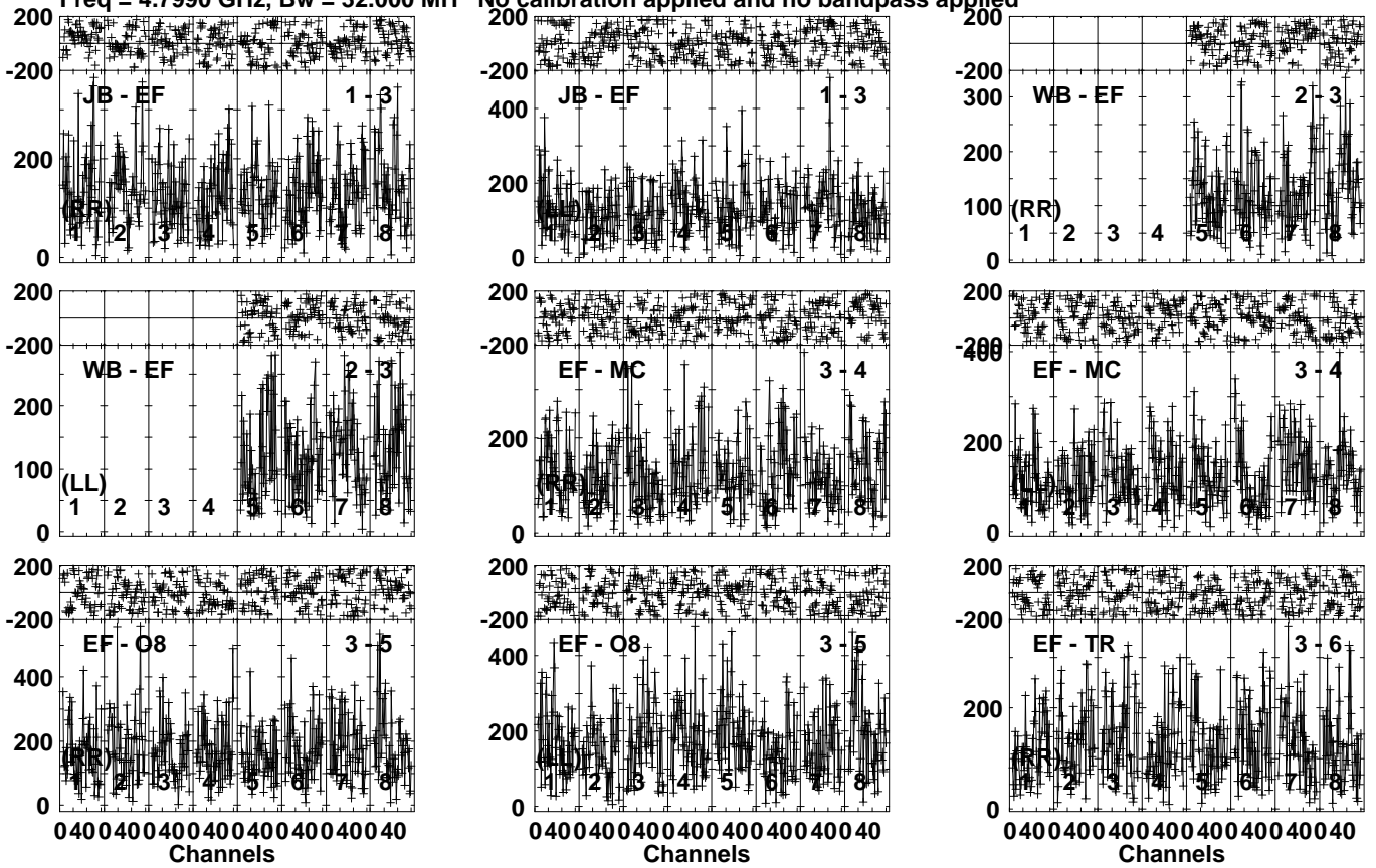
Lower frame: Micro Ampl Jy Top frame: Phas deg Vector averaged cross-power spectrum Several baselines displayed Timerange: 00/02:47:31 to 00/02:49:29
