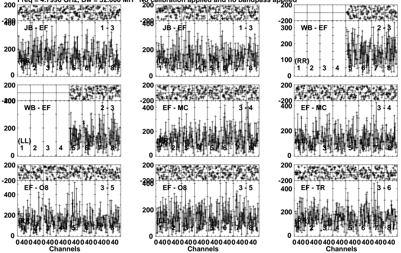
Lower frame: Micro Ampl Jy Top frame: Phas deg Vector averaged cross-power spectrum Several baselines displayed Timerange: 00/08:27:01 to 00/08:28:59
