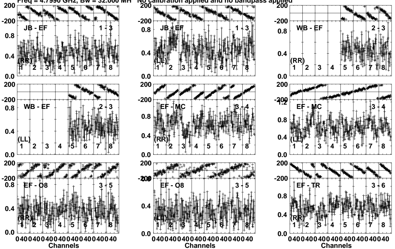
Lower frame: Milli Ampl Jy Top frame: Phas deg Vector averaged cross-power spectrum Several baselines displayed Timerange: 00/07:11:11 to 00/07:12:09
