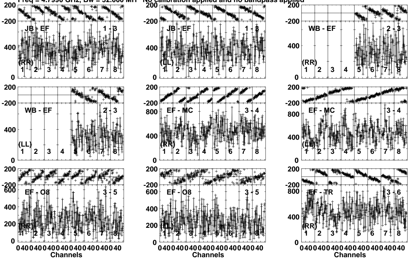
Lower frame: Micro Ampl Jy Top frame: Phas deg Vector averaged cross-power spectrum Several baselines displayed Timerange: 00/03:39:01 to 00/03:39:59
