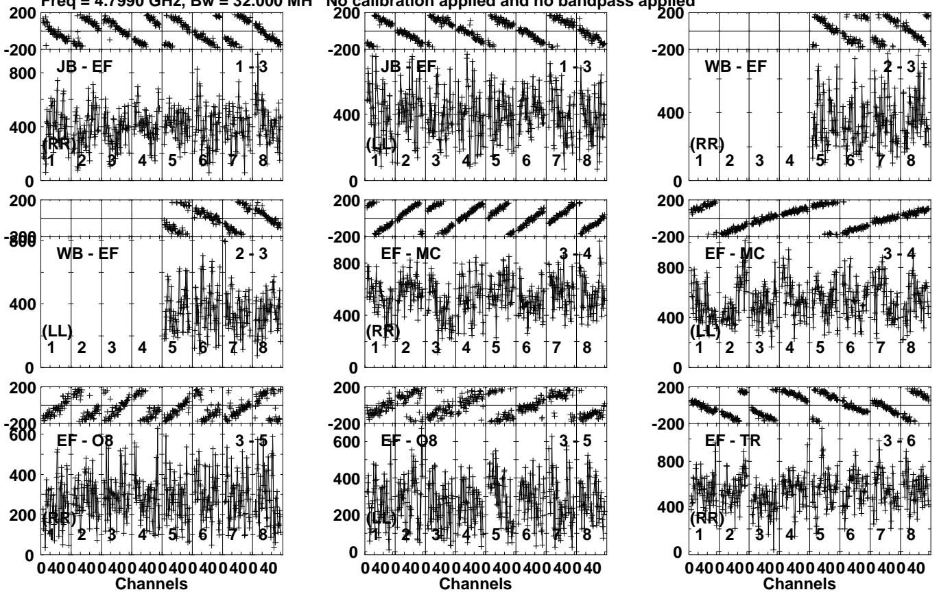
Lower frame: Micro Ampl Jy Top frame: Phas deg Vector averaged cross-power spectrum Several baselines displayed Timerange: 00/04:22:21 to 00/04:23:19
