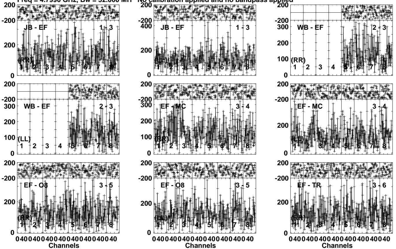
Lower frame: Micro Ampl Jy Top frame: Phas deg Vector averaged cross-power spectrum Several baselines displayed Timerange: 00/06:02:11 to 00/06:04:09
