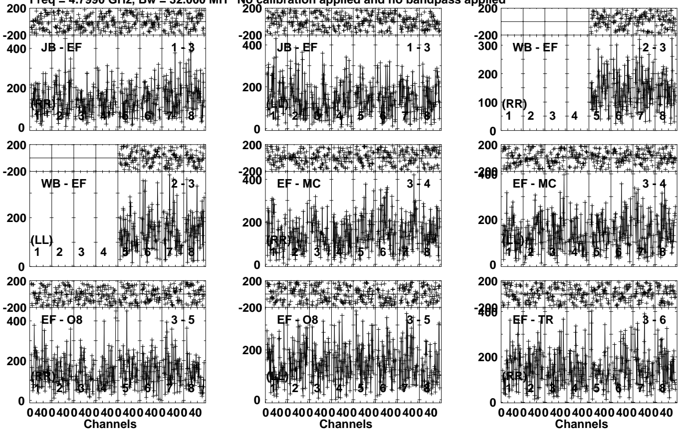
Lower frame: Micro Ampl Jy Top frame: Phas deg Vector averaged cross-power spectrum Several baselines displayed Timerange: 00/07:31:01 to 00/07:32:59
