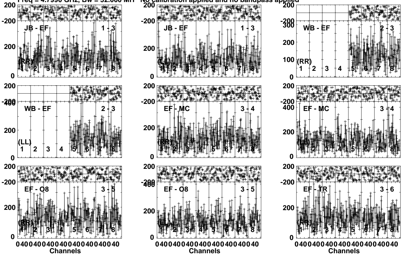
Lower frame: Micro Ampl Jy Top frame: Phas deg Vector averaged cross-power spectrum Several baselines displayed Timerange: 00/06:33:41 to 00/06:35:39
