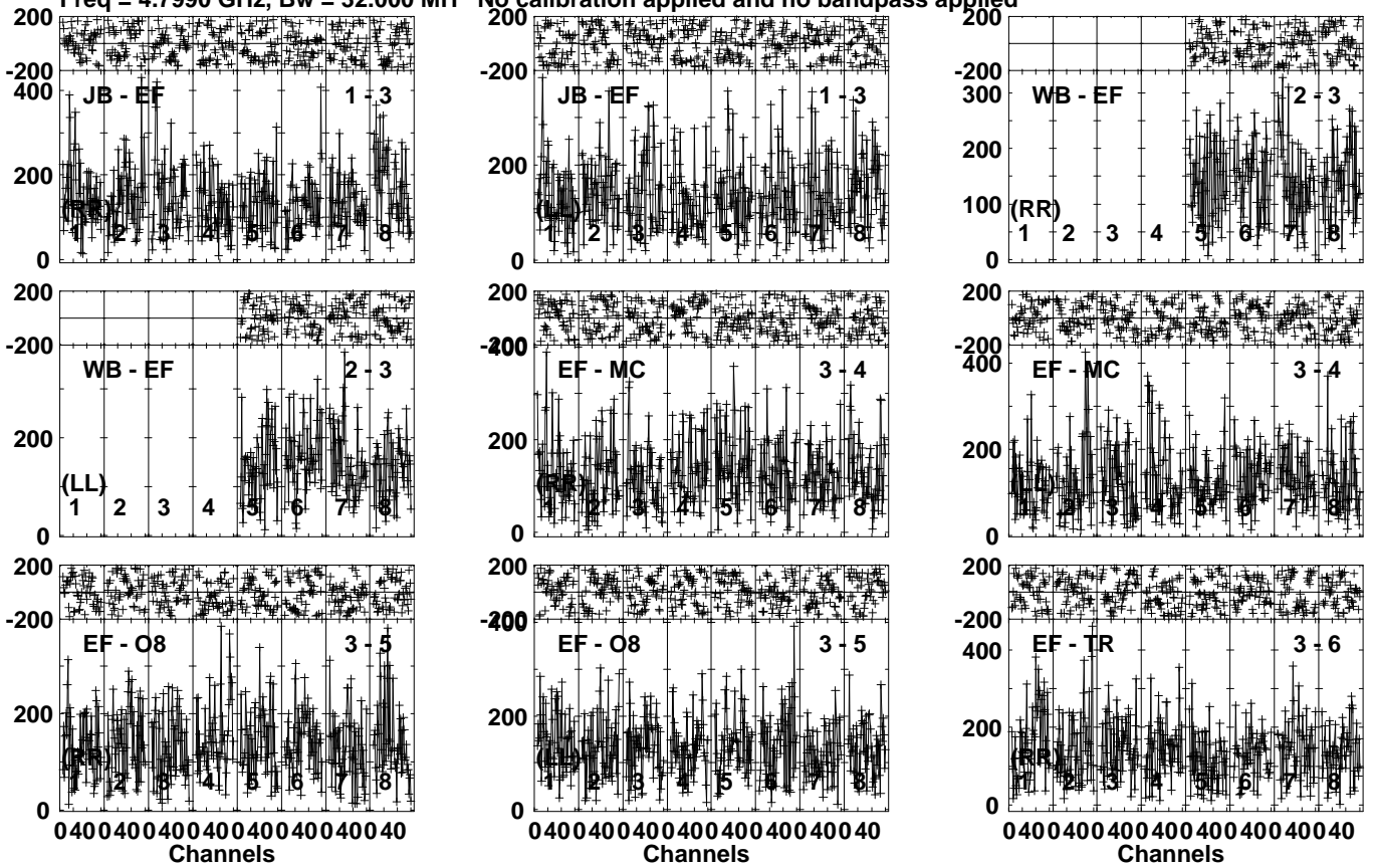
Lower frame: Micro Ampl Jy Top frame: Phas deg Vector averaged cross-power spectrum Several baselines displayed Timerange: 00/06:37:11 to 00/06:39:09
