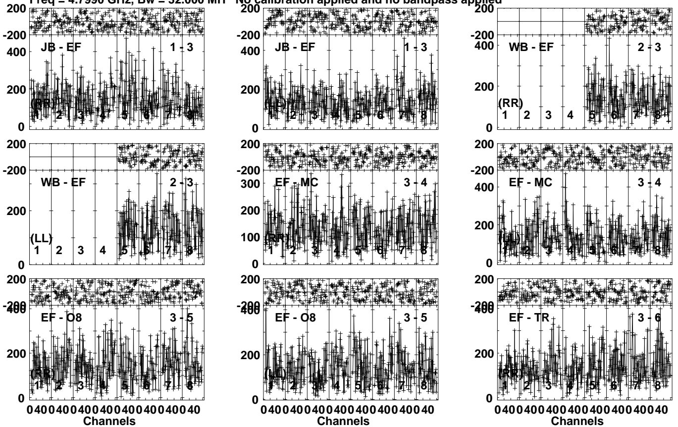
Lower frame: Micro Ampl Jy Top frame: Phas deg Vector averaged cross-power spectrum Several baselines displayed Timerange: 00/05:51:41 to 00/05:53:39
