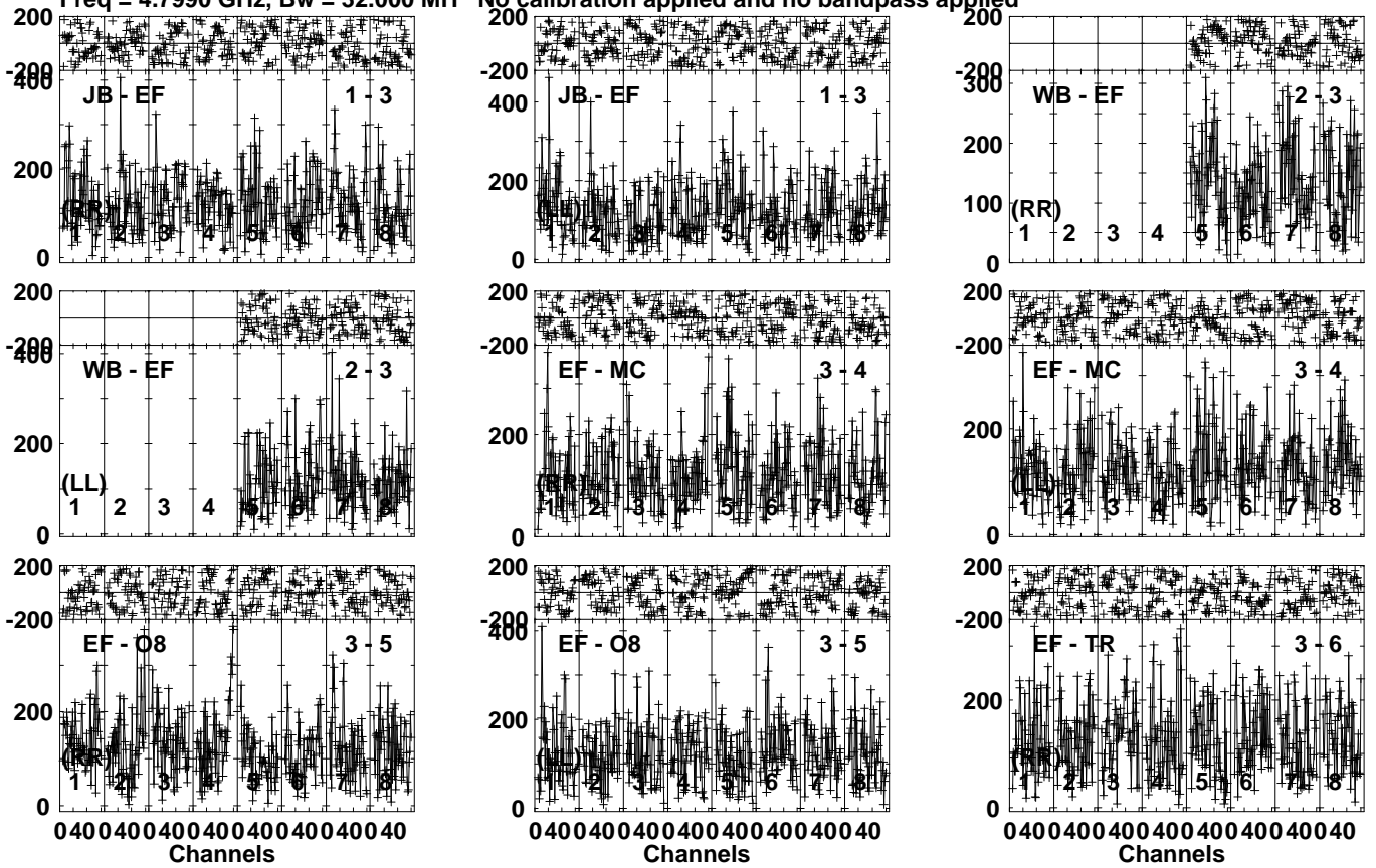
Lower frame: Micro Ampl Jy Top frame: Phas deg Vector averaged cross-power spectrum Several baselines displayed Timerange: 00/06:19:41 to 00/06:21:39
