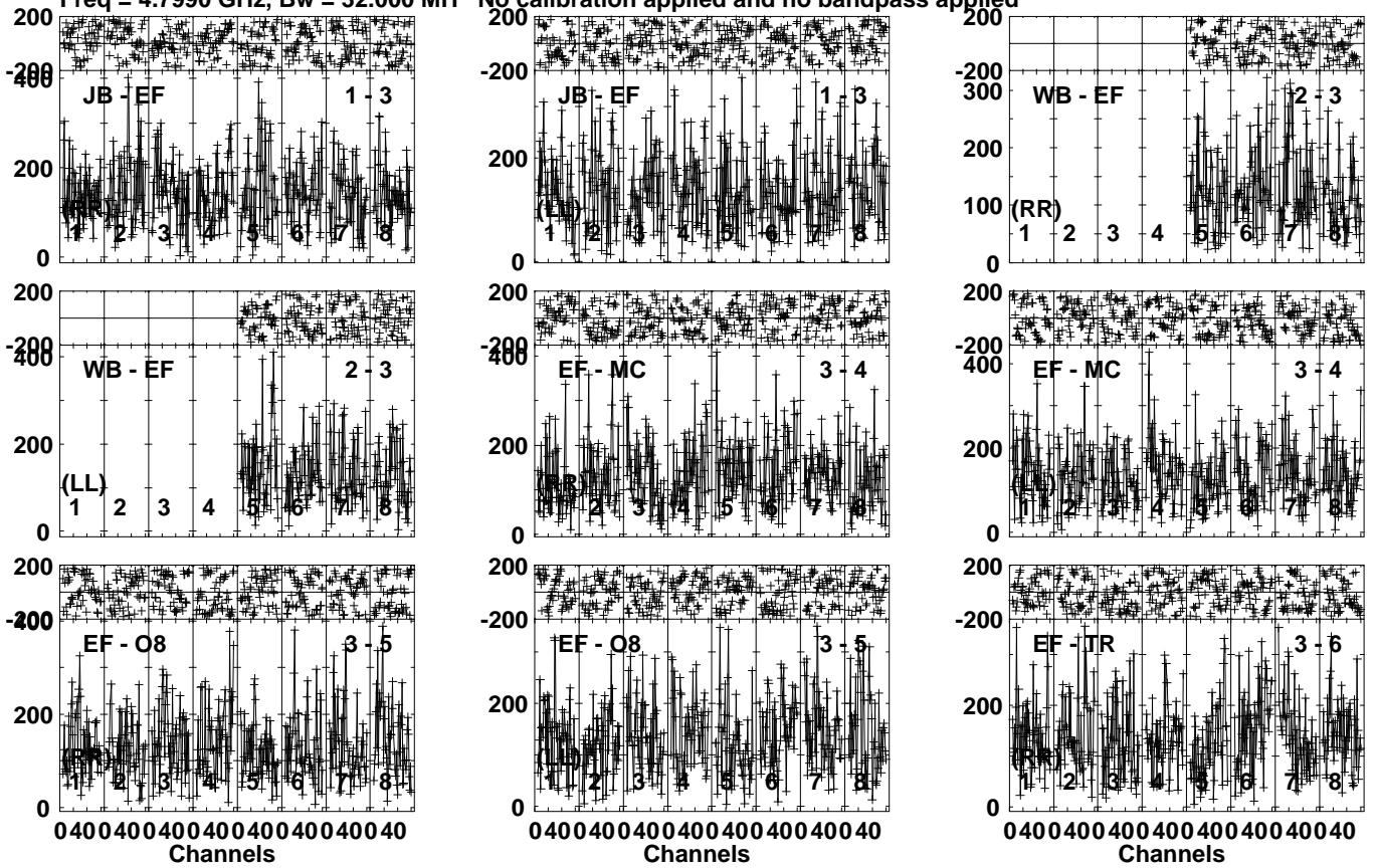
Lower frame: Micro Ampl Jy Top frame: Phas deg Vector averaged cross-power spectrum Several baselines displayed Timerange: 00/06:44:11 to 00/06:46:09
