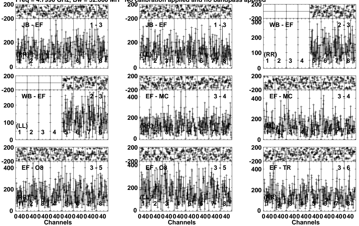
Lower frame: Micro Ampl Jy Top frame: Phas deg Vector averaged cross-power spectrum Several baselines displayed Timerange: 00/03:01:31 to 00/03:03:29
