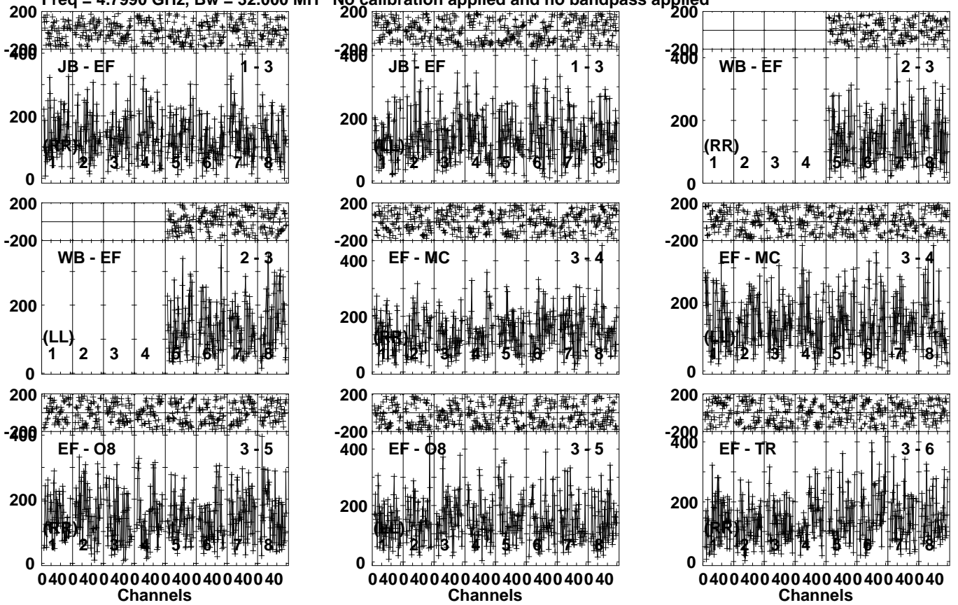
Lower frame: Micro Ampl Jy Top frame: Phas deg Vector averaged cross-power spectrum Several baselines displayed Timerange: 00/04:26:51 to 00/04:28:49
