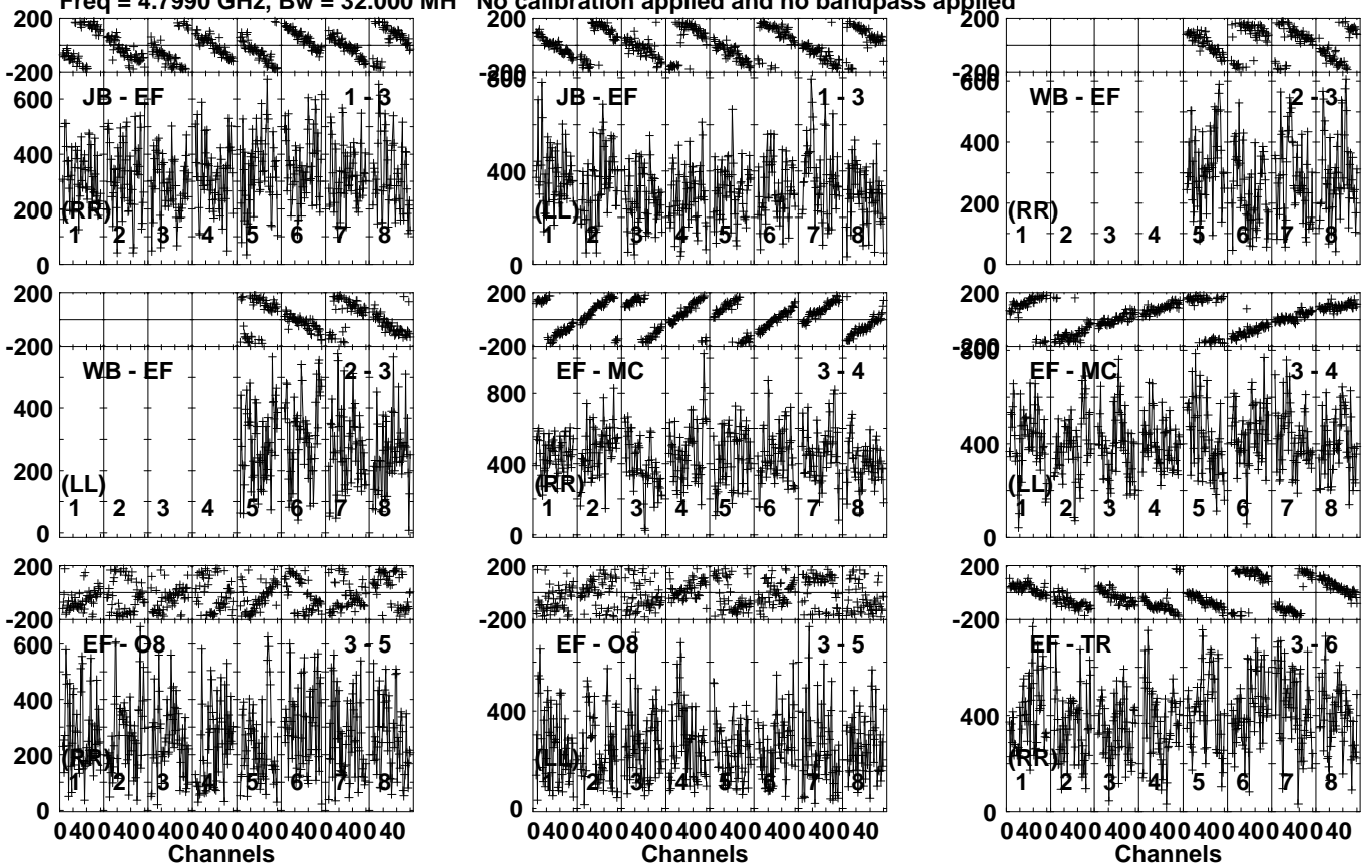
Lower frame: Micro Ampl Jy Top frame: Phas deg Vector averaged cross-power spectrum Several baselines displayed Timerange: 00/03:11:01 to 00/03:11:59
