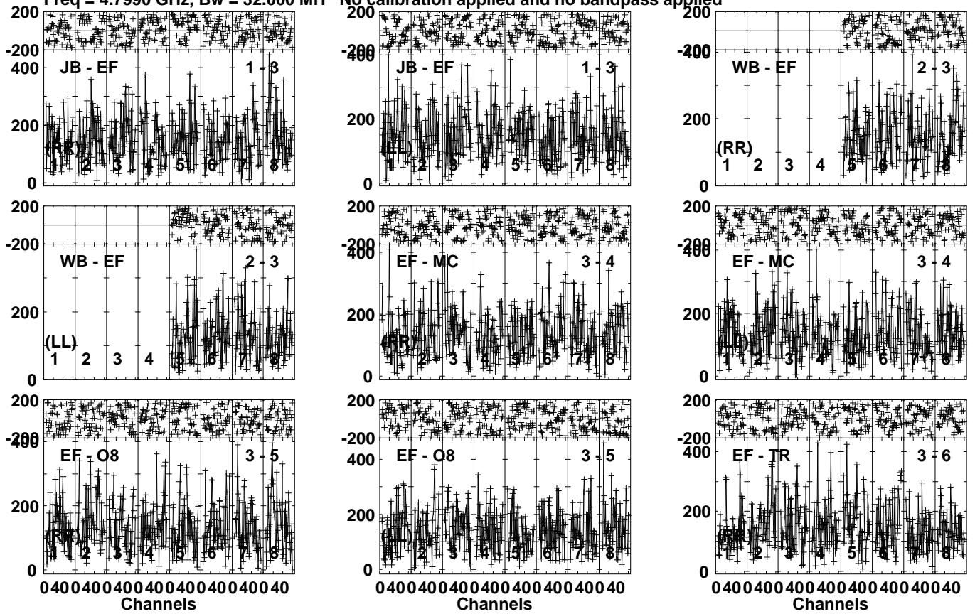
Lower frame: Micro Ampl Jy Top frame: Phas deg Vector averaged cross-power spectrum Several baselines displayed Timerange: 00/07:24:01 to 00/07:25:59
