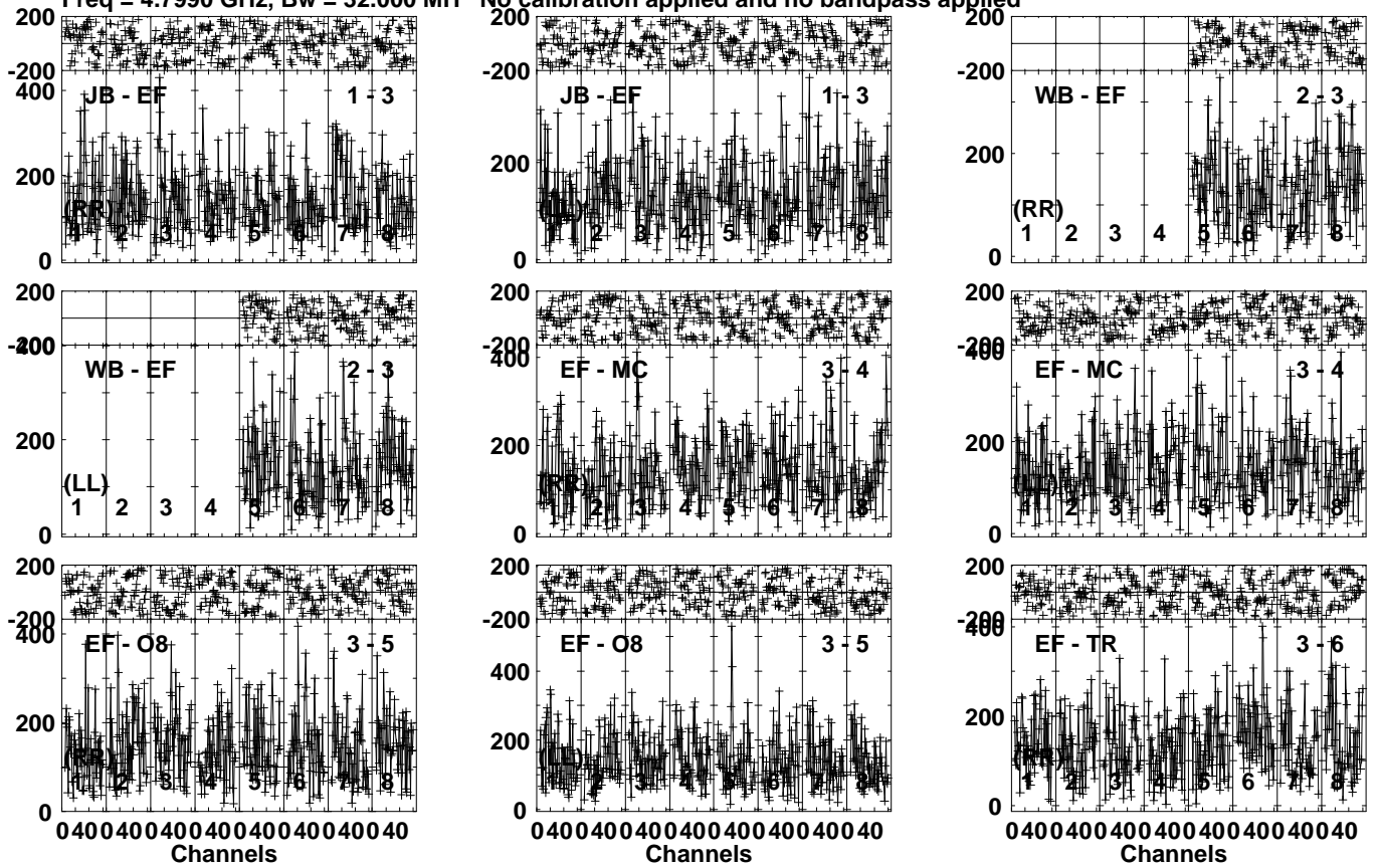
Lower frame: Micro Ampl Jy Top frame: Phas deg Vector averaged cross-power spectrum Several baselines displayed Timerange: 00/04:54:51 to 00/04:56:49
