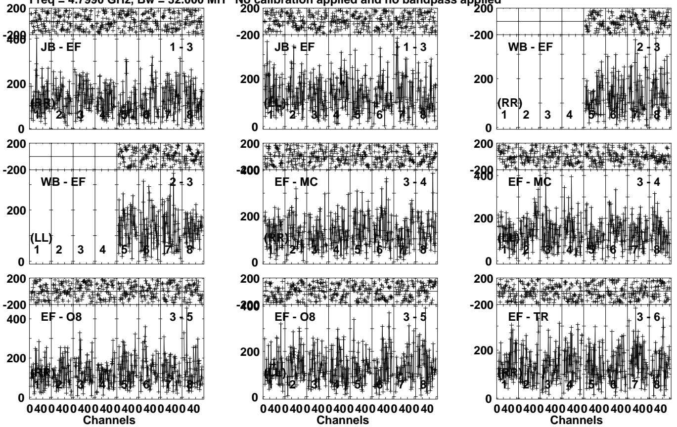
Lower frame: Micro Ampl Jy Top frame: Phas deg Vector averaged cross-power spectrum Several baselines displayed Timerange: 00/03:36:31 to 00/03:38:29
