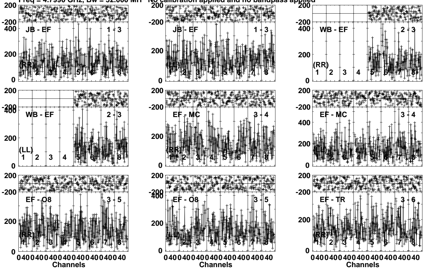
Lower frame: Micro Ampl Jy Top frame: Phas deg Vector averaged cross-power spectrum Several baselines displayed Timerange: 00/04:33:51 to 00/04:35:49
