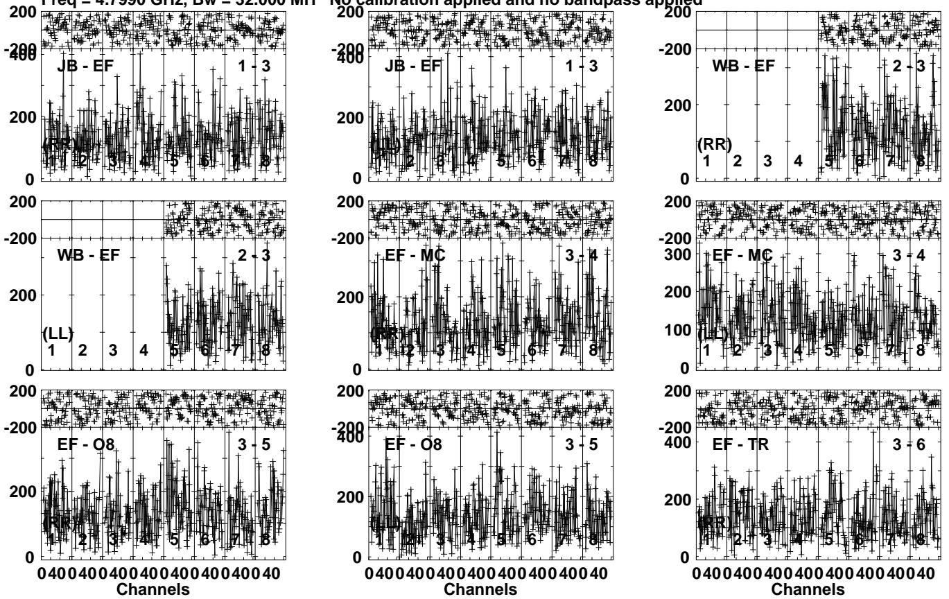
Lower frame: Micro Ampl Jy Top frame: Phas deg Vector averaged cross-power spectrum Several baselines displayed Timerange: 00/06:58:11 to 00/07:00:09
