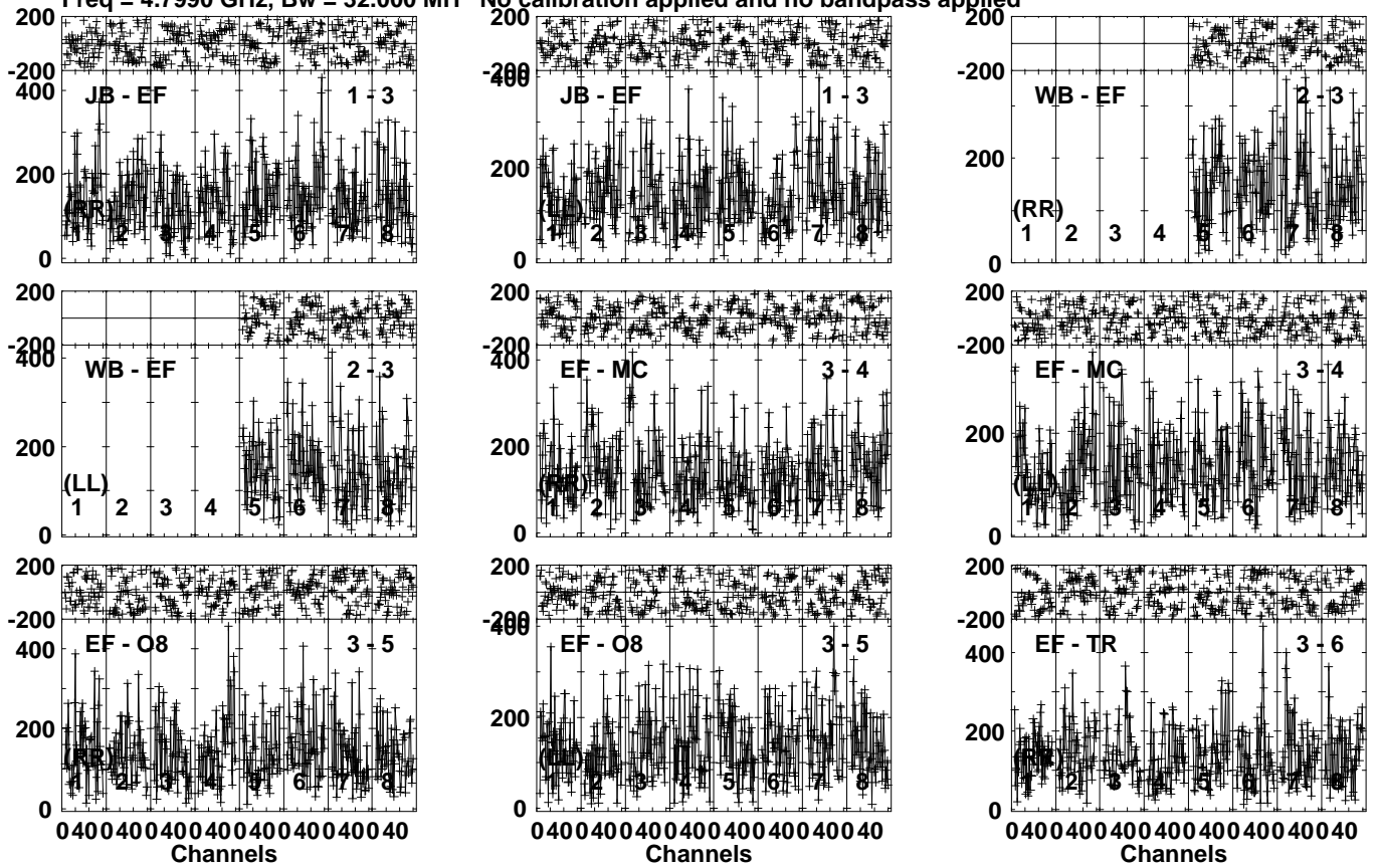
Lower frame: Micro Ampl Jy Top frame: Phas deg Vector averaged cross-power spectrum Several baselines displayed Timerange: 00/07:38:01 to 00/07:39:59
