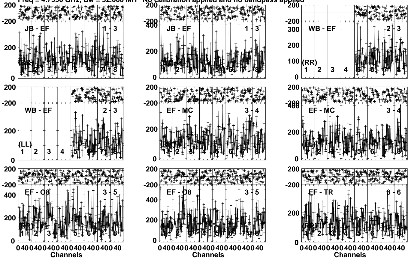
Lower frame: Micro Ampl Jy Top frame: Phas deg Vector averaged cross-power spectrum Several baselines displayed Timerange: 00/03:29:31 to 00/03:31:29
