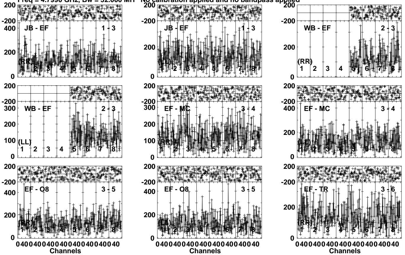
Lower frame: Micro Ampl Jy Top frame: Phas deg Vector averaged cross-power spectrum Several baselines displayed Timerange: 00/04:58:21 to 00/05:00:19
