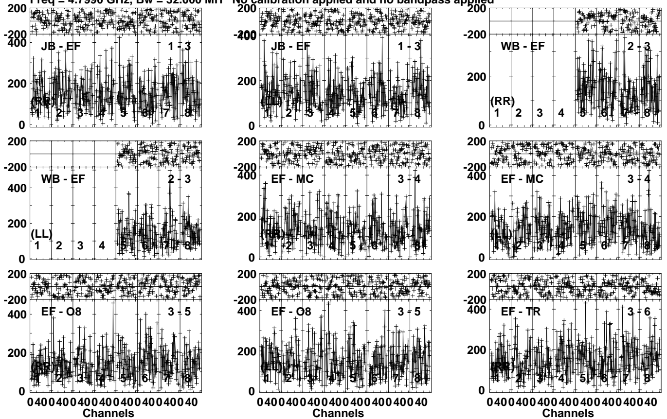
Lower frame: Micro Ampl Jy Top frame: Phas deg Vector averaged cross-power spectrum Several baselines displayed Timerange: 00/07:52:01 to 00/07:53:59
