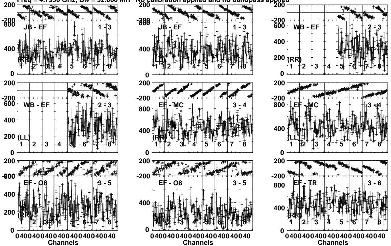
Lower frame: Micro Ampl Jy Top frame: Phas deg Vector averaged cross-power spectrum Several baselines displayed Timerange: 00/03:25:01 to 00/03:25:59
