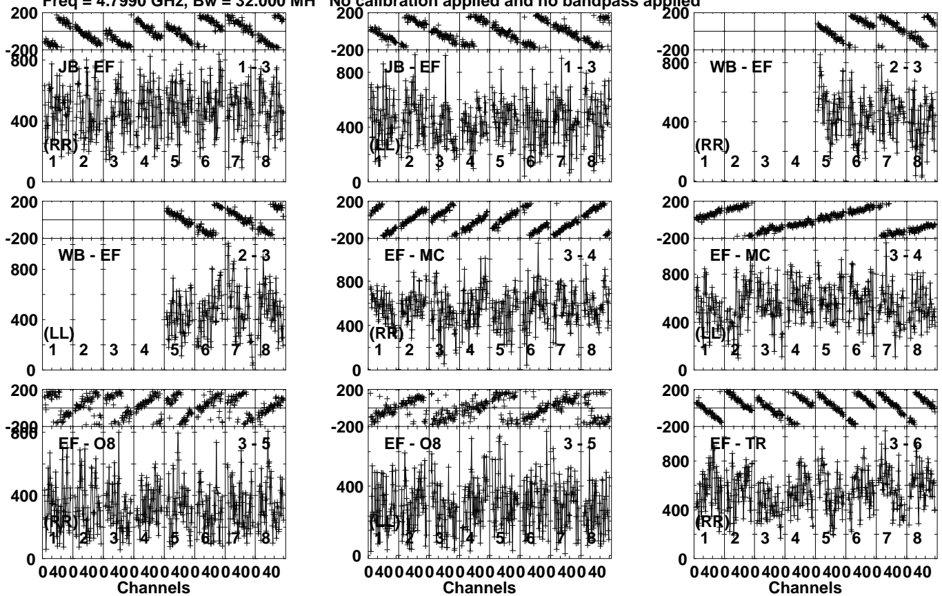
Lower frame: Micro Ampl Jy Top frame: Phas deg Vector averaged cross-power spectrum Several baselines displayed Timerange: 00/08:15:31 to 00/08:16:29
