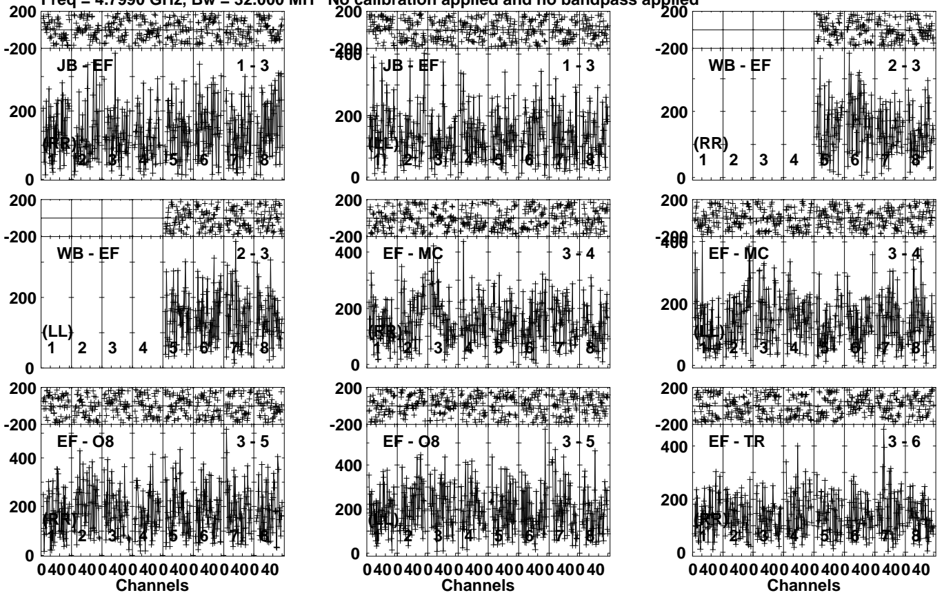
Lower frame: Micro Ampl Jy Top frame: Phas deg Vector averaged cross-power spectrum Several baselines displayed Timerange: 00/04:12:51 to 00/04:14:49
