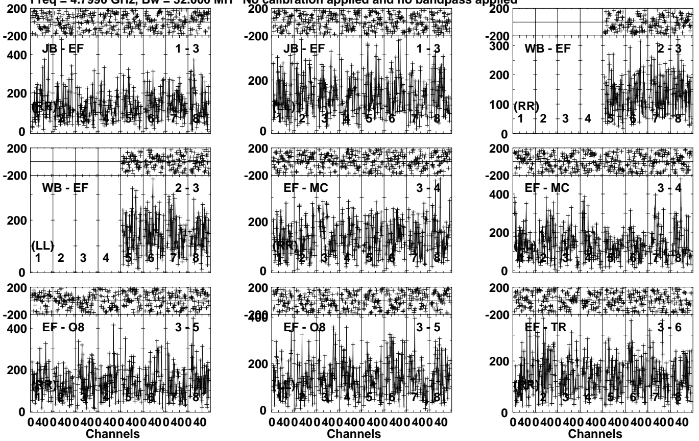
Lower frame: Micro Ampl Jy Top frame: Phas deg Vector averaged cross-power spectrum Several baselines displayed Timerange: 00/05:58:41 to 00/06:00:39
