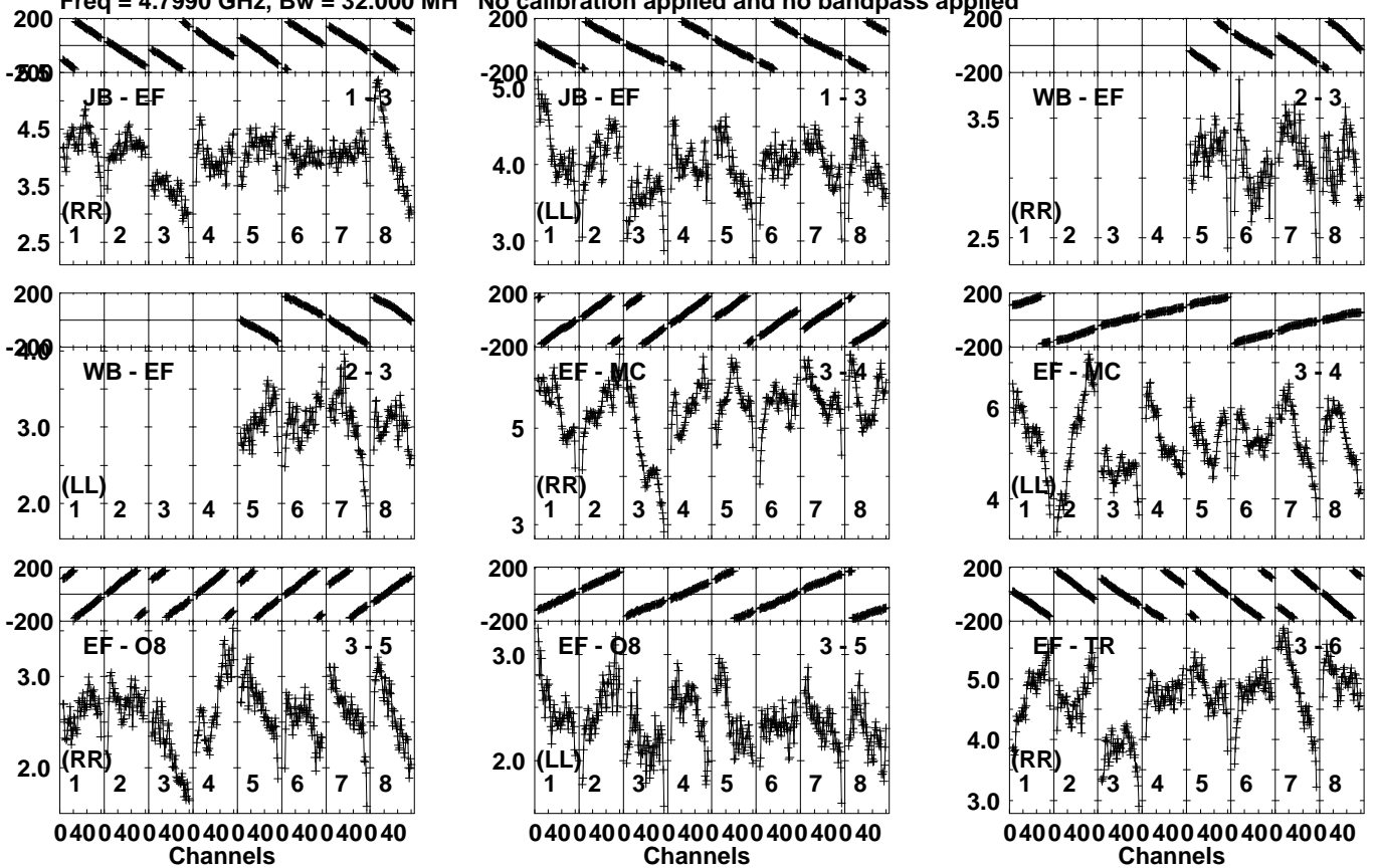
Lower frame: Milli Ampl Jy Top frame: Phas deg Vector averaged cross-power spectrum Several baselines displayed Timerange: 00/07:22:41 to 00/07:23:59
