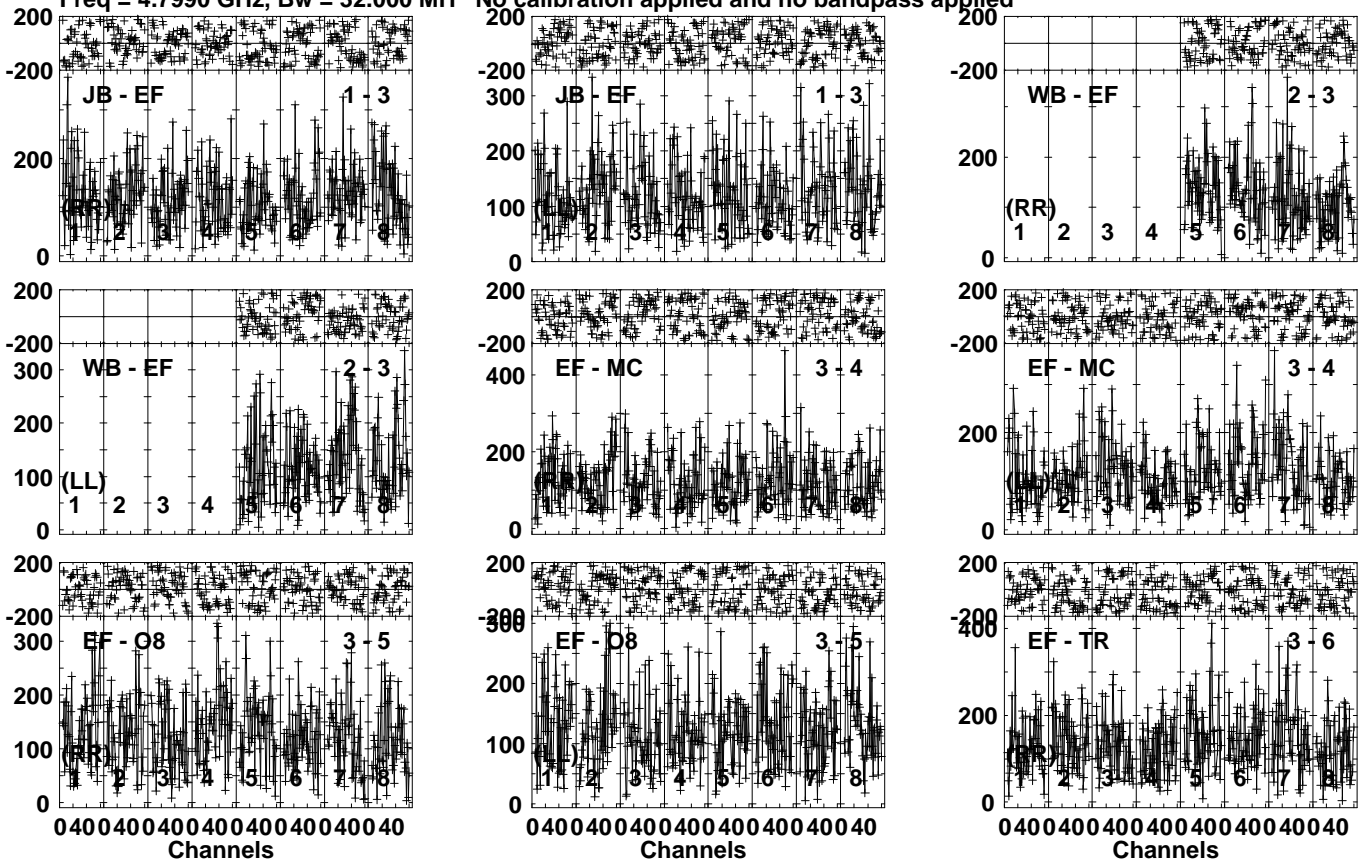
Lower frame: Micro Ampl Jy Top frame: Phas deg Vector averaged cross-power spectrum Several baselines displayed Timerange: 00/05:26:21 to 00/05:28:19
