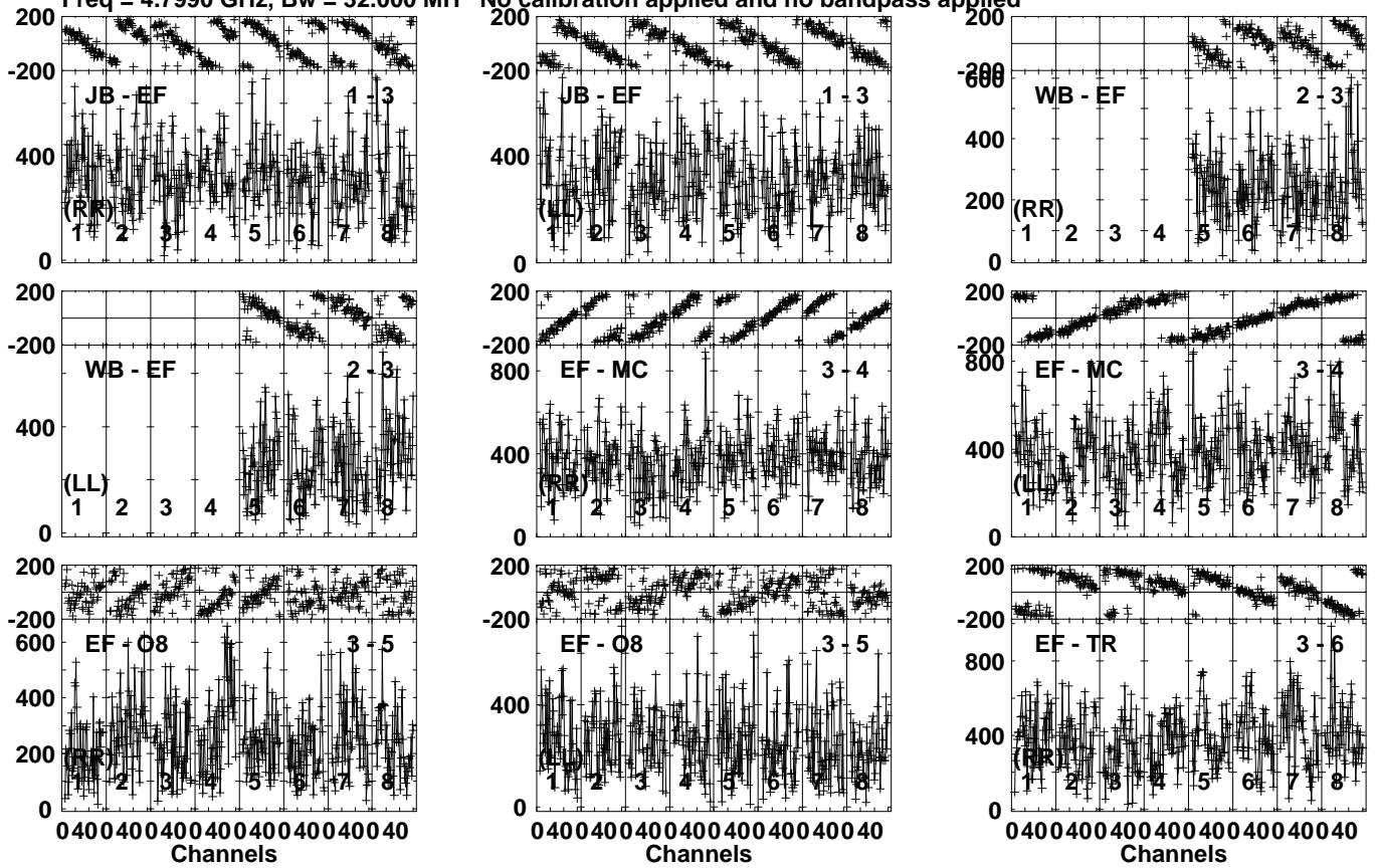
Lower frame: Micro Ampl Jy Top frame: Phas deg Vector averaged cross-power spectrum Several baselines displayed Timerange: 00/03:04:01 to 00/03:04:59
