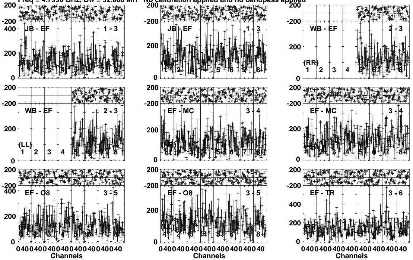
Lower frame: Micro Ampl Jy Top frame: Phas deg Vector averaged cross-power spectrum Several baselines displayed Timerange: 00/04:23:21 to 00/04:25:19
