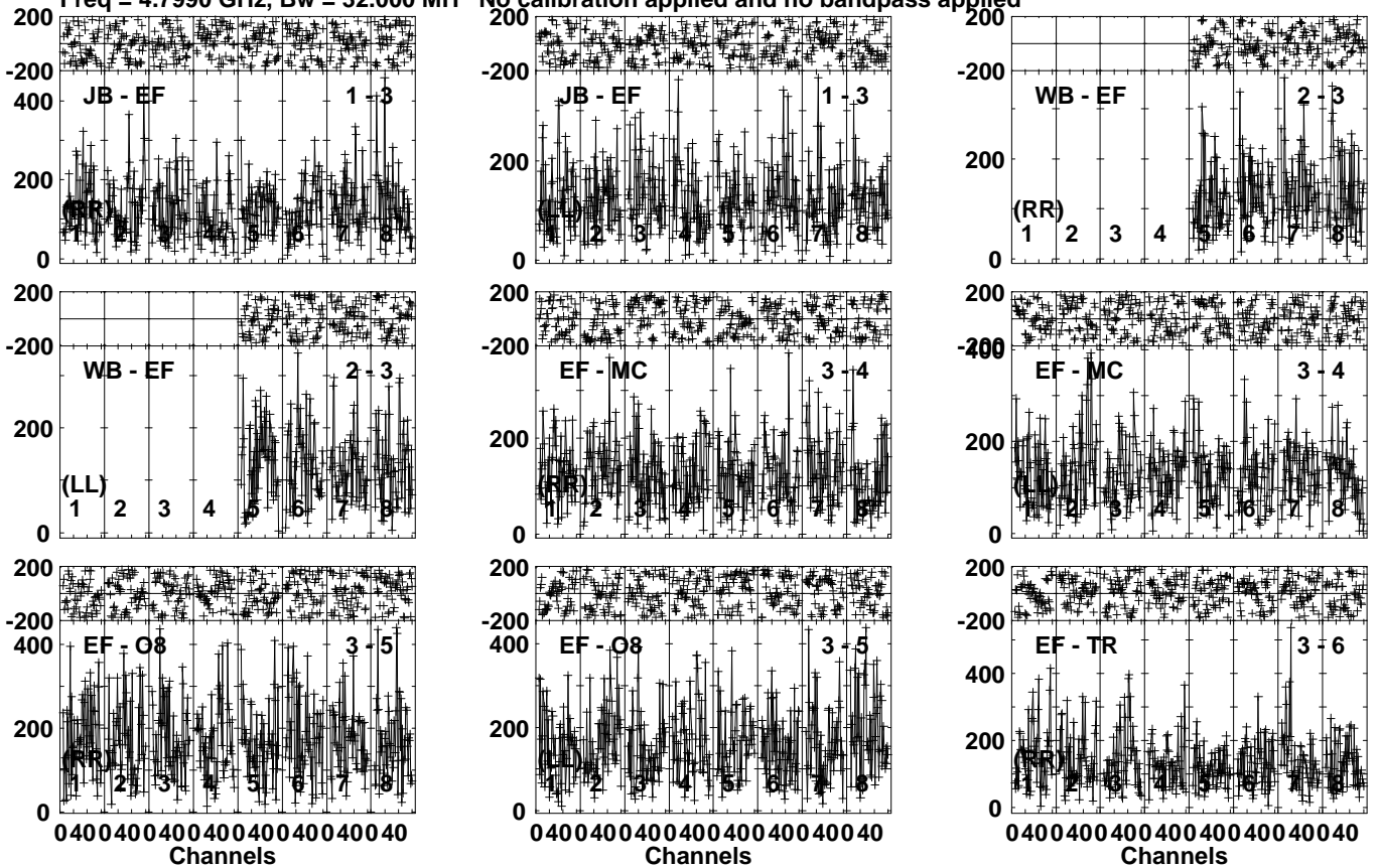
Lower frame: Micro Ampl Jy Top frame: Phas deg Vector averaged cross-power spectrum Several baselines displayed Timerange: 00/04:16:21 to 00/04:18:19
