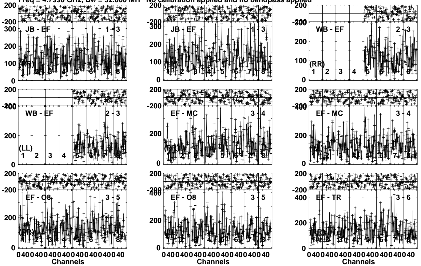
Lower frame: Micro Ampl Jy Top frame: Phas deg Vector averaged cross-power spectrum Several baselines displayed Timerange: 00/05:12:21 to 00/05:14:19
