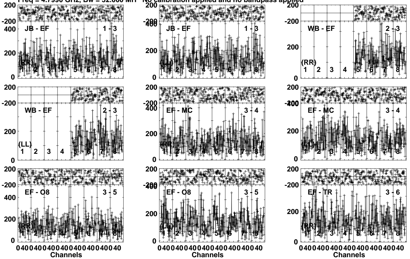
Lower frame: Micro Ampl Jy Top frame: Phas deg Vector averaged cross-power spectrum Several baselines displayed Timerange: 00/07:01:41 to 00/07:03:39
