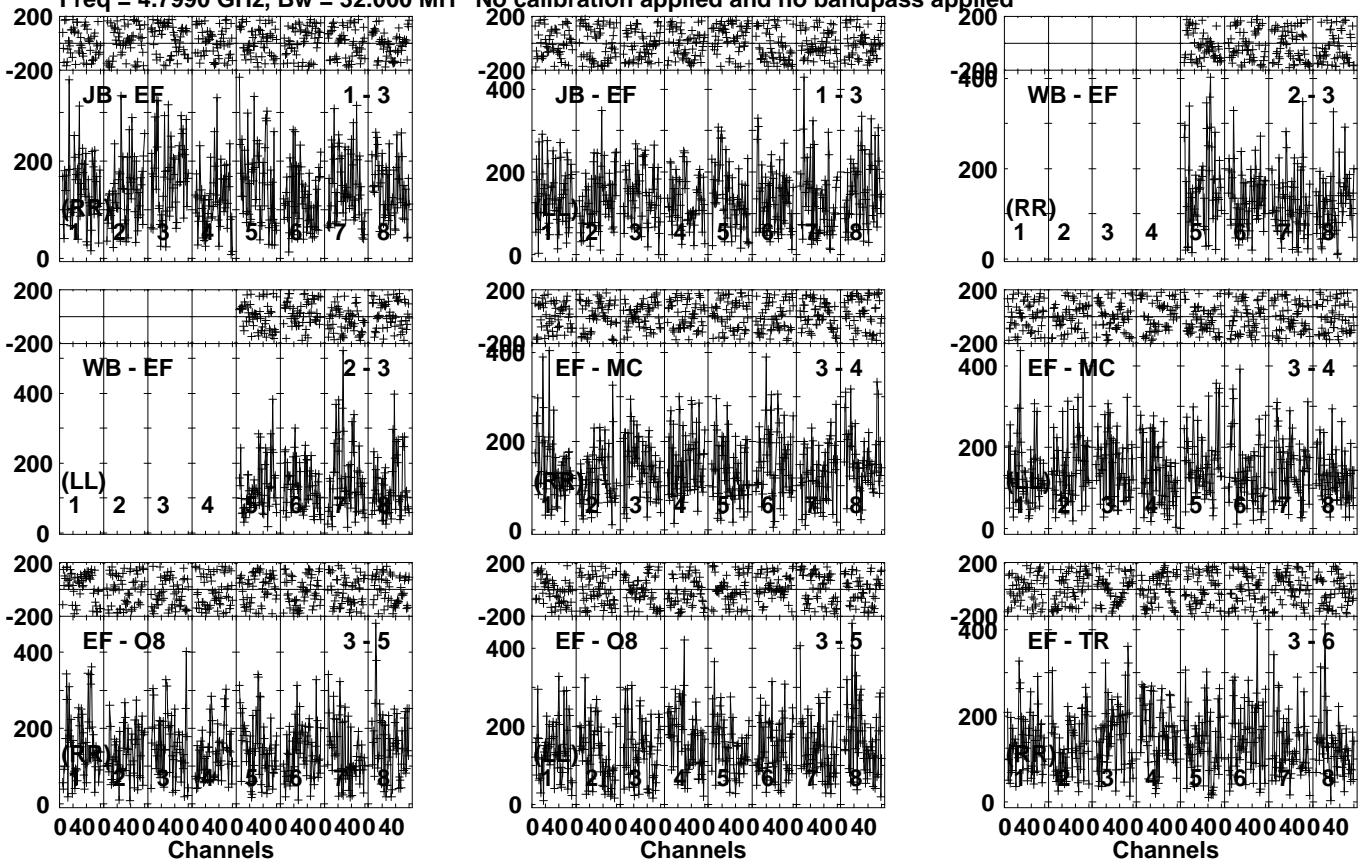
Lower frame: Micro Ampl Jy Top frame: Phas deg Vector averaged cross-power spectrum Several baselines displayed Timerange: 00/08:56:01 to 00/08:57:59
