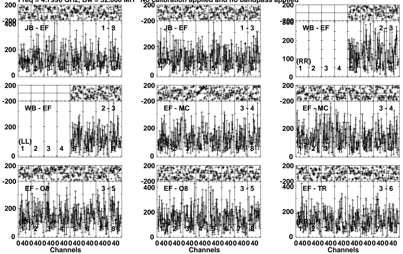
Lower frame: Micro Ampl Jy Top frame: Phas deg Vector averaged cross-power spectrum Several baselines displayed Timerange: 00/03:19:01 to 00/03:20:59
