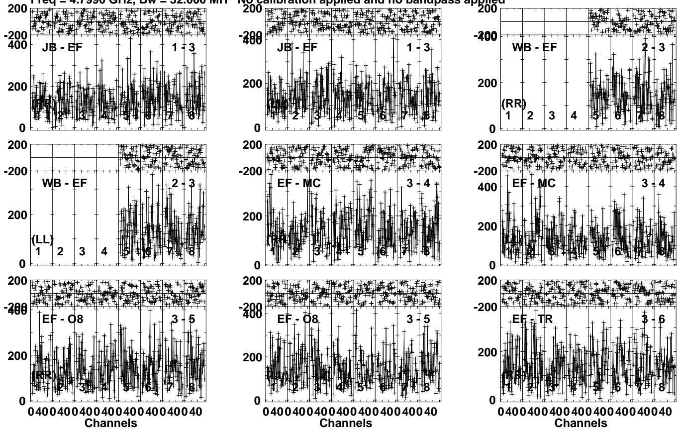
Lower frame: Micro Ampl Jy Top frame: Phas deg Vector averaged cross-power spectrum Several baselines displayed Timerange: 00/06:23:11 to 00/06:25:09
