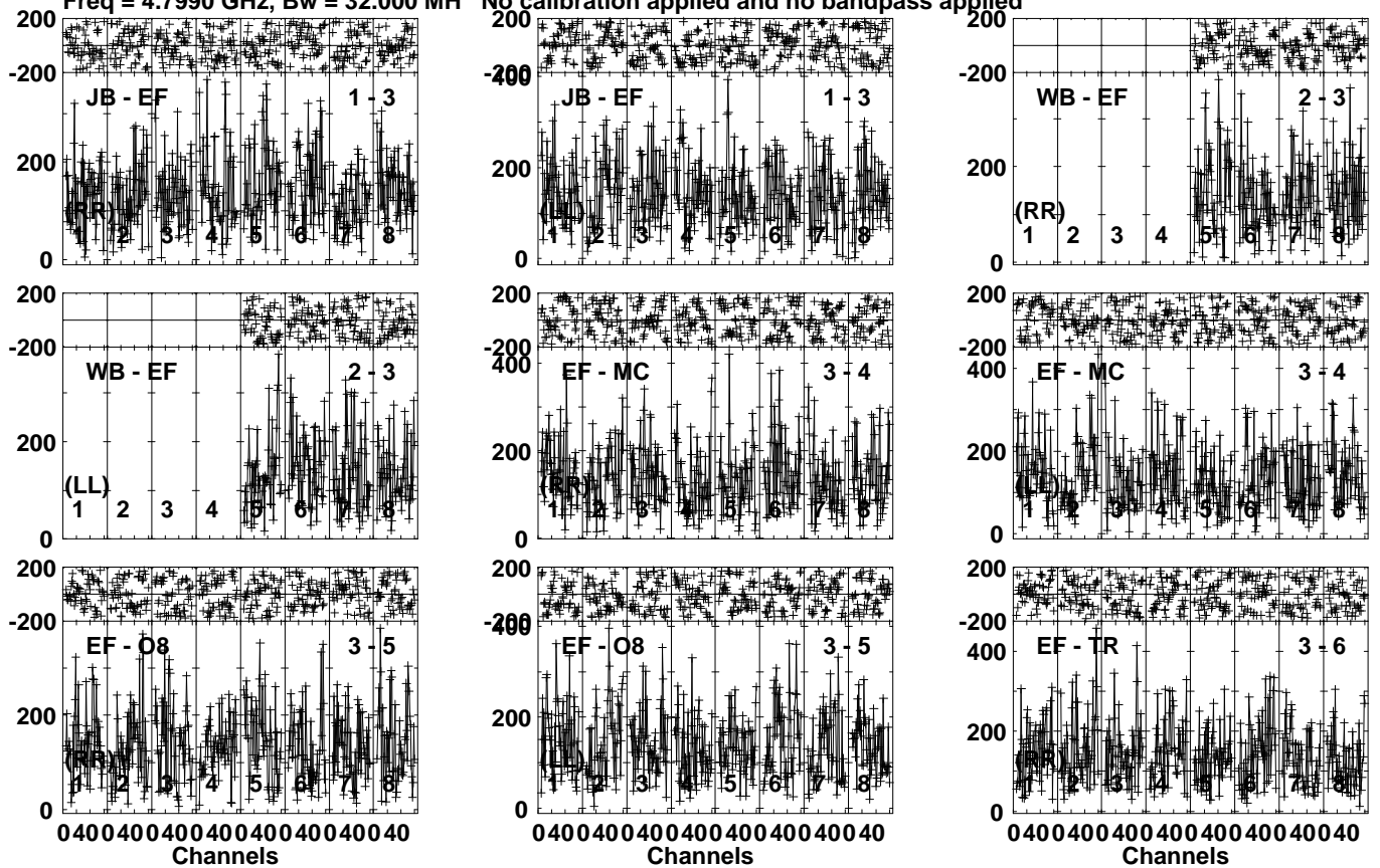
Lower frame: Micro Ampl Jy Top frame: Phas deg Vector averaged cross-power spectrum Several baselines displayed Timerange: 00/05:15:51 to 00/05:17:49
