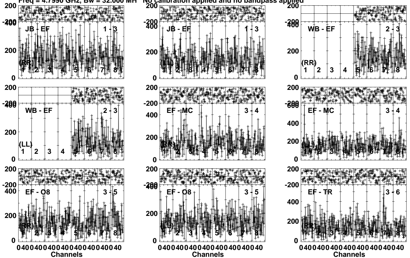
Lower frame: Micro Ampl Jy Top frame: Phas deg Vector averaged cross-power spectrum Several baselines displayed Timerange: 00/08:41:01 to 00/08:42:59
