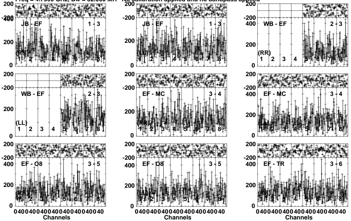
Lower frame: Micro Ampl Jy Top frame: Phas deg Vector averaged cross-power spectrum Several baselines displayed Timerange: 00/07:45:01 to 00/07:46:59
