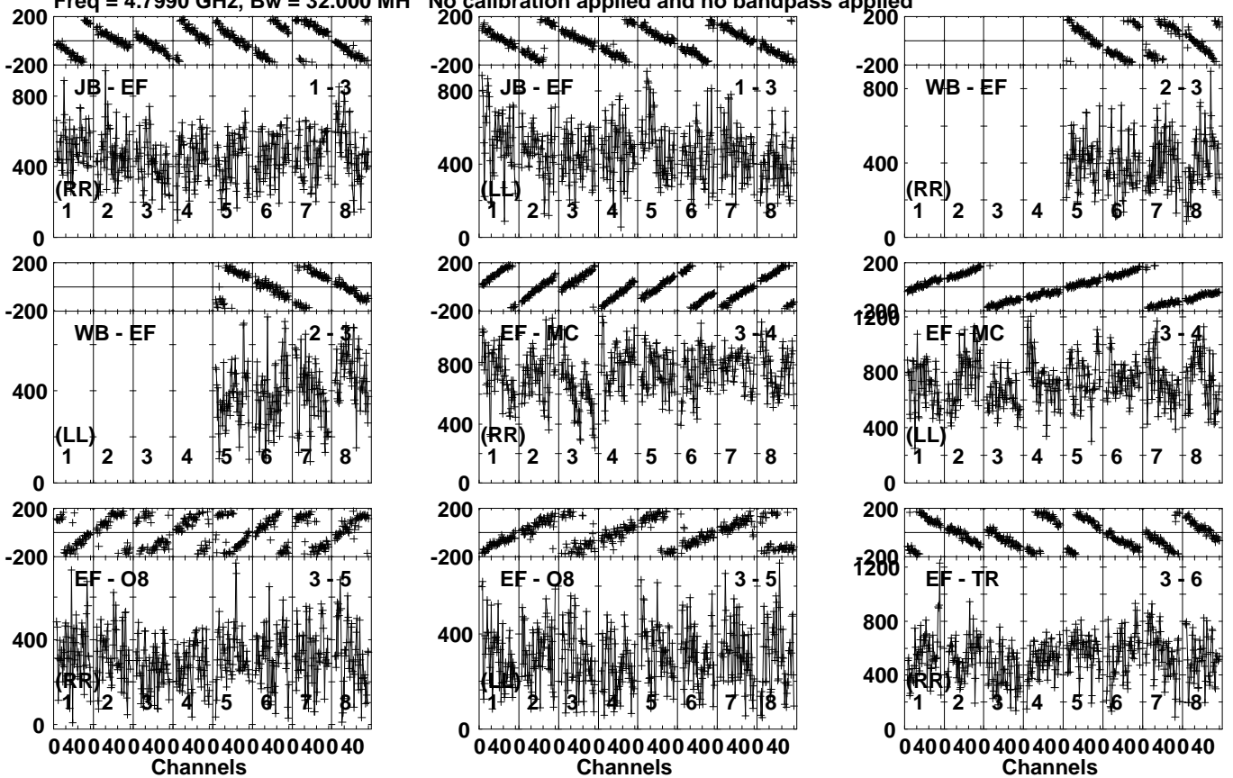
Lower frame: Micro Ampl Jy Top frame: Phas deg Vector averaged cross-power spectrum Several baselines displayed Timerange: 00/05:54:11 to 00/05:55:09
