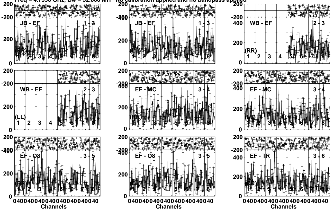
Lower frame: Micro Ampl Jy Top frame: Phas deg Vector averaged cross-power spectrum Several baselines displayed Timerange: 00/08:13:01 to 00/08:14:59
