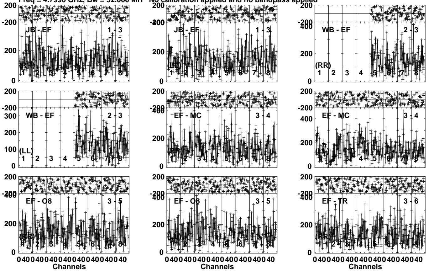
Lower frame: Micro Ampl Jy Top frame: Phas deg Vector averaged cross-power spectrum Several baselines displayed Timerange: 00/07:34:31 to 00/07:36:29
