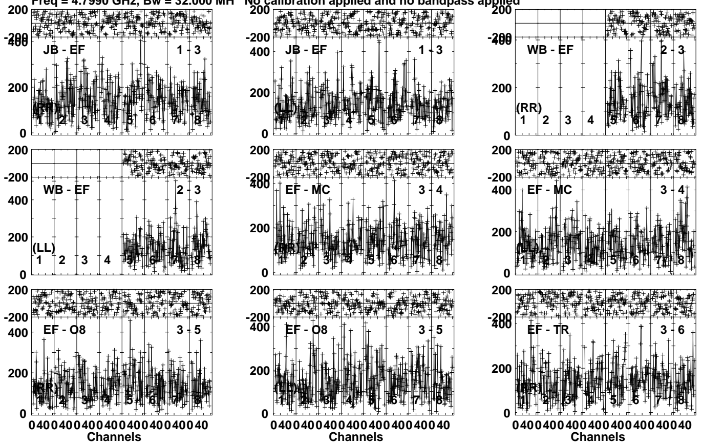
Lower frame: Micro Ampl Jy Top frame: Phas deg Vector averaged cross-power spectrum Several baselines displayed Timerange: 00/07:59:01 to 00/08:00:59
