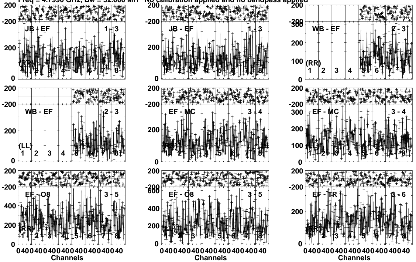
Lower frame: Micro Ampl Jy Top frame: Phas deg Vector averaged cross-power spectrum Several baselines displayed Timerange: 00/03:22:31 to 00/03:24:29
