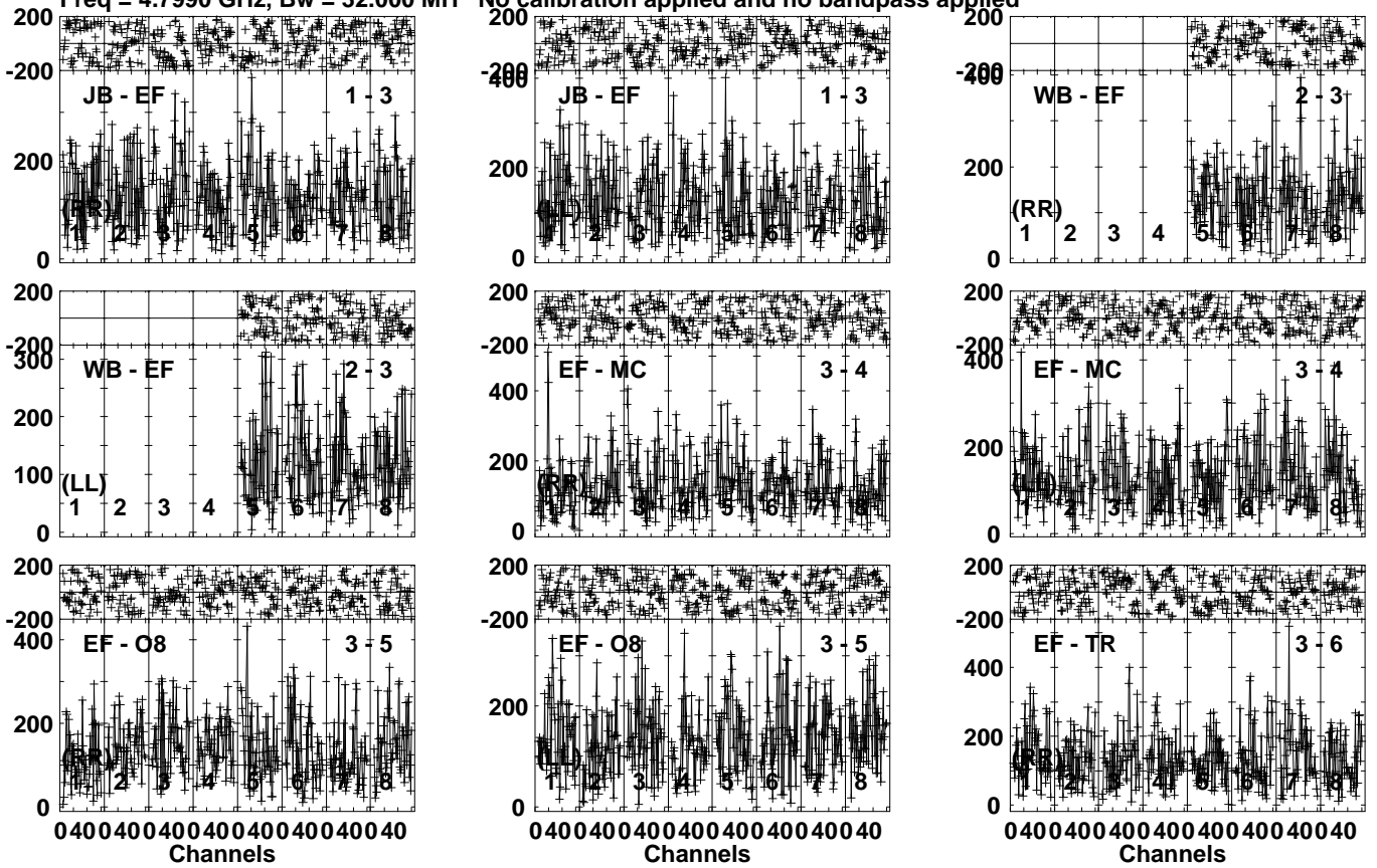
Lower frame: Micro Ampl Jy Top frame: Phas deg Vector averaged cross-power spectrum Several baselines displayed Timerange: 00/08:37:31 to 00/08:39:29
