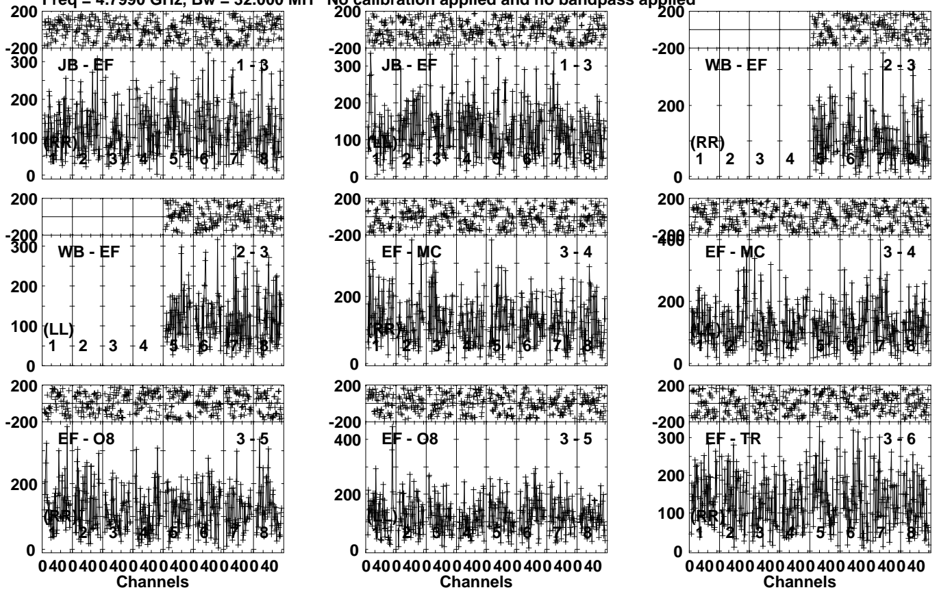
Lower frame: Micro Ampl Jy Top frame: Phas deg Vector averaged cross-power spectrum Several baselines displayed Timerange: 00/06:26:41 to 00/06:28:39
