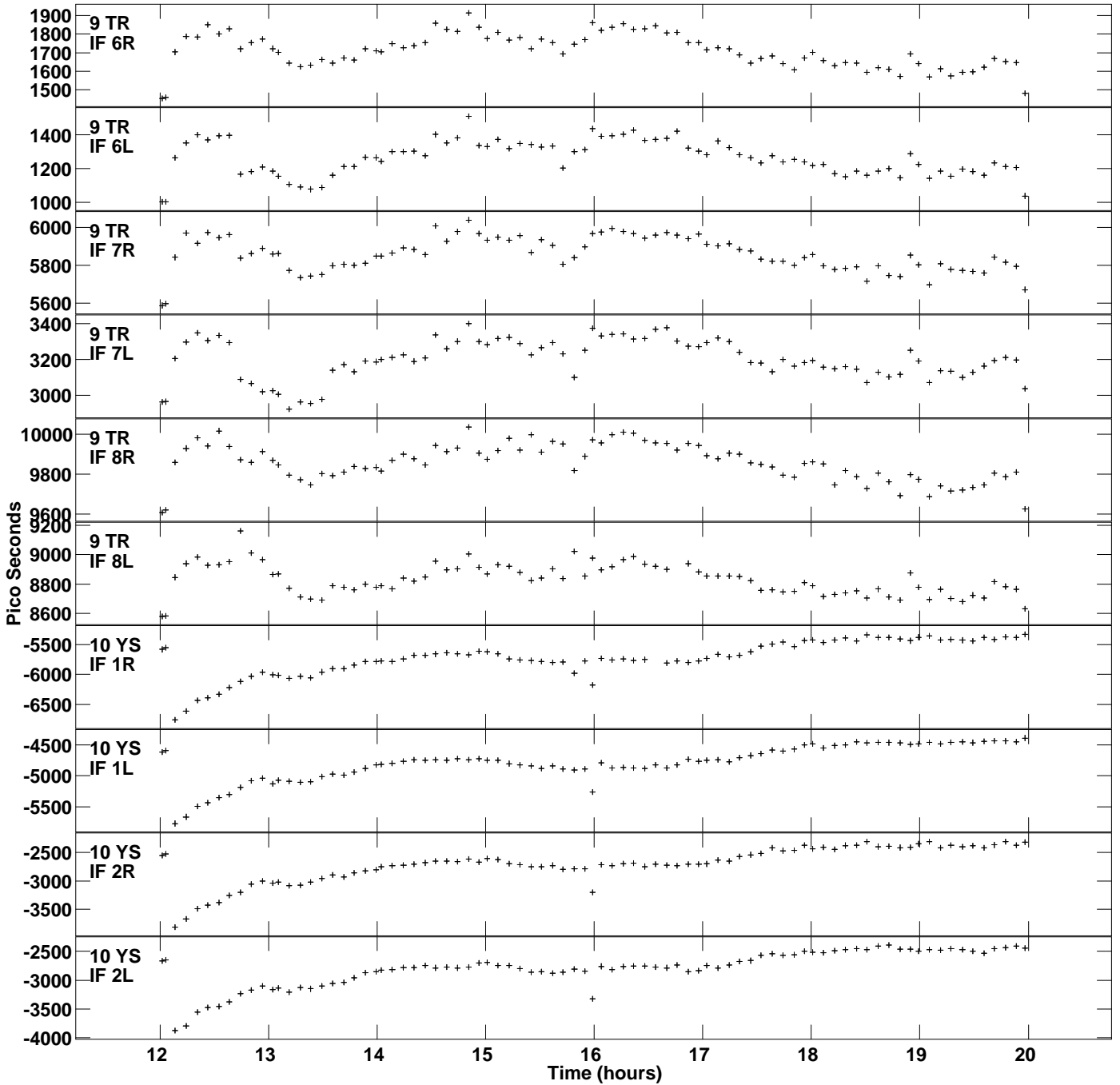
Plot file version 14 created 14-FEB-2023 14:24:38 Delay vs UTC time for EM166B.UVDATA.1 SN 3 Rpol & Lpol IF 1 - 8
