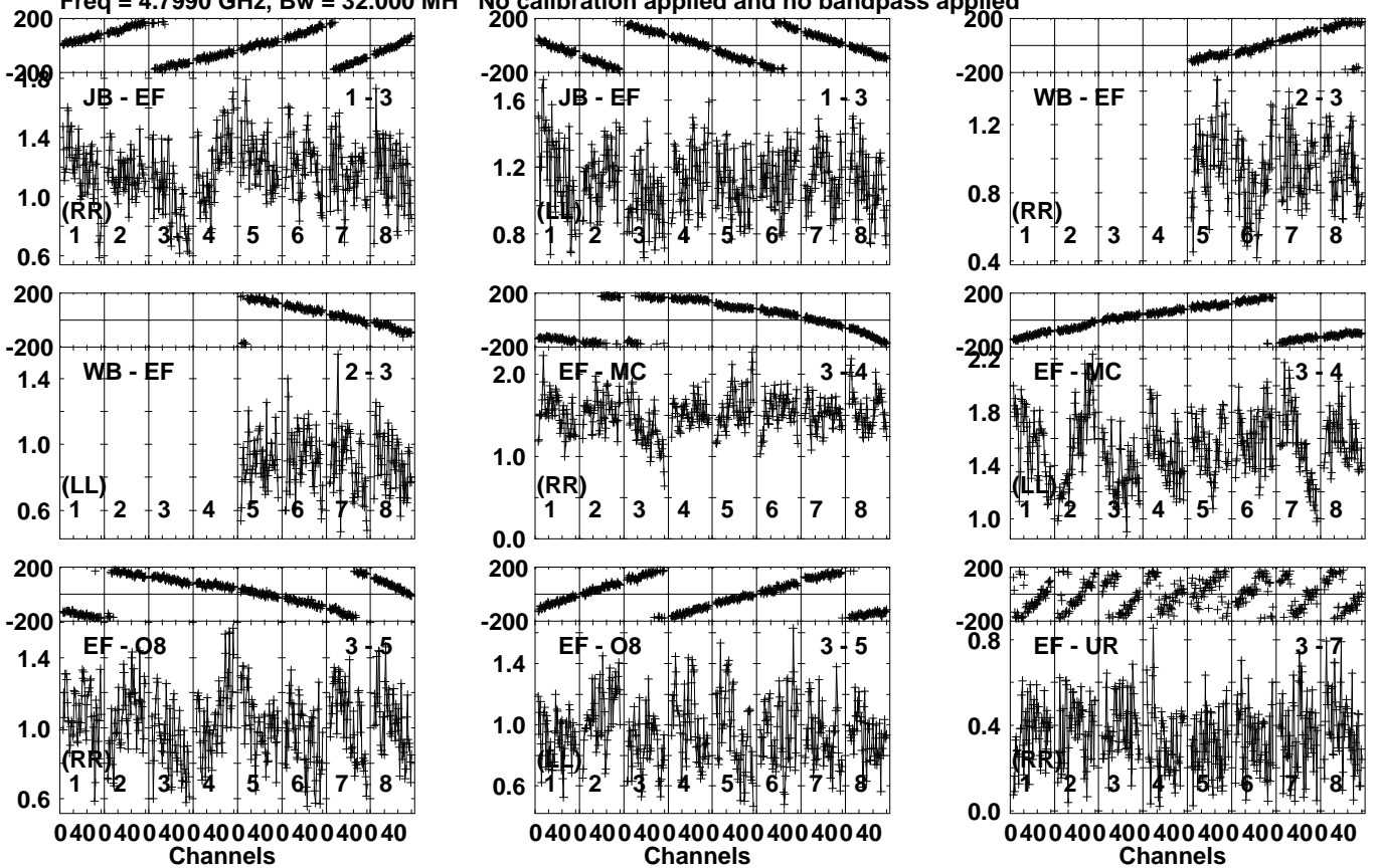
Lower frame: Milli Ampl Jy Top frame: Phas deg Vector averaged cross-power spectrum Several baselines displayed Timerange: 00/10:28:01 to 00/10:28:59
