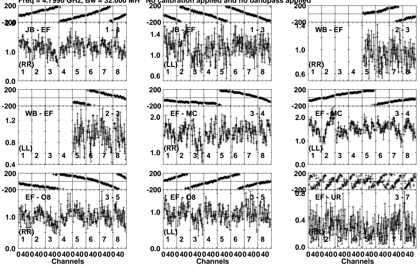
Lower frame: Milli Ampl Jy Top frame: Phas deg Vector averaged cross-power spectrum Several baselines displayed Timerange: 00/10:55:51 to 00/10:57:29
