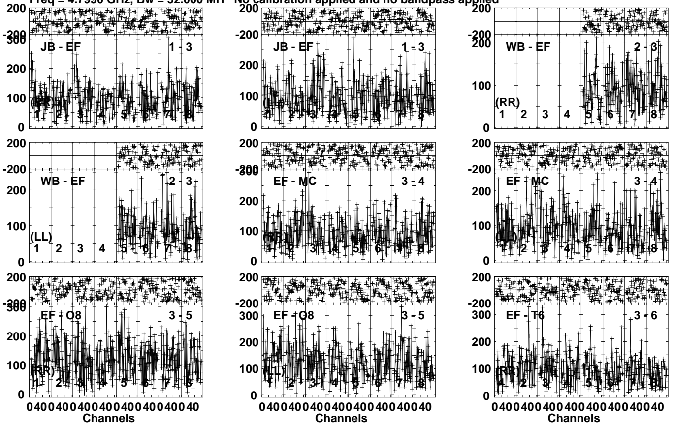
Lower frame: Micro Ampl Jy Top frame: Phas deg Vector averaged cross-power spectrum Several baselines displayed Timerange: 00/04:51:31 to 00/04:53:59
