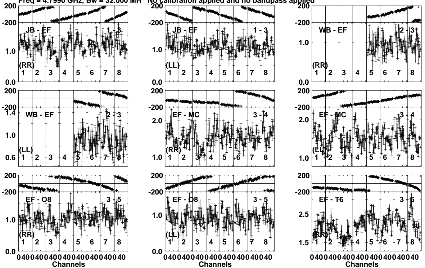
Lower frame: Milli Ampl Jy Top frame: Phas deg Vector averaged cross-power spectrum Several baselines displayed Timerange: 00/08:27:31 to 00/08:28:29
