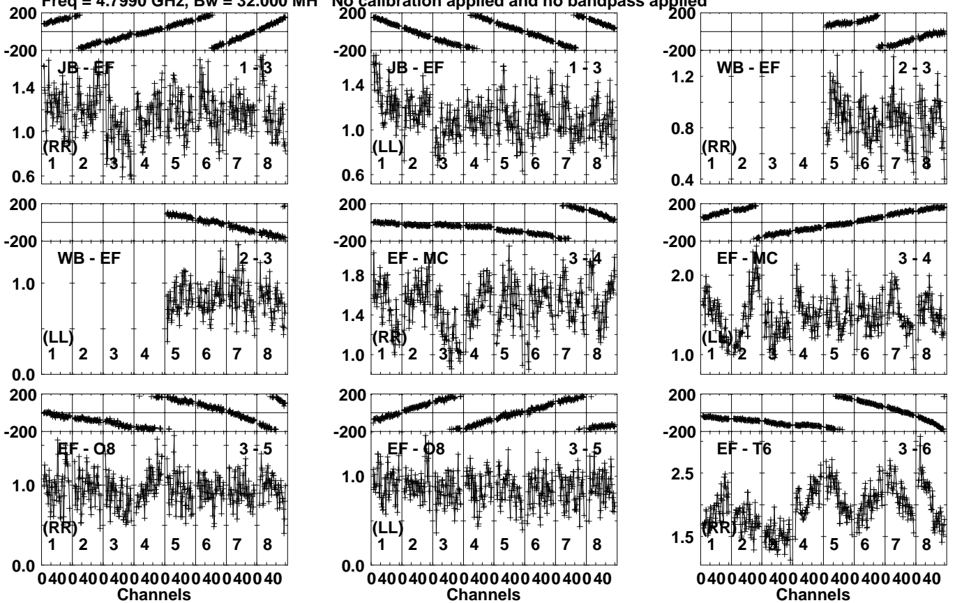
Lower frame: Milli Ampl Jy Top frame: Phas deg Vector averaged cross-power spectrum Several baselines displayed Timerange: 00/06:55:31 to 00/06:56:29
