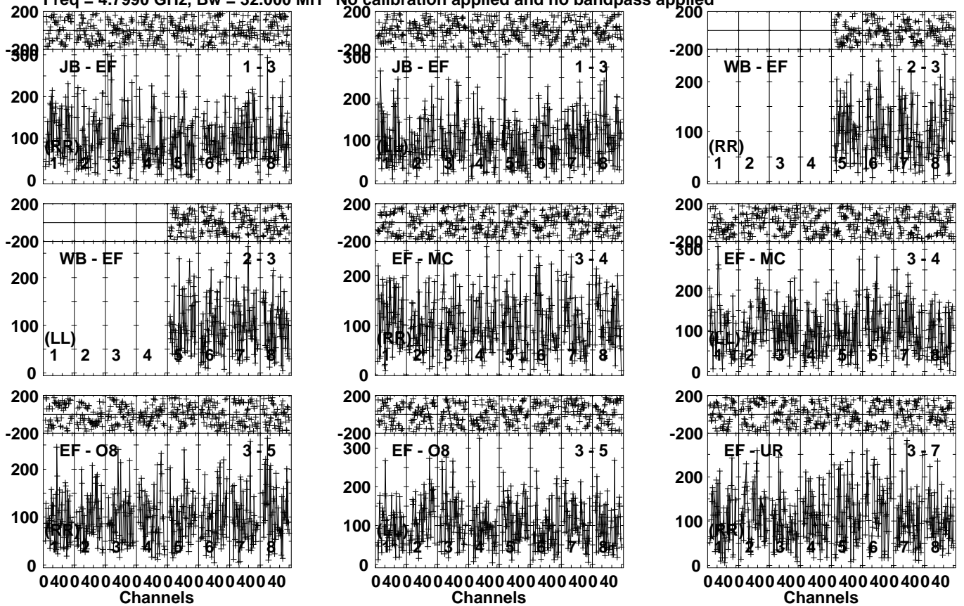
Lower frame: Micro Ampl Jy Top frame: Phas deg Vector averaged cross-power spectrum Several baselines displayed Timerange: 00/10:35:03 to 00/10:37:29
