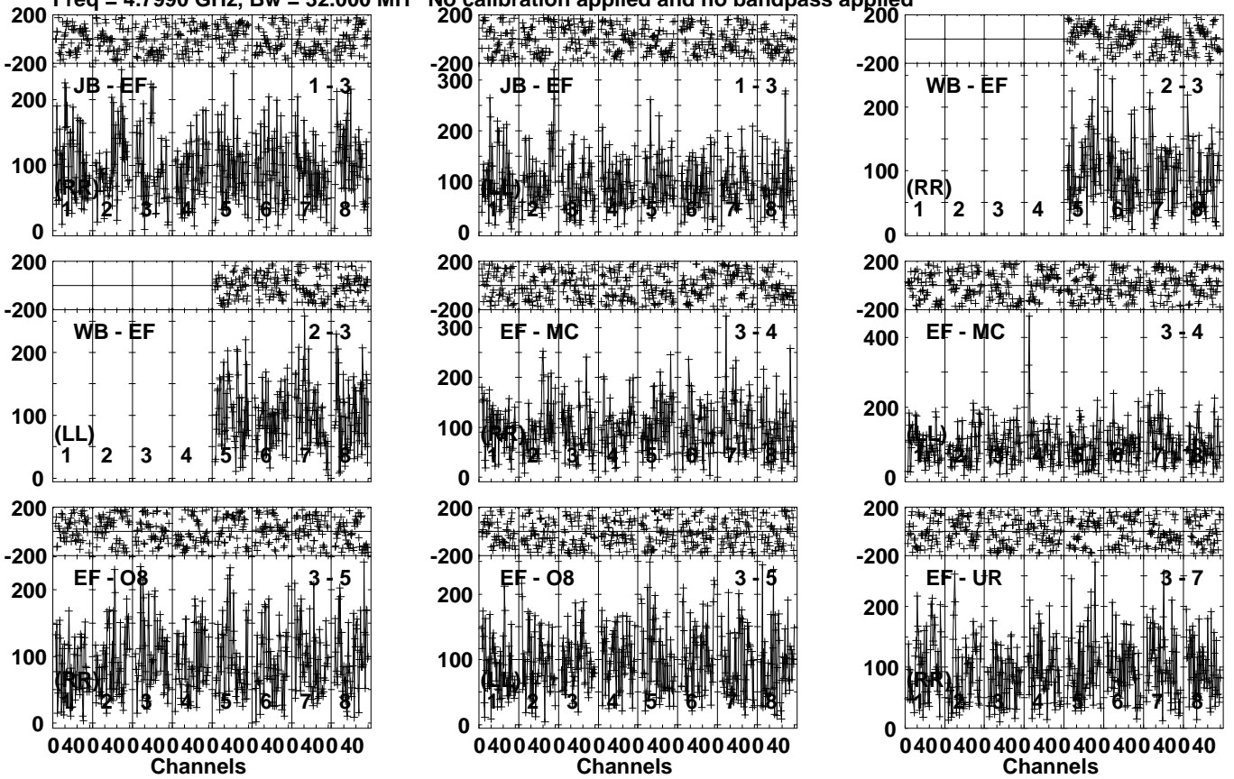
Lower frame: Micro Ampl Jy Top frame: Phas deg Vector averaged cross-power spectrum Several baselines displayed Timerange: 00/11:21:03 to 00/11:23:29
