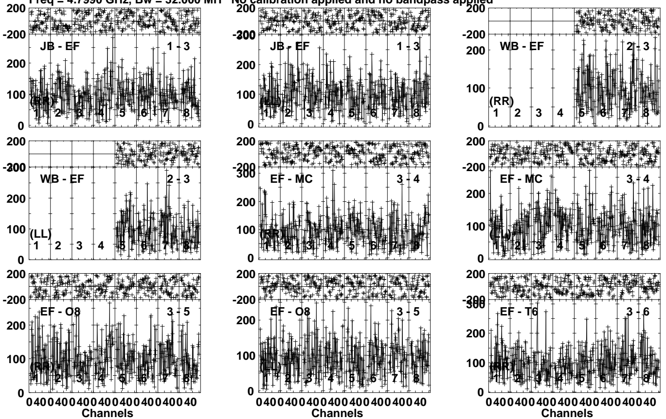
Lower frame: Micro Ampl Jy Top frame: Phas deg Vector averaged cross-power spectrum Several baselines displayed Timerange: 00/06:39:31 to 00/06:41:59
