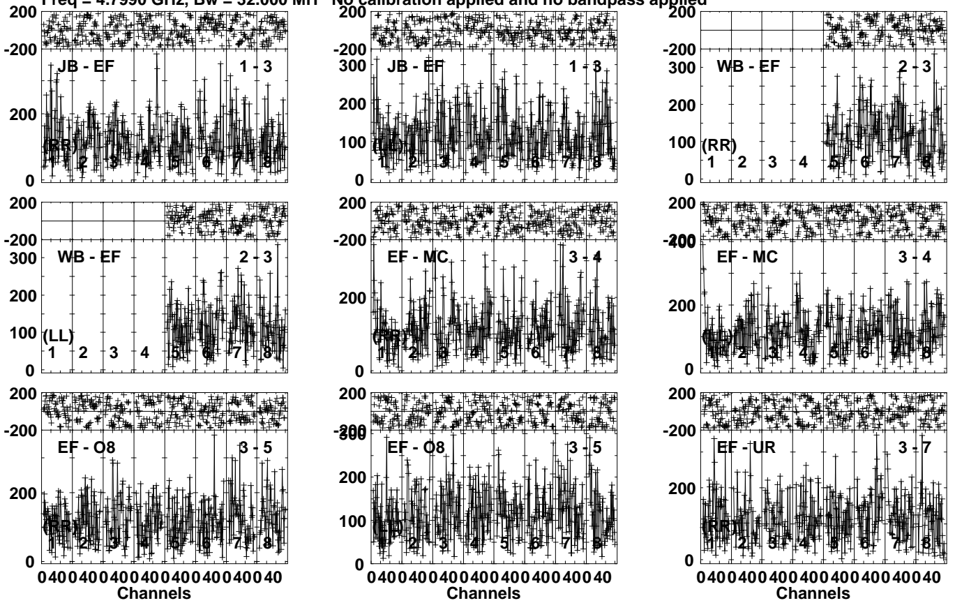
Lower frame: Micro Ampl Jy Top frame: Phas deg Vector averaged cross-power spectrum Several baselines displayed Timerange: 00/09:31:31 to 00/09:33:59
