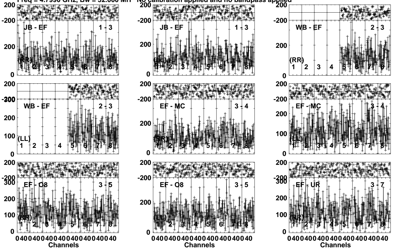
Lower frame: Micro Ampl Jy Top frame: Phas deg Vector averaged cross-power spectrum Several baselines displayed Timerange: 00/10:06:01 to 00/10:08:29
