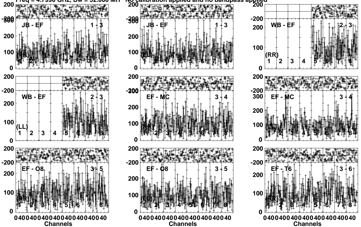
Lower frame: Micro Ampl Jy Top frame: Phas deg Vector averaged cross-power spectrum Several baselines displayed Timerange: 00/06:28:01 to 00/06:30:29
