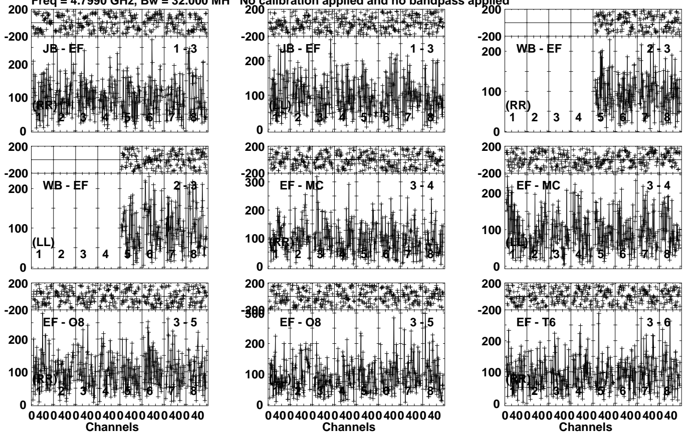
Lower frame: Micro Ampl Jy Top frame: Phas deg Vector averaged cross-power spectrum Several baselines displayed Timerange: 00/07:02:31 to 00/07:04:59
