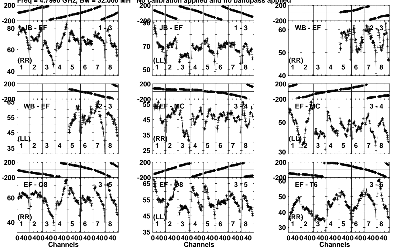
Lower frame: Milli Ampl Jy Top frame: Phas deg Vector averaged cross-power spectrum Several baselines displayed Timerange: 00/02:30:01 to 00/02:32:59
