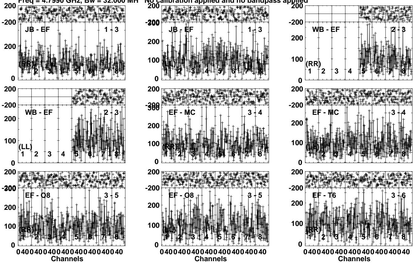
Lower frame: Micro Ampl Jy Top frame: Phas deg Vector averaged cross-power spectrum Several baselines displayed Timerange: 00/08:11:31 to 00/08:13:59
