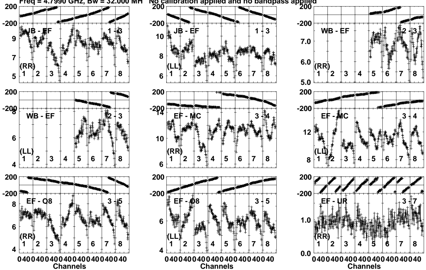
Lower frame: Milli Ampl Jy Top frame: Phas deg Vector averaged cross-power spectrum Several baselines displayed Timerange: 00/09:22:31 to 00/09:23:49
