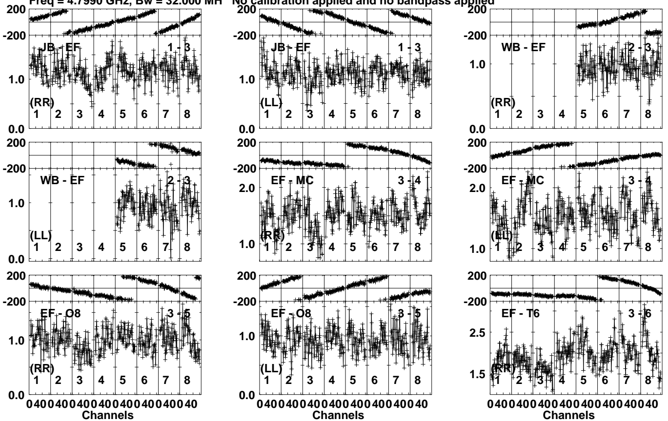
Lower frame: Milli Ampl Jy Top frame: Phas deg Vector averaged cross-power spectrum Several baselines displayed Timerange: 00/09:12:21 to 00/09:13:59
