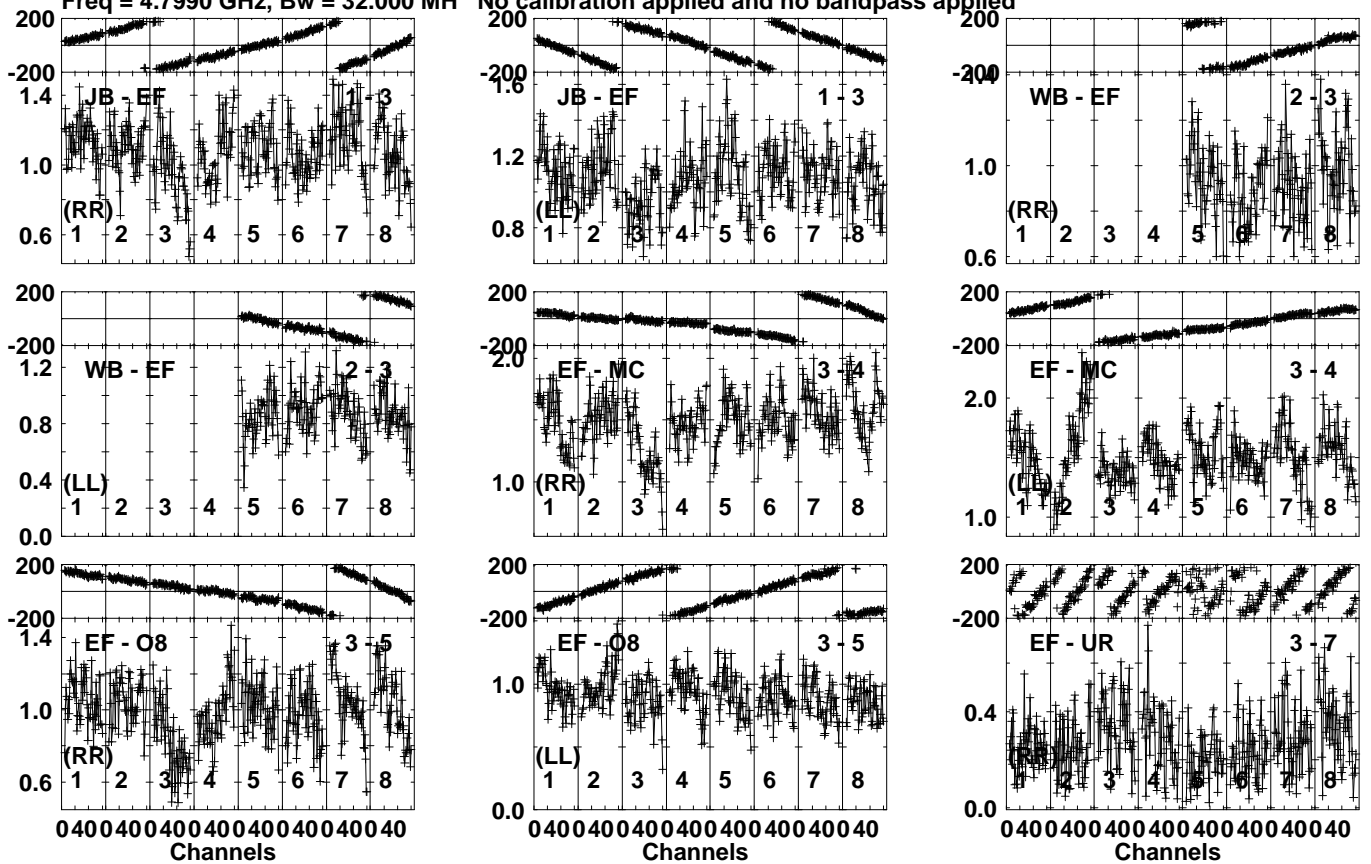
Lower frame: Milli Ampl Jy Top frame: Phas deg Vector averaged cross-power spectrum Several baselines displayed Timerange: 00/11:18:51 to 00/11:20:29
