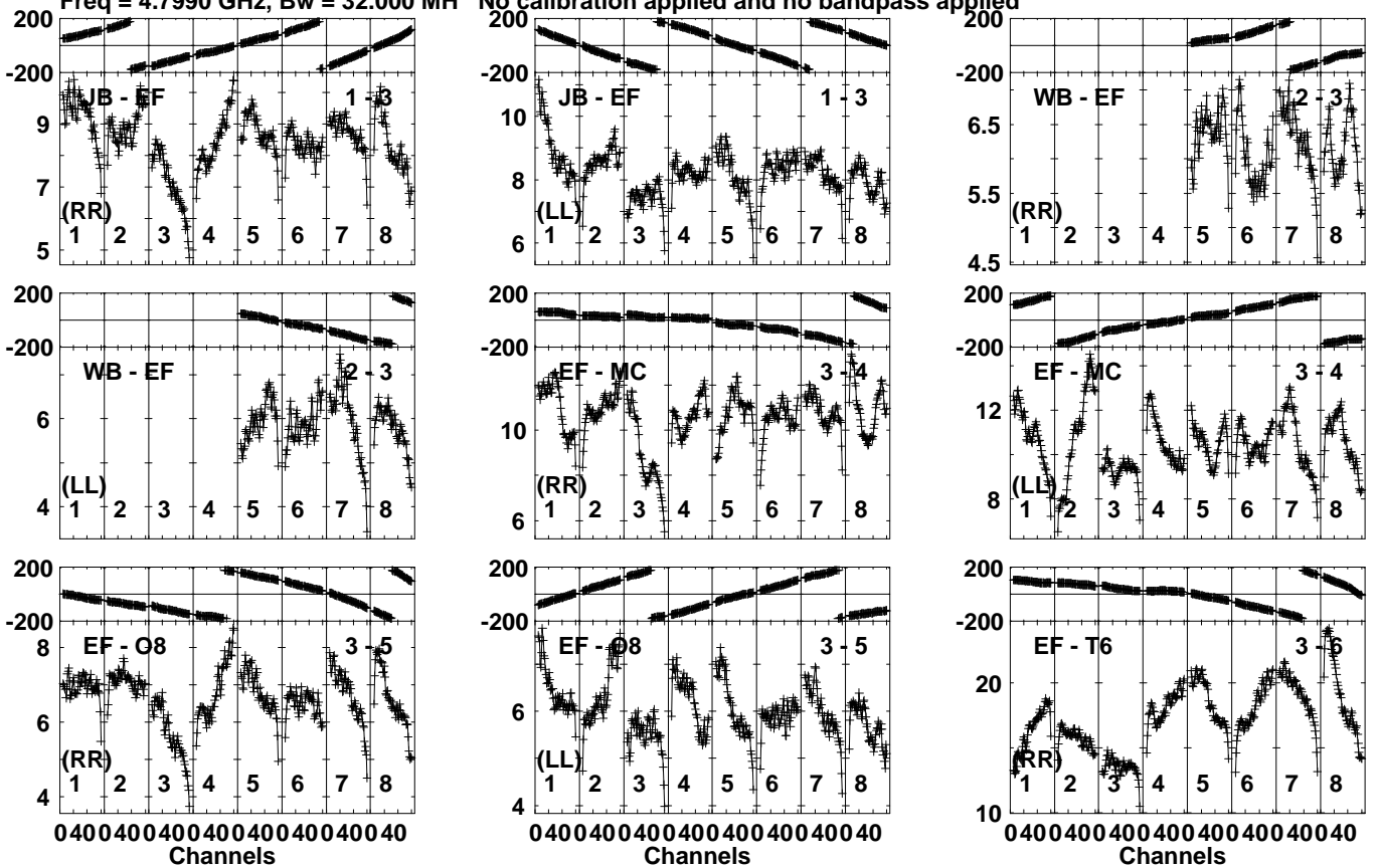
Lower frame: Milli Ampl Jy Top frame: Phas deg Vector averaged cross-power spectrum Several baselines displayed Timerange: 00/06:47:31 to 00/06:48:49
