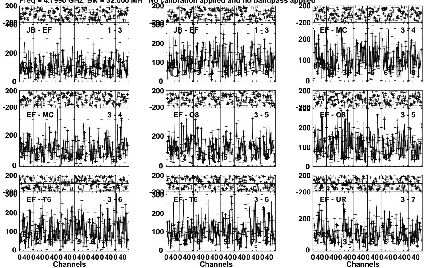
Lower frame: Micro Ampl Jy Top frame: Phas deg Vector averaged cross-power spectrum Several baselines displayed Timerange: 00/03:59:31 to 00/04:01:59
