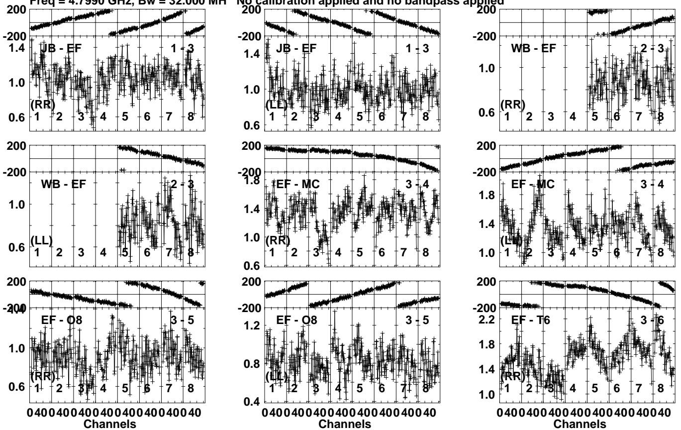
Lower frame: Milli Ampl Jy Top frame: Phas deg Vector averaged cross-power spectrum Several baselines displayed Timerange: 00/05:12:21 to 00/05:13:59
