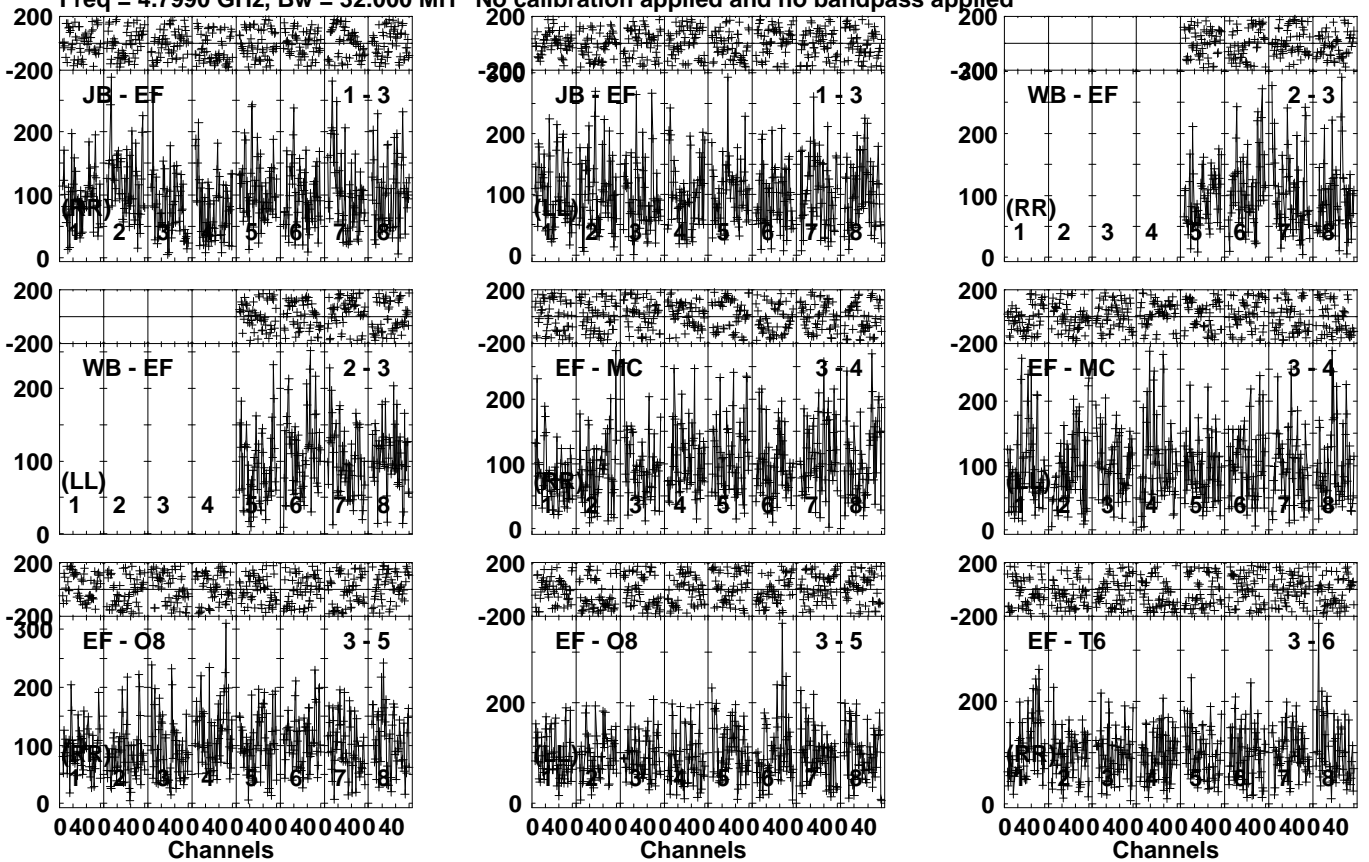
Lower frame: Micro Ampl Jy Top frame: Phas deg Vector averaged cross-power spectrum Several baselines displayed Timerange: 00/07:48:31 to 00/07:50:59
