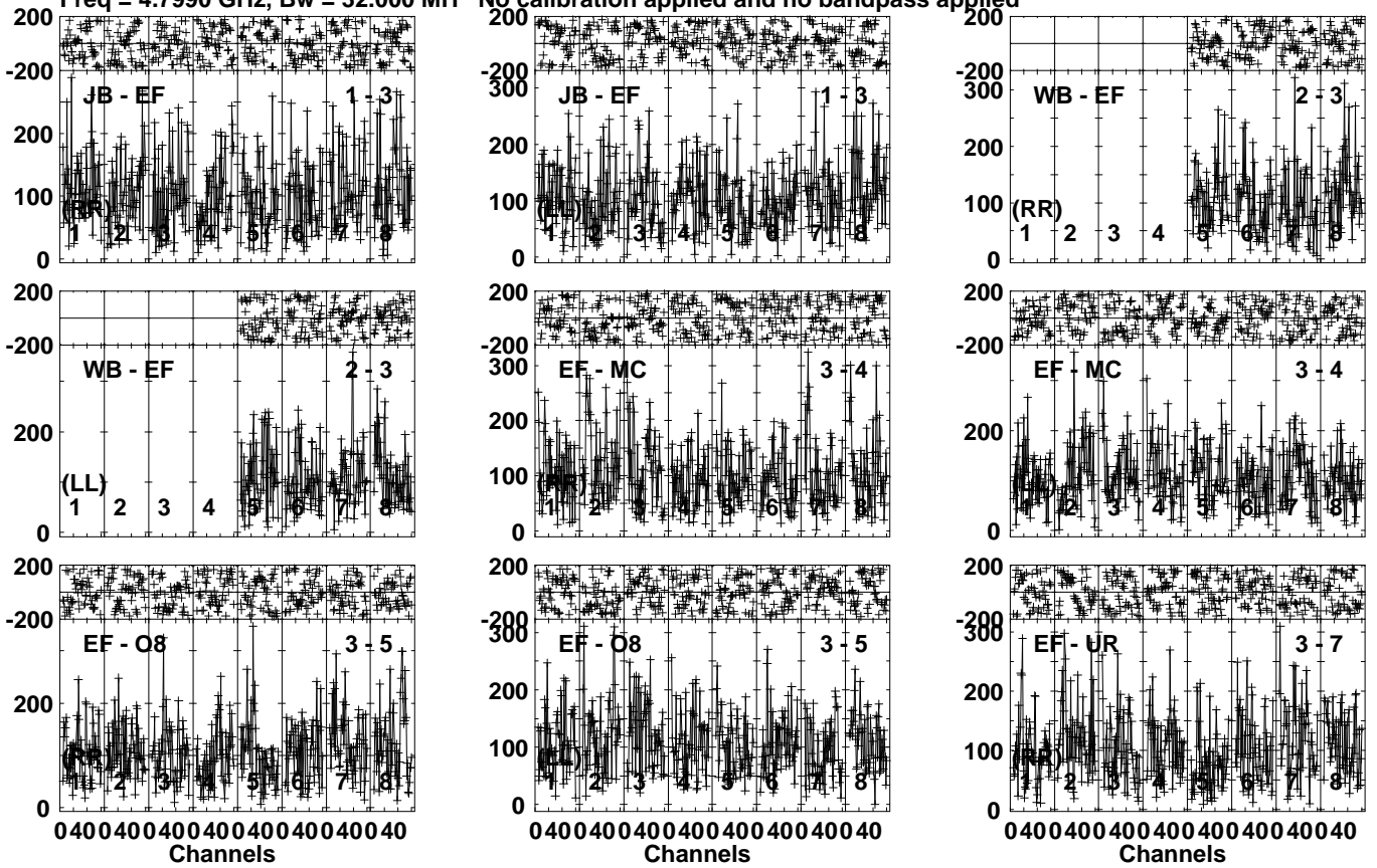
Lower frame: Micro Ampl Jy Top frame: Phas deg Vector averaged cross-power spectrum Several baselines displayed Timerange: 00/11:26:31 to 00/11:28:59
