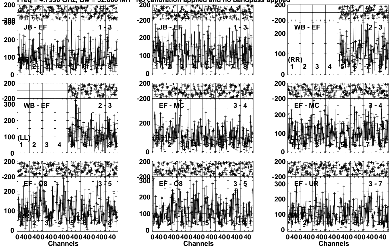
Lower frame: Micro Ampl Jy Top frame: Phas deg Vector averaged cross-power spectrum Several baselines displayed Timerange: 00/11:49:31 to 00/11:51:59
