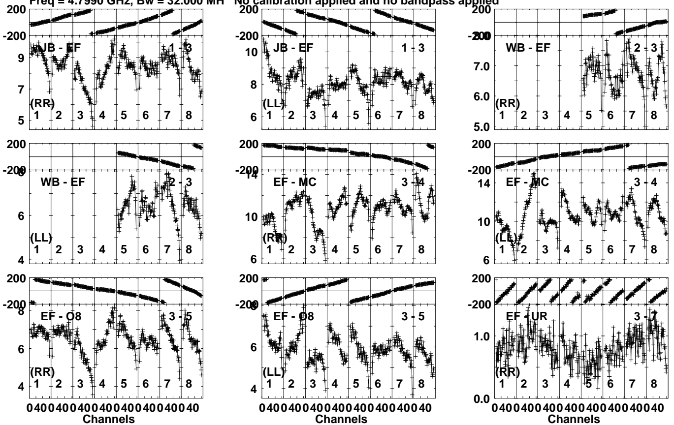
Lower frame: Milli Ampl Jy Top frame: Phas deg Vector averaged cross-power spectrum Several baselines displayed Timerange: 00/09:28:33 to 00/09:29:49
