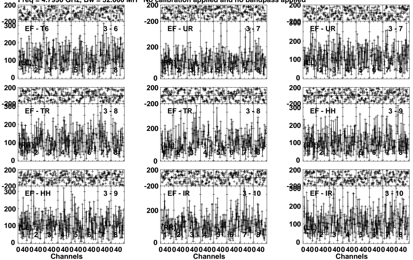
Lower frame: Micro Ampl Jy Top frame: Phas deg Vector averaged cross-power spectrum Several baselines displayed Timerange: 00/05:52:33 to 00/05:54:59
