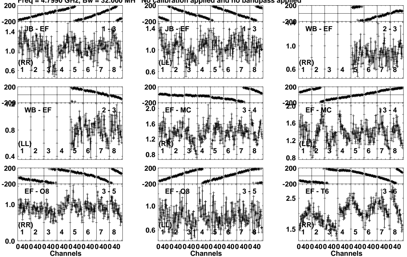
Lower frame: Milli Ampl Jy Top frame: Phas deg Vector averaged cross-power spectrum Several baselines displayed Timerange: 00/05:42:01 to 00/05:42:59
