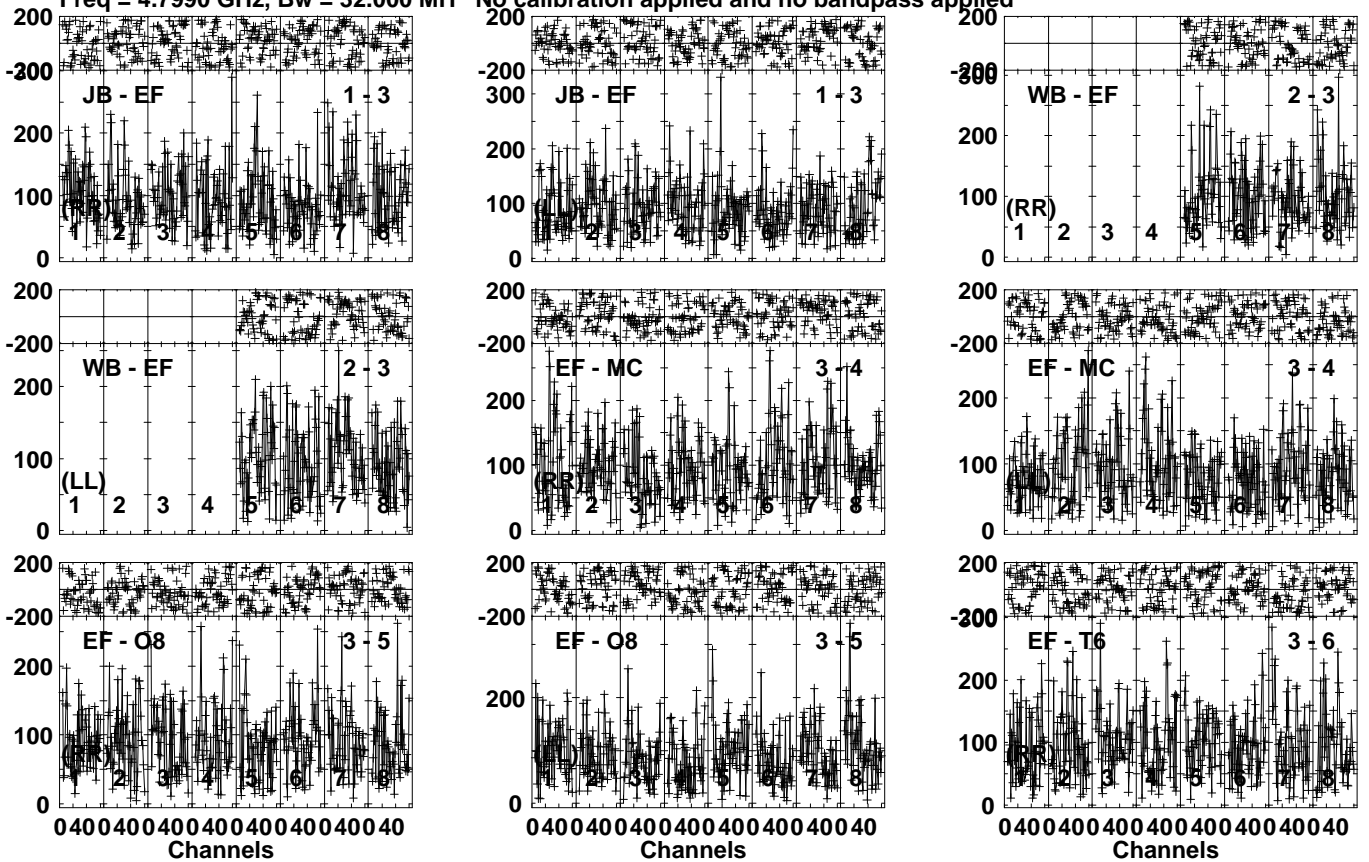
Lower frame: Micro Ampl Jy Top frame: Phas deg Vector averaged cross-power spectrum Several baselines displayed Timerange: 00/04:28:31 to 00/04:30:59
