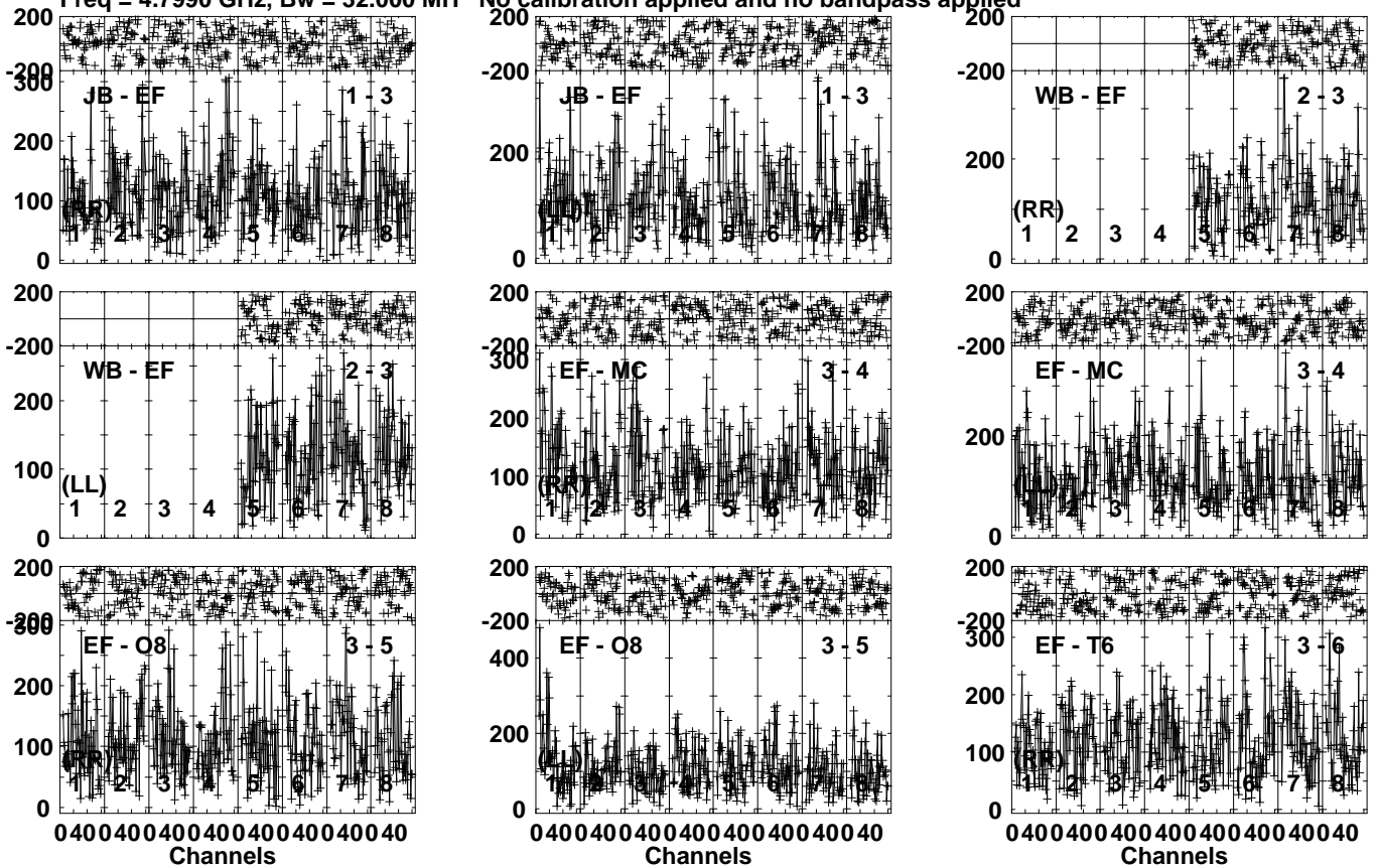
Lower frame: Micro Ampl Jy Top frame: Phas deg Vector averaged cross-power spectrum Several baselines displayed Timerange: 00/08:05:31 to 00/08:07:59
