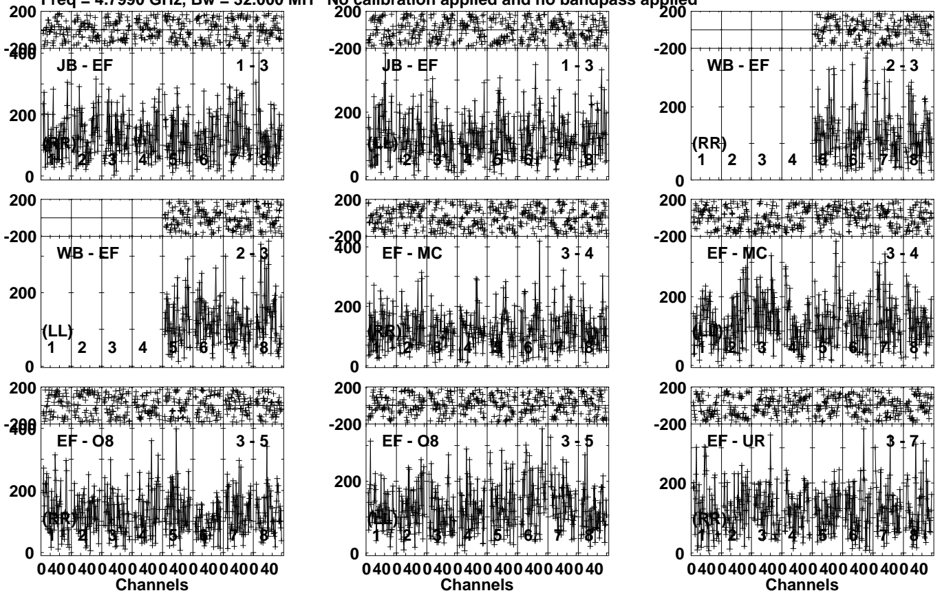
Lower frame: Micro Ampl Jy Top frame: Phas deg Vector averaged cross-power spectrum Several baselines displayed Timerange: 00/10:29:01 to 00/10:31:29
