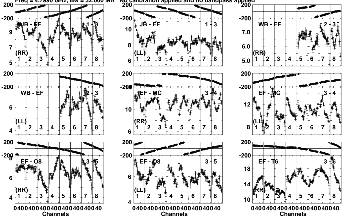
Lower frame: Milli Ampl Jy Top frame: Phas deg Vector averaged cross-power spectrum Several baselines displayed Timerange: 00/07:51:03 to 00/07:52:19
