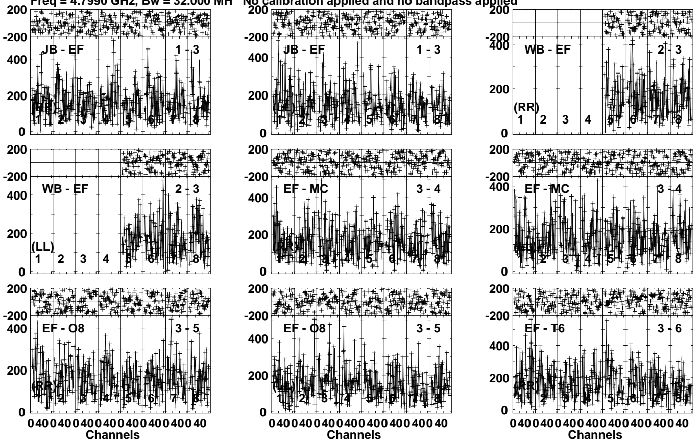
Lower frame: Micro Ampl Jy Top frame: Phas deg Vector averaged cross-power spectrum Several baselines displayed Timerange: 00/07:07:01 to 00/07:07:59
