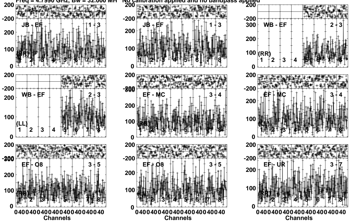
Lower frame: Micro Ampl Jy Top frame: Phas deg Vector averaged cross-power spectrum Several baselines displayed Timerange: 00/10:12:03 to 00/10:14:29
