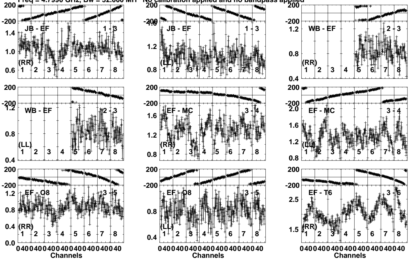
Lower frame: Milli Ampl Jy Top frame: Phas deg Vector averaged cross-power spectrum Several baselines displayed Timerange: 00/05:35:21 to 00/05:36:59
