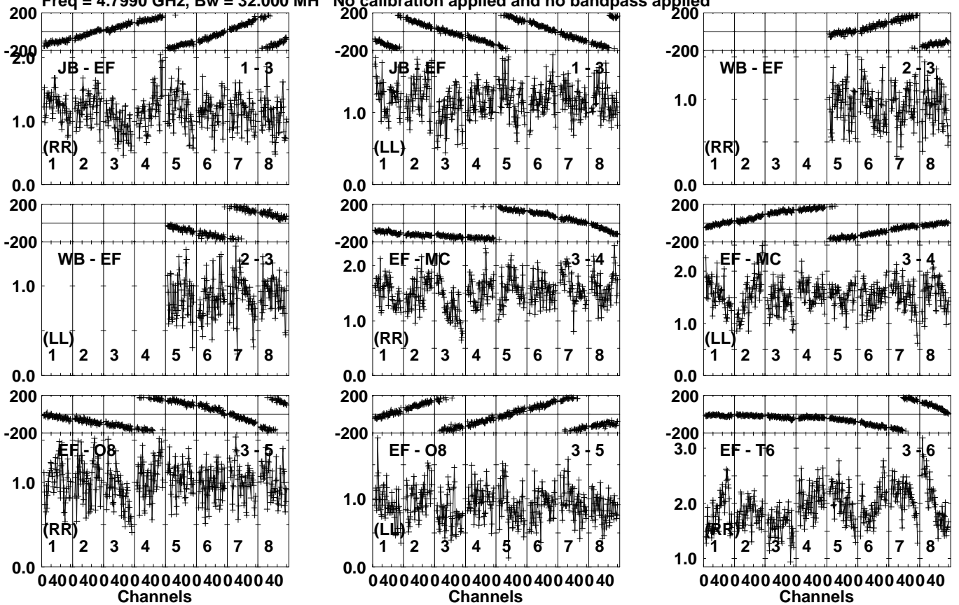
Lower frame: Milli Ampl Jy Top frame: Phas deg Vector averaged cross-power spectrum Several baselines displayed Timerange: 00/09:19:01 to 00/09:19:59
