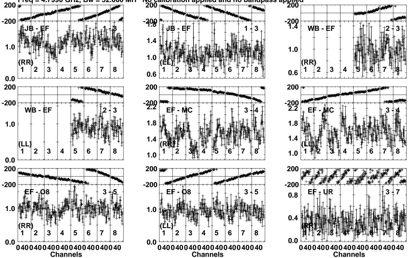
Lower frame: Milli Ampl Jy Top frame: Phas deg Vector averaged cross-power spectrum Several baselines displayed Timerange: 00/10:44:21 to 00/10:45:59
