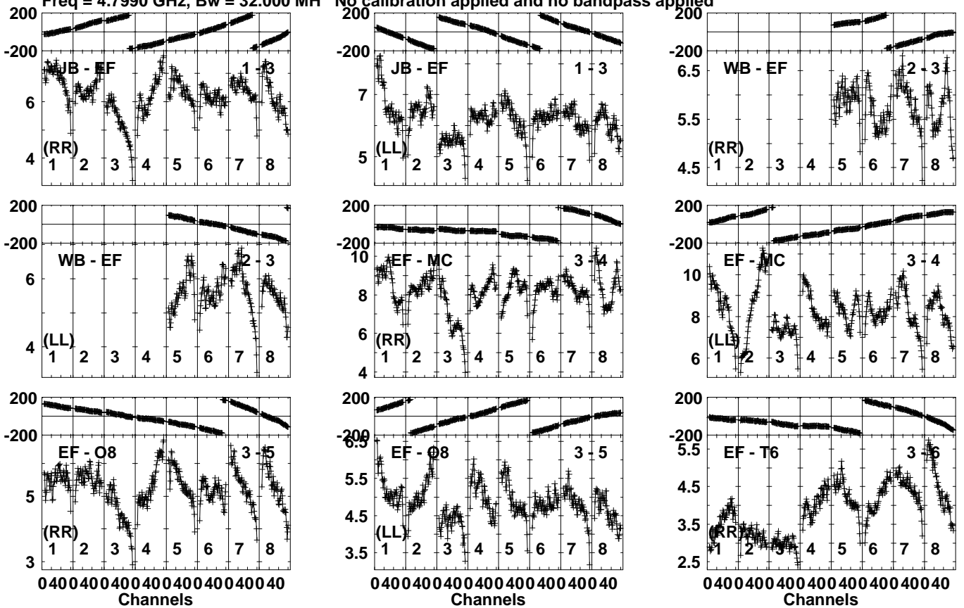
Lower frame: Milli Ampl Jy Top frame: Phas deg Vector averaged cross-power spectrum Several baselines displayed Timerange: 00/04:13:31 to 00/04:14:49
