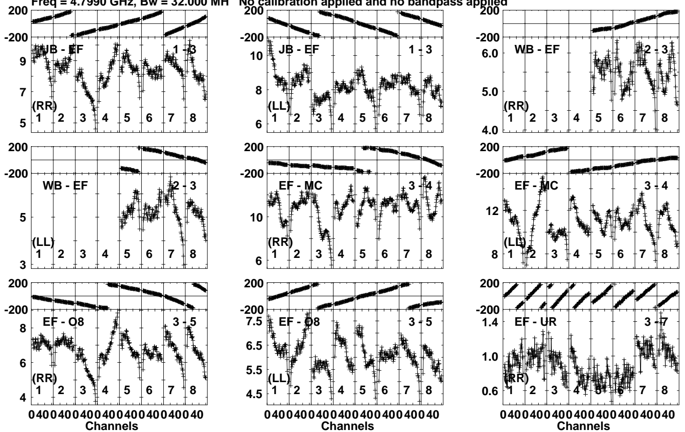
Lower frame: Milli Ampl Jy Top frame: Phas deg Vector averaged cross-power spectrum Several baselines displayed Timerange: 00/09:11:01 to 00/09:12:19
