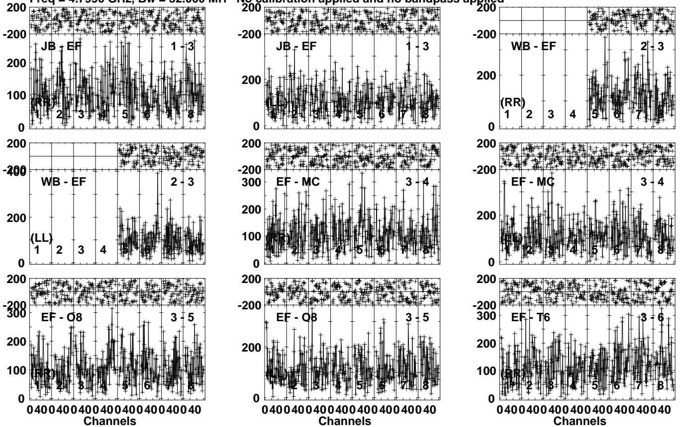
Lower frame: Micro Ampl Jy Top frame: Phas deg Vector averaged cross-power spectrum Several baselines displayed Timerange: 00/06:56:31 to 00/06:58:59
