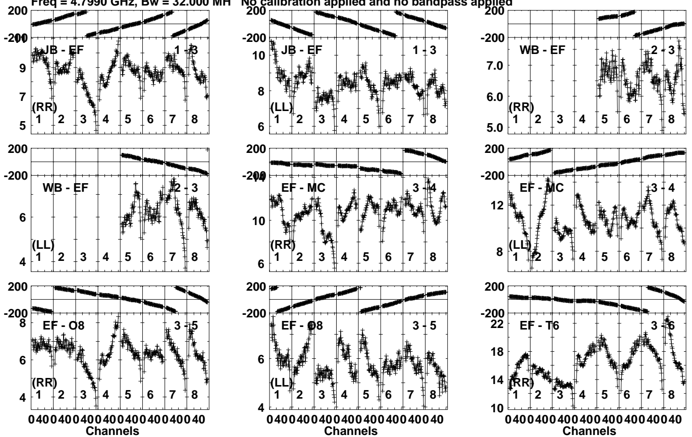
Lower frame: Milli Ampl Jy Top frame: Phas deg Vector averaged cross-power spectrum Several baselines displayed Timerange: 00/07:33:31 to 00/07:34:49
