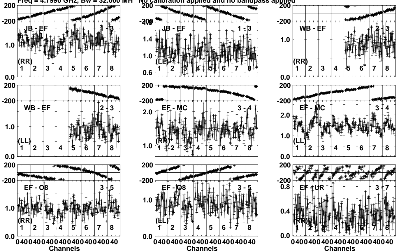
Lower frame: Milli Ampl Jy Top frame: Phas deg Vector averaged cross-power spectrum Several baselines displayed Timerange: 00/10:09:51 to 00/10:11:29
