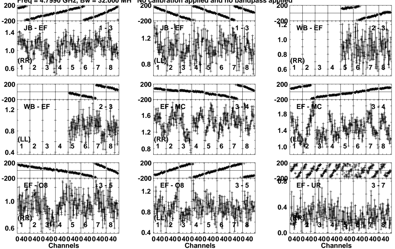
Lower frame: Milli Ampl Jy Top frame: Phas deg Vector averaged cross-power spectrum Several baselines displayed Timerange: 00/11:41:53 to 00/11:43:29
