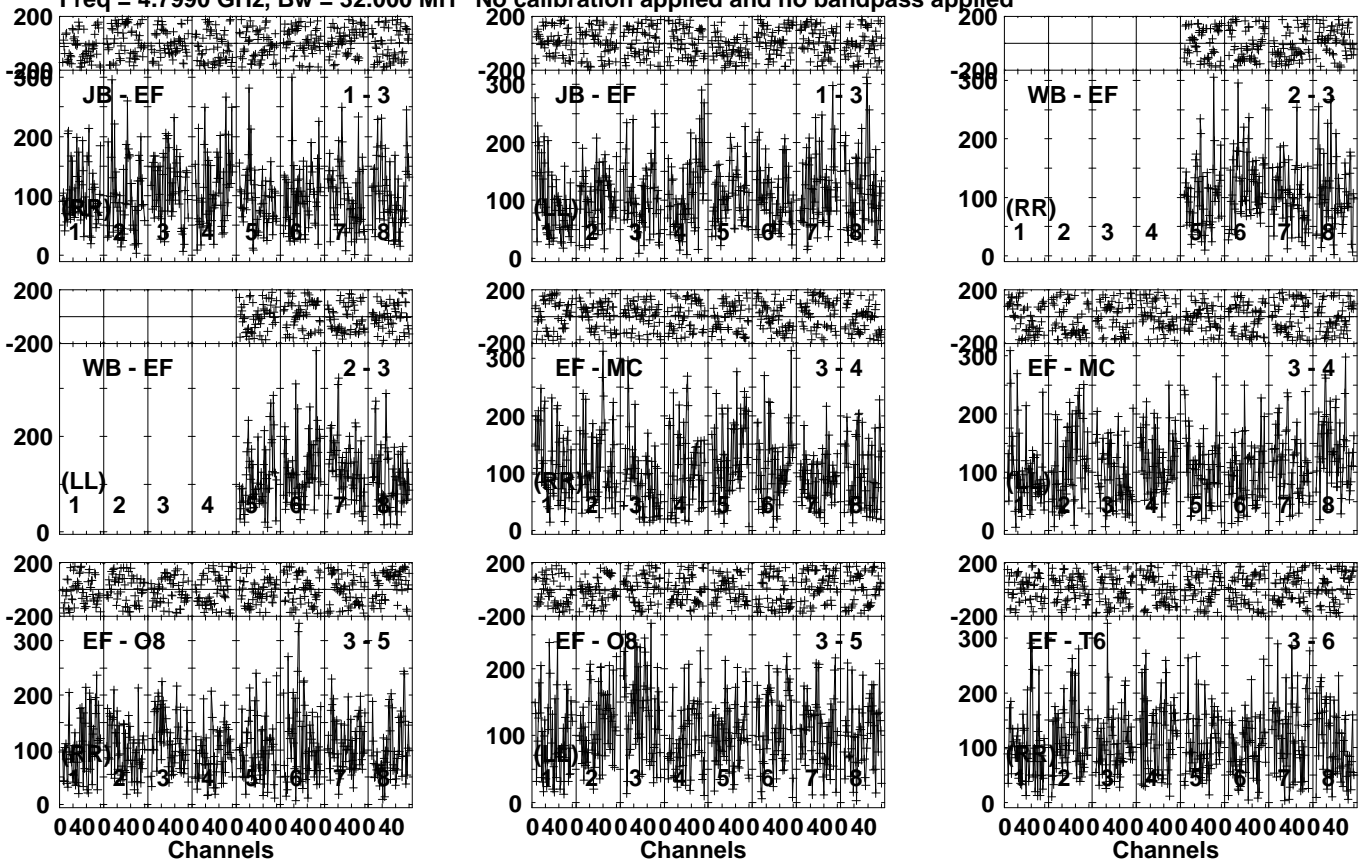
Lower frame: Micro Ampl Jy Top frame: Phas deg Vector averaged cross-power spectrum Several baselines displayed Timerange: 00/06:10:31 to 00/06:12:59
