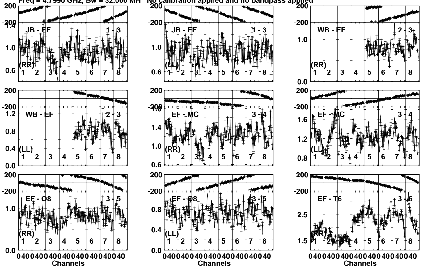
Lower frame: Milli Ampl Jy Top frame: Phas deg Vector averaged cross-power spectrum Several baselines displayed Timerange: 00/04:26:21 to 00/04:27:59
