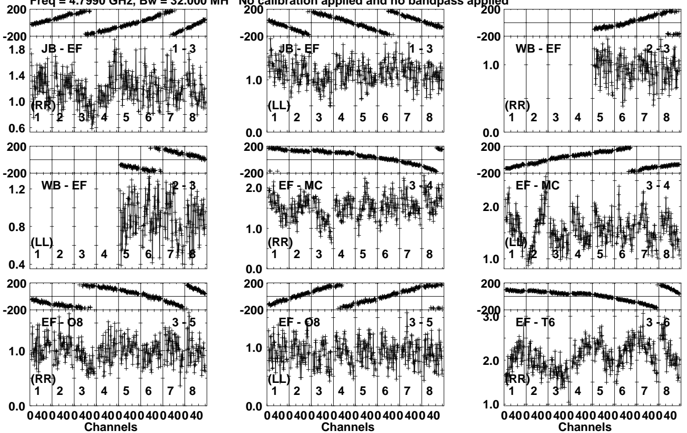
Lower frame: Milli Ampl Jy Top frame: Phas deg Vector averaged cross-power spectrum Several baselines displayed Timerange: 00/08:39:01 to 00/08:39:59
