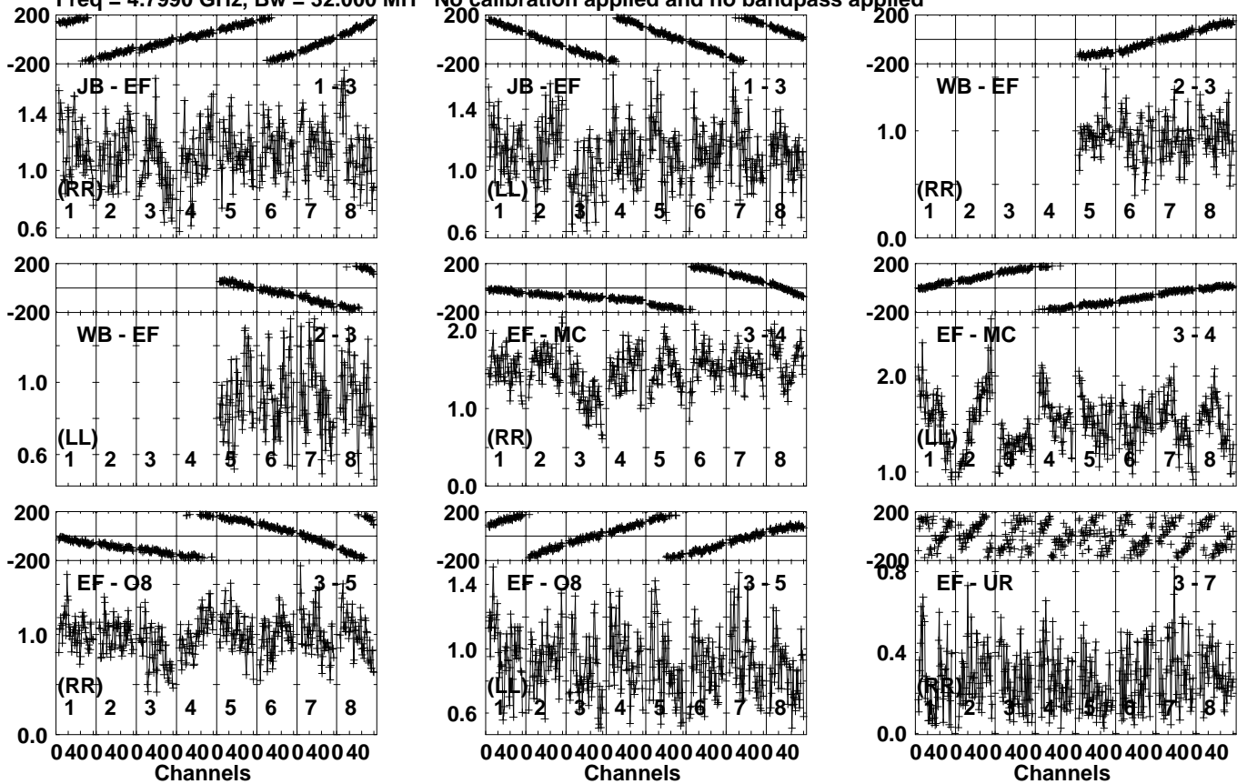
Lower frame: Milli Ampl Jy Top frame: Phas deg Vector averaged cross-power spectrum Several baselines displayed Timerange: 00/12:16:11 to 00/12:17:39
