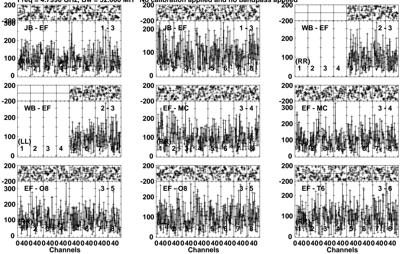
Lower frame: Micro Ampl Jy Top frame: Phas deg Vector averaged cross-power spectrum Several baselines displayed Timerange: 00/05:03:01 to 00/05:05:29
