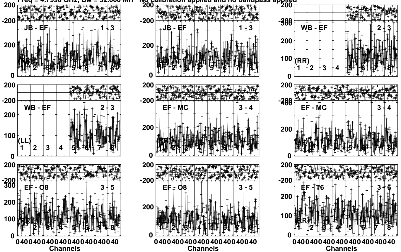
Lower frame: Micro Ampl Jy Top frame: Phas deg Vector averaged cross-power spectrum Several baselines displayed Timerange: 00/07:19:31 to 00/07:21:59
