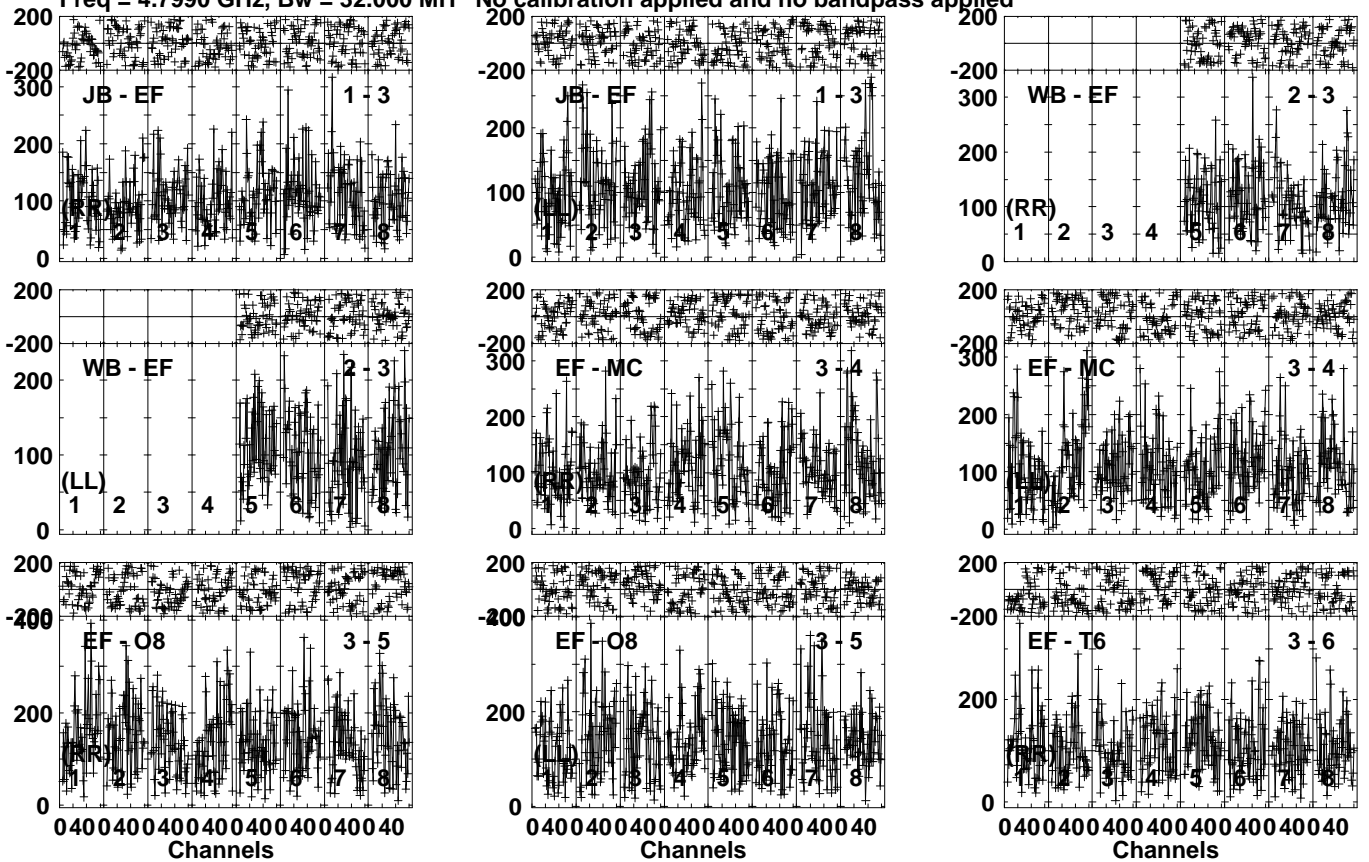
Lower frame: Micro Ampl Jy Top frame: Phas deg Vector averaged cross-power spectrum Several baselines displayed Timerange: 00/04:34:01 to 00/04:36:29
