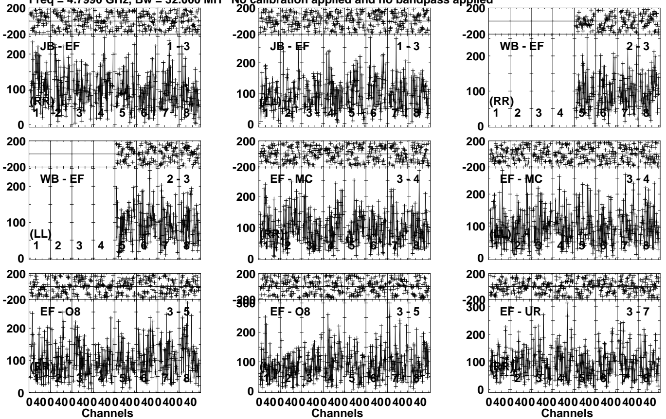
Lower frame: Micro Ampl Jy Top frame: Phas deg Vector averaged cross-power spectrum Several baselines displayed Timerange: 00/10:23:33 to 00/10:25:59
