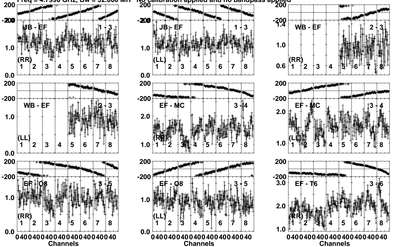
Lower frame: Milli Ampl Jy Top frame: Phas deg Vector averaged cross-power spectrum Several baselines displayed Timerange: 00/08:50:31 to 00/08:51:29
