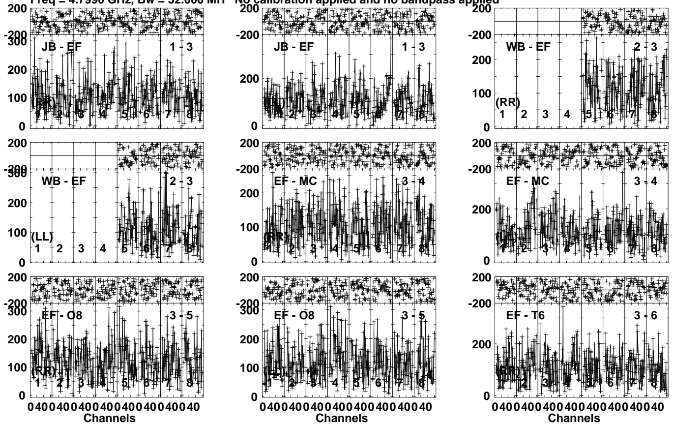
Lower frame: Micro Ampl Jy Top frame: Phas deg Vector averaged cross-power spectrum Several baselines displayed Timerange: 00/06:33:31 to 00/06:35:59
