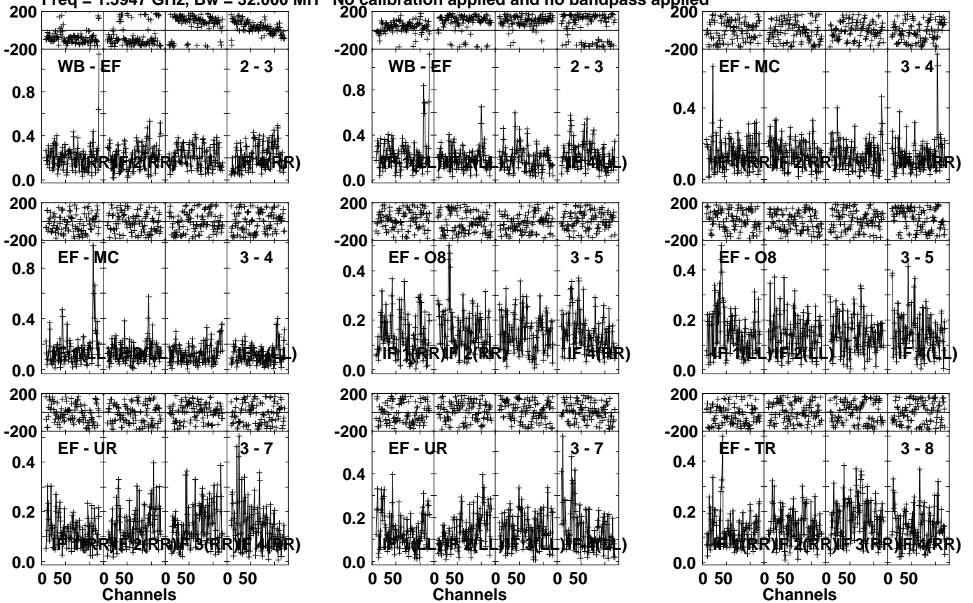
Lower frame: Milli Ampl Jy Top frame: Phas deg Vector averaged cross-power spectrum Several baselines displayed Timerange: 00/16:18:31 to 00/16:20:29
