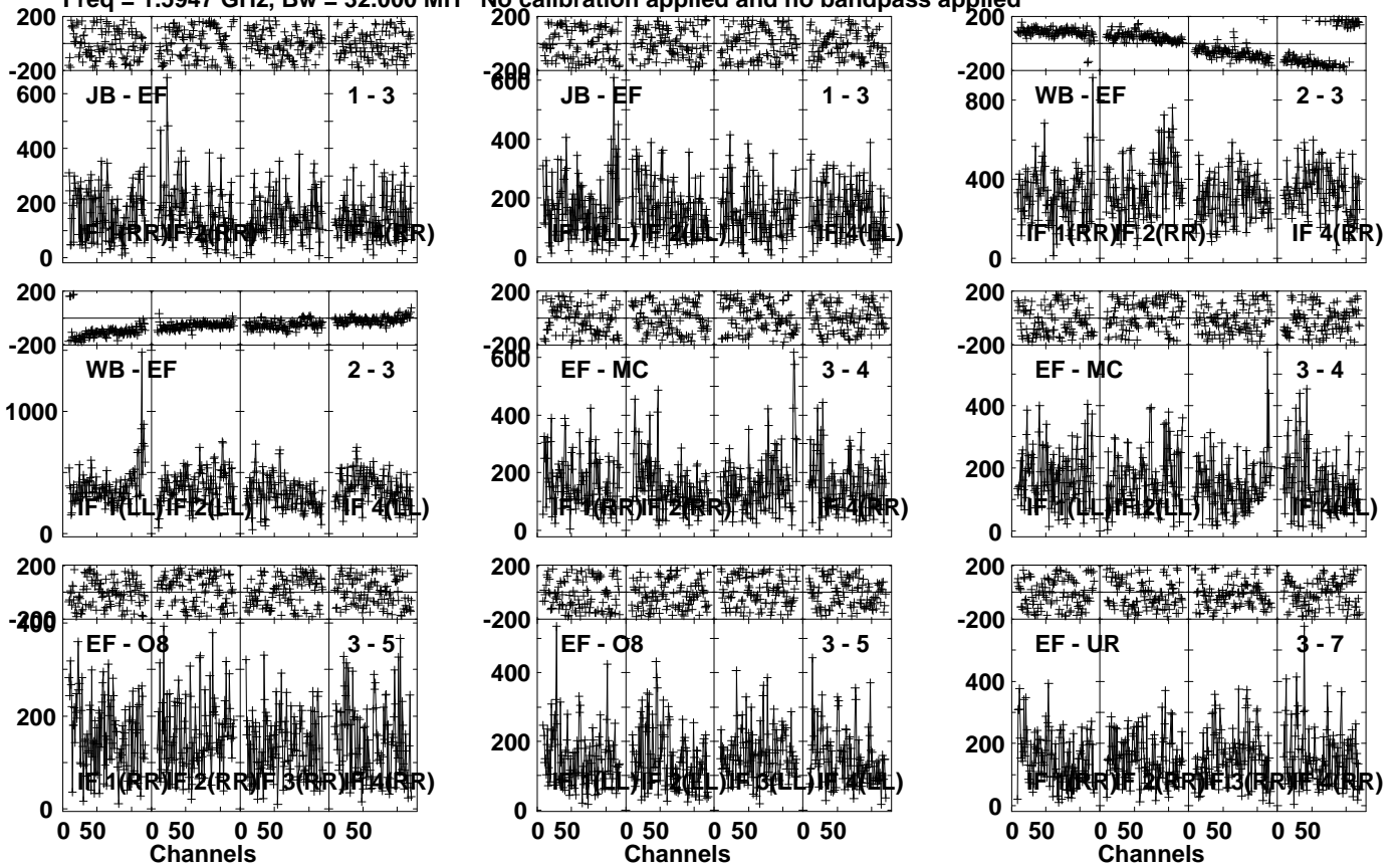
Lower frame: Micro Ampl Jy Top frame: Phas deg Vector averaged cross-power spectrum Several baselines displayed Timerange: 00/15:32:01 to 00/15:34:29
