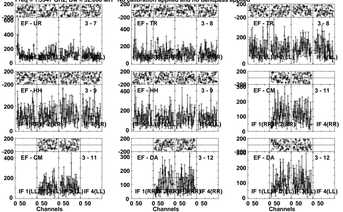
Lower frame: Micro Ampl Jy Top frame: Phas deg Vector averaged cross-power spectrum Several baselines displayed Timerange: 00/14:50:01 to 00/14:53:29
