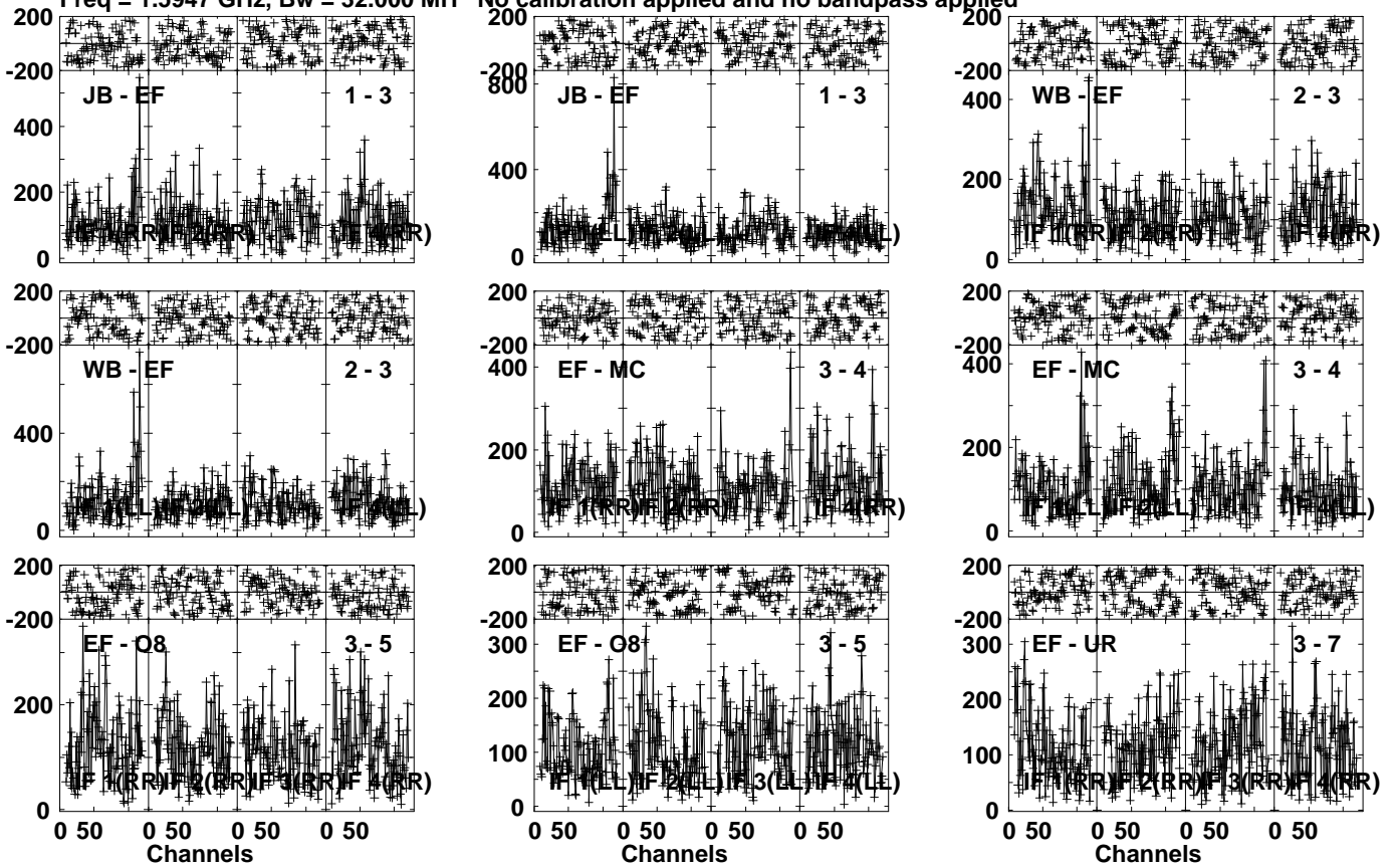
Lower frame: Micro Ampl Jy Top frame: Phas deg Vector averaged cross-power spectrum Several baselines displayed Timerange: 00/16:26:31 to 00/16:29:59
