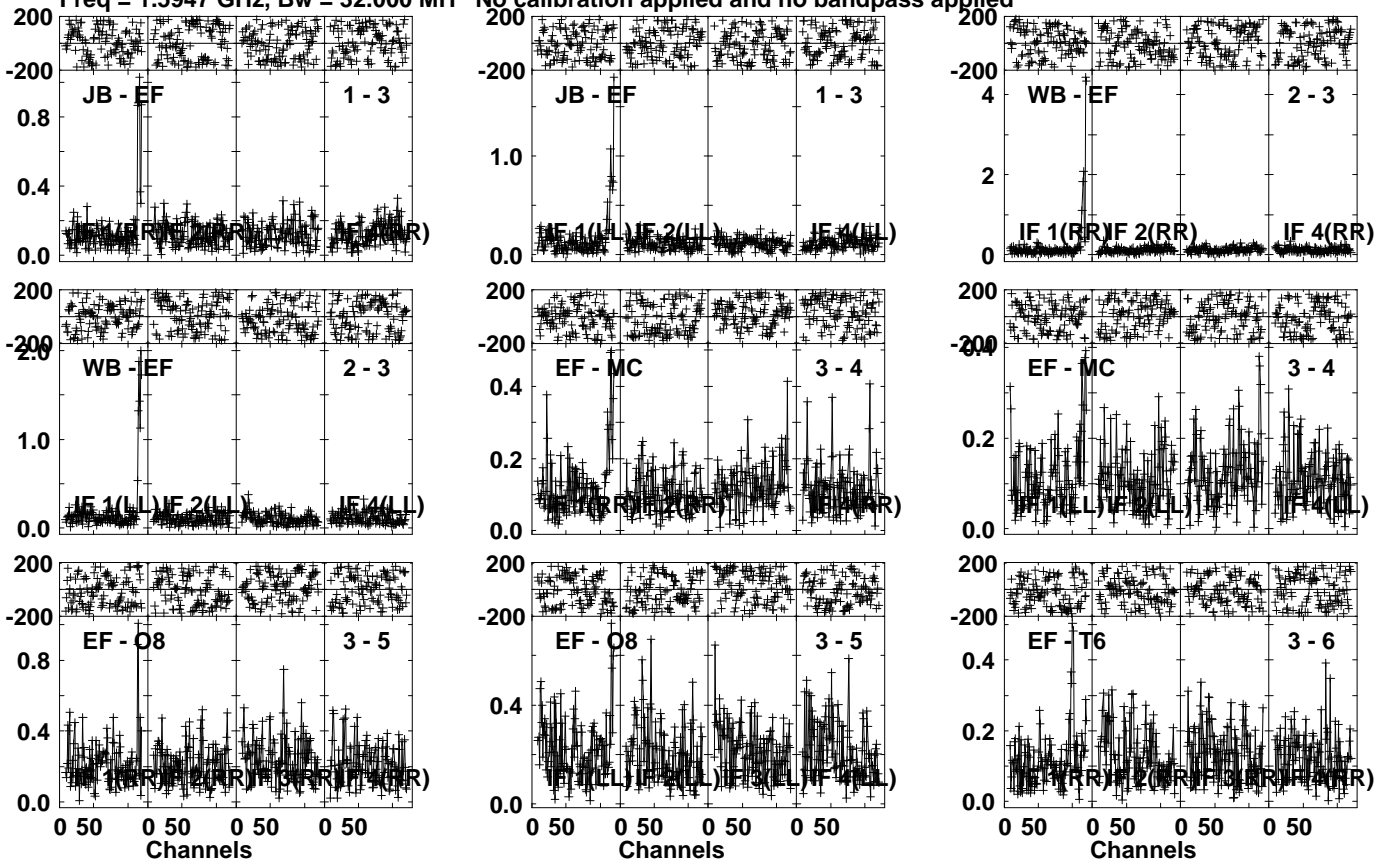
Lower frame: Milli Ampl Jy Top frame: Phas deg Vector averaged cross-power spectrum Several baselines displayed Timerange: 00/12:27:31 to 00/12:30:59
