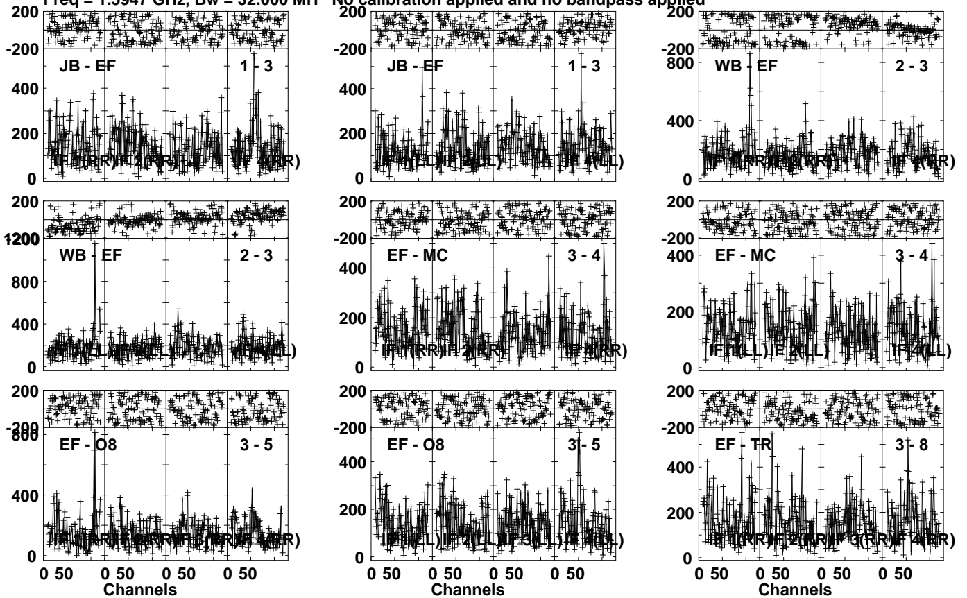
Lower frame: Micro Ampl Jy Top frame: Phas deg Vector averaged cross-power spectrum Several baselines displayed Timerange: 00/19:03:31 to 00/19:05:29
