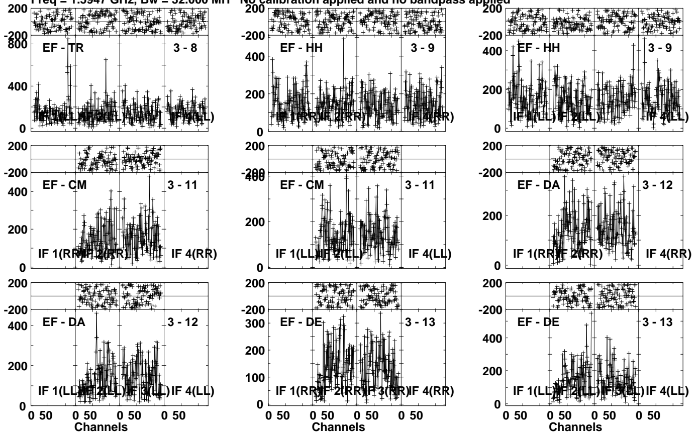
Lower frame: Micro Ampl Jy Top frame: Phas deg Vector averaged cross-power spectrum Several baselines displayed Timerange: 00/18:26:31 to 00/18:28:29
