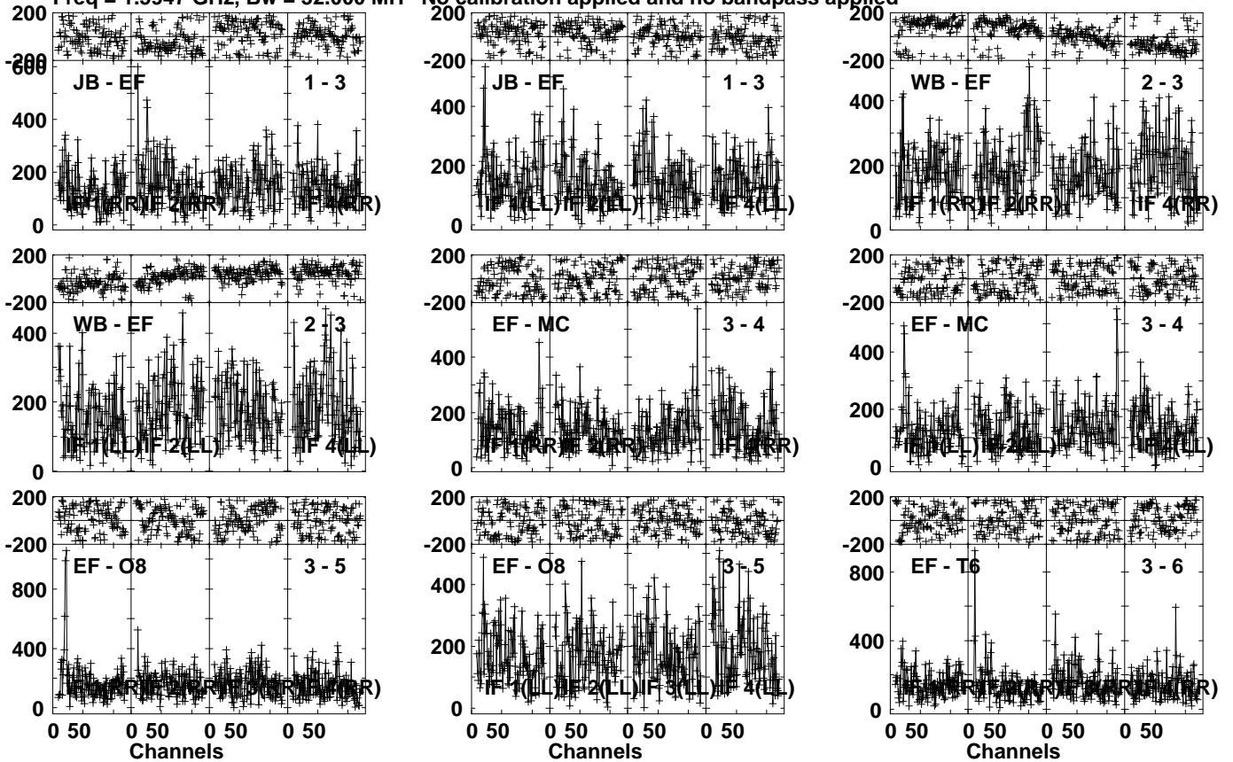
Lower frame: Micro Ampl Jy Top frame: Phas deg Vector averaged cross-power spectrum Several baselines displayed Timerange: 00/14:33:31 to 00/14:35:29
