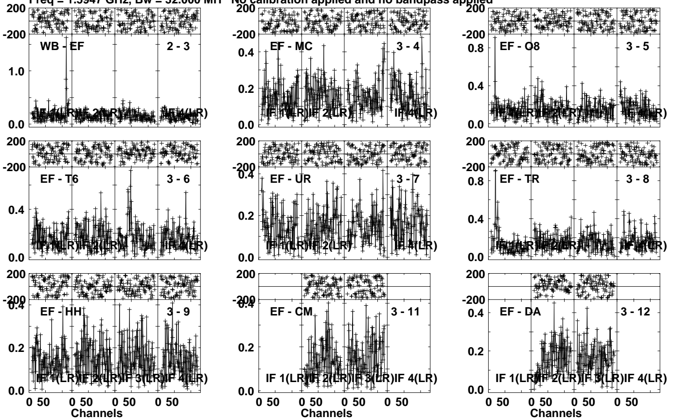
Lower frame: Milli Ampl Jy Top frame: Phas deg Vector averaged cross-power spectrum Several baselines displayed Timerange: 00/13:14:31 to 00/13:16:29
