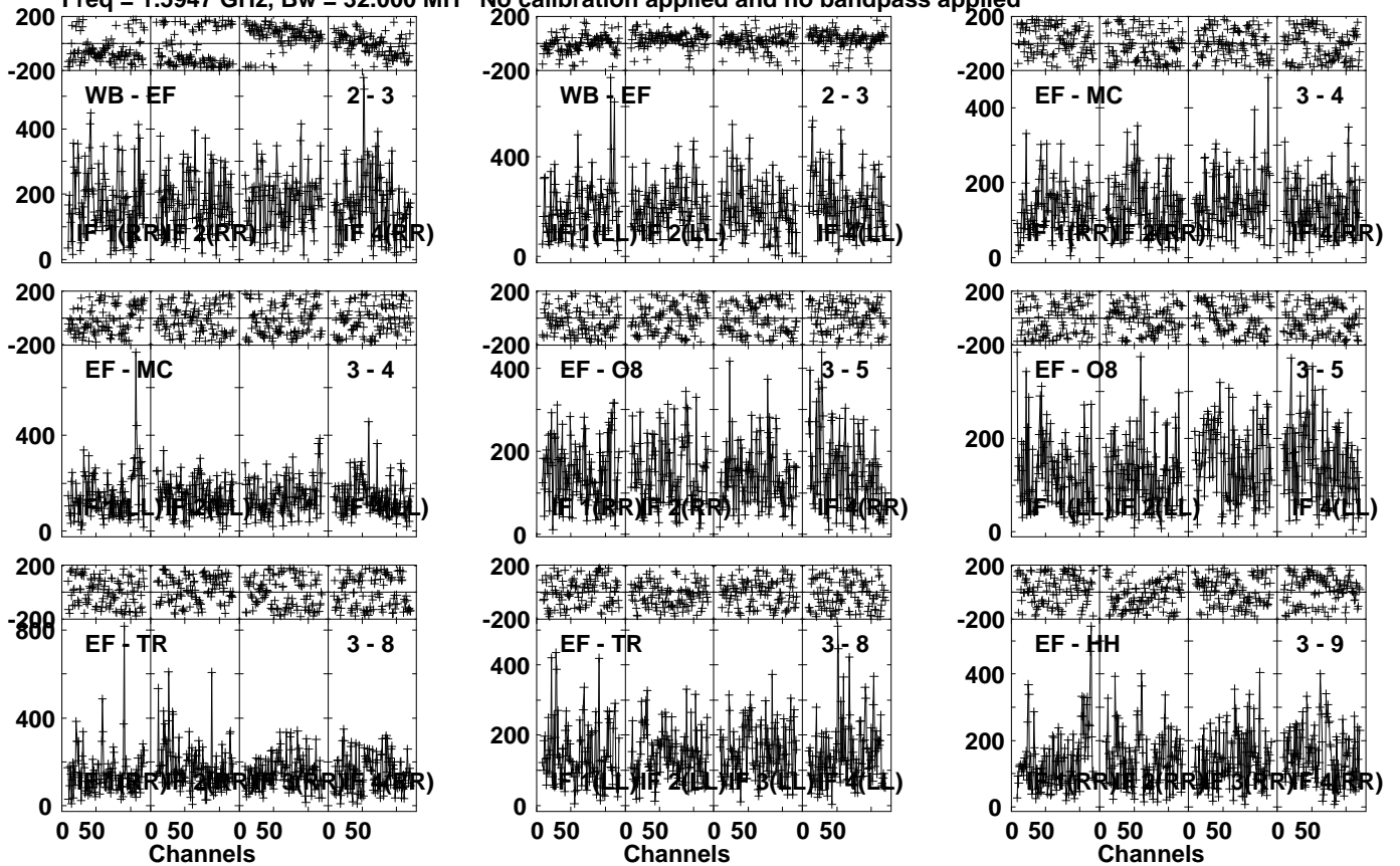
Lower frame: Micro Ampl Jy Top frame: Phas deg Vector averaged cross-power spectrum Several baselines displayed Timerange: 00/18:32:31 to 00/18:34:29
