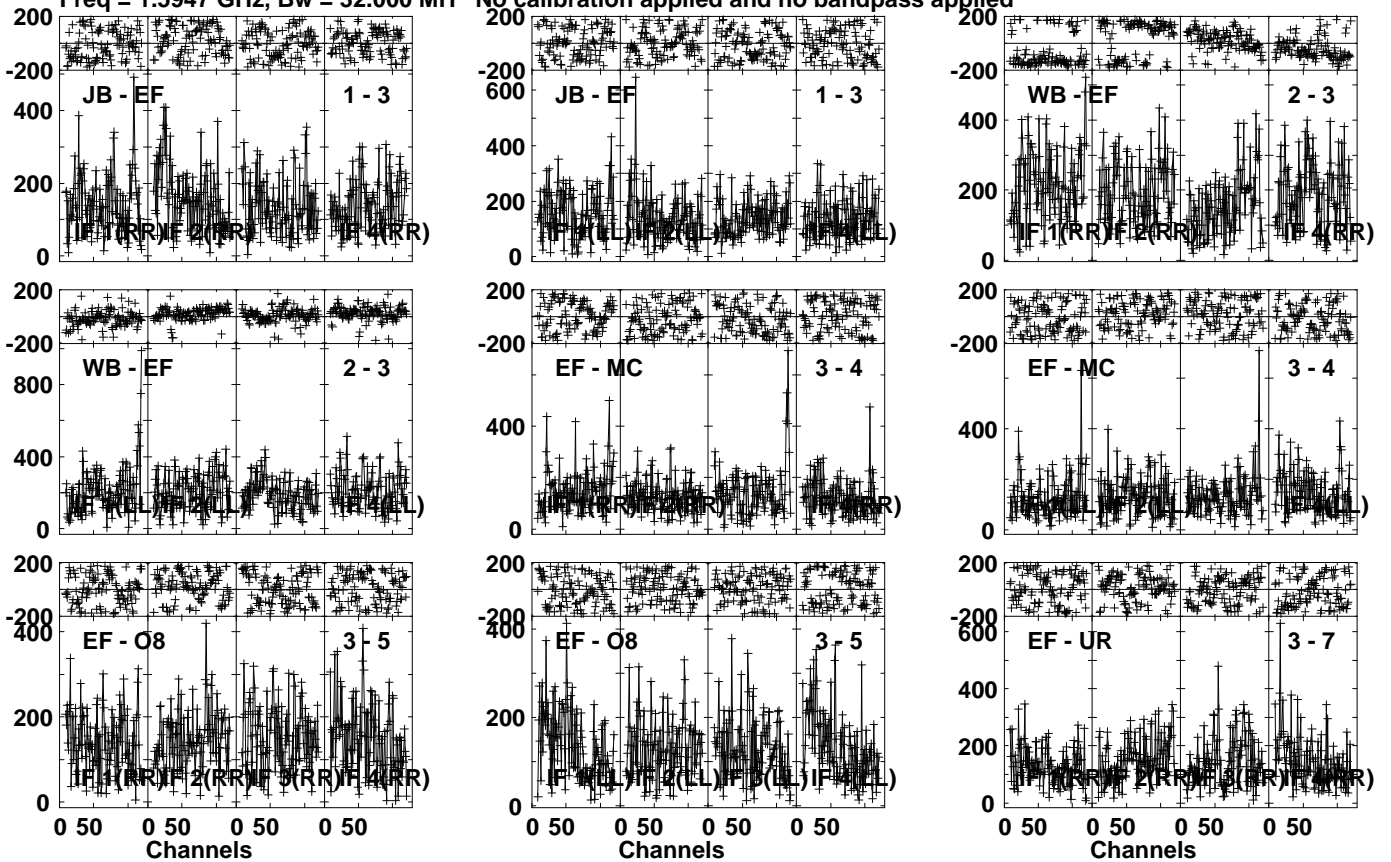
Lower frame: Micro Ampl Jy Top frame: Phas deg Vector averaged cross-power spectrum Several baselines displayed Timerange: 00/17:01:31 to 00/17:03:29
