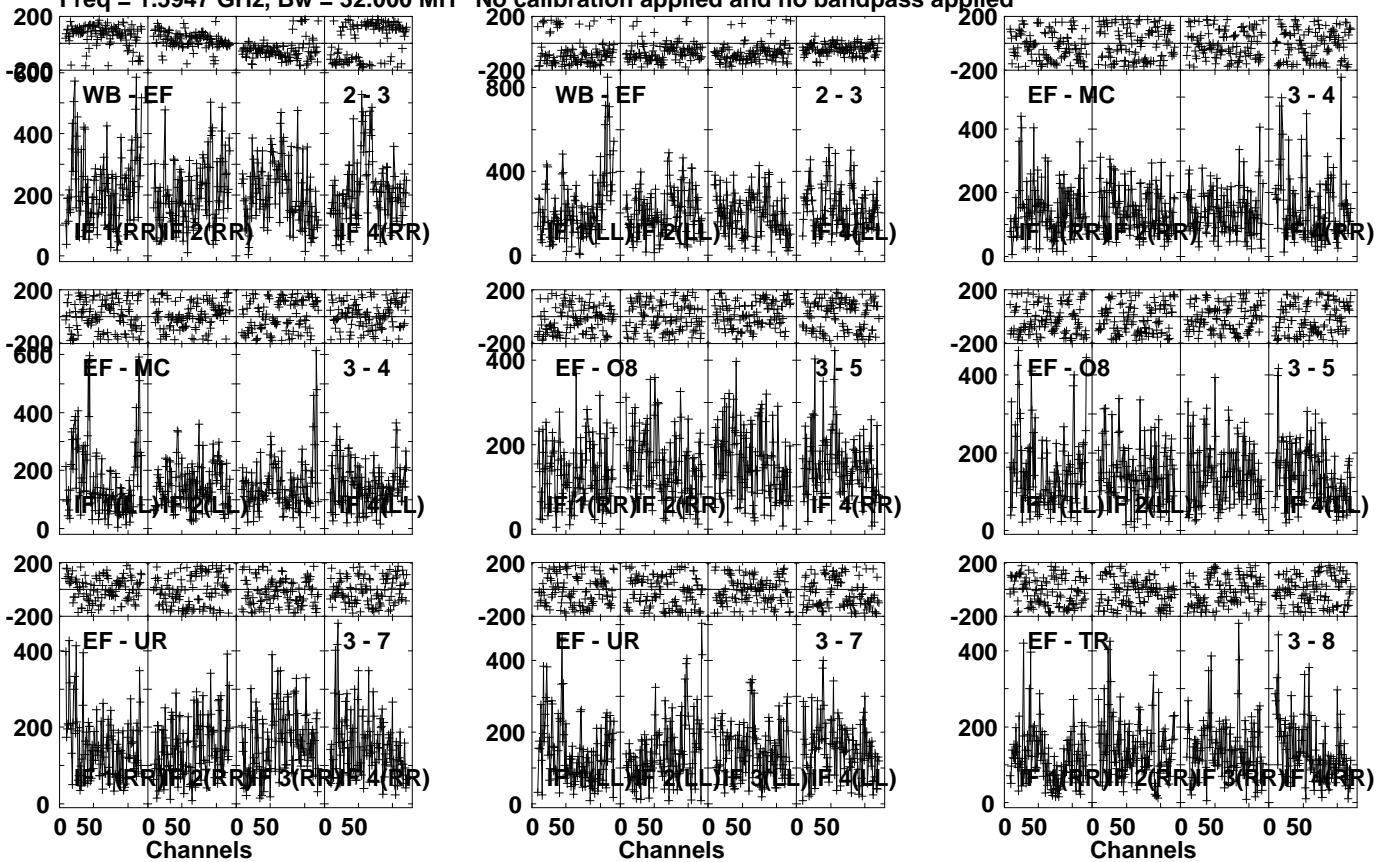
Lower frame: Micro Ampl Jy Top frame: Phas deg Vector averaged cross-power spectrum Several baselines displayed Timerange: 00/15:54:31 to 00/15:56:29
