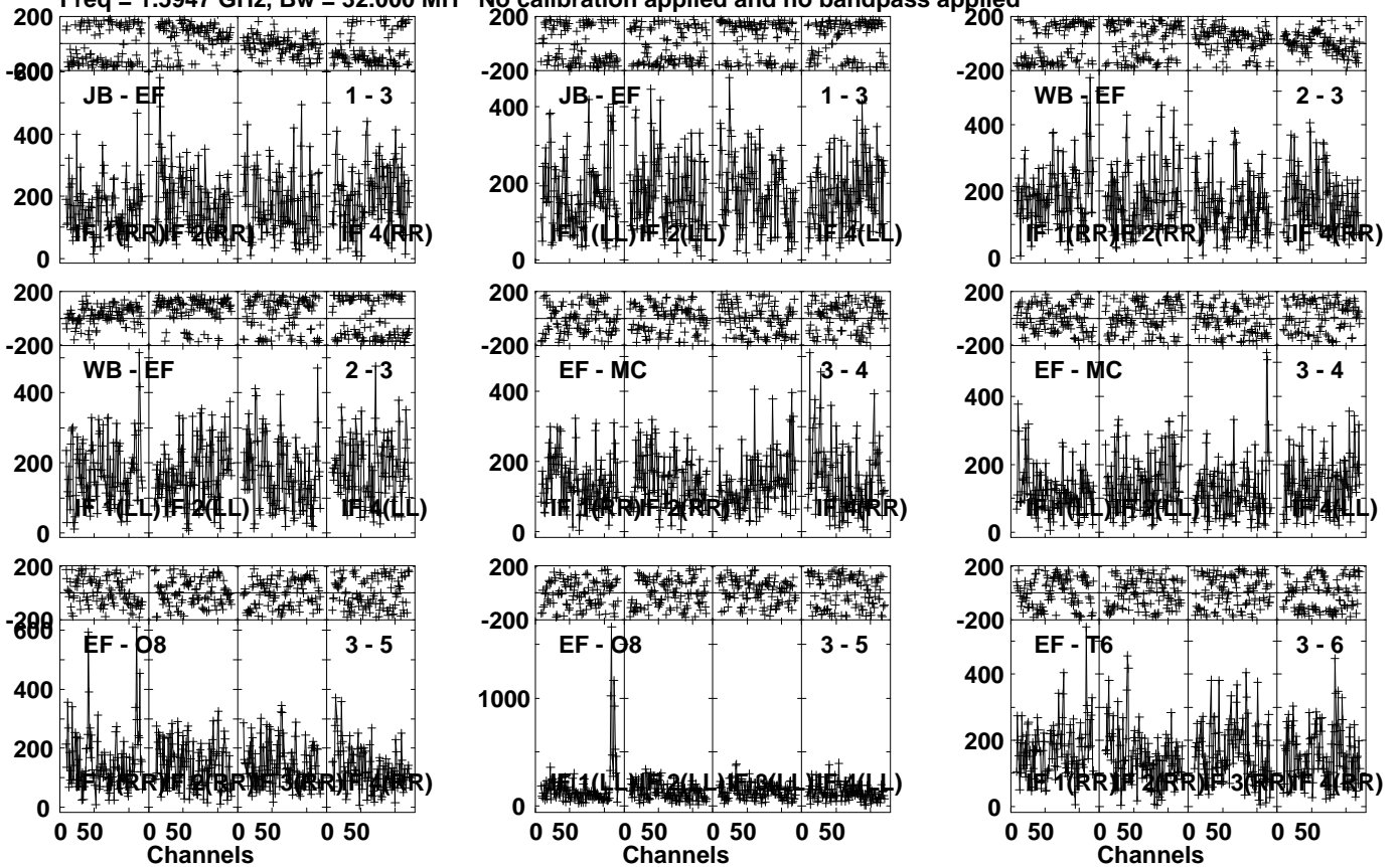
Lower frame: Micro Ampl Jy Top frame: Phas deg Vector averaged cross-power spectrum Several baselines displayed Timerange: 00/13:32:31 to 00/13:34:29
