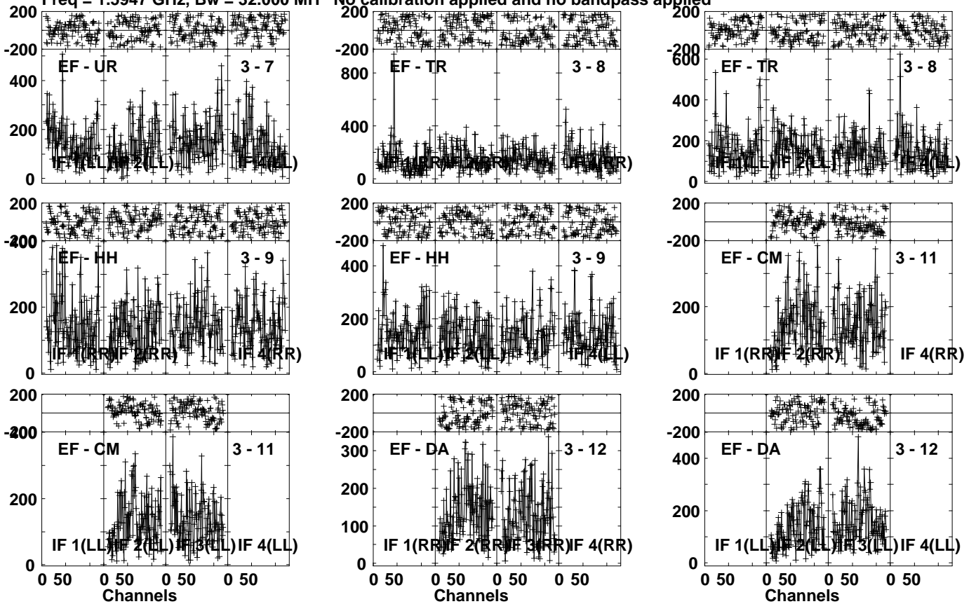
Lower frame: Micro Ampl Jy Top frame: Phas deg Vector averaged cross-power spectrum Several baselines displayed Timerange: 00/14:27:31 to 00/14:29:29
