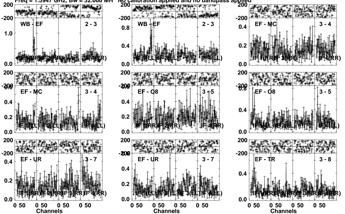
Lower frame: Milli Ampl Jy Top frame: Phas deg Vector averaged cross-power spectrum Several baselines displayed Timerange: 00/16:30:31 to 00/16:32:29
