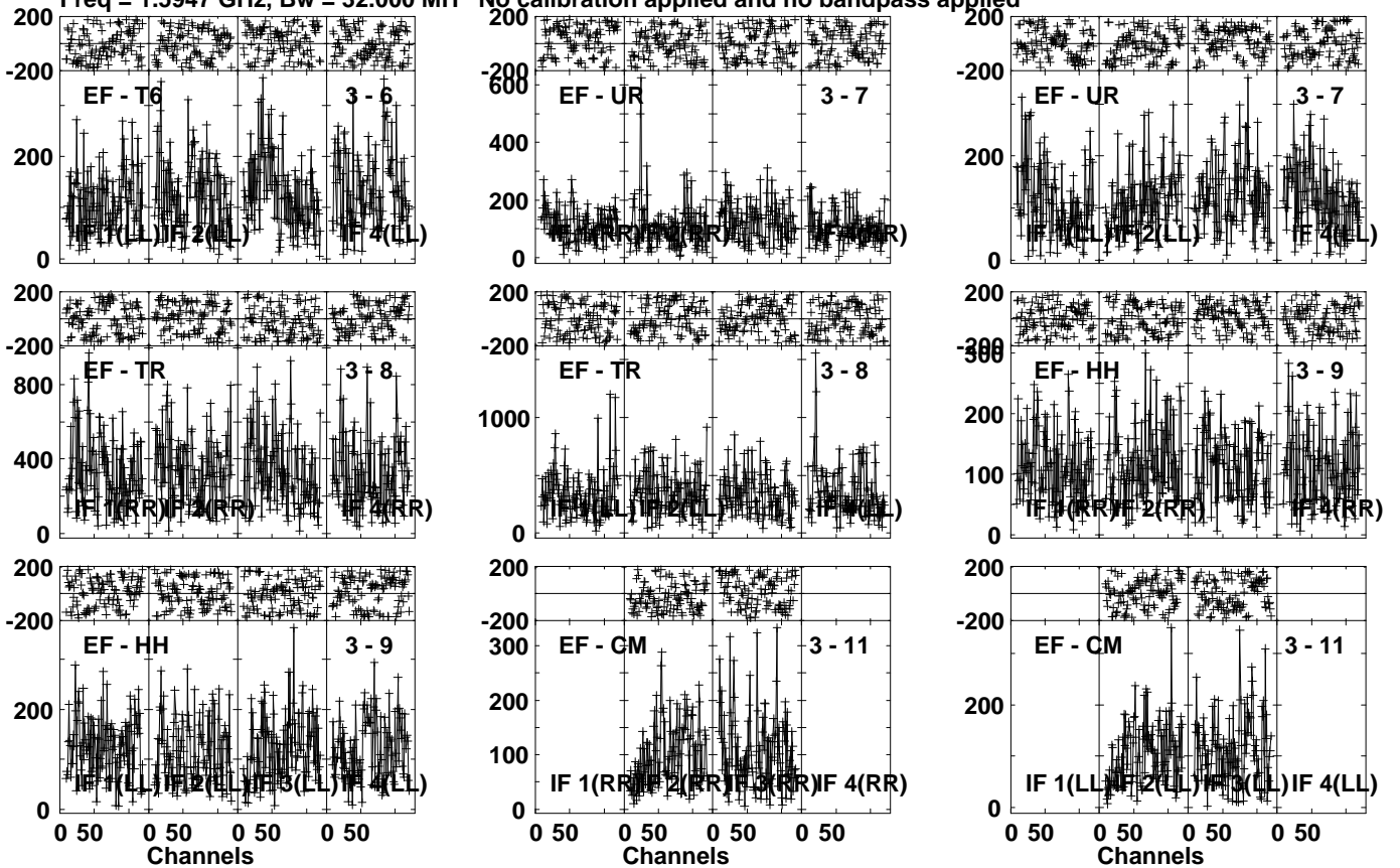
Lower frame: Micro Ampl Jy Top frame: Phas deg Vector averaged cross-power spectrum Several baselines displayed Timerange: 00/13:47:31 to 00/13:50:59
