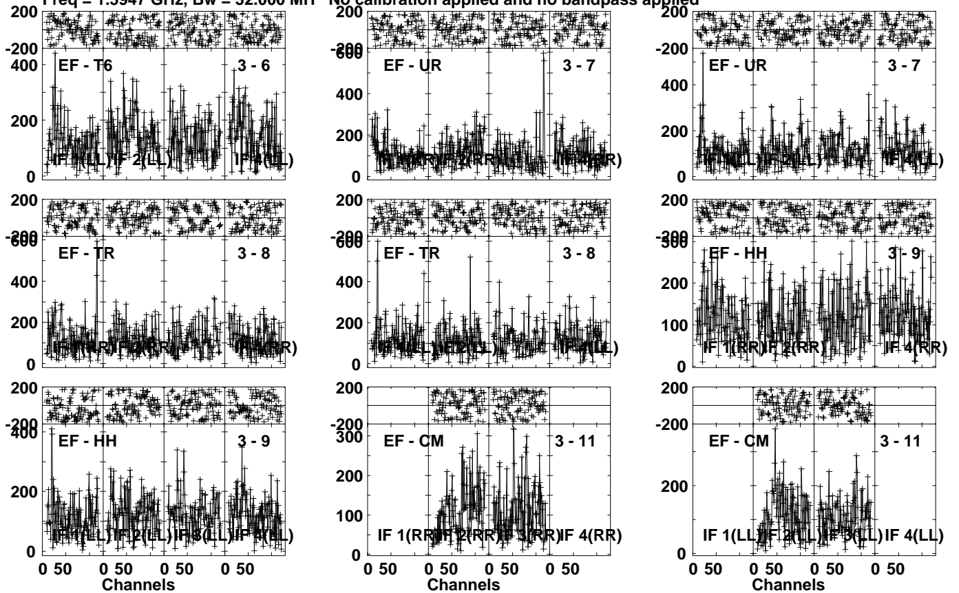
Lower frame: Micro Ampl Jy Top frame: Phas deg Vector averaged cross-power spectrum Several baselines displayed Timerange: 00/12:27:31 to 00/12:30:59
