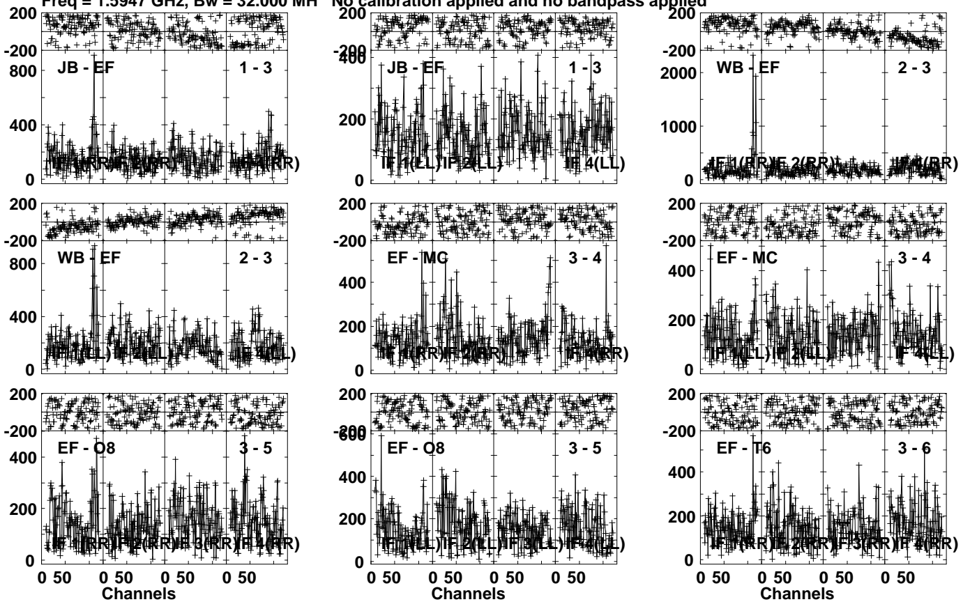
Lower frame: Micro Ampl Jy Top frame: Phas deg Vector averaged cross-power spectrum Several baselines displayed Timerange: 00/14:09:31 to 00/14:11:29
