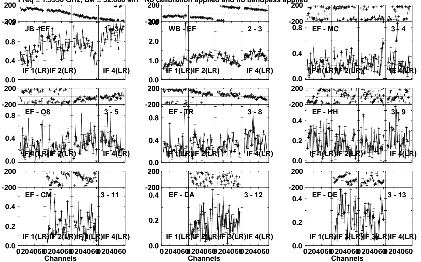
Lower frame: Milli Ampl Jy Top frame: Phas deg Vector averaged cross-power spectrum Several baselines displayed Timerange: 00:18:27:11 to 00:18:28:09
