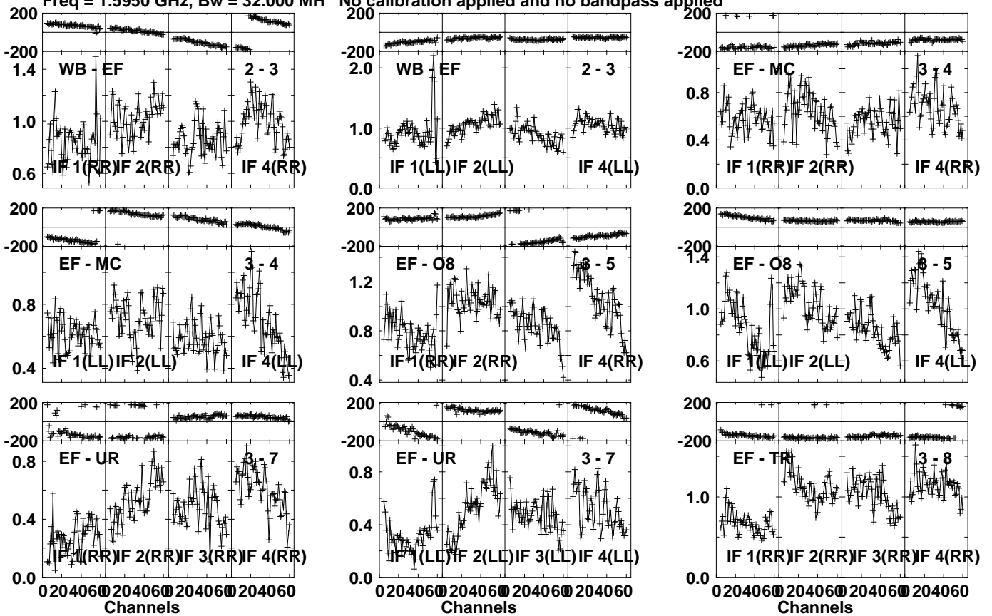
Lower frame: Milli Ampl Jy Top frame: Phas deg Vector averaged cross-power spectrum Several baselines displayed Timerange: 00/13:55:01 to 00/13:56:29
