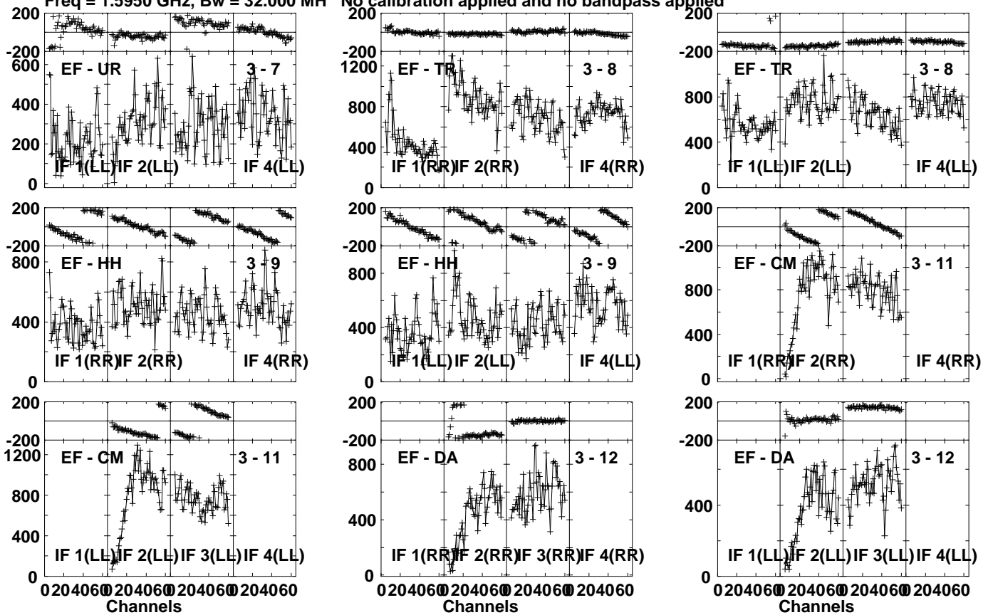
Lower frame: Micro Ampl Jy Top frame: Phas deg Vector averaged cross-power spectrum Several baselines displayed Timerange: 00/14:38:11 to 00/14:39:39
