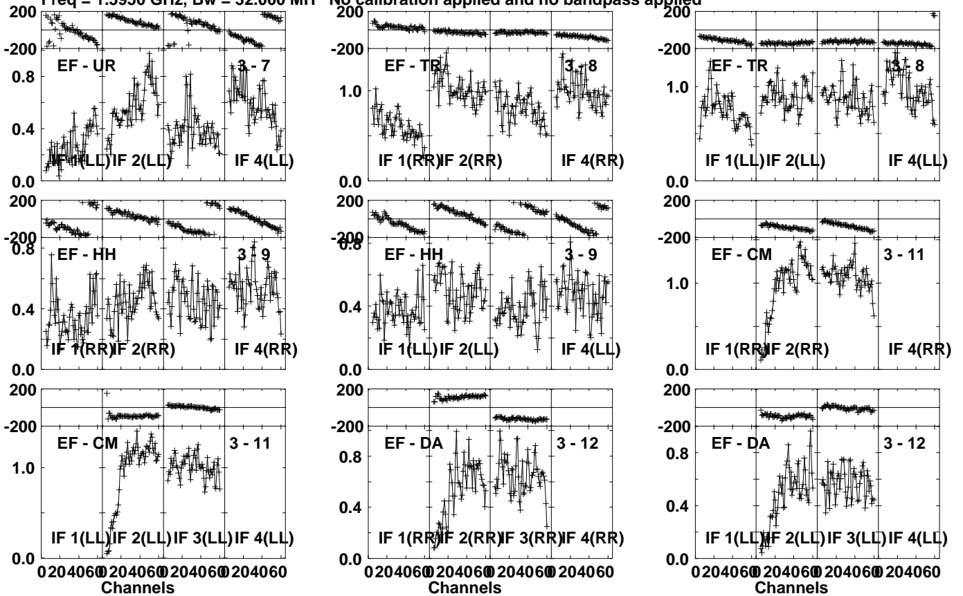
Lower frame: Milli Ampl Jy Top frame: Phas deg Vector averaged cross-power spectrum Several baselines displayed Timerange: 00/10:44:31 to 00/10:45:59
