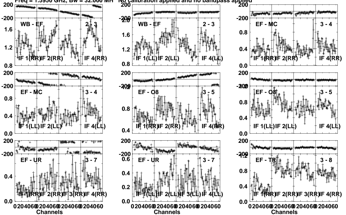
Lower frame: Milli Ampl Jy Top frame: Phas deg Vector averaged cross-power spectrum Several baselines displayed Timerange: 00:14:53:31 to 00:14:54:59
