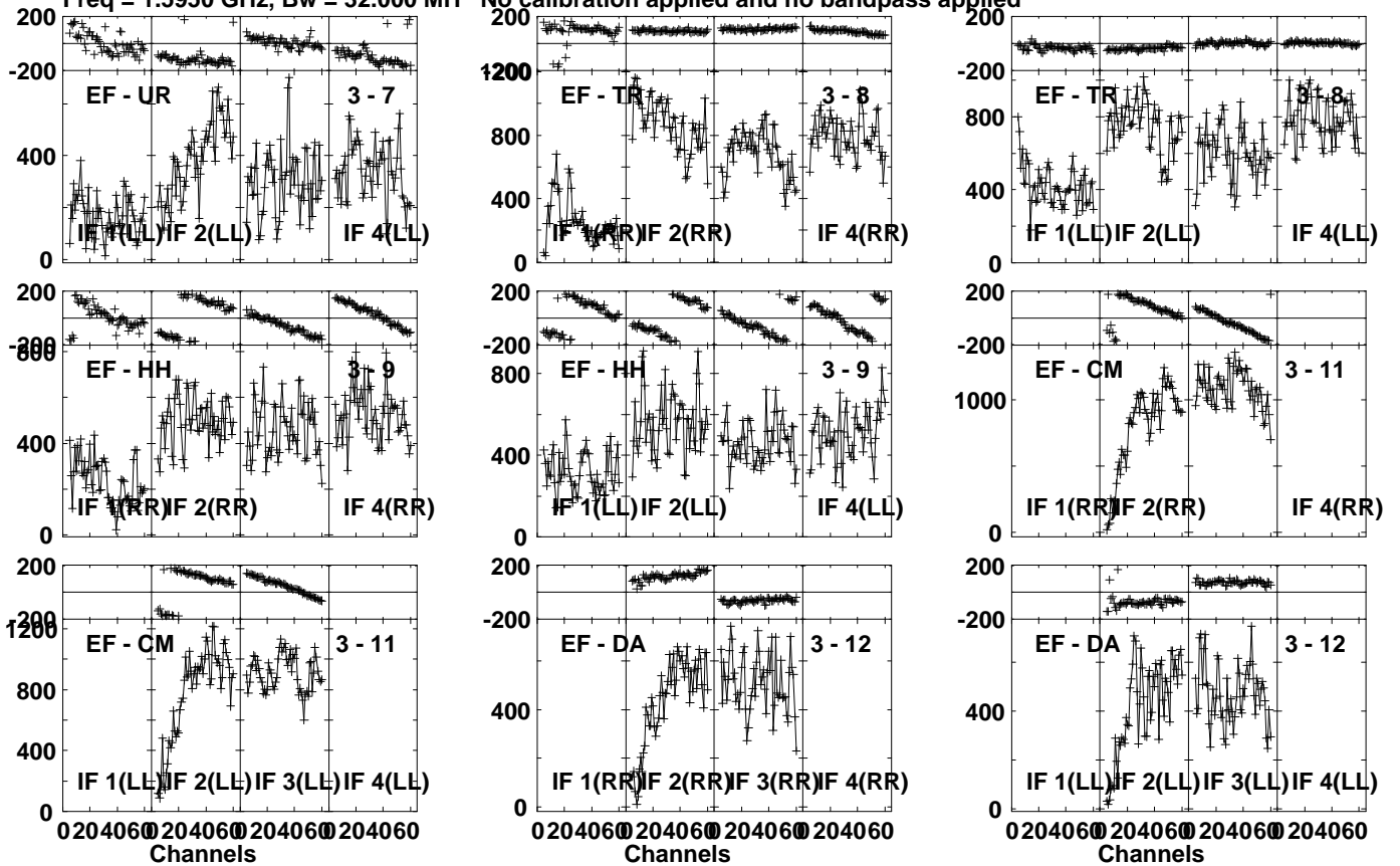
Lower frame: Micro Ampl Jy Top frame: Phas deg Vector averaged cross-power spectrum Several baselines displayed Timerange: 00/14:15:51 to 00/14:17:19
