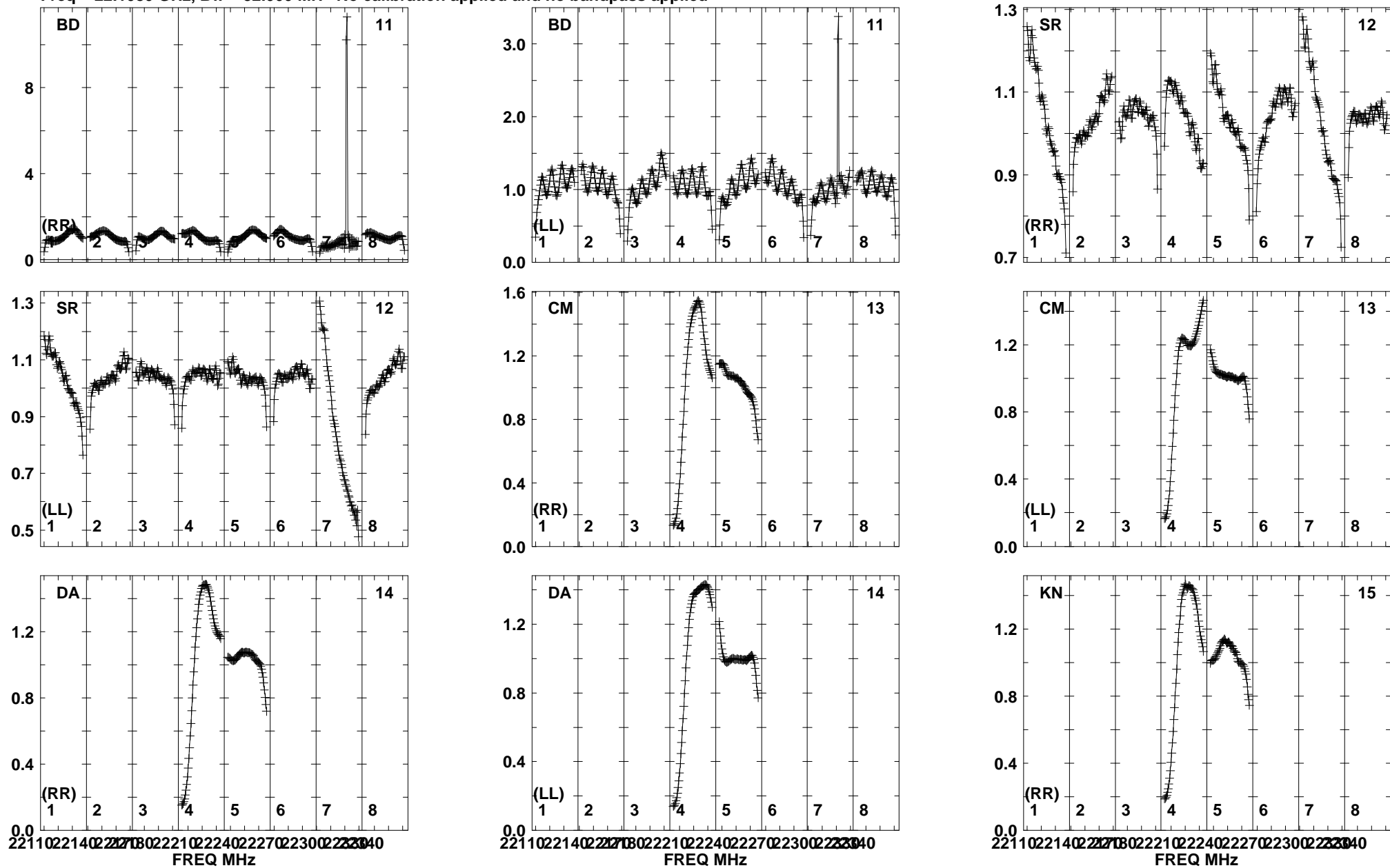
Lower frame: Real Jy Total-power spectrum Antenna: BD (11) Timerange: 00/22:05:11 to 00/22:06:29
