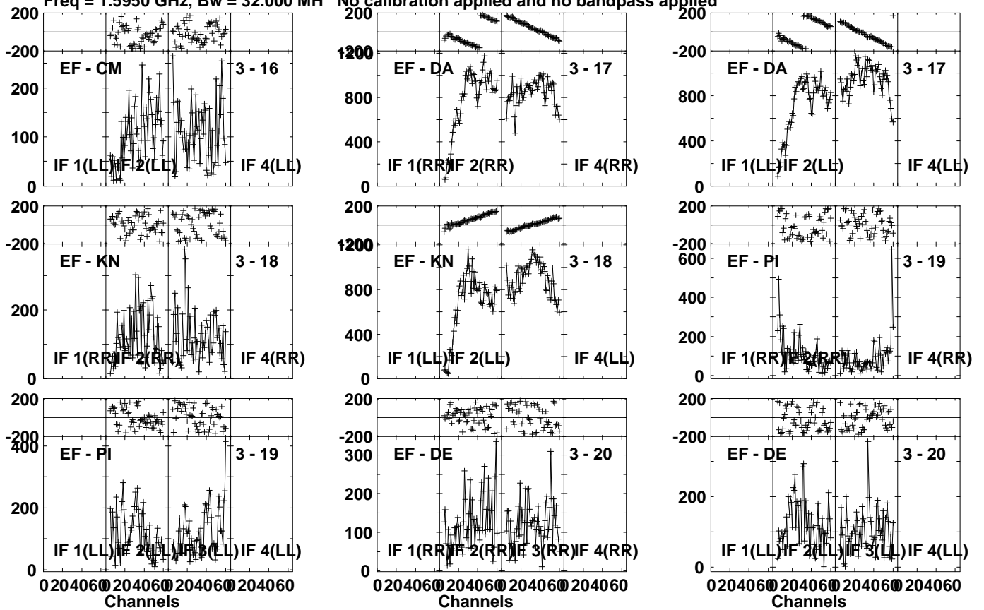
Lower frame: Micro Ampl Jy Top frame: Phas deg Vector averaged cross-power spectrum Several baselines displayed Timerange: 00/17:22:31 to 00/17:24:19
