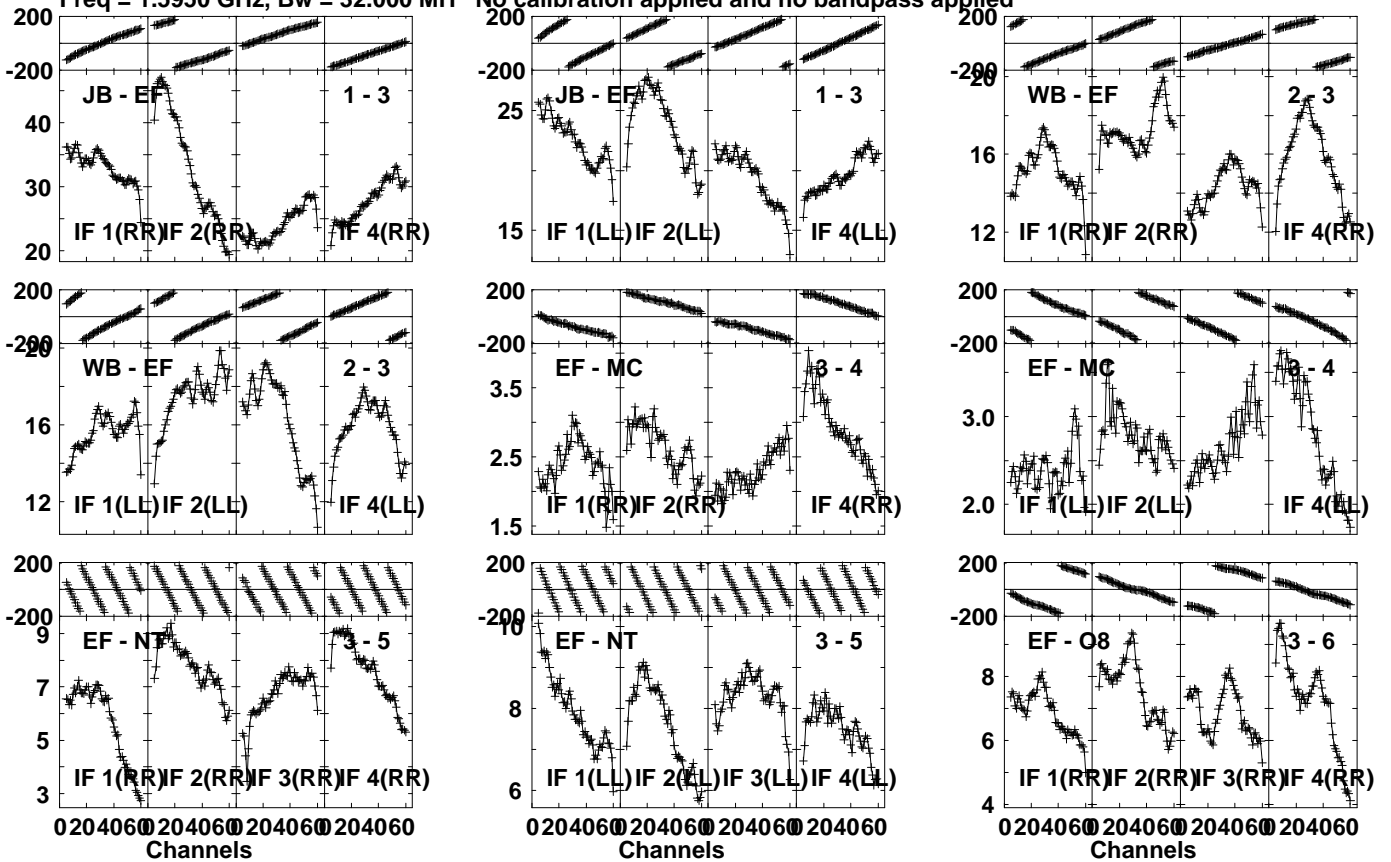
Lower frame: Milli Ampl Jy Top frame: Phas deg Vector averaged cross-power spectrum Several baselines displayed Timerange: 01/08:40:51 to 01/08:42:39
