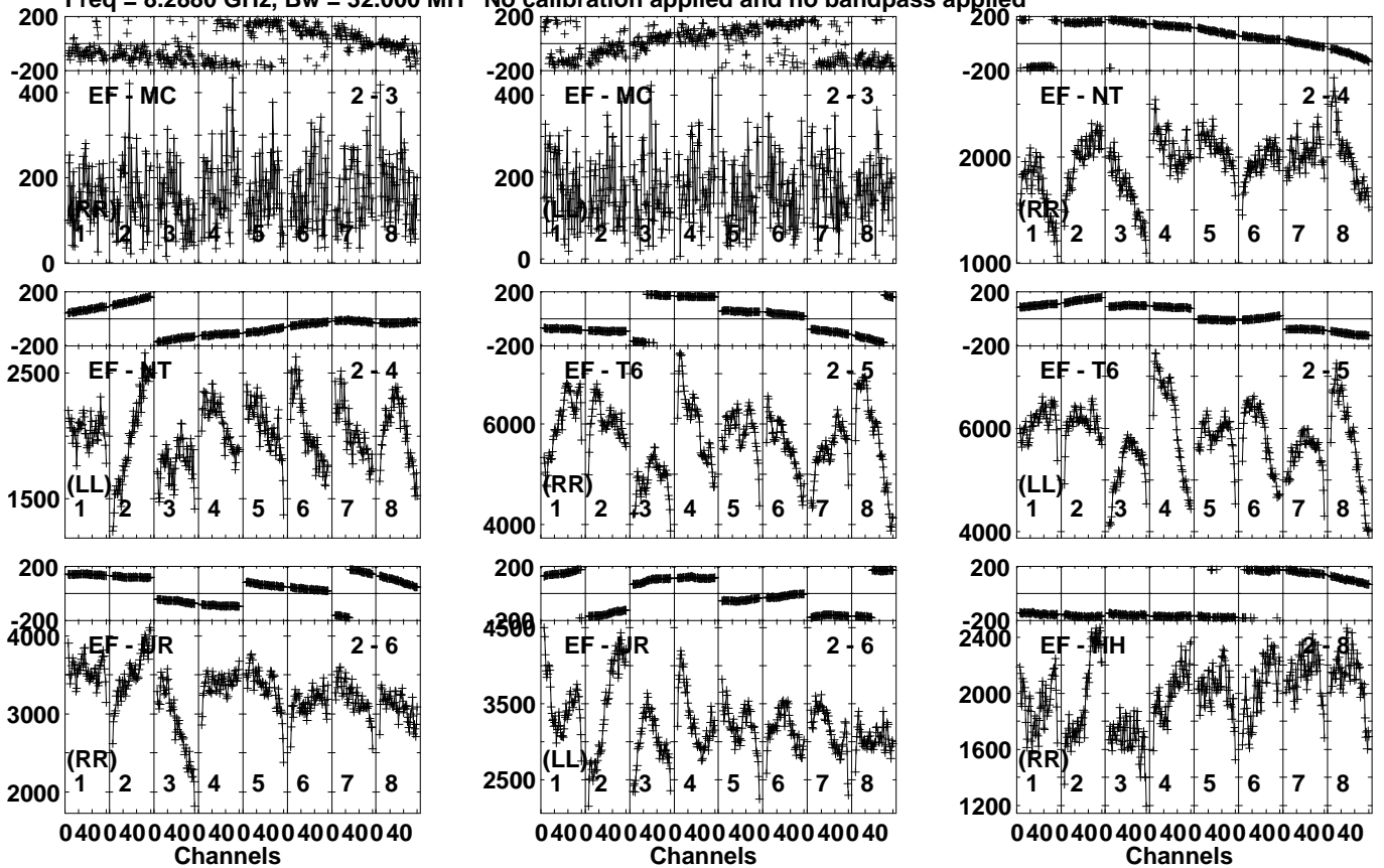
Lower frame: Micro Ampl Jy Top frame: Phas deg Vector averaged cross-power spectrum Several baselines displayed Timerange: 00/21:27:01 to 00/21:28:29
