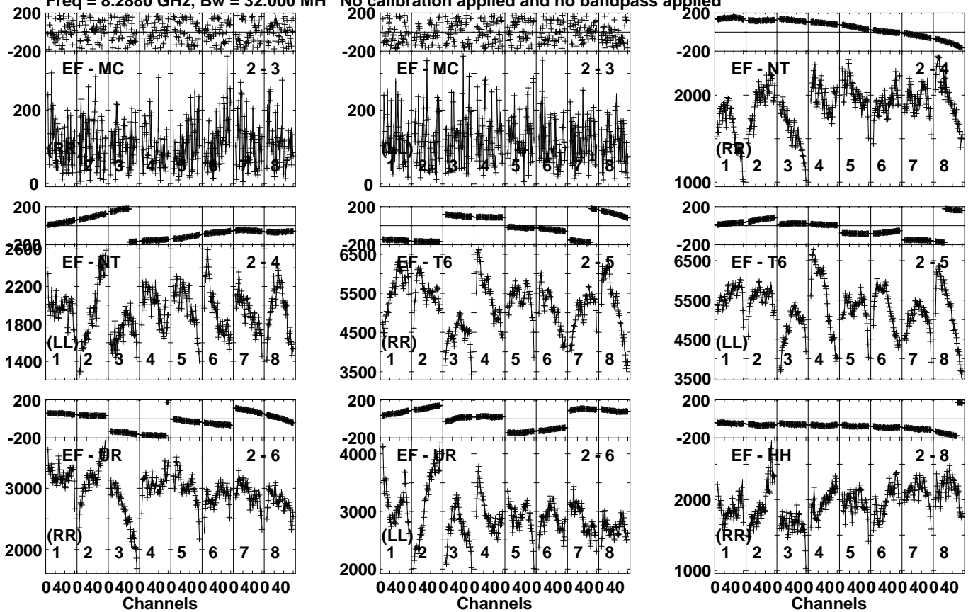
Lower frame: Micro Ampl Jy Top frame: Phas deg Vector averaged cross-power spectrum Several baselines displayed Timerange: 00/21:37:31 to 00/21:38:59
