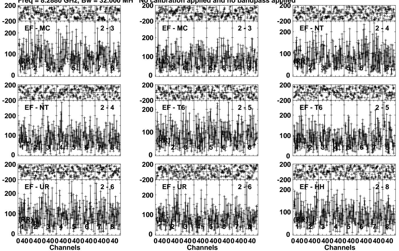
Lower frame: Micro Ampl Jy Top frame: Phas deg Vector averaged cross-power spectrum Several baselines displayed Timerange: 00/22:26:41 to 00/22:29:29
