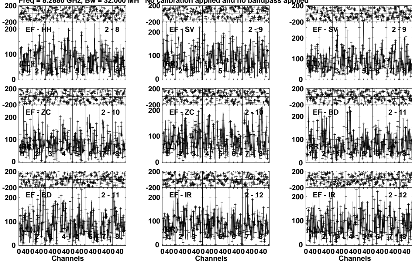
Lower frame: Micro Ampl Jy Top frame: Phas deg Vector averaged cross-power spectrum Several baselines displayed Timerange: 00/21:55:11 to 00/21:57:59
