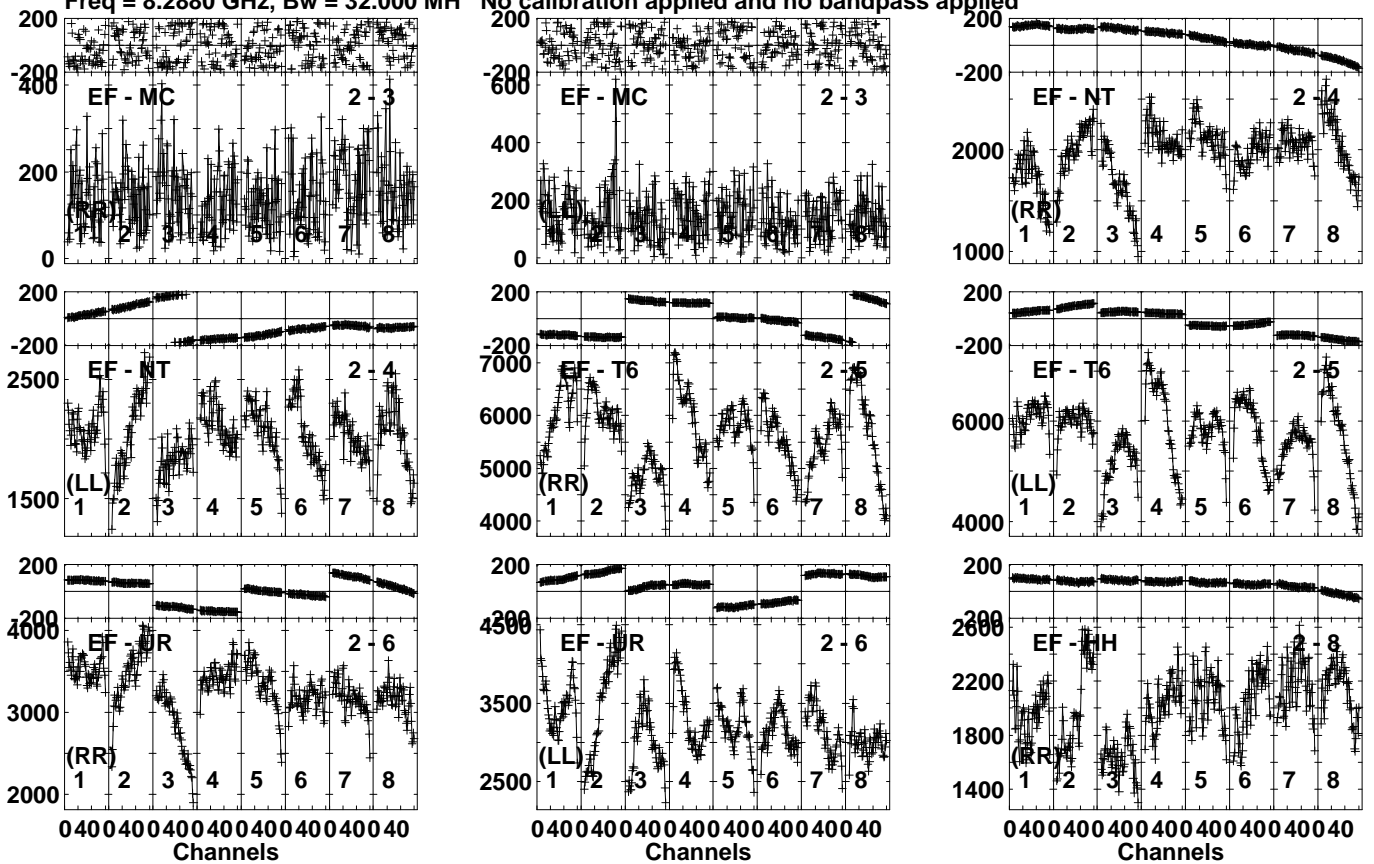
Lower frame: Micro Ampl Jy Top frame: Phas deg Vector averaged cross-power spectrum Several baselines displayed Timerange: 00/21:32:01 to 00/21:33:29
