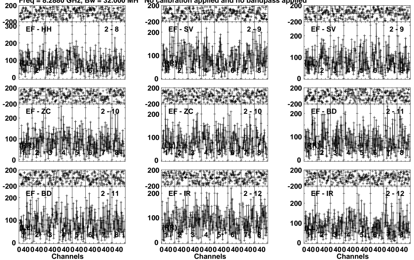
Lower frame: Micro Ampl Jy Top frame: Phas deg Vector averaged cross-power spectrum Several baselines displayed Timerange: 00/22:16:11 to 00/22:18:59
