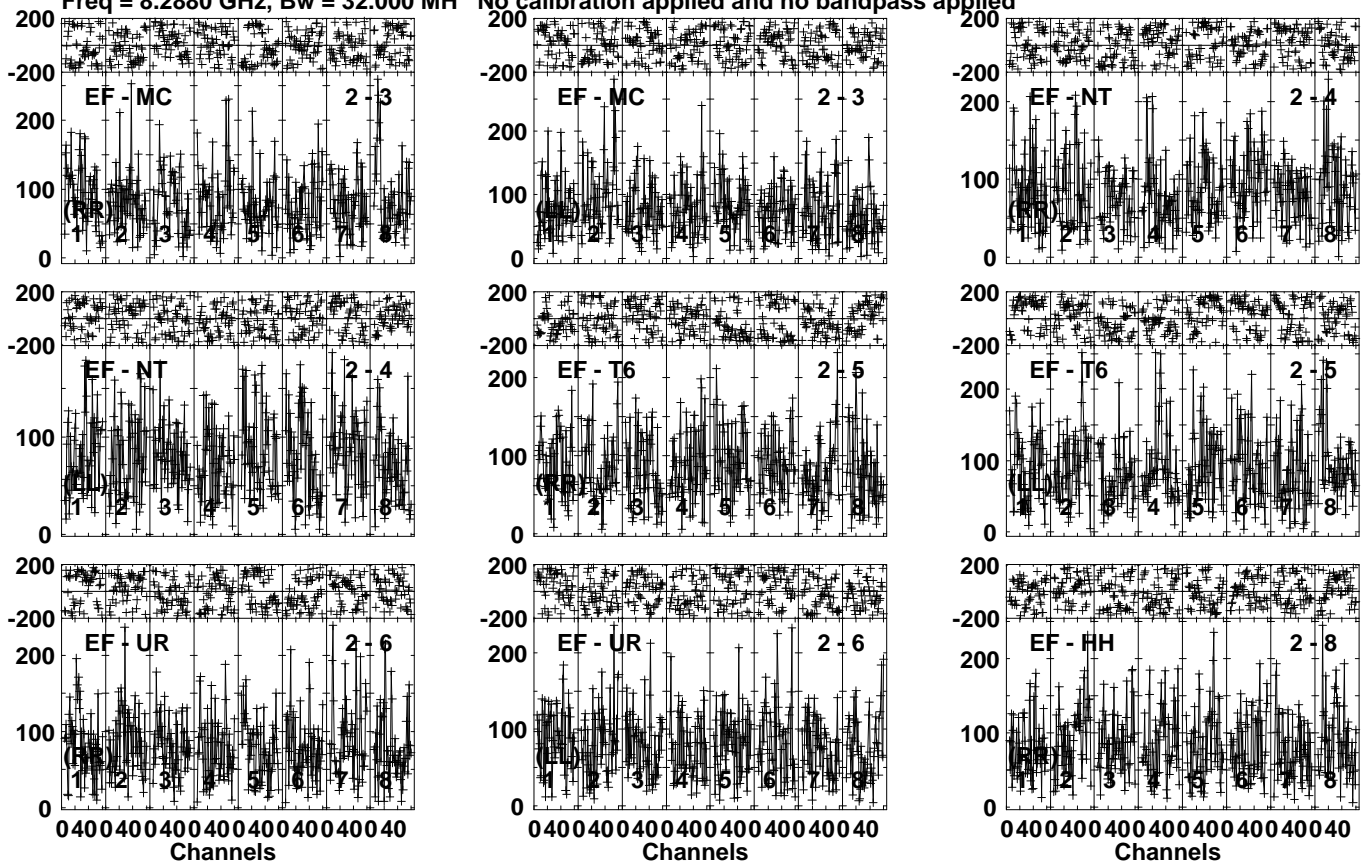
Lower frame: Micro Ampl Jy Top frame: Phas deg Vector averaged cross-power spectrum Several baselines displayed Timerange: 00/21:34:11 to 00/21:36:59
