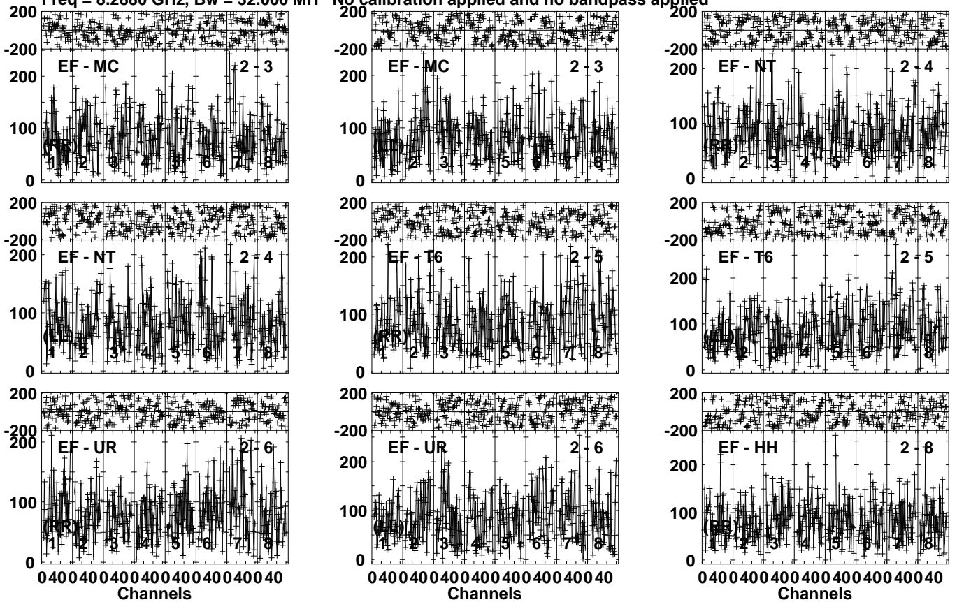
Lower frame: Micro Ampl Jy Top frame: Phas deg Vector averaged cross-power spectrum Several baselines displayed Timerange: 00/23:40:11 to 00/23:42:59
