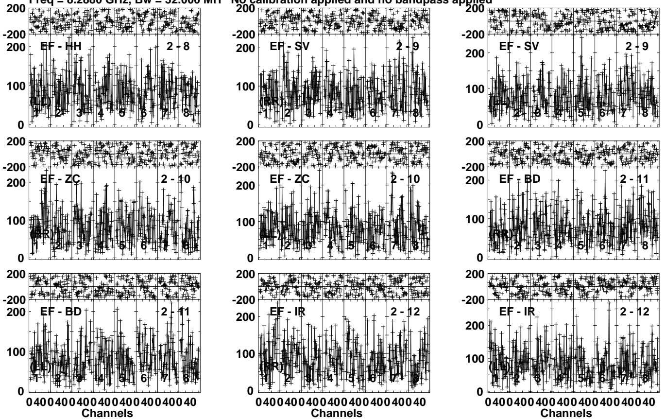
Lower frame: Micro Ampl Jy Top frame: Phas deg Vector averaged cross-power spectrum Several baselines displayed Timerange: 00/22:52:33 to 00/22:55:59
