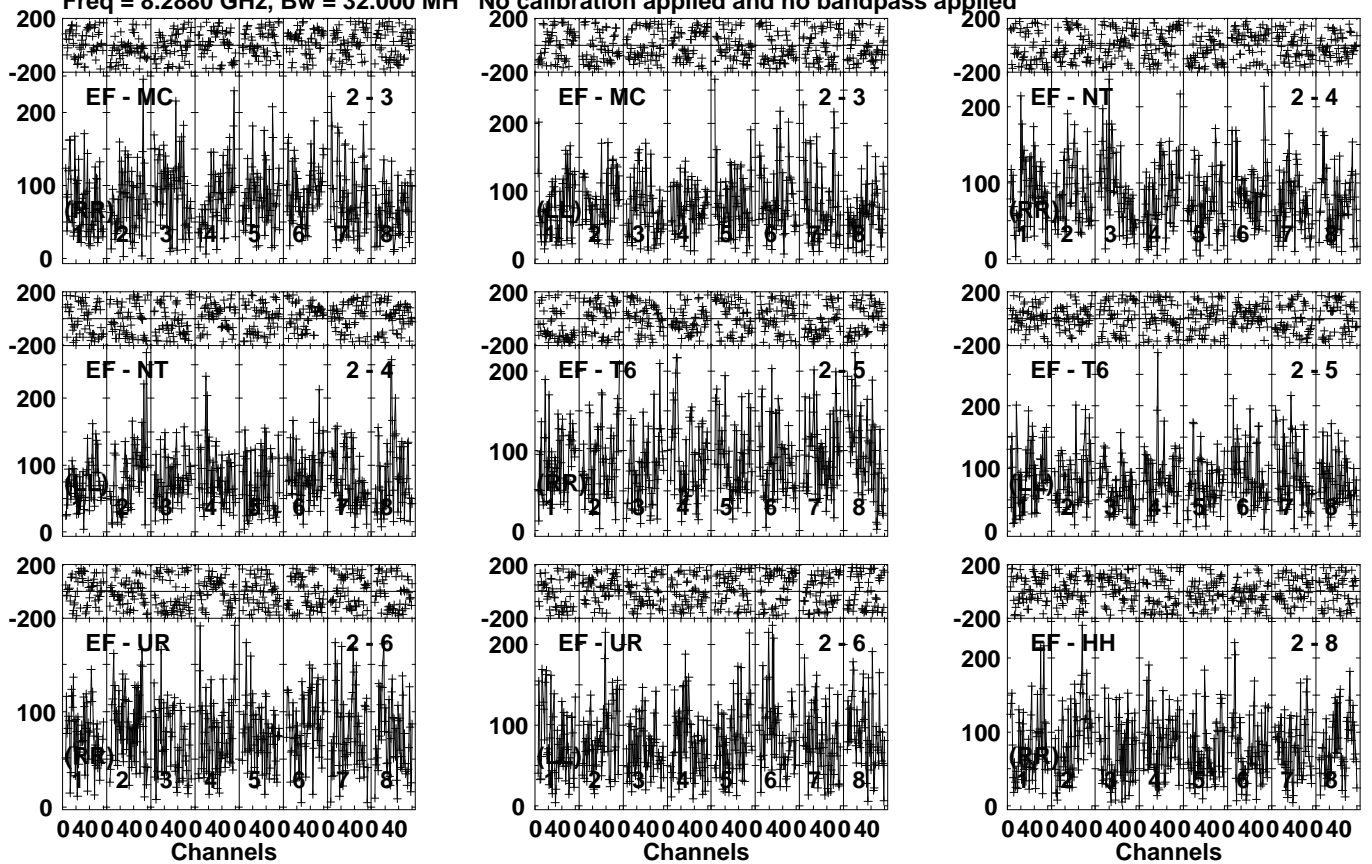
Lower frame: Micro Ampl Jy Top frame: Phas deg Vector averaged cross-power spectrum Several baselines displayed Timerange: 00/21:28:31 to 00/21:31:59
