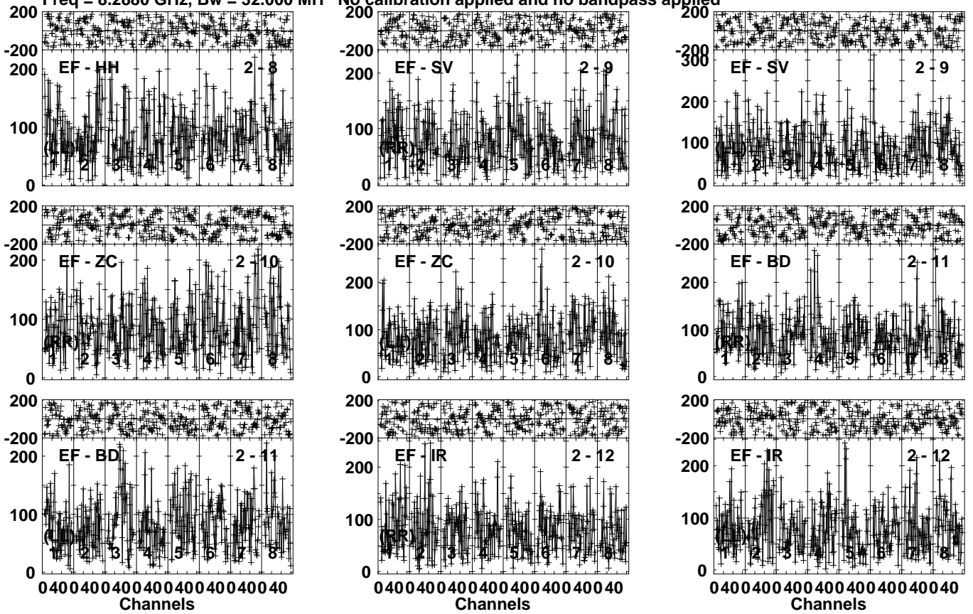
Lower frame: Micro Ampl Jy Top frame: Phas deg Vector averaged cross-power spectrum Several baselines displayed Timerange: 00/22:47:41 to 00/22:50:29
