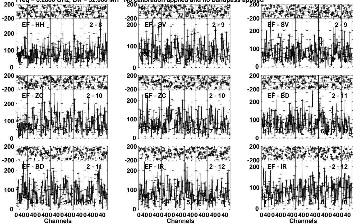
Lower frame: Micro Ampl Jy Top frame: Phas deg Vector averaged cross-power spectrum Several baselines displayed Timerange: 00/22:37:11 to 00/22:39:59
