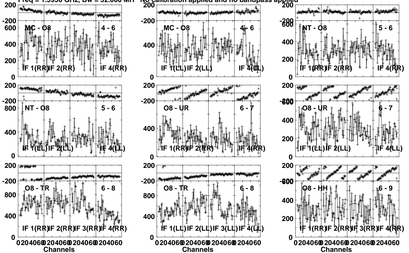
Lower frame: Micro Ampl Jy Top frame: Phas deg Vector averaged cross-power spectrum Several baselines displayed Timerange: 00/07:15:12 to 00/07:16:10
