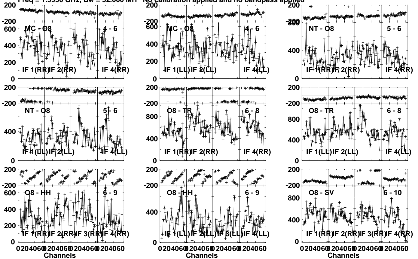
Lower frame: Micro Ampl Jy Top frame: Phas deg Vector averaged cross-power spectrum Several baselines displayed Timerange: 00/04:23:25 to 00/04:24:23
