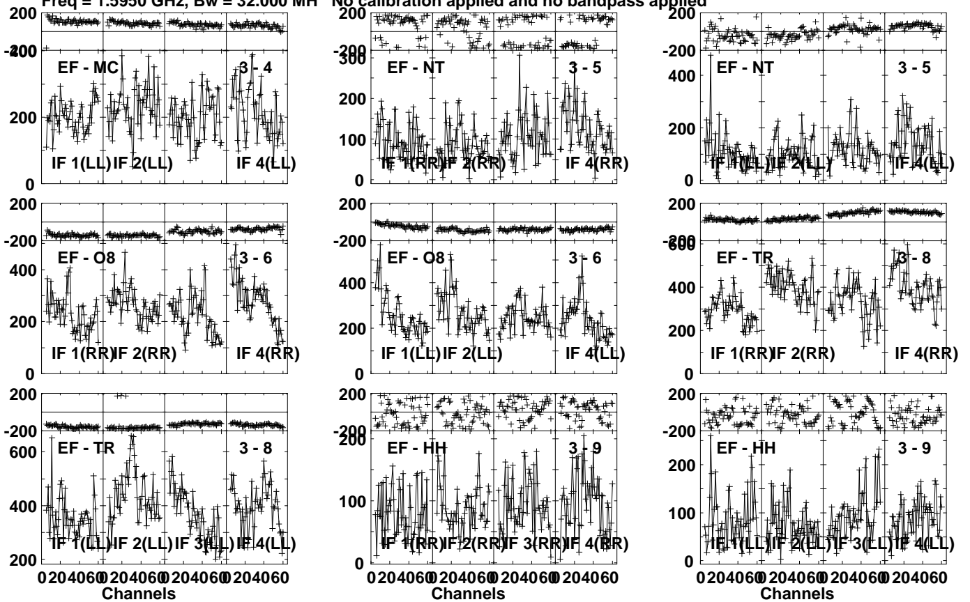
Lower frame: Micro Ampl Jy Top frame: Phas deg Vector averaged cross-power spectrum Several baselines displayed Timerange: 00/04:45:15 to 00/04:48:43
