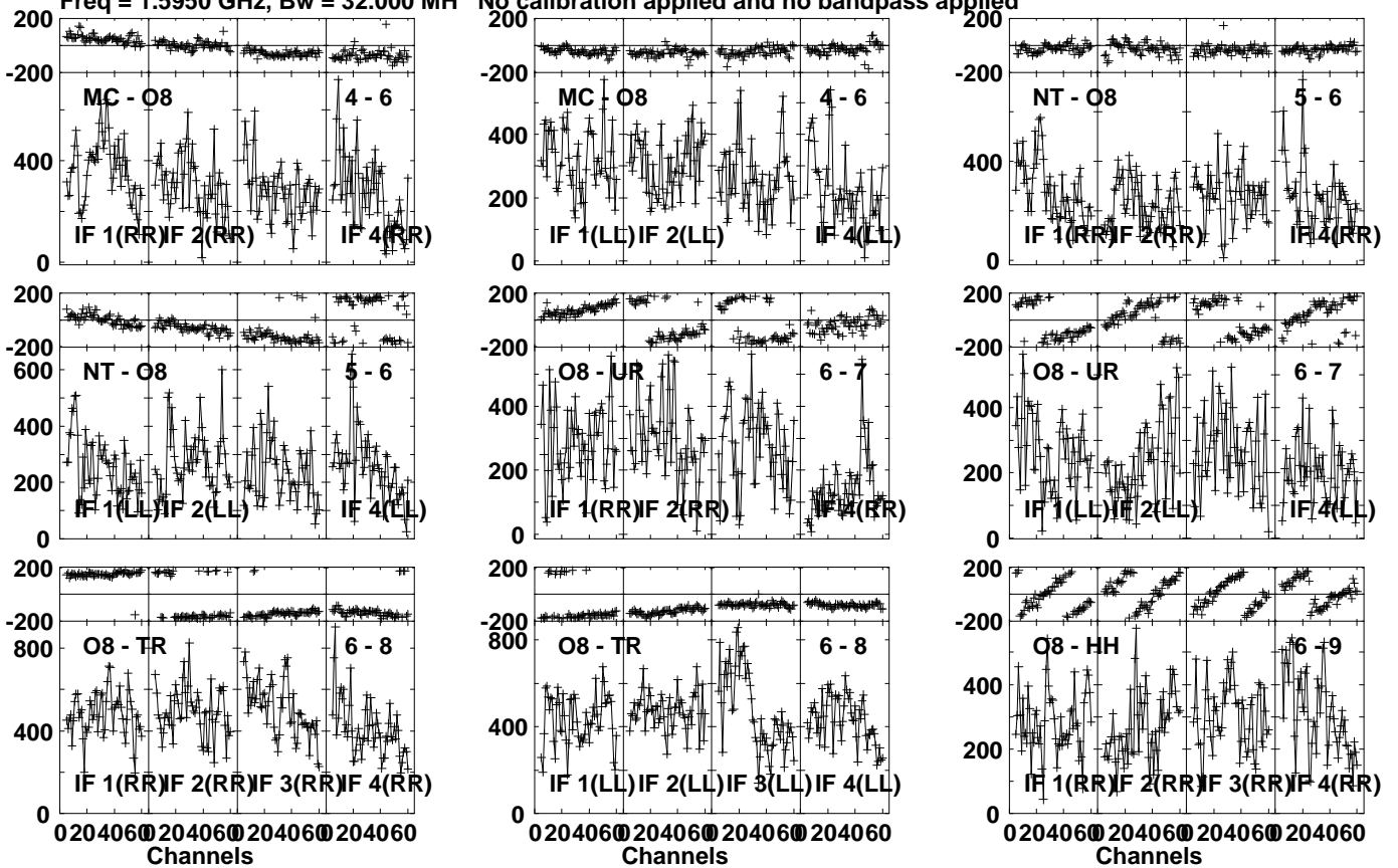
Lower frame: Micro Ampl Jy Top frame: Phas deg Vector averaged cross-power spectrum Several baselines displayed Timerange: 00/07:26:42 to 00/07:27:40
