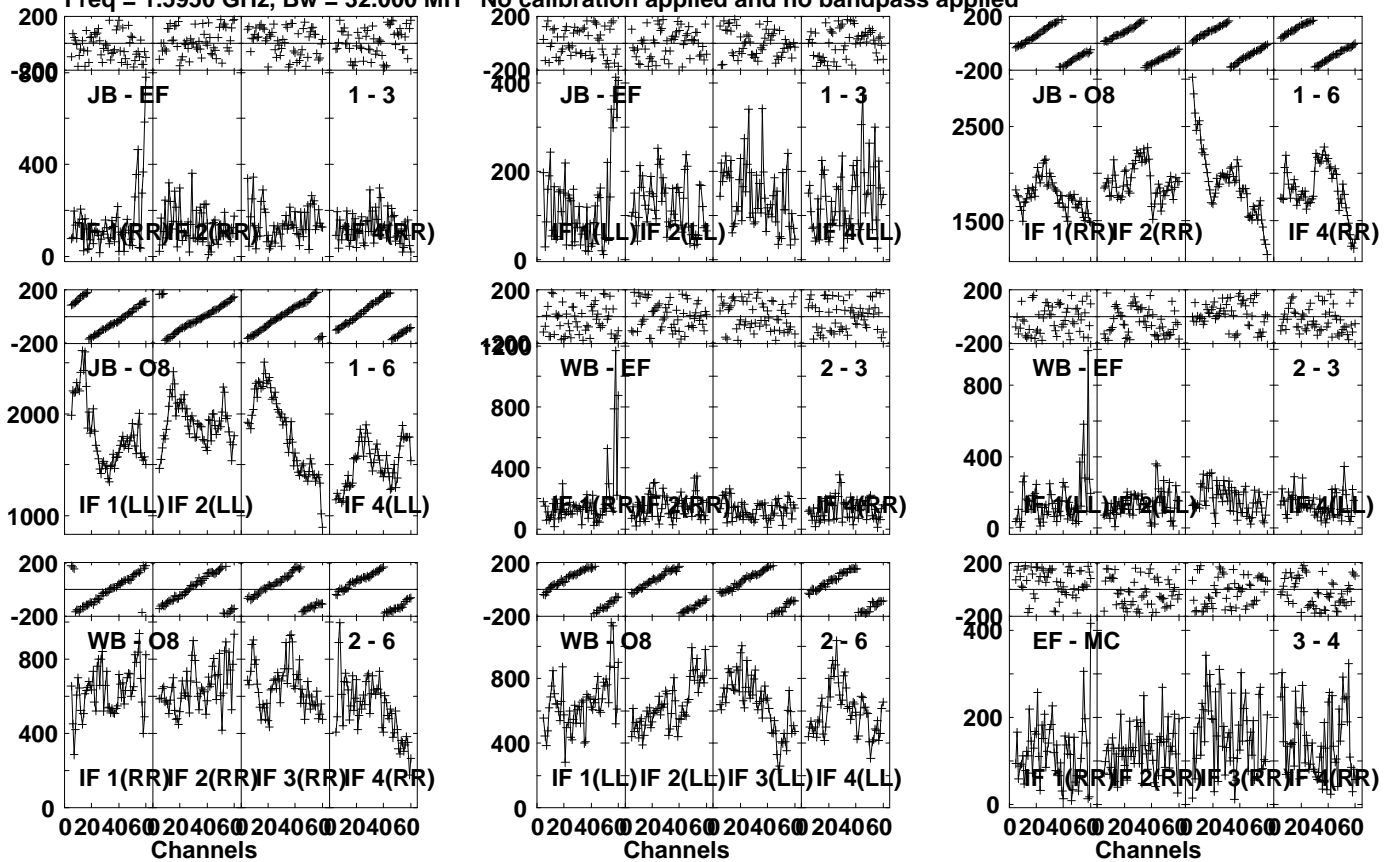
Lower frame: Micro Ampl Jy Top frame: Phas deg Vector averaged cross-power spectrum Several baselines displayed Timerange: 00/11:43:22 to 00/11:44:20
