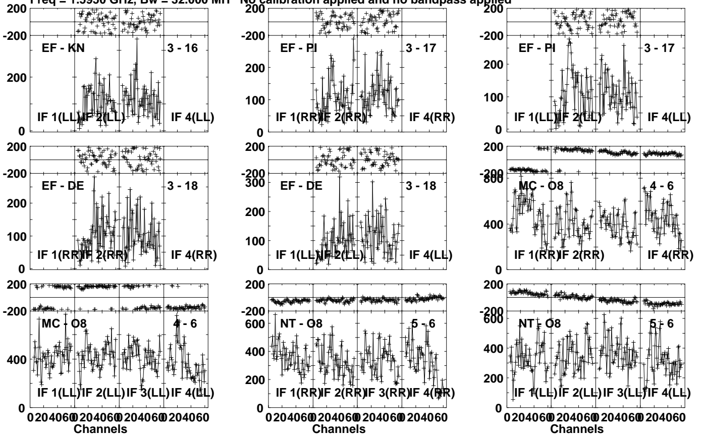
Lower frame: Micro Ampl Jy Top frame: Phas deg Vector averaged cross-power spectrum Several baselines displayed Timerange: 00/10:59:39 to 00/11:01:07
