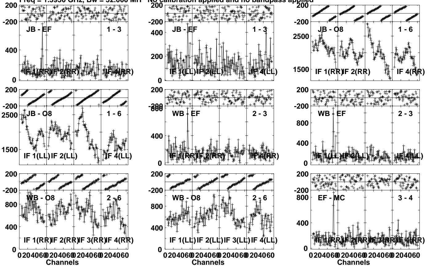
Lower frame: Micro Ampl Jy Top frame: Phas deg Vector averaged cross-power spectrum Several baselines displayed Timerange: 00/11:49:52 to 00/11:50:50
