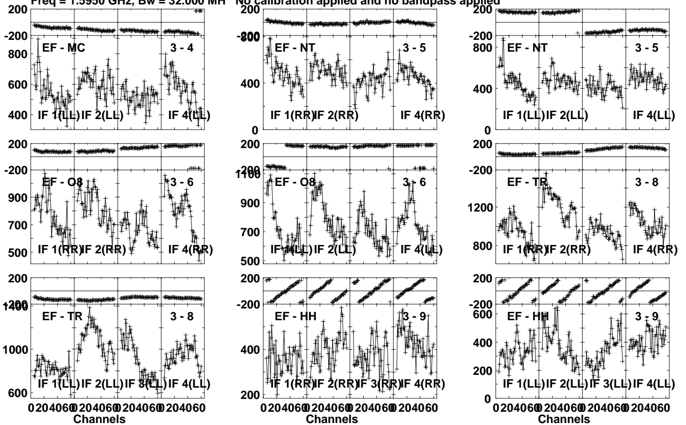
Lower frame: Micro Ampl Jy Top frame: Phas deg Vector averaged cross-power spectrum Several baselines displayed Timerange: 00/04:19:25 to 00/04:22:53
