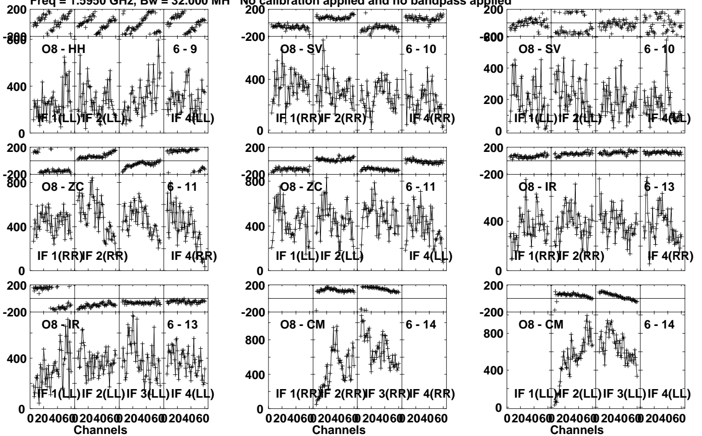
Lower frame: Micro Ampl Jy Top frame: Phas deg Vector averaged cross-power spectrum Several baselines displayed Timerange: 00/07:05:11 to 00/07:06:09
