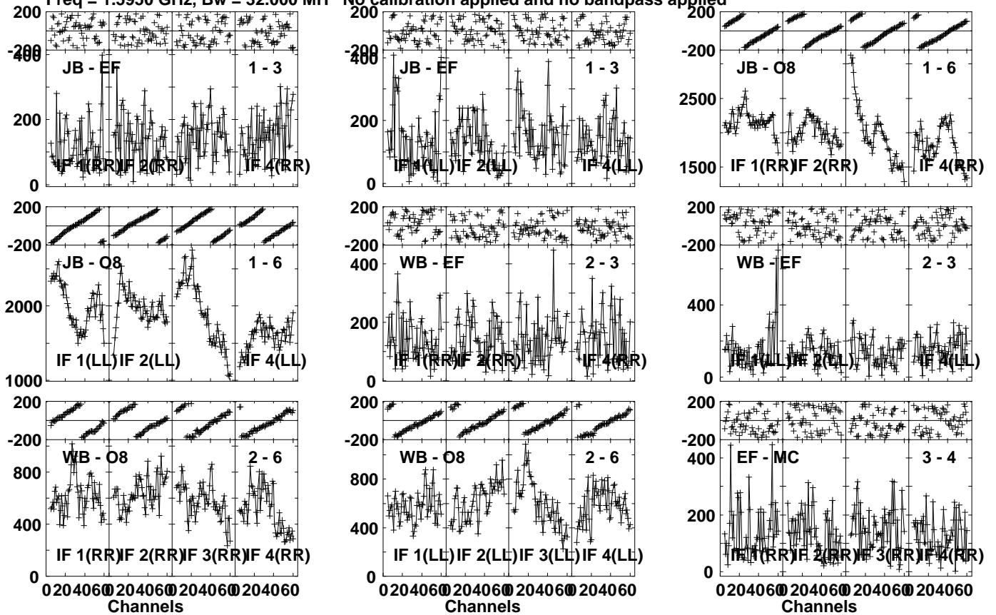
Lower frame: Micro Ampl Jy Top frame: Phas deg Vector averaged cross-power spectrum Several baselines displayed Timerange: 00/11:59:01 to 00/11:59:59
