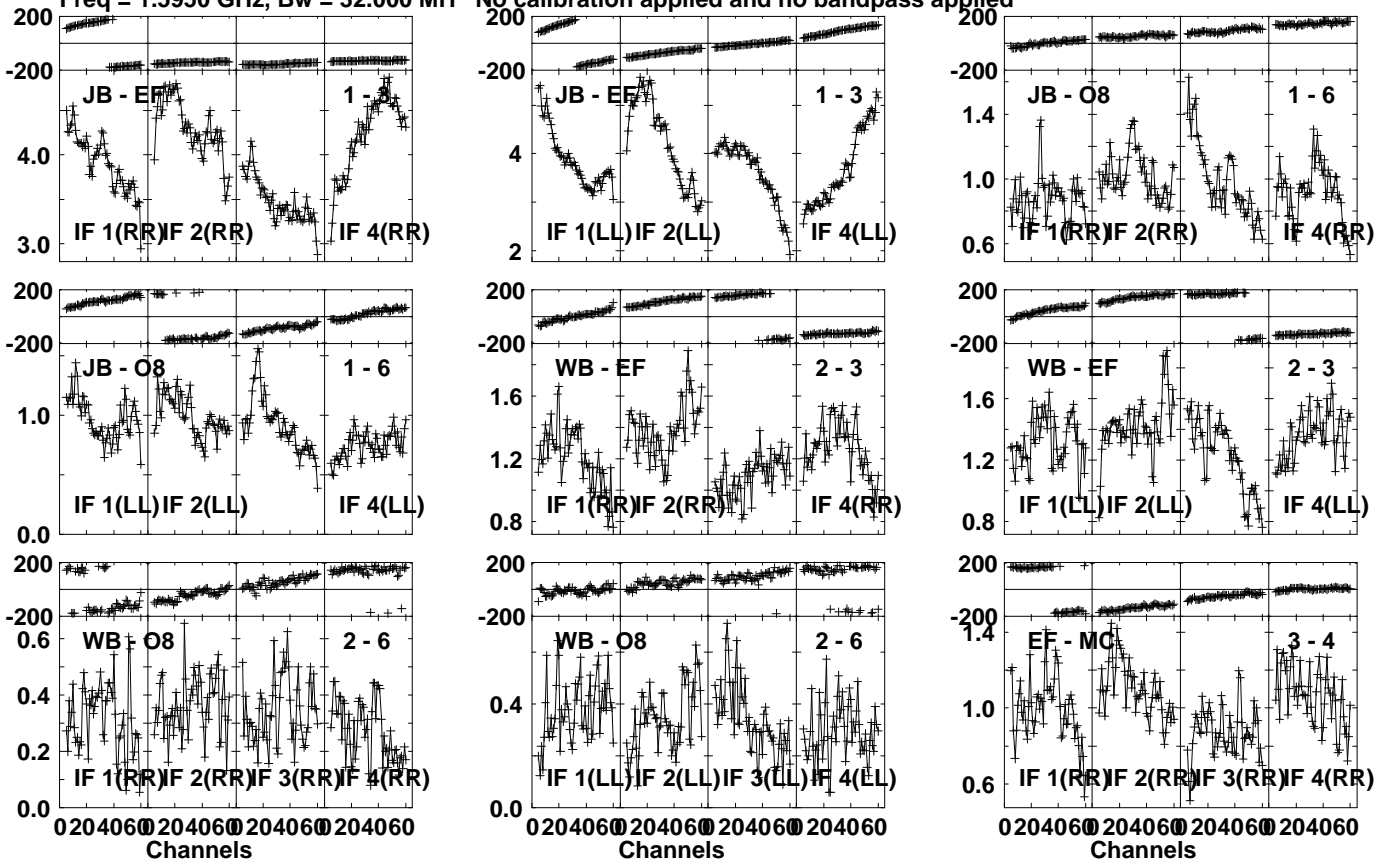
Lower frame: Milli Ampl Jy Top frame: Phas deg Vector averaged cross-power spectrum Several baselines displayed Timerange: 00/04:49:20 to 00/04:50:18
