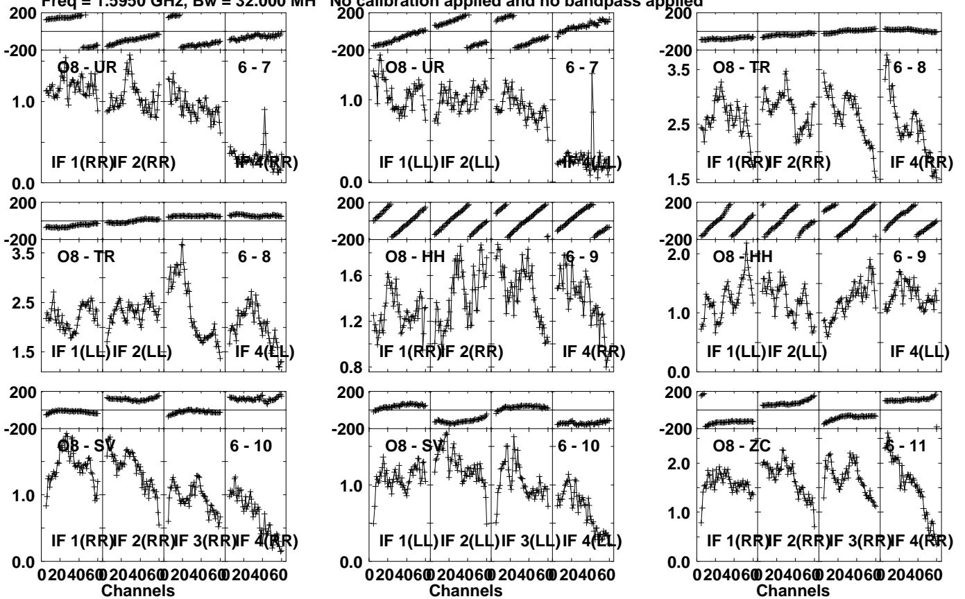
Lower frame: Milli Ampl Jy Top frame: Phas deg Vector averaged cross-power spectrum Several baselines displayed Timerange: 00/08:33:35 to 00/08:35:03
