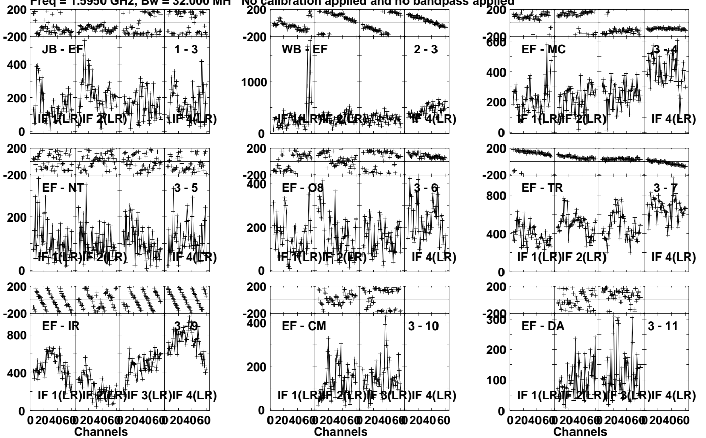
Lower frame: Micro Ampl Jy Top frame: Phas deg Vector averaged cross-power spectrum Several baselines displayed Timerange: 01/08:16:26 to 01/08:17:54
