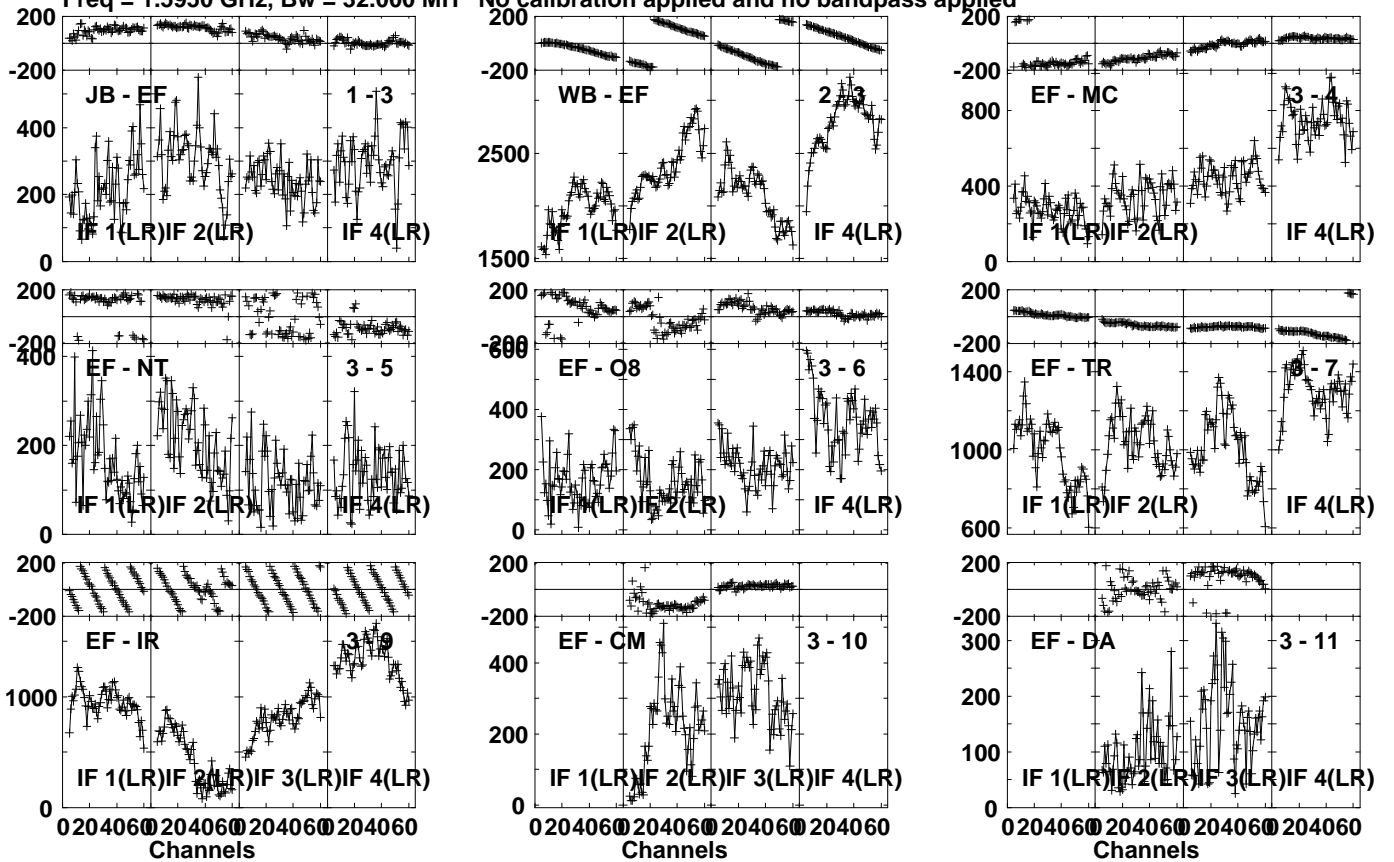
Lower frame: Micro Ampl Jy Top frame: Phas deg Vector averaged cross-power spectrum Several baselines displayed Timerange: 01/04:18:56 to 01/04:20:54
