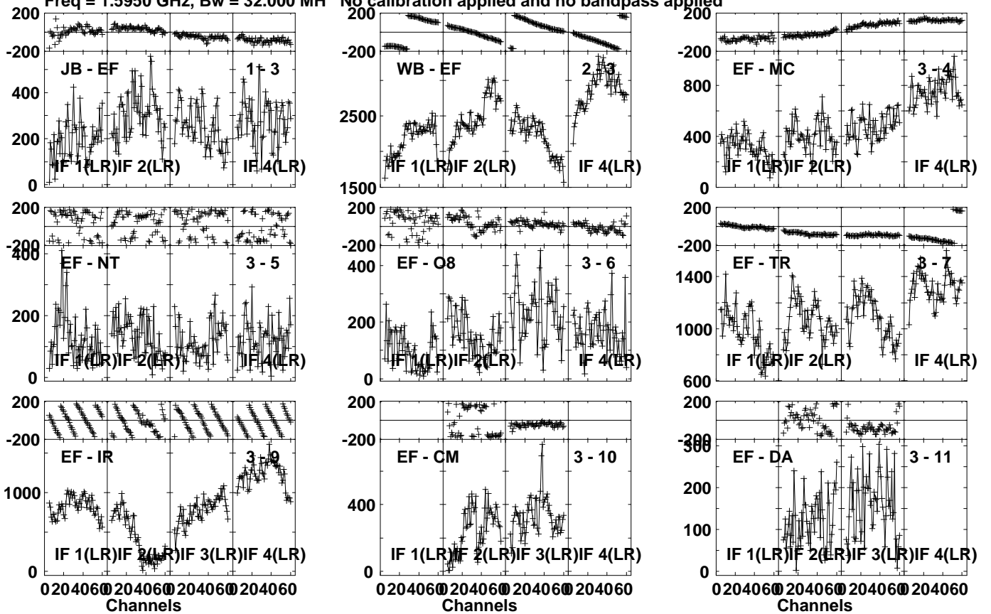
Lower frame: Micro Ampl Jy Top frame: Phas deg Vector averaged cross-power spectrum Several baselines displayed Timerange: 01/06:14:26 to 01/06:15:54
