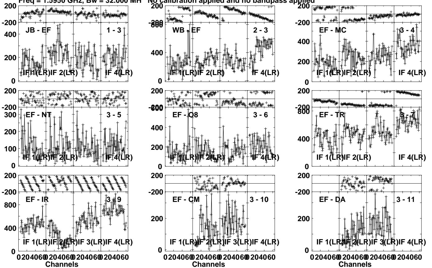
Lower frame: Micro Ampl Jy Top frame: Phas deg Vector averaged cross-power spectrum Several baselines displayed Timerange: 01/08:40:26 to 01/08:41:54
