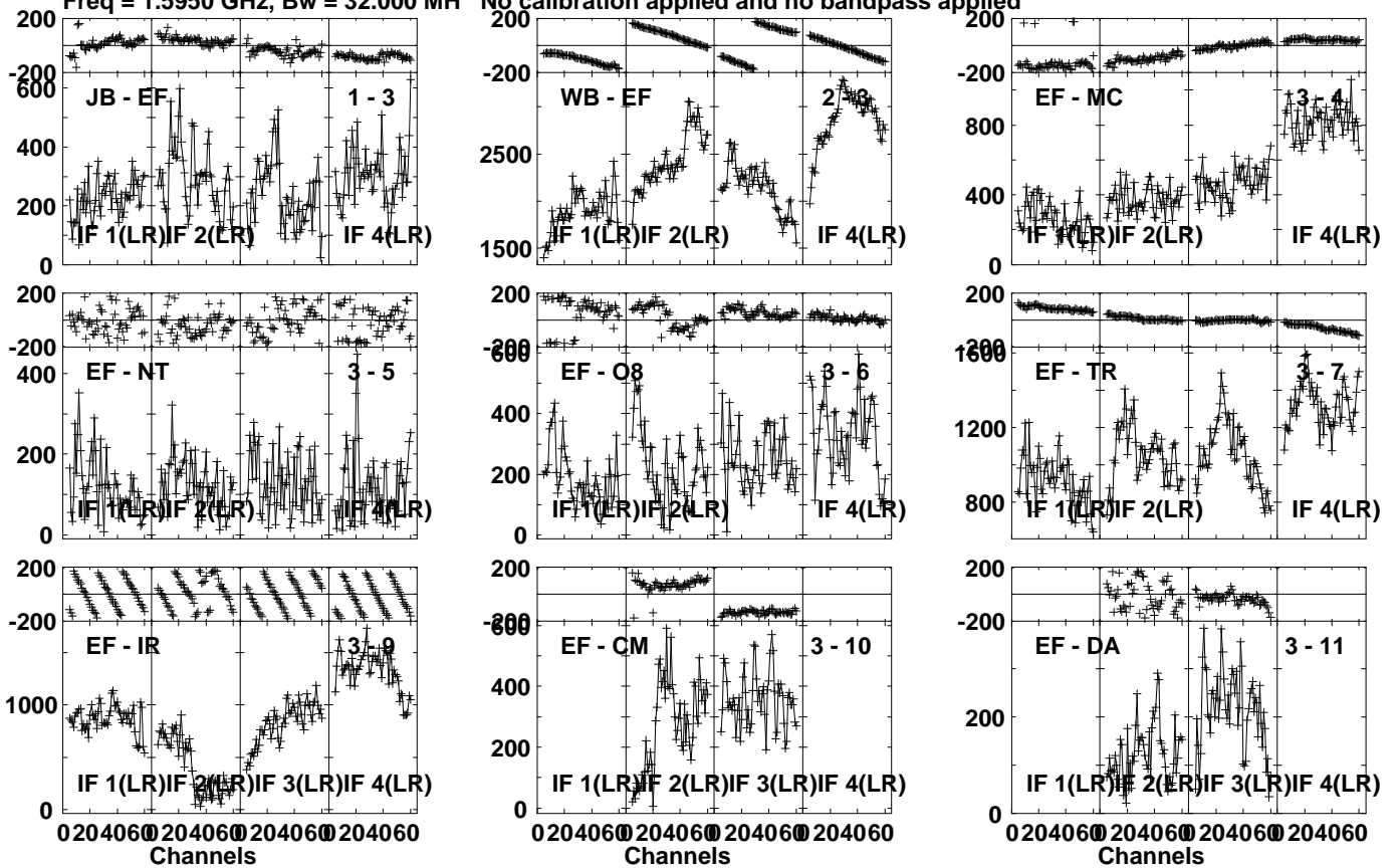
Lower frame: Micro Ampl Jy Top frame: Phas deg Vector averaged cross-power spectrum Several baselines displayed Timerange: 01/04:50:56 to 01/04:52:24
