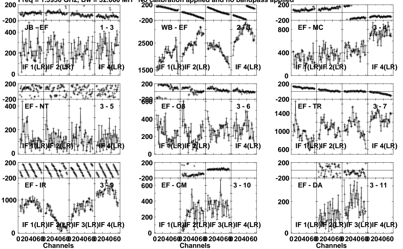
Lower frame: Micro Ampl Jy Top frame: Phas deg Vector averaged cross-power spectrum Several baselines displayed Timerange: 01/05:45:46 to 01/05:47:14
