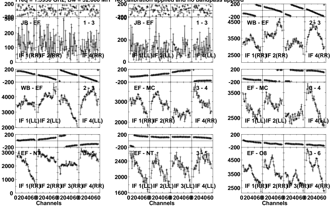
Lower frame: Micro Ampl Jy Top frame: Phas deg Vector averaged cross-power spectrum Several baselines displayed Timerange: 00/14:56:31 to 00/14:57:59
