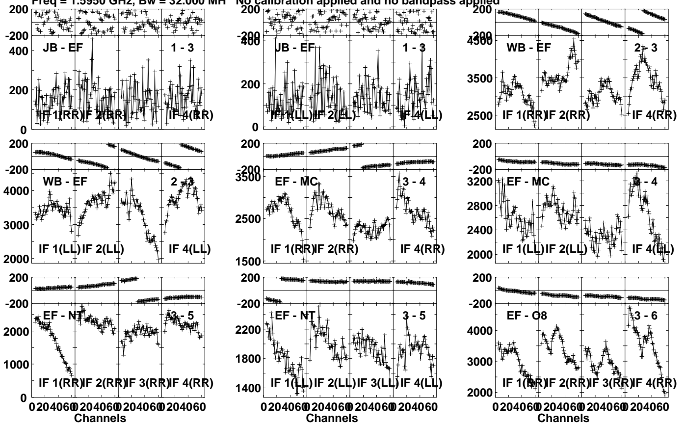
Lower frame: Micro Ampl Jy Top frame: Phas deg Vector averaged cross-power spectrum Several baselines displayed Timerange: 00/13:01:01 to 00/13:02:59
