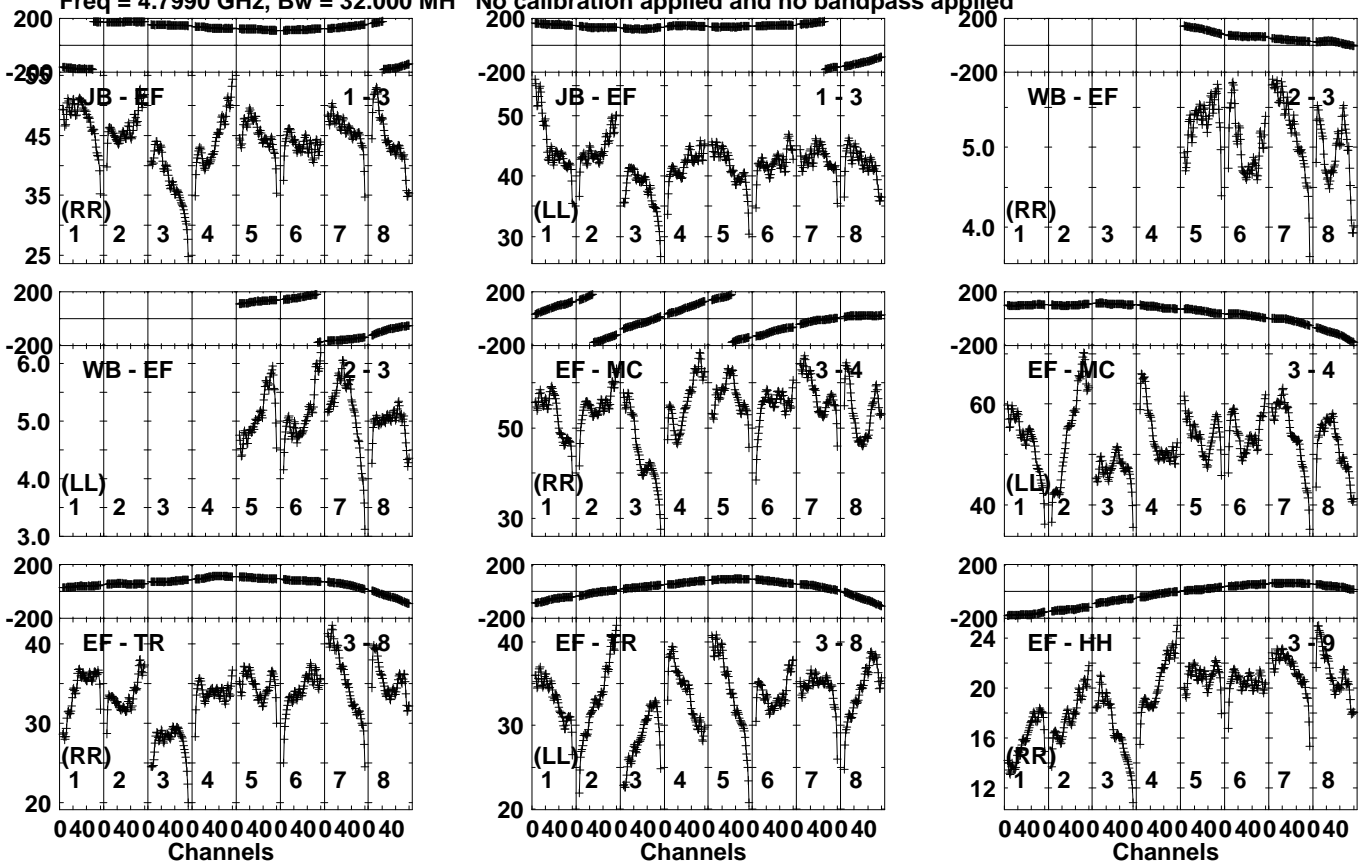
Lower frame: Milli Ampl Jy Top frame: Phas deg Vector averaged cross-power spectrum Several baselines displayed Timerange: 00/05:00:11 to 00/05:05:09
