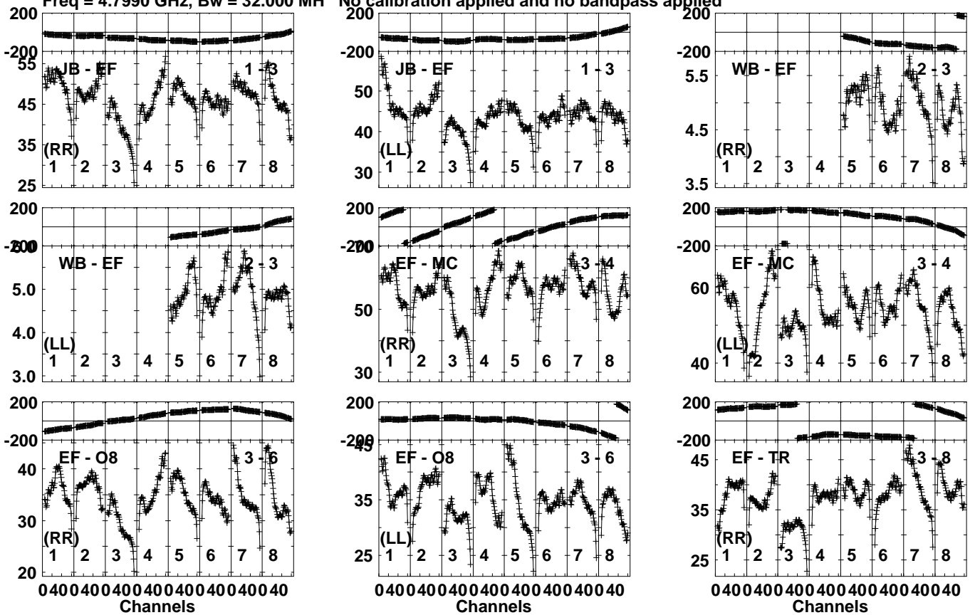
Lower frame: Milli Ampl Jy Top frame: Phas deg Vector averaged cross-power spectrum Several baselines displayed Timerange: 00/06:44:51 to 00/06:49:49
