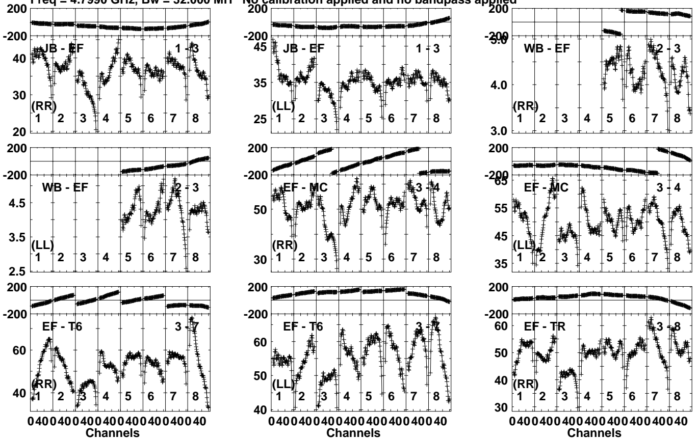
Lower frame: Milli Ampl Jy Top frame: Phas deg Vector averaged cross-power spectrum Several baselines displayed Timerange: 00/04:26:31 to 00/04:31:29
