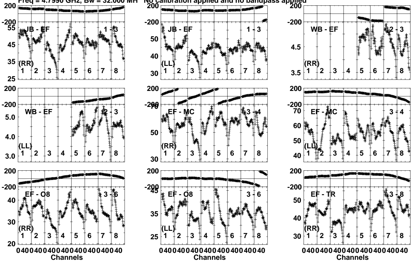
Lower frame: Milli Ampl Jy Top frame: Phas deg Vector averaged cross-power spectrum Several baselines displayed Timerange: 00/06:21:51 to 00/06:26:49
