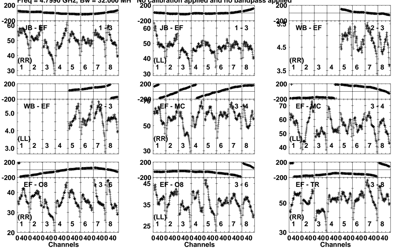
Lower frame: Milli Ampl Jy Top frame: Phas deg Vector averaged cross-power spectrum Several baselines displayed Timerange: 00/07:07:51 to 00/07:12:49
