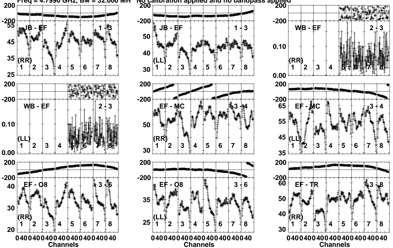
Lower frame: Milli Ampl Jy Top frame: Phas deg Vector averaged cross-power spectrum Several baselines displayed Timerange: 00/06:04:11 to 00/06:09:09
