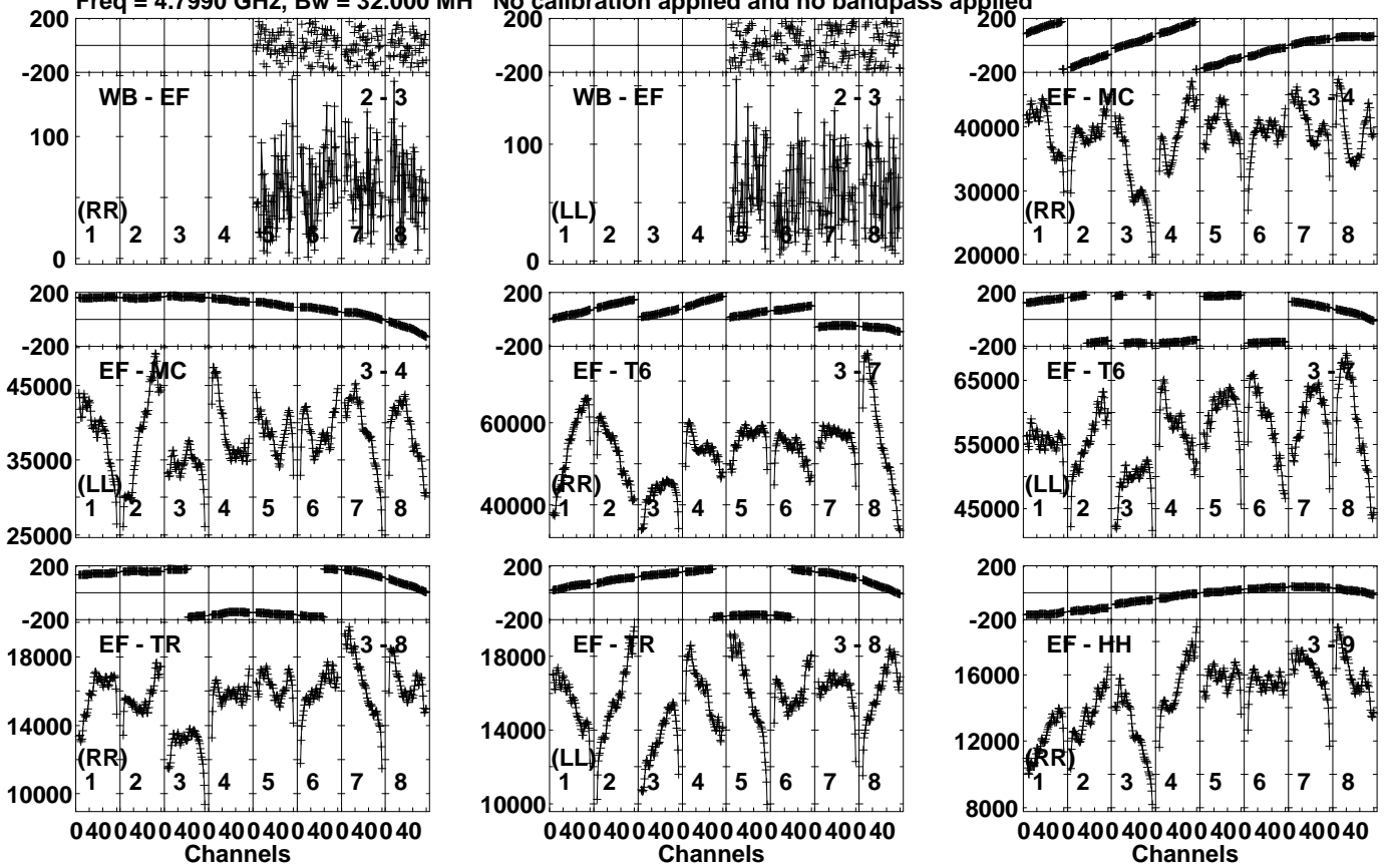
Lower frame: Micro Ampl Jy Top frame: Phas deg Vector averaged cross-power spectrum Several baselines displayed Timerange: 00/03:35:11 to 00/03:40:09
