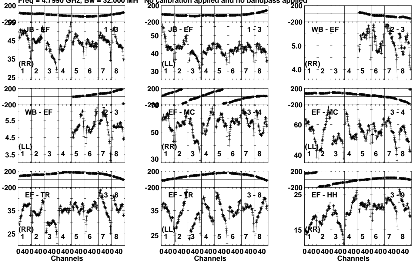
Lower frame: Milli Ampl Jy Top frame: Phas deg Vector averaged cross-power spectrum Several baselines displayed Timerange: 00/05:35:51 to 00/05:40:49
