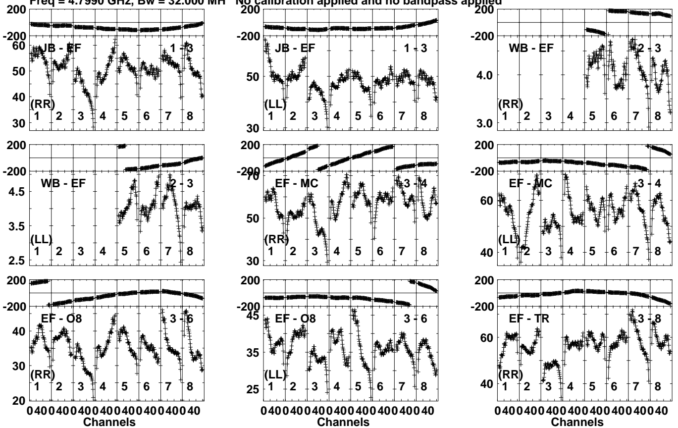
Lower frame: Milli Ampl Jy Top frame: Phas deg Vector averaged cross-power spectrum Several baselines displayed Timerange: 00/07:25:31 to 00/07:30:29
