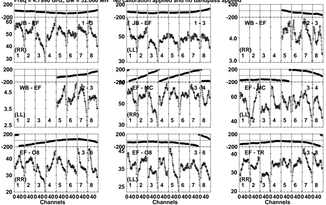
Lower frame: Milli Ampl Jy Top frame: Phas deg Vector averaged cross-power spectrum Several baselines displayed Timerange: 00/07:13:11 to 00/07:18:09
