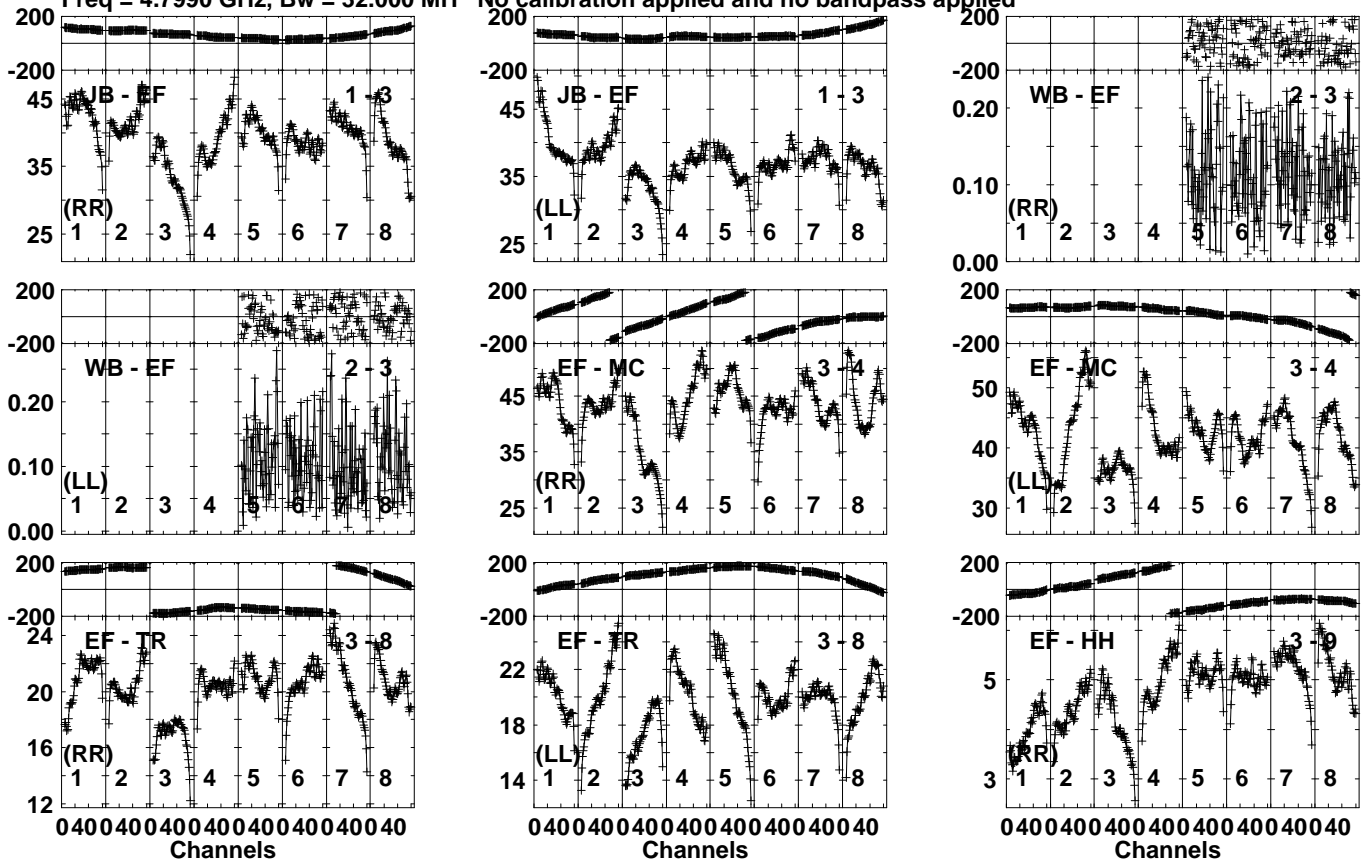
Lower frame: Milli Ampl Jy Top frame: Phas deg Vector averaged cross-power spectrum Several baselines displayed Timerange: 00/05:09:41 to 00/05:11:39
