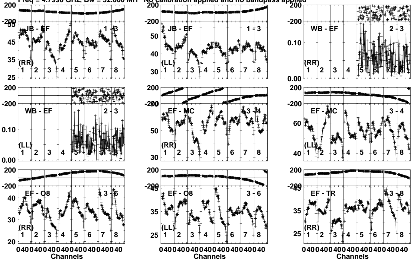
Lower frame: Milli Ampl Jy Top frame: Phas deg Vector averaged cross-power spectrum Several baselines displayed Timerange: 00/05:53:31 to 00/05:58:29
