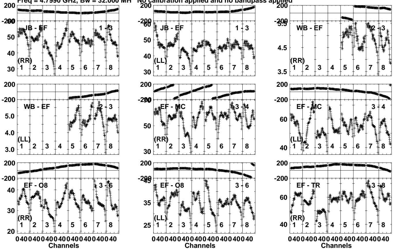
Lower frame: Milli Ampl Jy Top frame: Phas deg Vector averaged cross-power spectrum Several baselines displayed Timerange: 00/05:48:11 to 00/05:53:09
