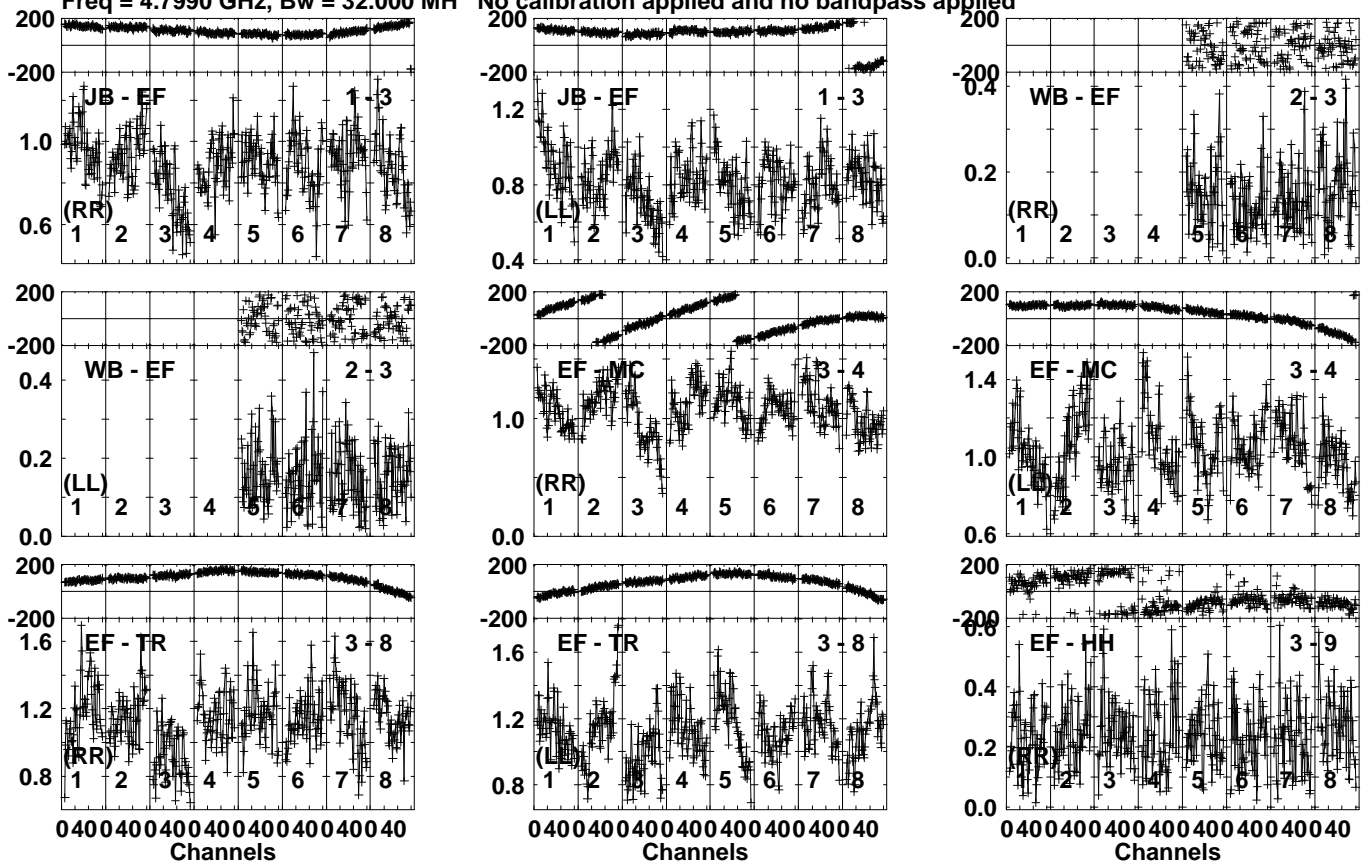
Lower frame: Milli Ampl Jy Top frame: Phas deg Vector averaged cross-power spectrum Several baselines displayed Timerange: 00/05:05:41 to 00/05:06:39
