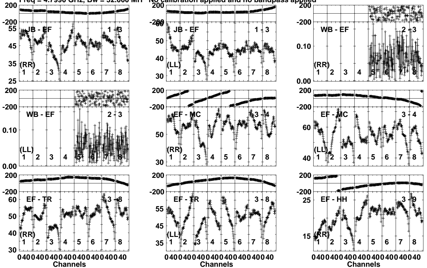
Lower frame: Milli Ampl Jy Top frame: Phas deg Vector averaged cross-power spectrum Several baselines displayed Timerange: 00/05:41:11 to 00/05:46:09
