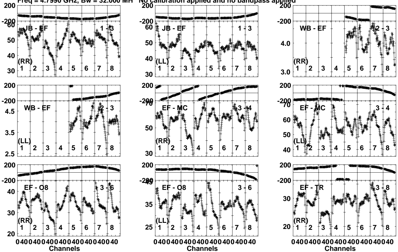
Lower frame: Milli Ampl Jy Top frame: Phas deg Vector averaged cross-power spectrum Several baselines displayed Timerange: 00/07:53:51 to 00/07:58:49
