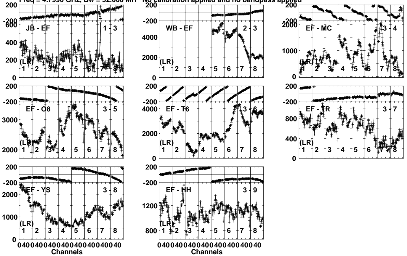
Lower frame: Micro Ampl Jy Top frame: Phas deg Vector averaged cross-power spectrum Several baselines displayed Timerange: 00/09:05:51 to 00/09:10:49
