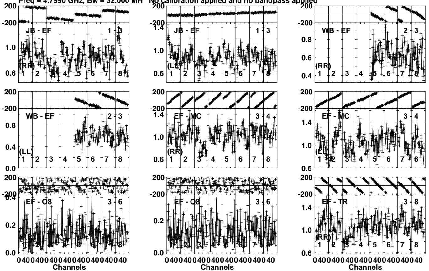
Lower frame: Milli Ampl Jy Top frame: Phas deg Vector averaged cross-power spectrum Several baselines displayed Timerange: 00/10:18:01 to 00/10:18:59
