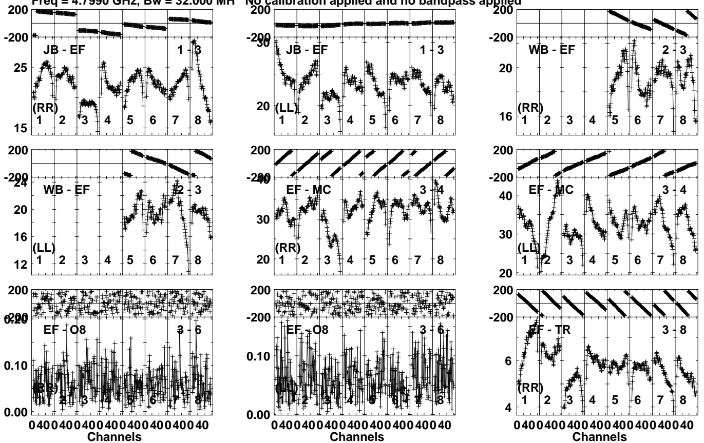
Lower frame: Milli Ampl Jy Top frame: Phas deg Vector averaged cross-power spectrum Several baselines displayed Timerange: 00/09:44:11 to 00/09:49:09
