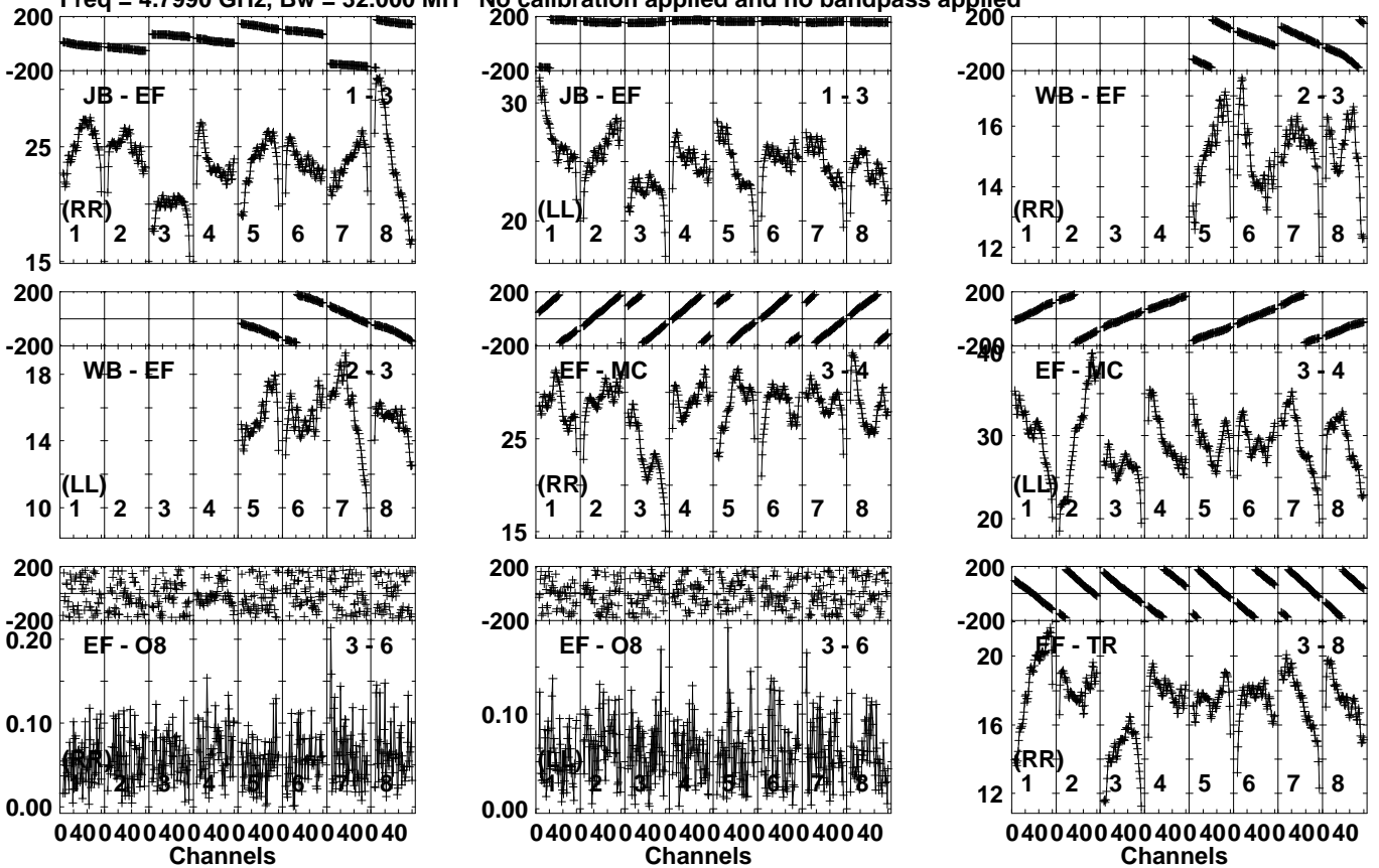
Lower frame: Milli Ampl Jy Top frame: Phas deg Vector averaged cross-power spectrum Several baselines displayed Timerange: 00/07:48:51 to 00/07:53:49
