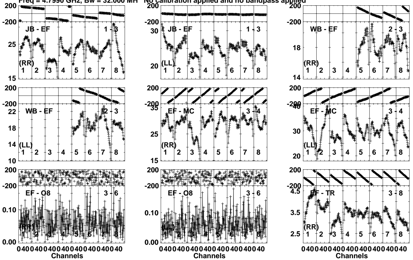
Lower frame: Milli Ampl Jy Top frame: Phas deg Vector averaged cross-power spectrum Several baselines displayed Timerange: 00/07:36:31 to 00/07:41:29
