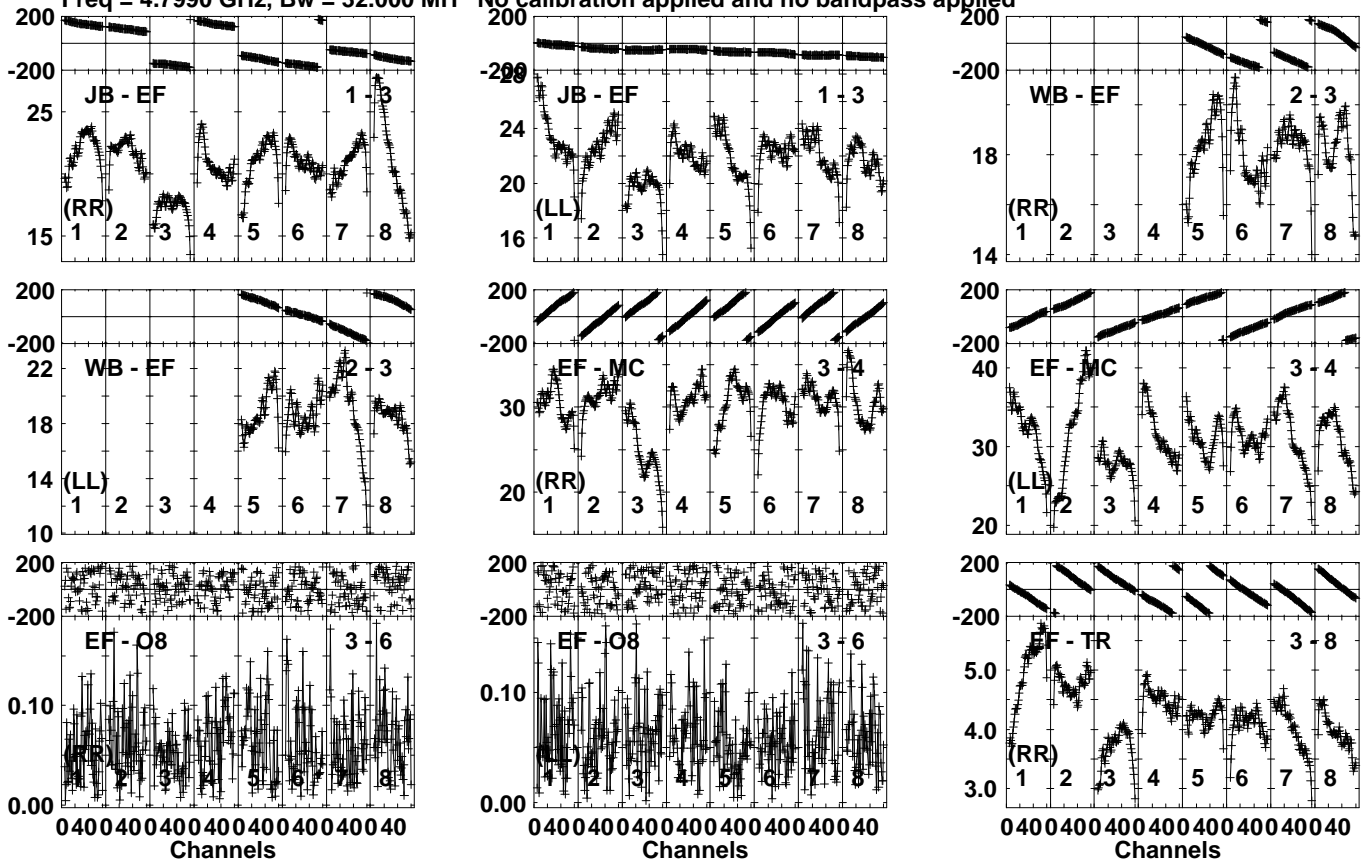
Lower frame: Milli Ampl Jy Top frame: Phas deg Vector averaged cross-power spectrum Several baselines displayed Timerange: 00/05:59:11 to 00/06:04:09
