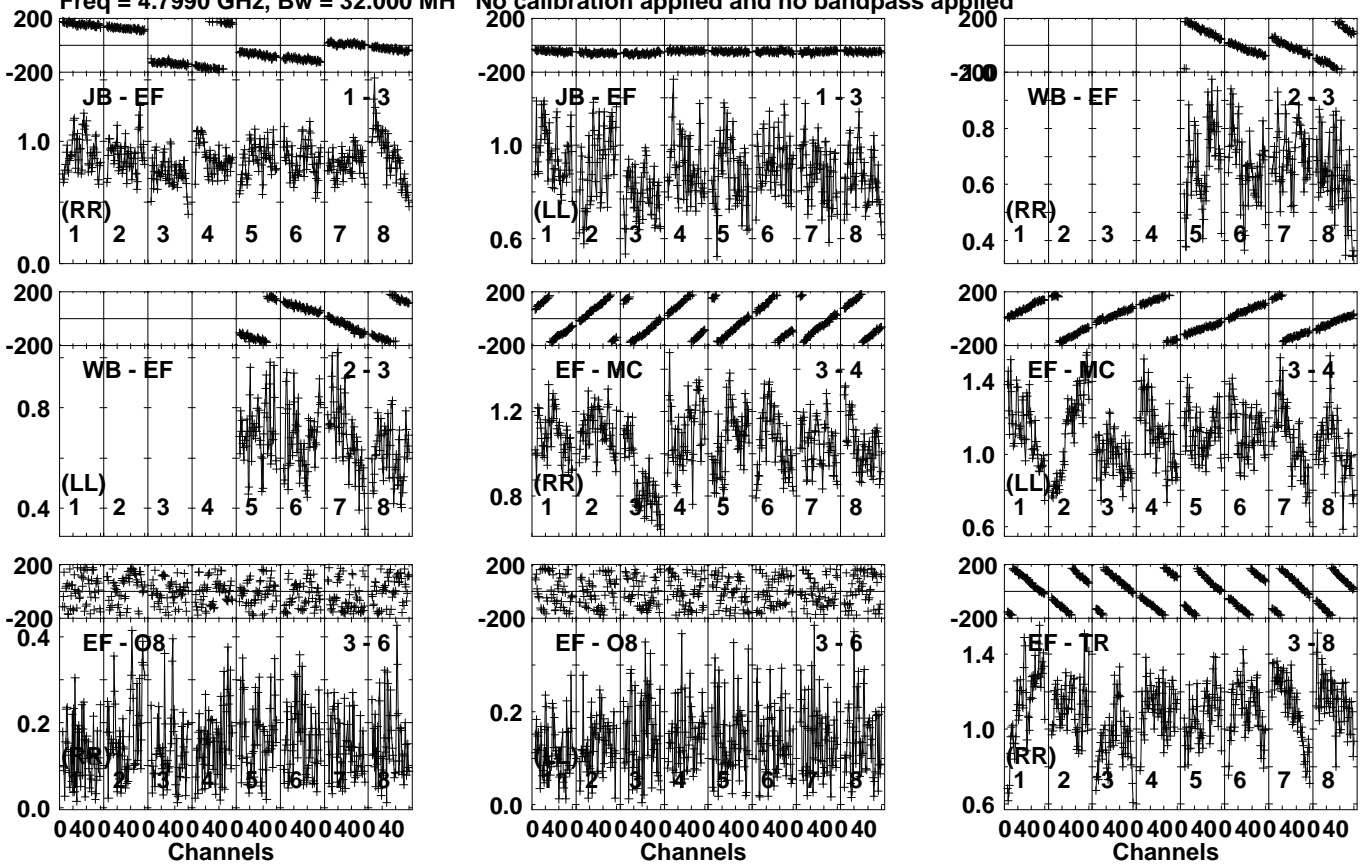
Lower frame: Milli Ampl Jy Top frame: Phas deg Vector averaged cross-power spectrum Several baselines displayed Timerange: 00/08:28:01 to 00/08:28:59
