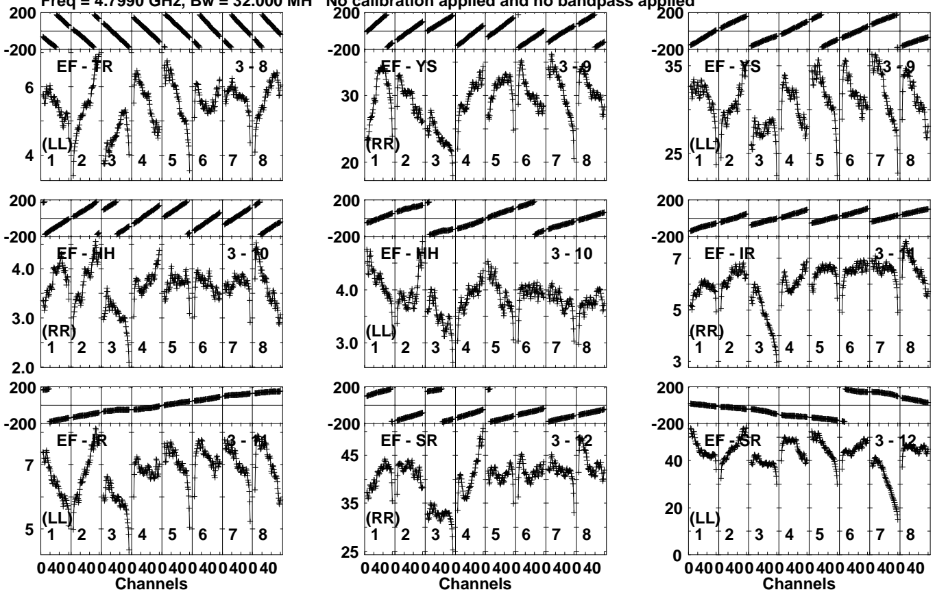
Lower frame: Milli Ampl Jy Top frame: Phas deg Vector averaged cross-power spectrum Several baselines displayed Timerange: 00/10:30:11 to 00/10:35:09
