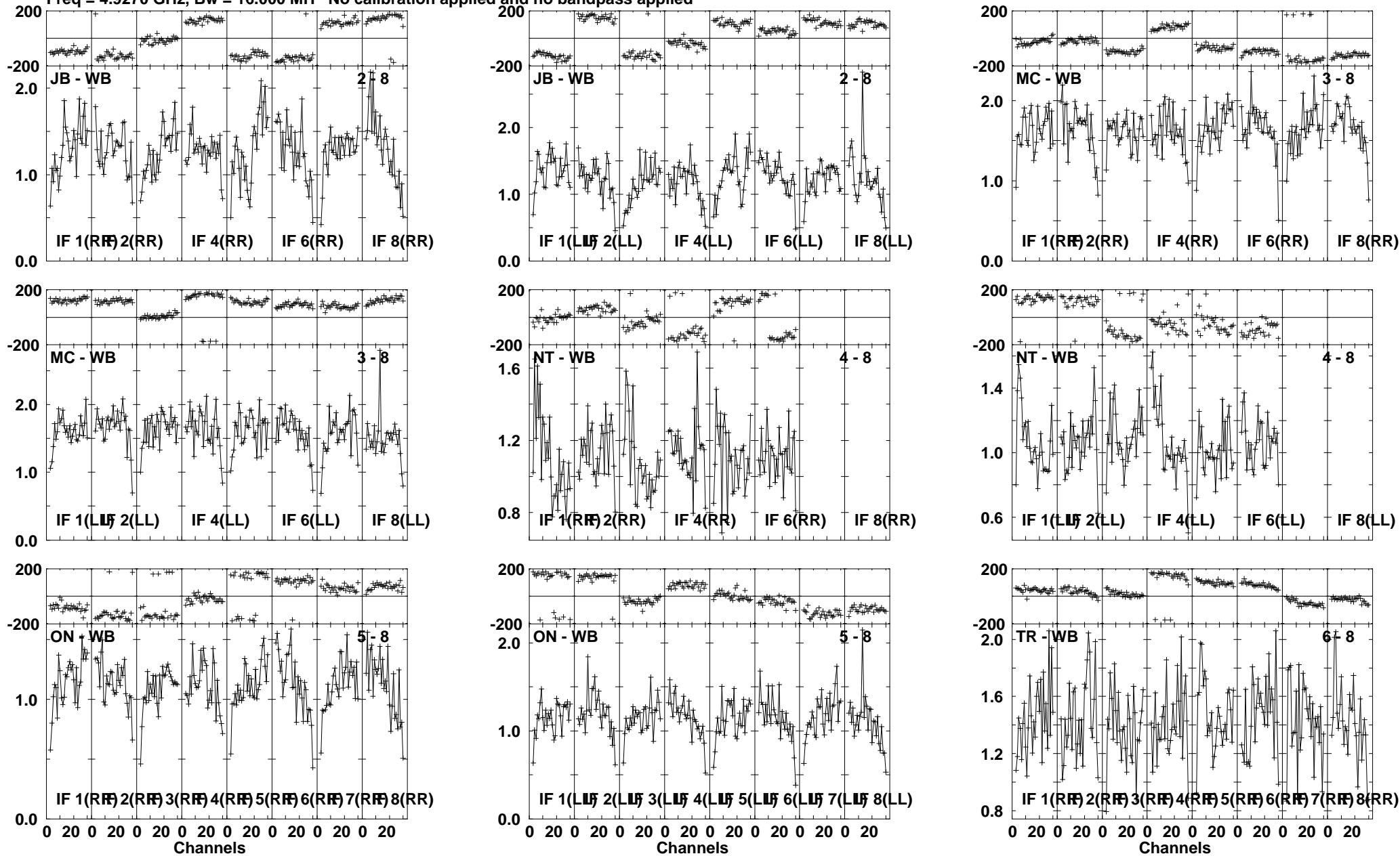
Lower frame: Milli Ampl Jy Top frame: Phas deg Scalar averaged cross-power spectrum Several baselines displayed Timerange: 00/20:47:53 to 00/20:48:47
