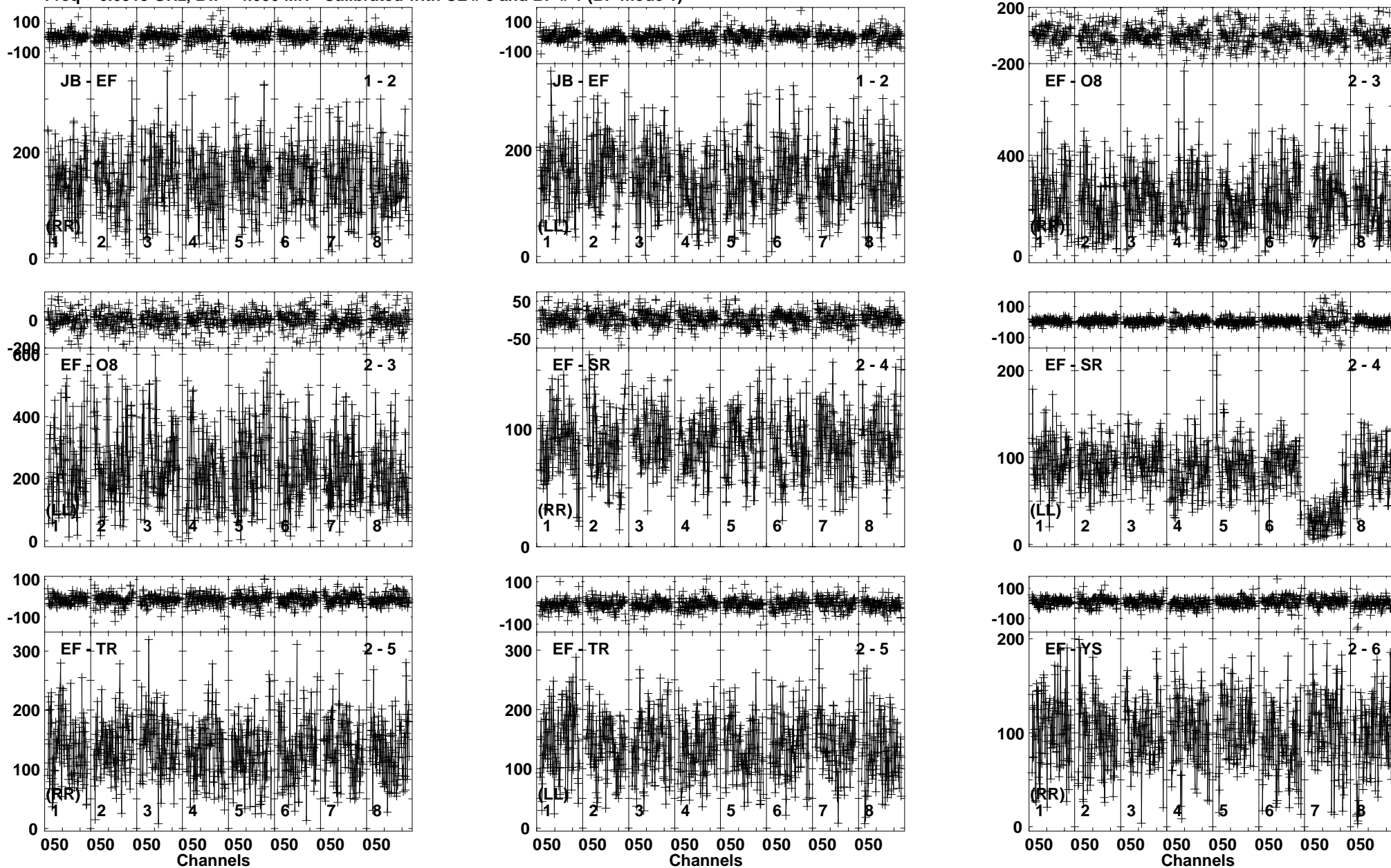
Lower frame: Milli Ampl Jy Top frame: Phas deg Vector averaged cross-power spectrum Baseline: JB (01) - EF (02) Timerange: 00/01:40:00 to 00/01:41:45
