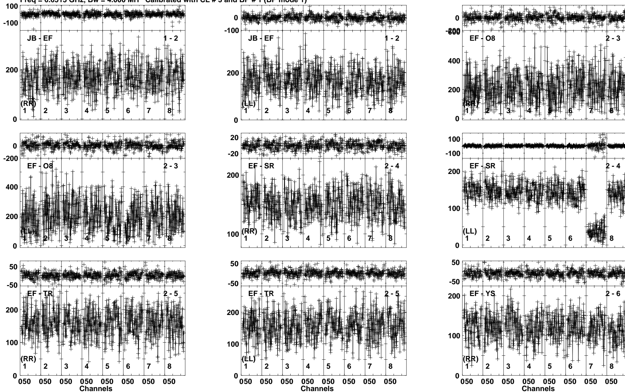
Lower frame: Milli Ampl Jy Top frame: Phas deg Vector averaged cross-power spectrum Baseline: JB (01) - EF (02) Timerange: 00/04:51:35 to 00/04:53:20
