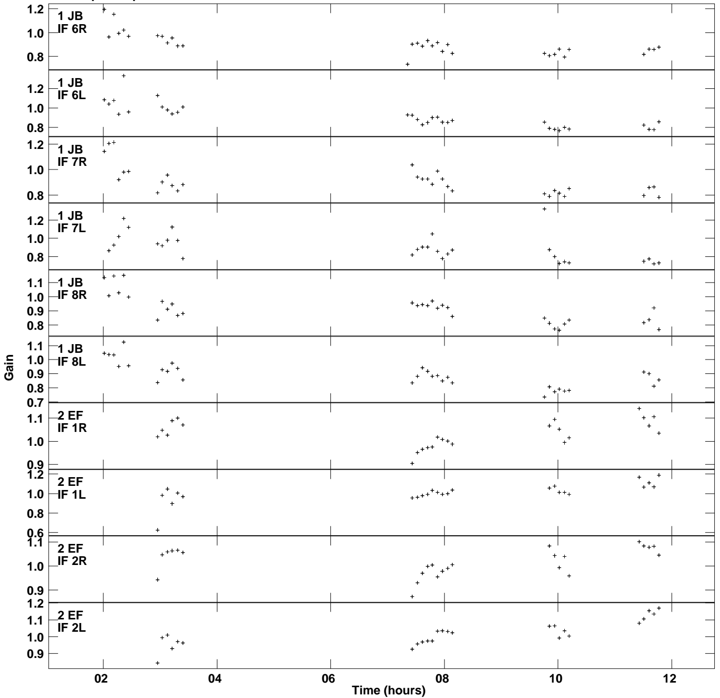
Plot file version 2 created 15-APR-2020 14:42:23 Gain amp vs UTC time for J1946+2300.MULTI.1 SN 2 Rpol & Lpol IF 1 - 8
