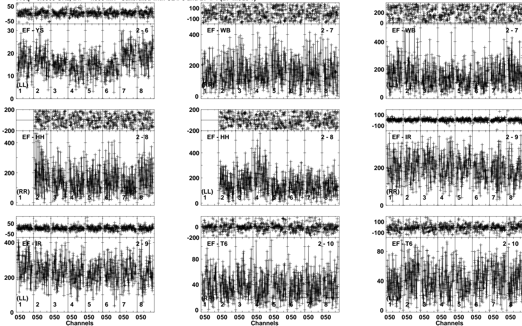
Lower frame: Milli Ampl Jy Top frame: Phas deg Vector averaged cross-power spectrum Baseline: EF (02) - YS (06) Timerange: 00/04:26:00 to 00/04:27:45
