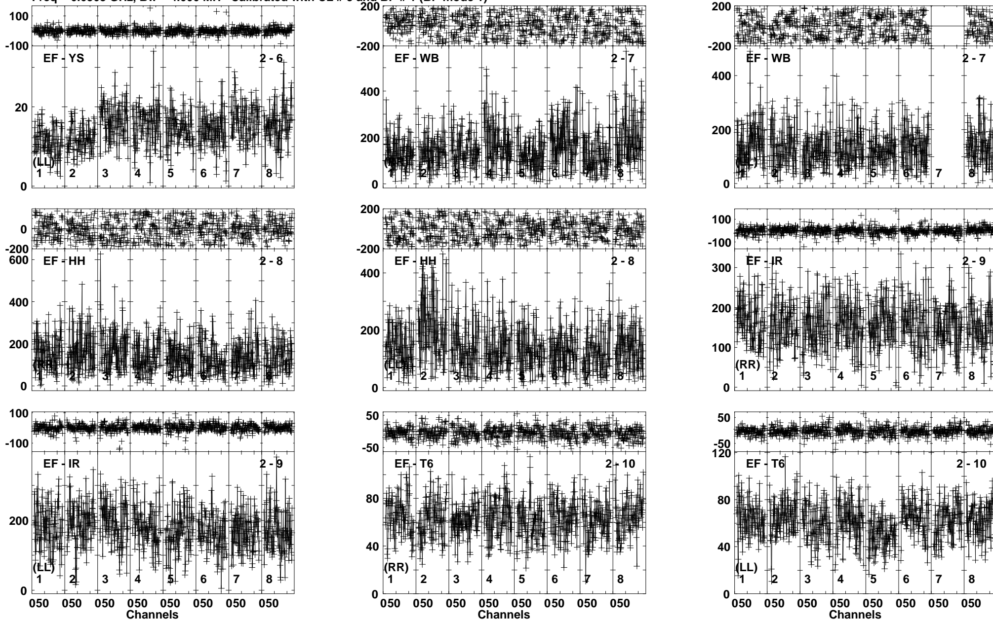
Lower frame: Milli Ampl Jy Top frame: Phas deg Vector averaged cross-power spectrum Baseline: EF (02) - YS (06) Timerange: 00/03:06:50 to 00/03:08:35
