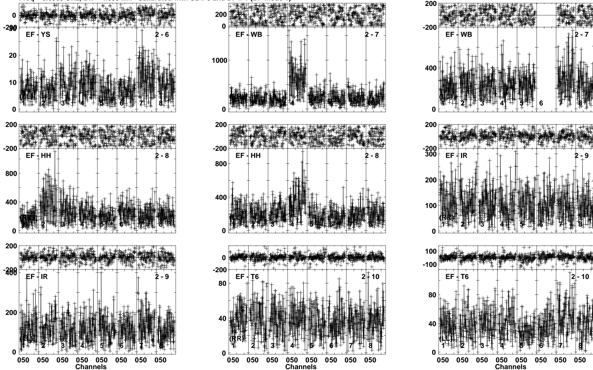
Lower frame: Milli Ampl Jy Top frame: Phas deg Vector averaged cross-power spectrum Baseline: EF (02) - YS (06) Timerange: 00/02:32:30 to 00/02:34:15
