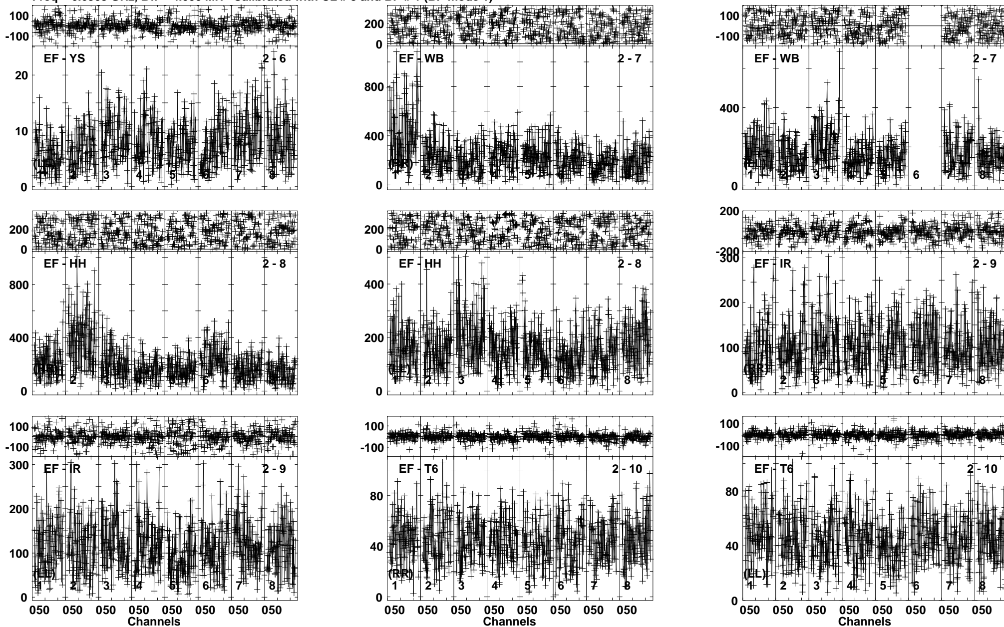
Lower frame: Milli Ampl Jy Top frame: Phas deg Vector averaged cross-power spectrum Baseline: EF (02) - YS (06) Timerange: 00/02:38:11 to 00/02:39:55
