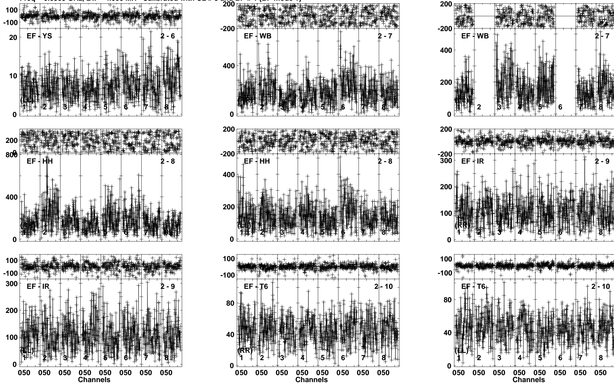
Lower frame: Milli Ampl Jy Top frame: Phas deg Vector averaged cross-power spectrum Baseline: EF (02) - YS (06) Timerange: 00/02:48:51 to 00/02:50:34
