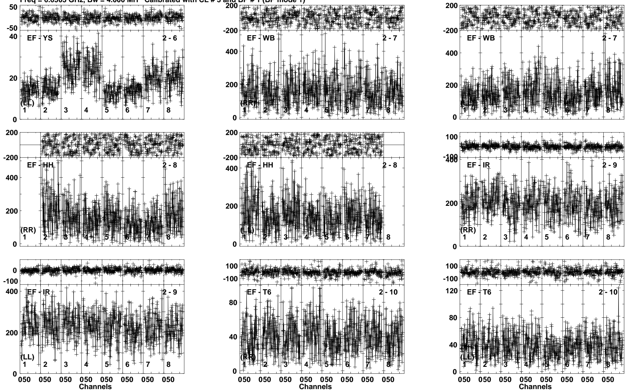
Lower frame: Milli Ampl Jy Top frame: Phas deg Vector averaged cross-power spectrum Baseline: EF (02) - YS (06) Timerange: 00/04:04:40 to 00/04:06:25
