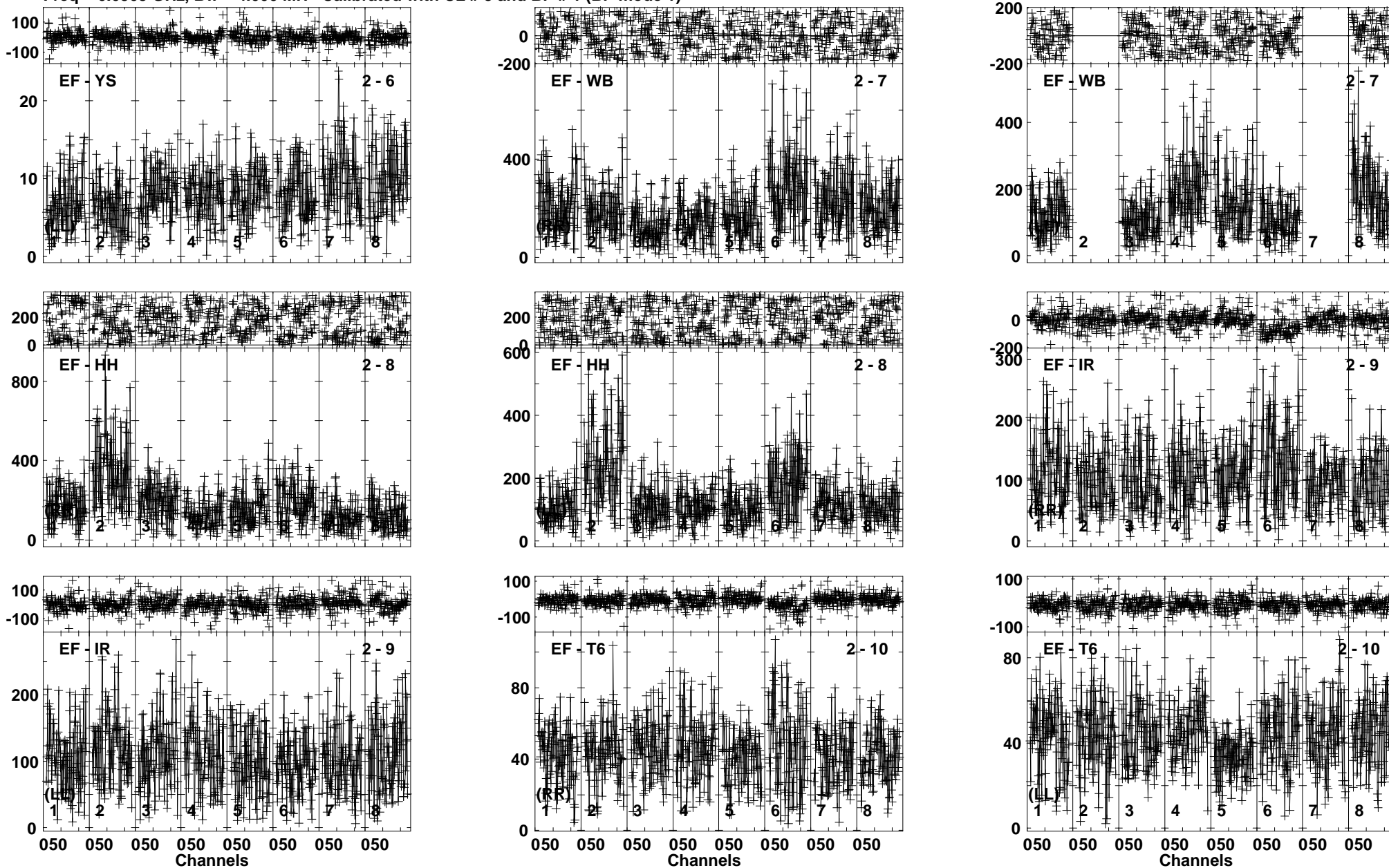
Lower frame: Milli Ampl Jy Top frame: Phas deg Vector averaged cross-power spectrum Baseline: EF (02) - YS (06) Timerange: 00/03:51:45 to 00/03:53:29
