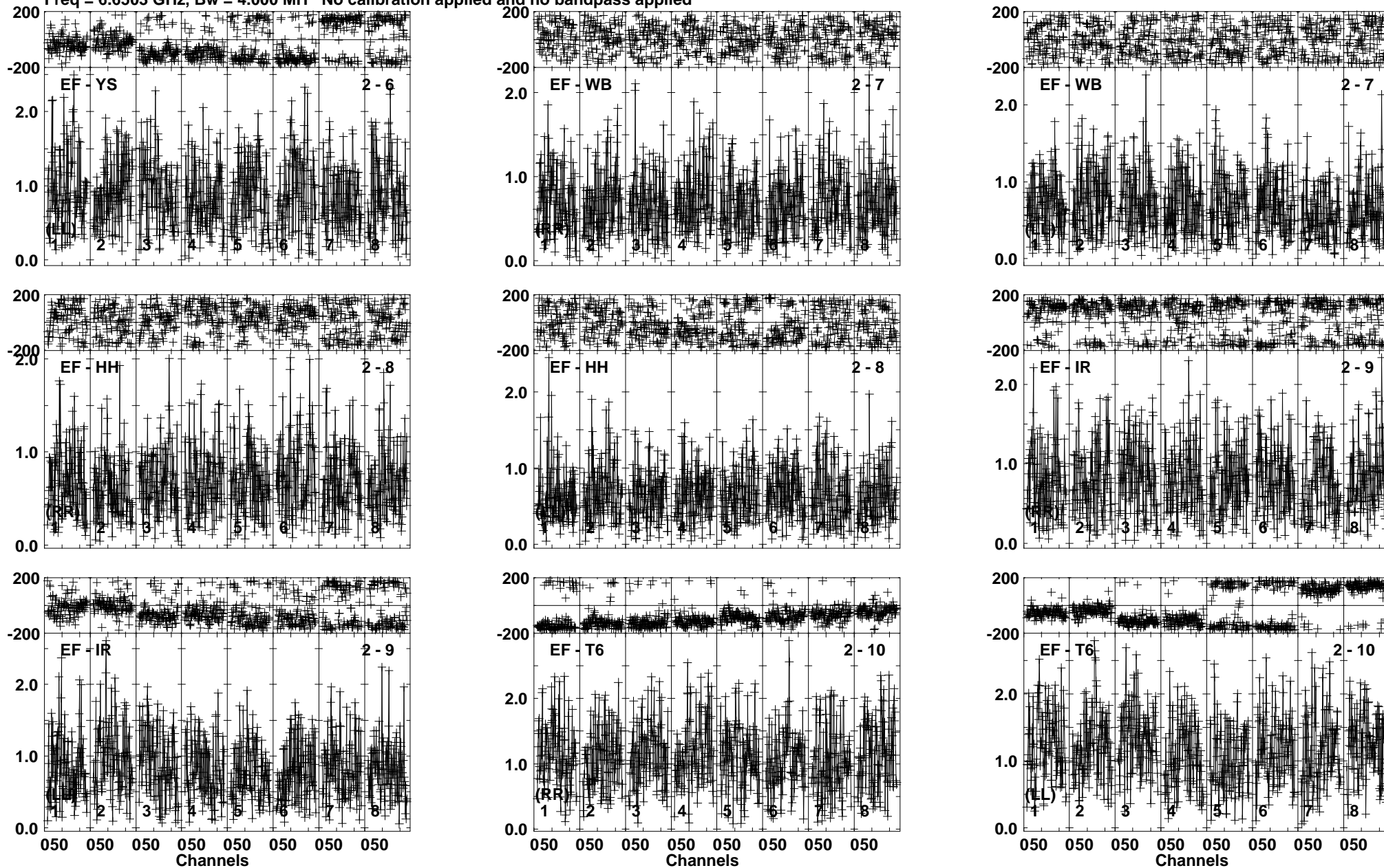
Lower frame: Milli Ampl Jy Top frame: Phas deg Vector averaged cross-power spectrum Baseline: EF (02) - YS (06) Timerange: 00/03:29:45 to 00/03:31:29
