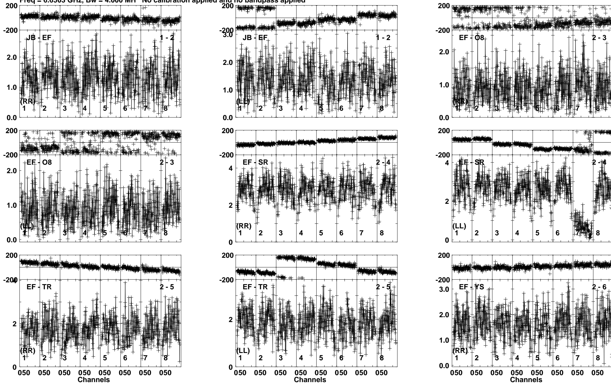
Lower frame: Milli Ampl Jy Top frame: Phas deg Vector averaged cross-power spectrum Baseline: JB (01) - EF (02) Timerange: 00/10:11:06 to 00/10:12:44
