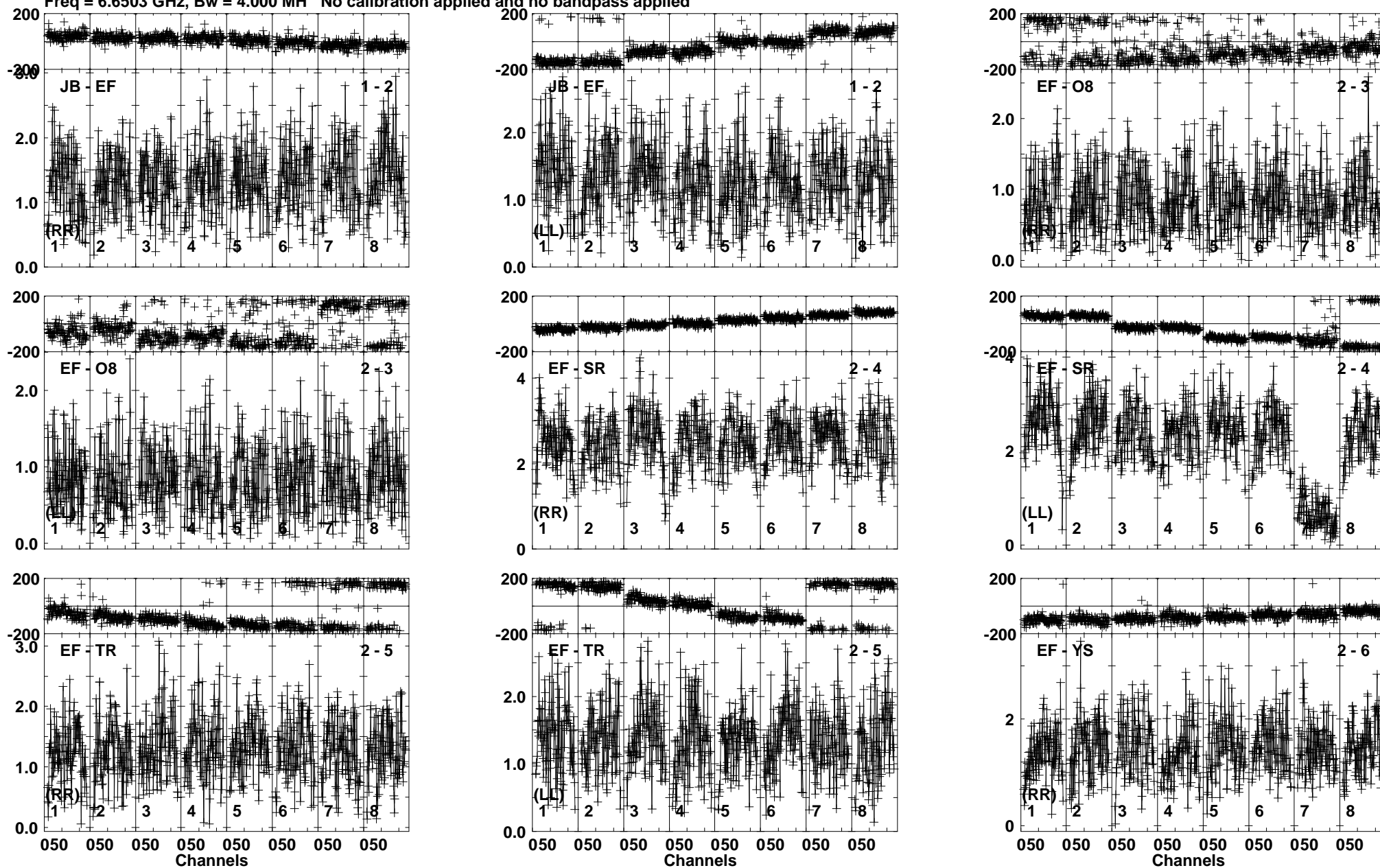
Lower frame: Milli Ampl Jy Top frame: Phas deg Vector averaged cross-power spectrum Baseline: JB (01) - EF (02) Timerange: 00/11:29:51 to 00/11:31:34
