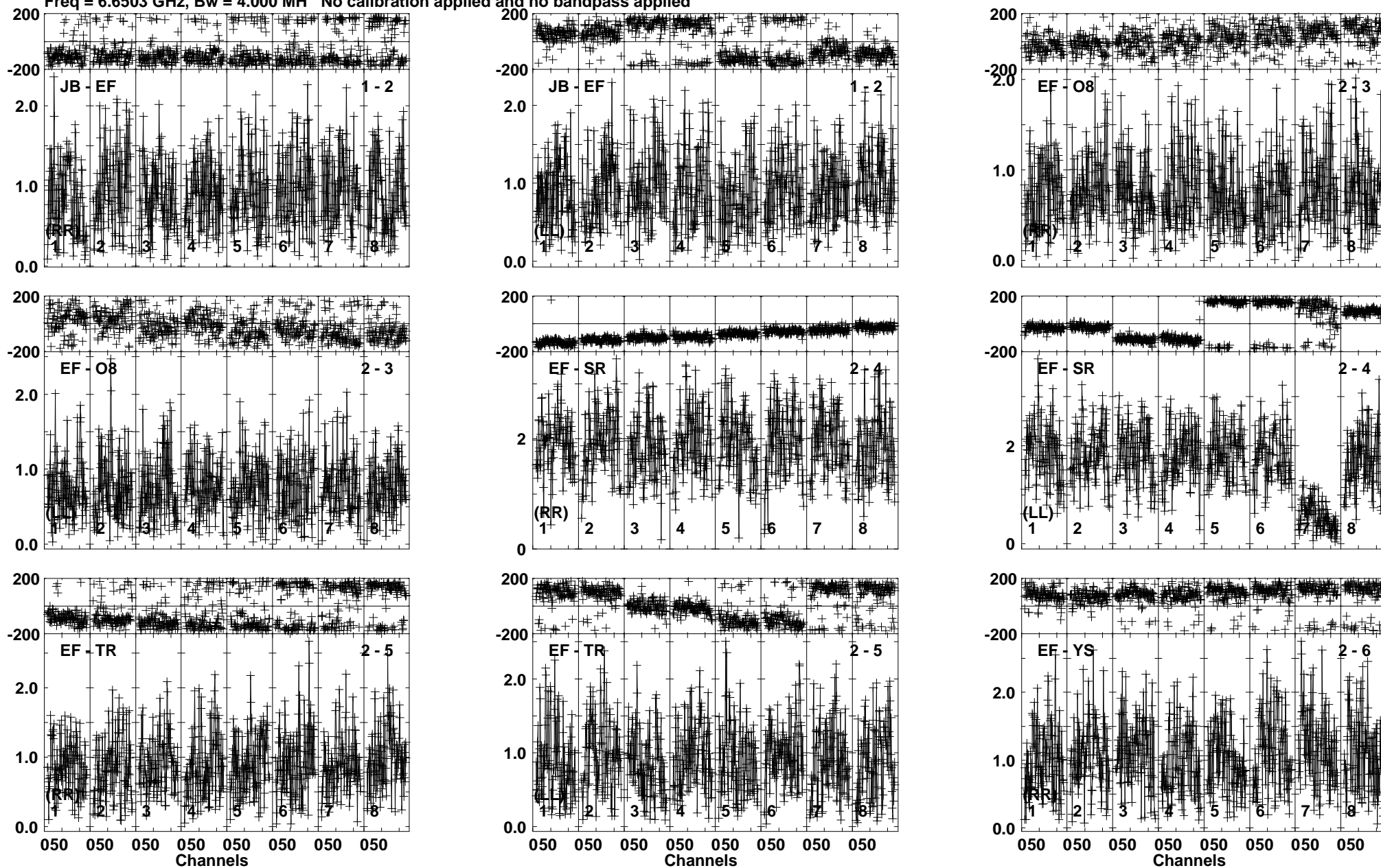
Lower frame: Milli Ampl Jy Top frame: Phas deg Vector averaged cross-power spectrum Baseline: JB (01) - EF (02) Timerange: 00/09:21:11 to 00/09:22:54
