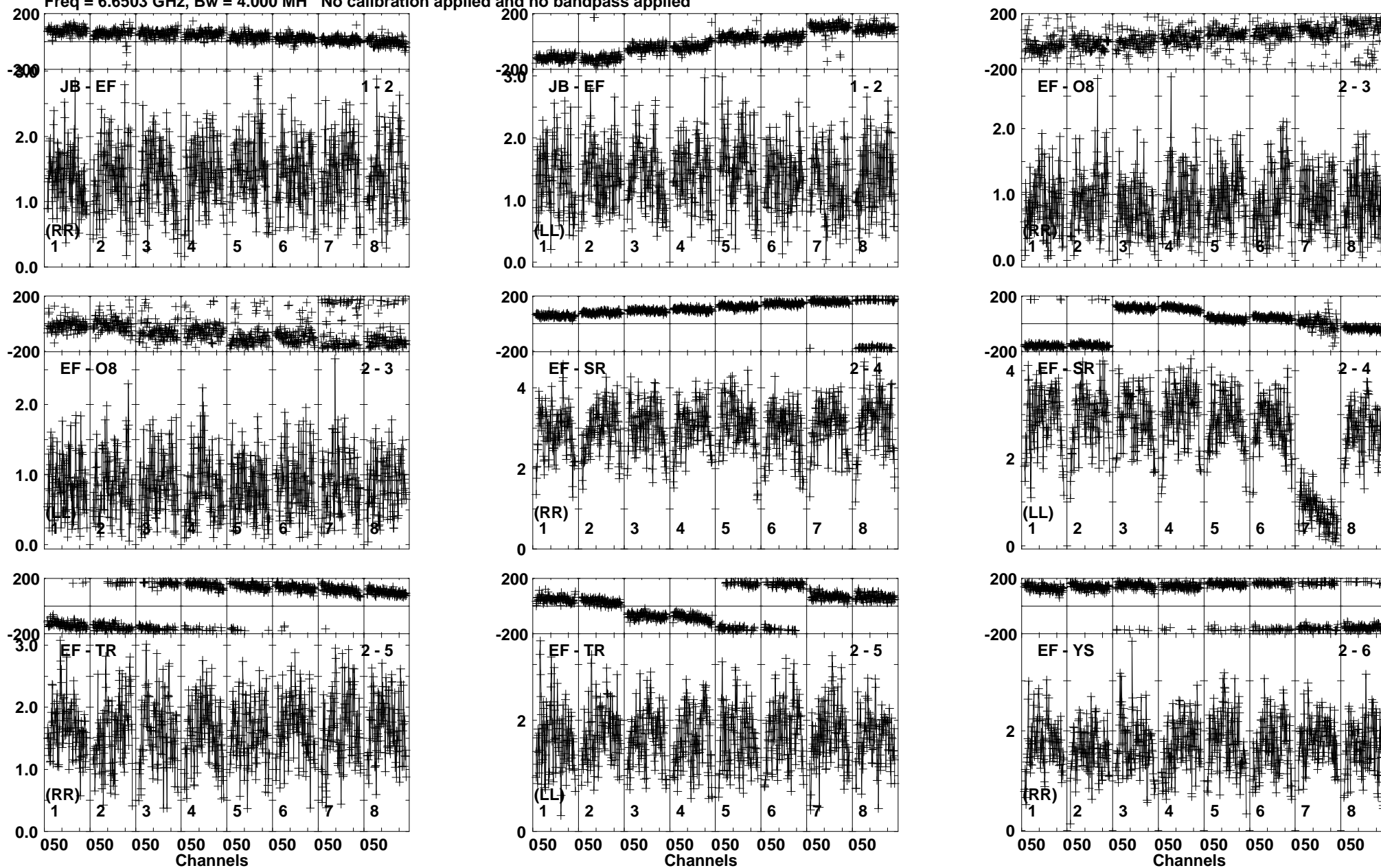
Lower frame: Milli Ampl Jy Top frame: Phas deg Vector averaged cross-power spectrum Baseline: JB (01) - EF (02) Timerange: 00/07:46:25 to 00/07:48:10
