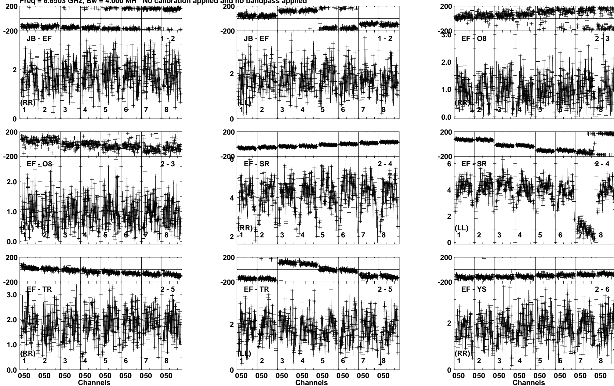
Lower frame: Milli Ampl Jy Top frame: Phas deg Vector averaged cross-power spectrum Baseline: JB (01) - EF (02) Timerange: 00/06:12:05 to 00/06:13:50
