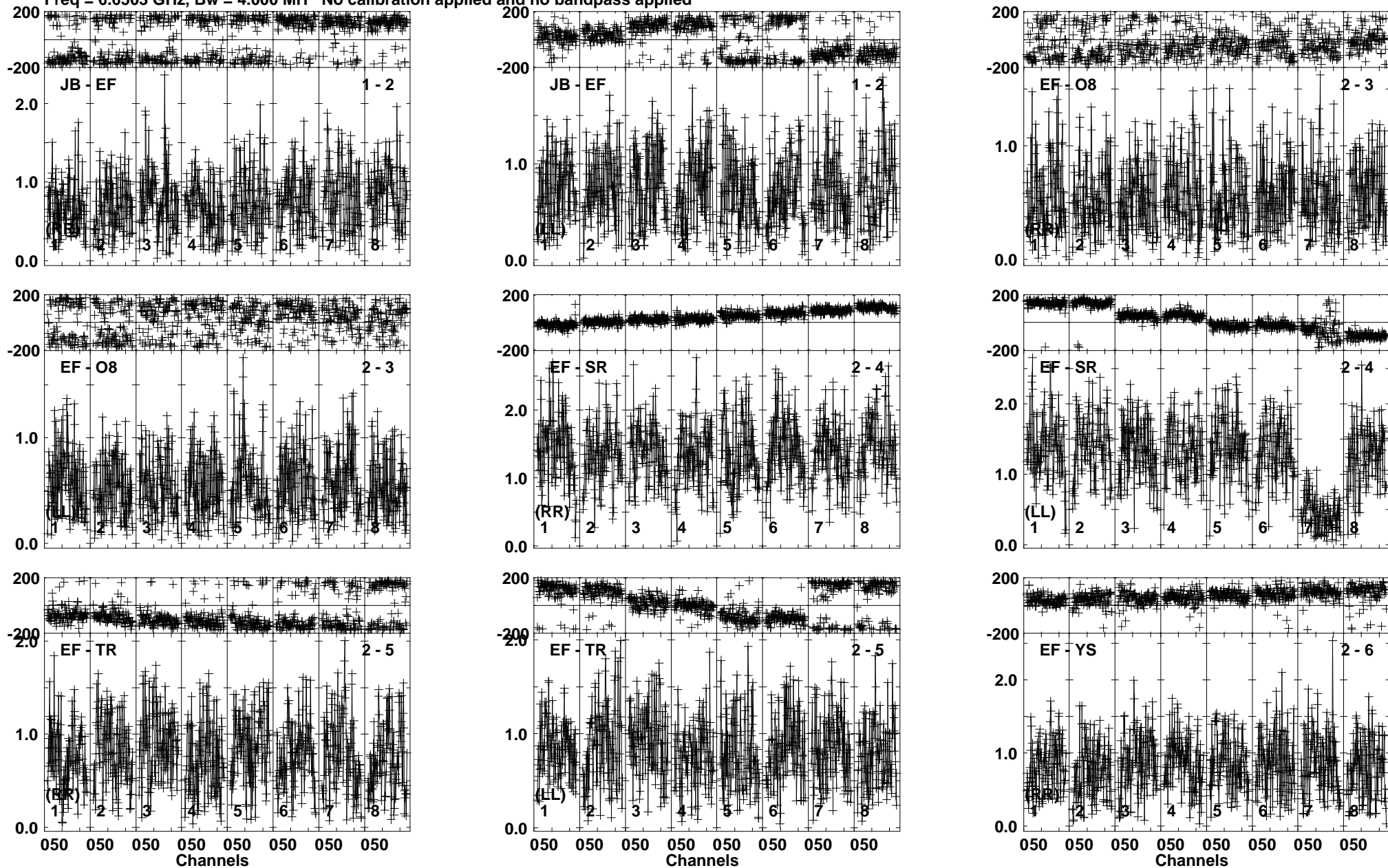
Lower frame: Milli Ampl Jy Top frame: Phas deg Vector averaged cross-power spectrum Baseline: JB (01) - EF (02) Timerange: 00/03:35:25 to 00/03:37:10
