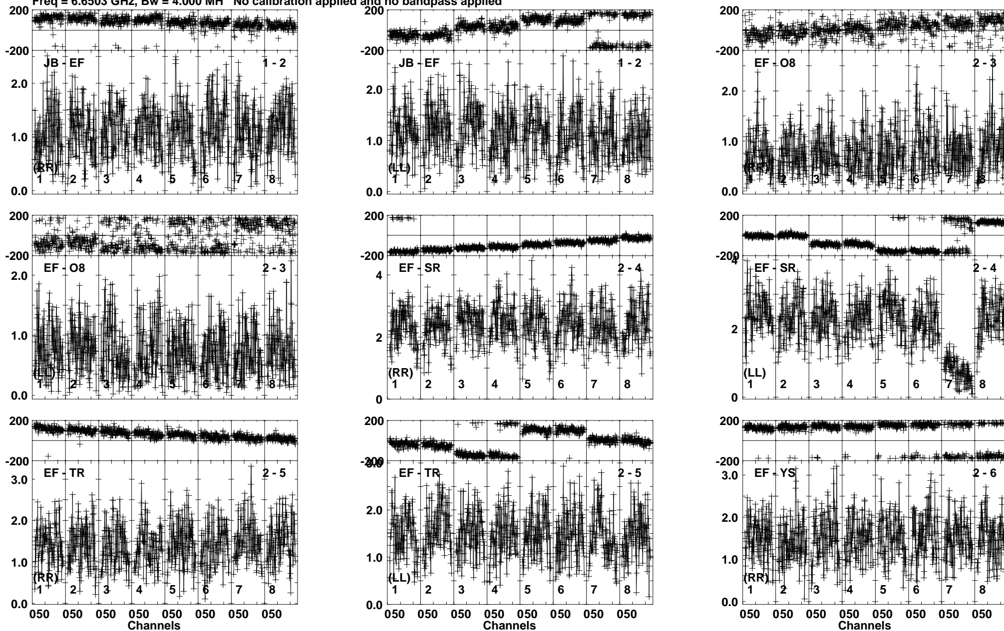
Lower frame: Milli Ampl Jy Top frame: Phas deg Vector averaged cross-power spectrum Baseline: JB (01) - EF (02) Timerange: 00/03:11:51 to 00/03:13:35
