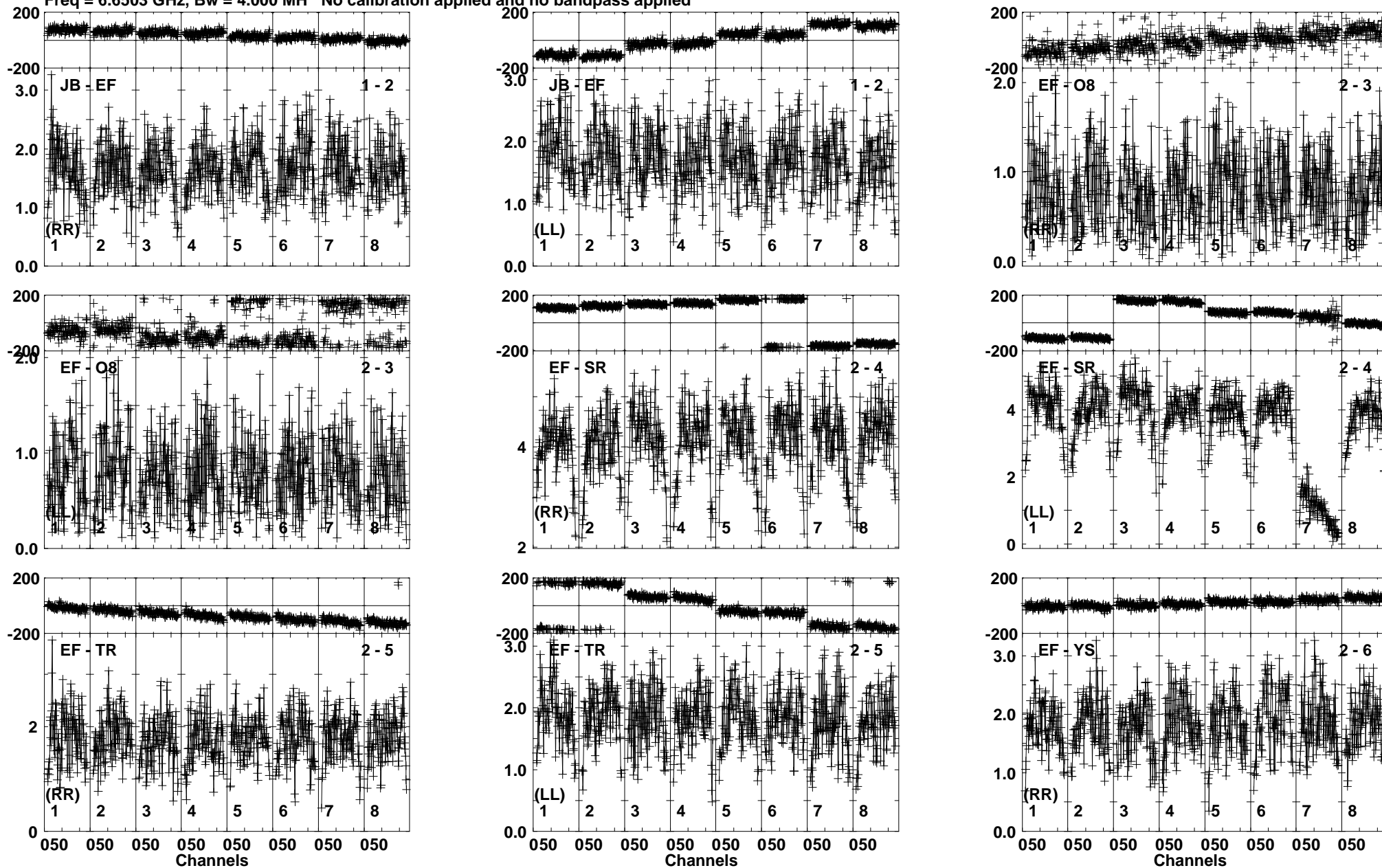
Lower frame: Milli Ampl Jy Top frame: Phas deg Vector averaged cross-power spectrum Baseline: JB (01) - EF (02) Timerange: 00/05:45:46 to 00/05:47:29
