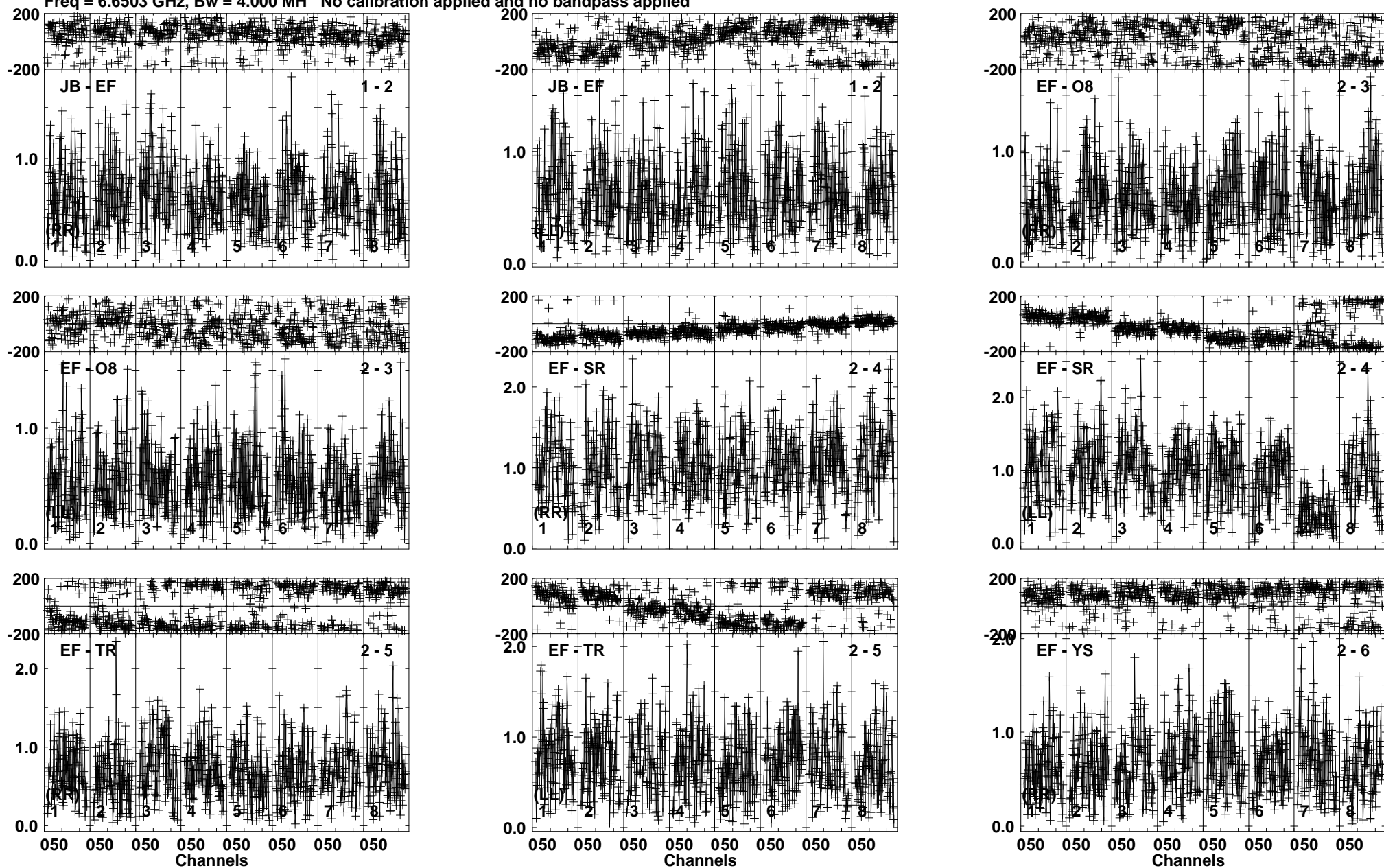
Lower frame: Milli Ampl Jy Top frame: Phas deg Vector averaged cross-power spectrum Baseline: JB (01) - EF (02) Timerange: 00/02:48:51 to 00/02:50:34
