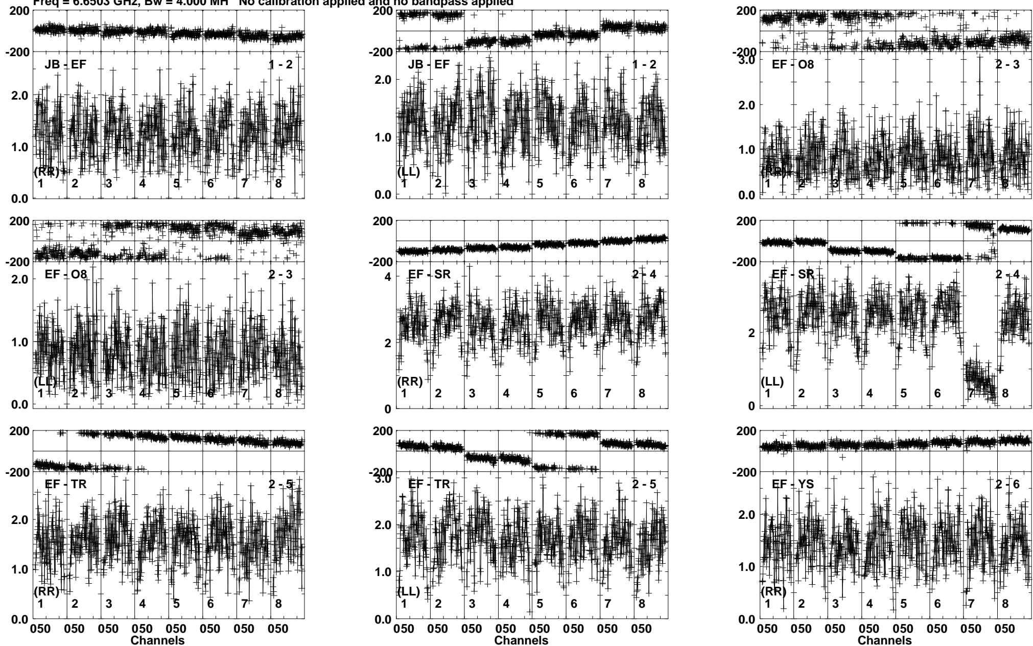
Lower frame: Milli Ampl Jy Top frame: Phas deg Vector averaged cross-power spectrum Baseline: JB (01) - EF (02) Timerange: 00/09:55:30 to 00/09:57:15
