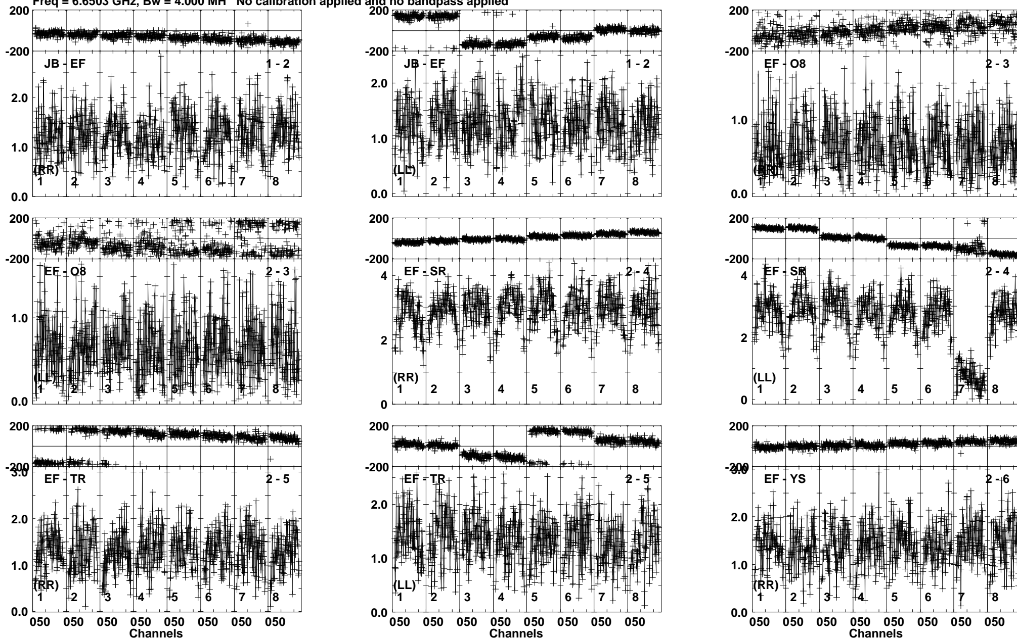
Lower frame: Milli Ampl Jy Top frame: Phas deg Vector averaged cross-power spectrum Baseline: JB (01) - EF (02) Timerange: 00/05:56:25 to 00/05:58:09
