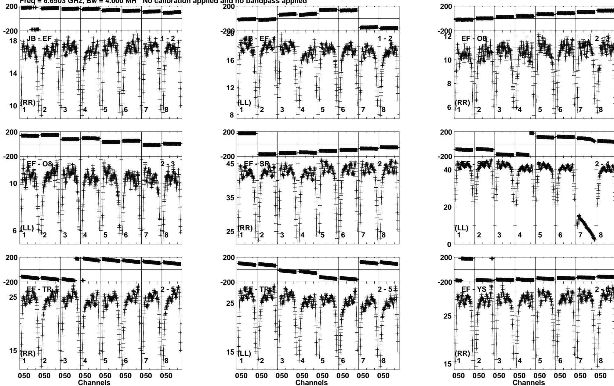
Lower frame: Milli Ampl Jy Top frame: Phas deg Vector averaged cross-power spectrum Baseline: JB (01) - EF (02) Timerange: 00/08:15:06 to 00/08:18:04
