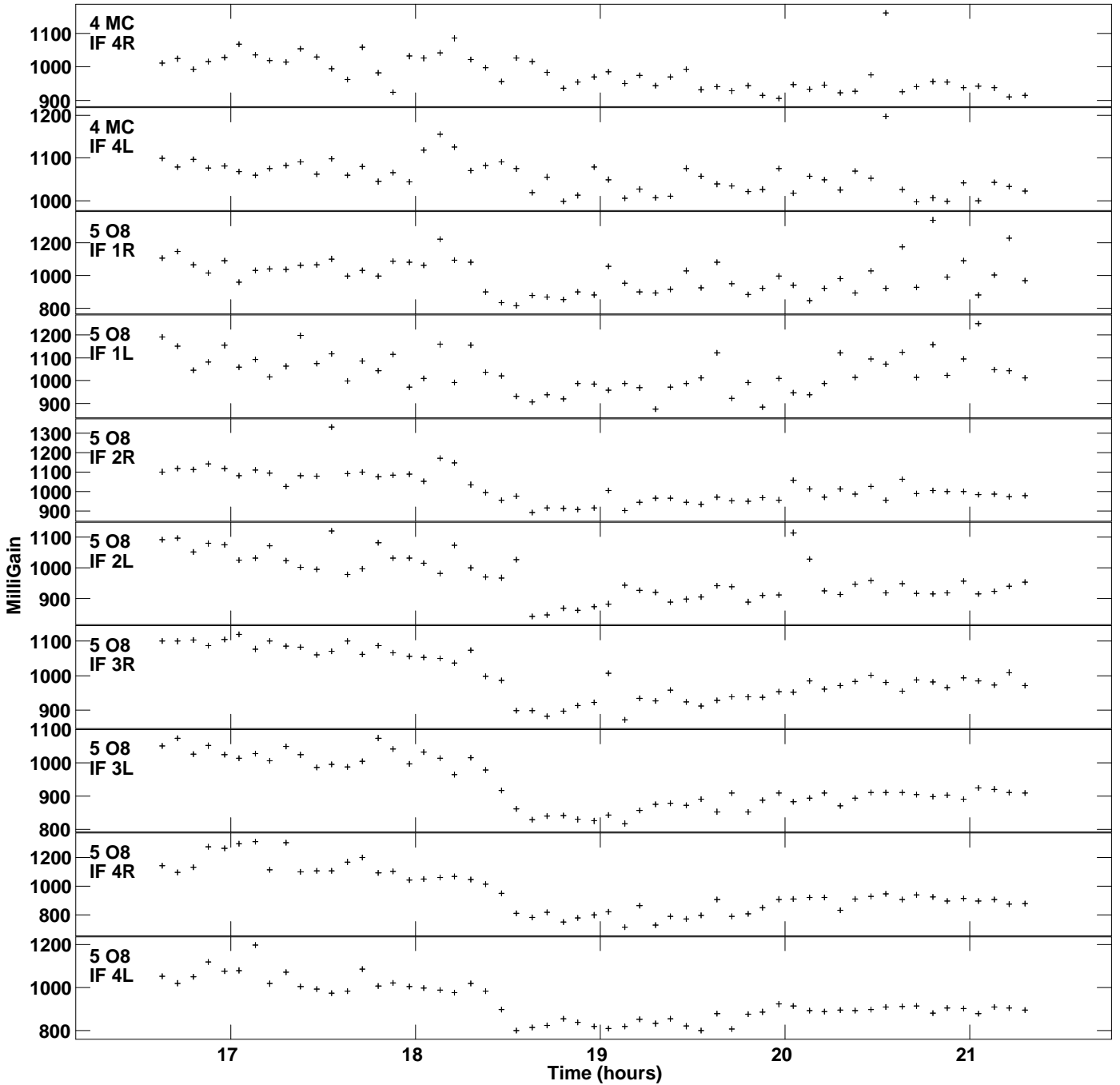
Plot file version 4 created 19-APR-2021 18:29:09 Gain amp vs UTC time for J1028+0255.MULTI.1 SN 2 Rpol & Lpol IF 1 - 4
