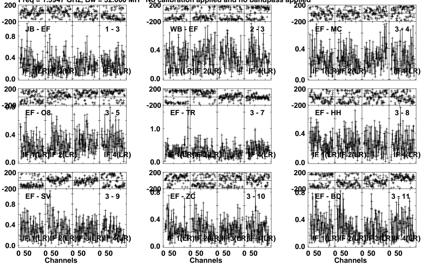
Lower frame: Milli Ampl Jy Top frame: Phas deg Vector averaged cross-power spectrum Several baselines displayed Timerange: 00/19:17:31 to 00/19:18:29
