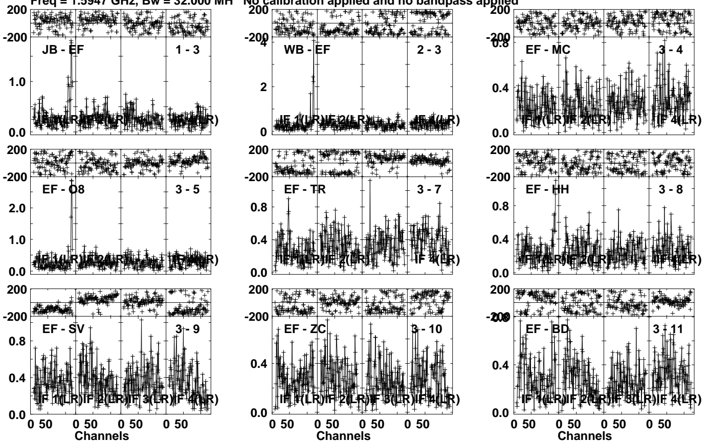
Lower frame: Milli Ampl Jy Top frame: Phas deg Vector averaged cross-power spectrum Several baselines displayed Timerange: 00/19:07:31 to 00/19:08:29
