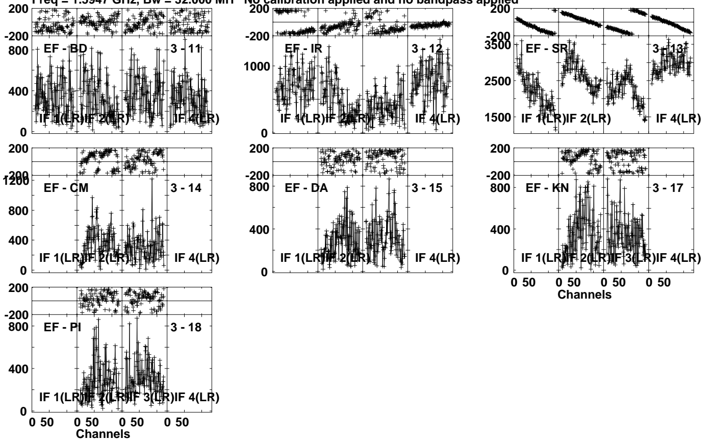
Lower frame: Micro Ampl Jy Top frame: Phas deg Vector averaged cross-power spectrum Several baselines displayed Timerange: 01/05:50:31 to 01/05:51:29
