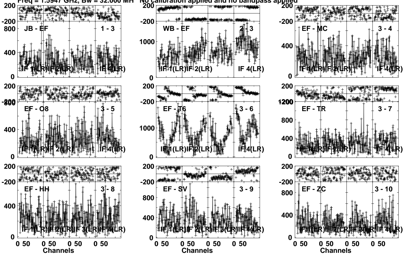
Lower frame: Micro Ampl Jy Top frame: Phas deg Vector averaged cross-power spectrum Several baselines displayed Timerange: 00/17:32:01 to 00/17:33:29
