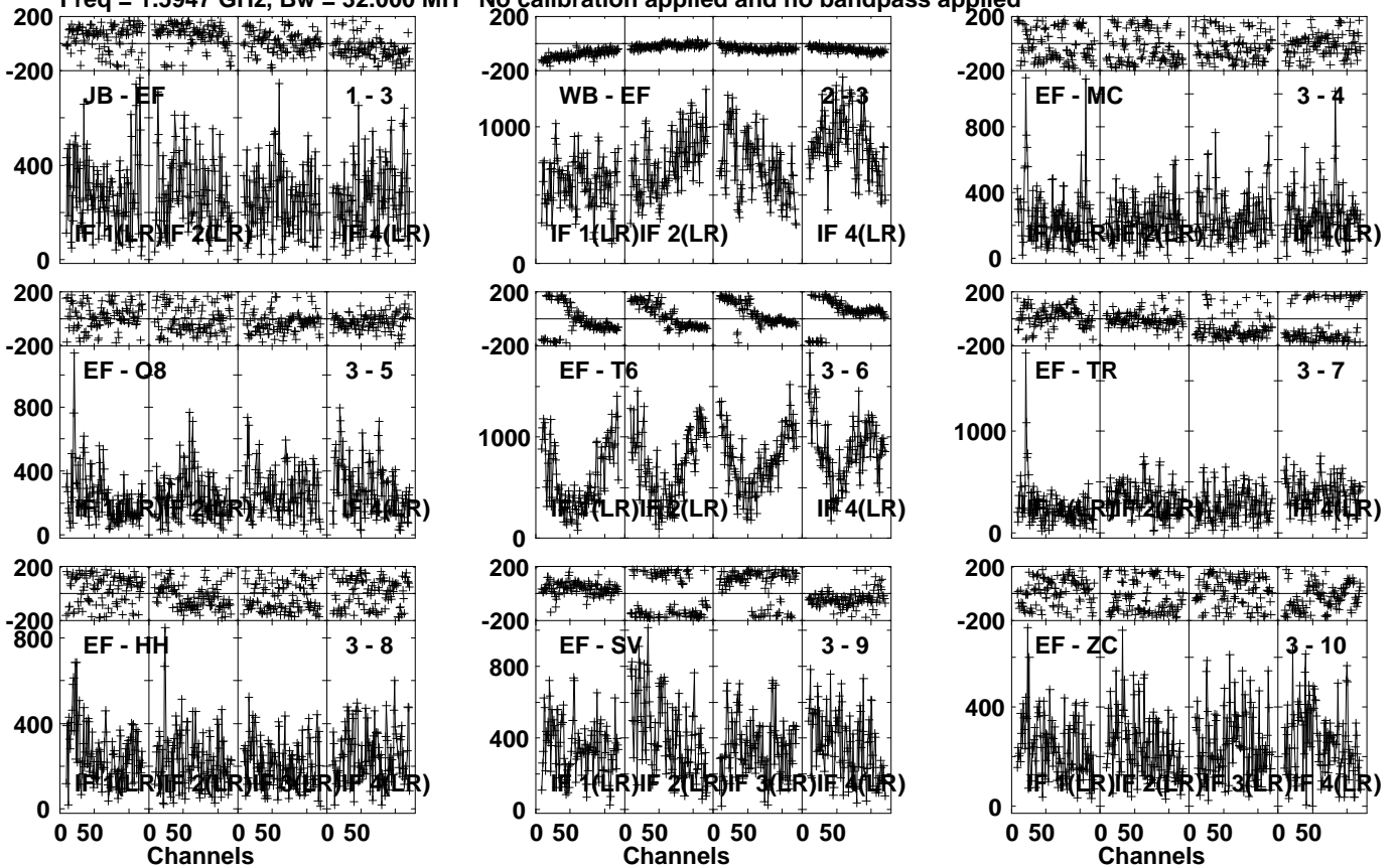
Lower frame: Micro Ampl Jy Top frame: Phas deg Vector averaged cross-power spectrum Several baselines displayed Timerange: 00/18:12:01 to 00/18:13:29
