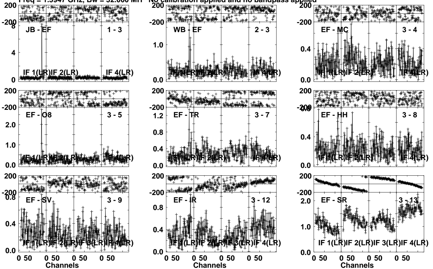
Lower frame: Milli Ampl Jy Top frame: Phas deg Vector averaged cross-power spectrum Several baselines displayed Timerange: 00/20:27:31 to 00/20:28:29
