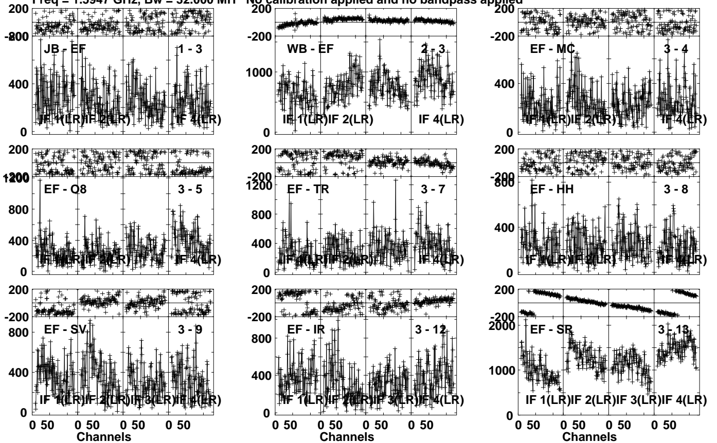
Lower frame: Micro Ampl Jy Top frame: Phas deg Vector averaged cross-power spectrum Several baselines displayed Timerange: 00/19:32:01 to 00/19:33:29
