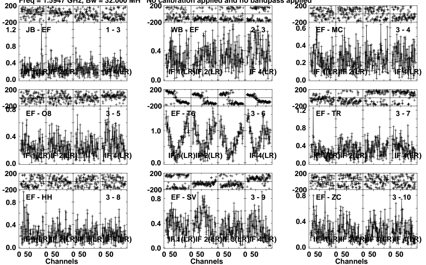
Lower frame: Milli Ampl Jy Top frame: Phas deg Vector averaged cross-power spectrum Several baselines displayed Timerange: 00/17:37:31 to 00/17:38:29
