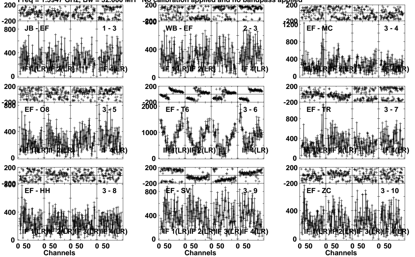
Lower frame: Micro Ampl Jy Top frame: Phas deg Vector averaged cross-power spectrum Several baselines displayed Timerange: 00/17:47:31 to 00/17:48:29
