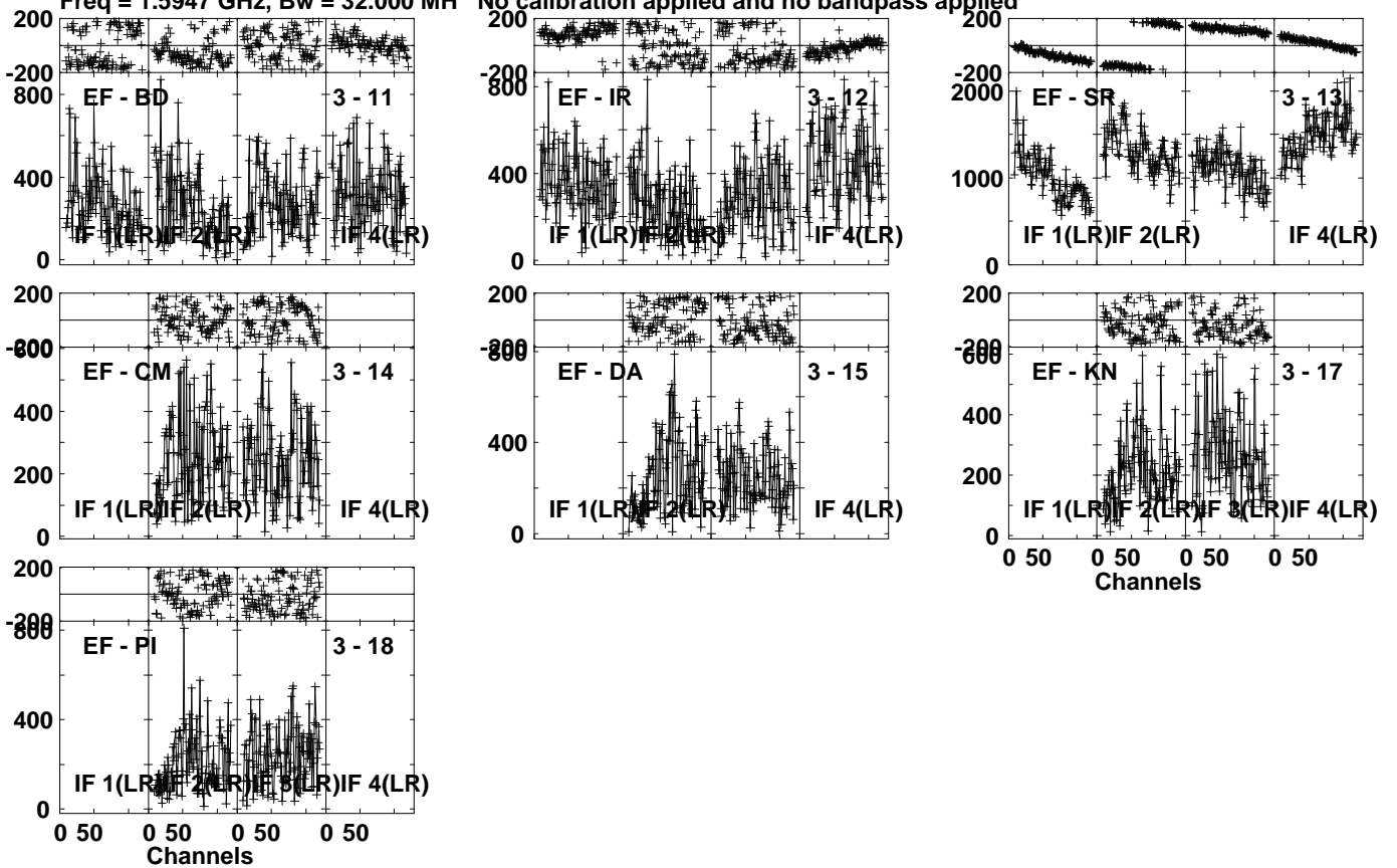
Lower frame: Micro Ampl Jy Top frame: Phas deg Vector averaged cross-power spectrum Several baselines displayed Timerange: 00/17:52:01 to 00/17:53:29
