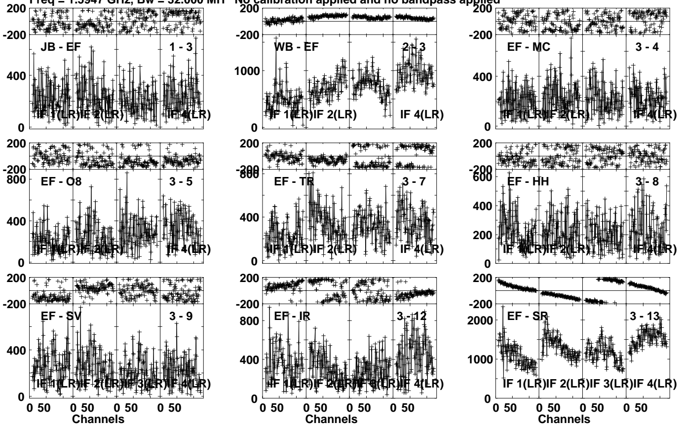
Lower frame: Micro Ampl Jy Top frame: Phas deg Vector averaged cross-power spectrum Several baselines displayed Timerange: 00/20:17:31 to 00/20:18:29
