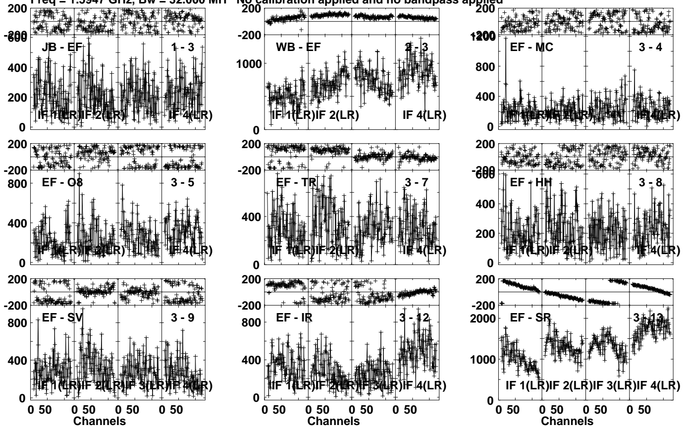
Lower frame: Micro Ampl Jy Top frame: Phas deg Vector averaged cross-power spectrum Several baselines displayed Timerange: 00/20:47:31 to 00/20:48:29
