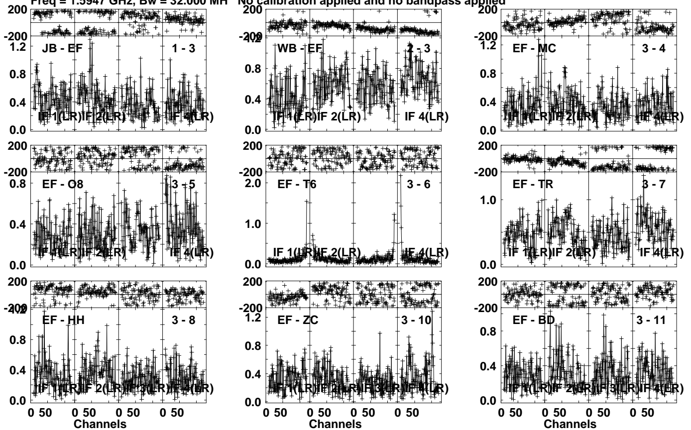
Lower frame: Milli Ampl Jy Top frame: Phas deg Vector averaged cross-power spectrum Several baselines displayed Timerange: 01/07:45:01 to 01/07:46:29
