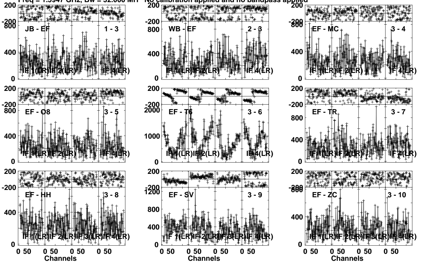
Lower frame: Micro Ampl Jy Top frame: Phas deg Vector averaged cross-power spectrum Several baselines displayed Timerange: 00/17:07:31 to 00/17:08:29
