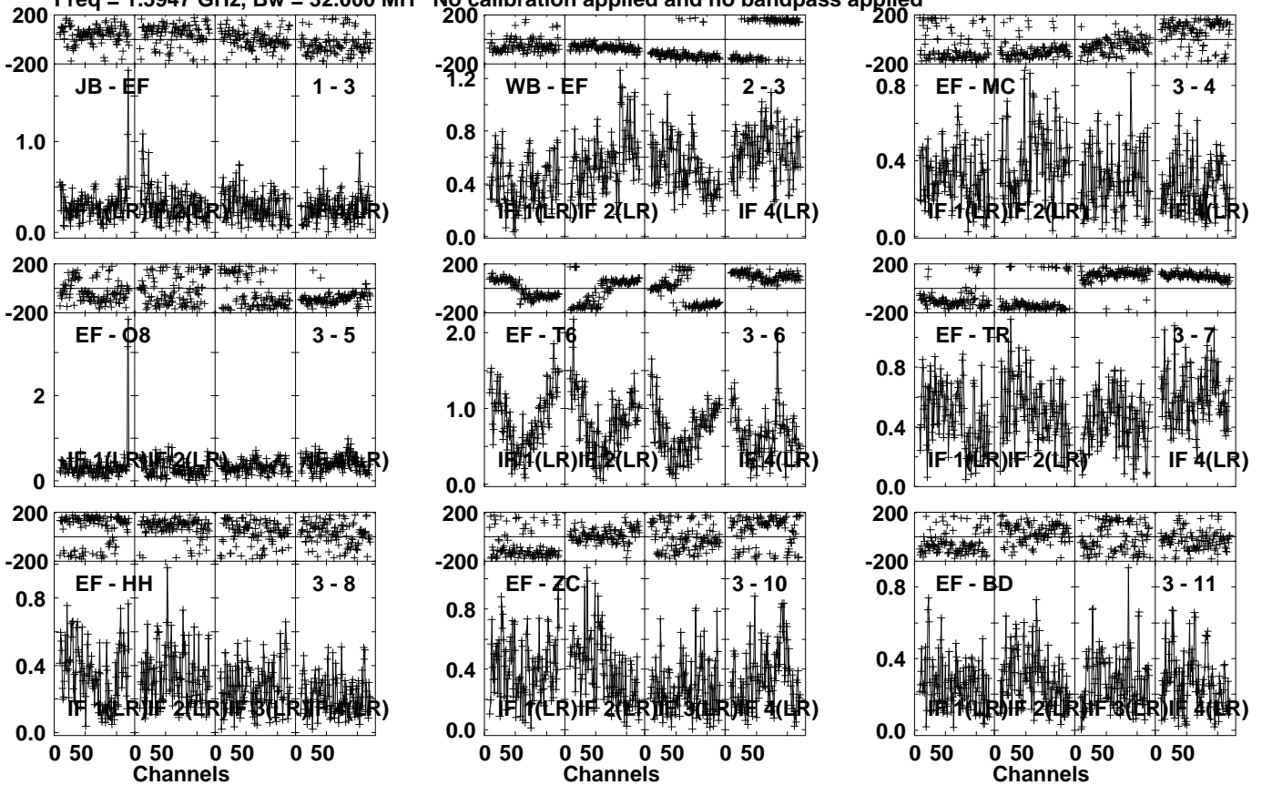
Lower frame: Milli Ampl Jy Top frame: Phas deg Vector averaged cross-power spectrum Several baselines displayed Timerange: 01/08:30:31 to 01/08:31:29
