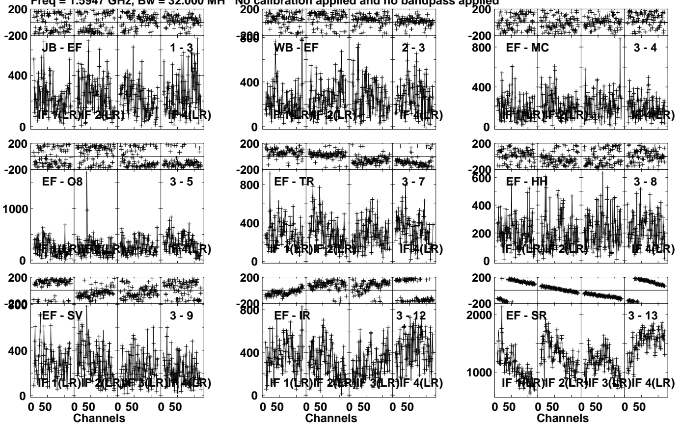
Lower frame: Micro Ampl Jy Top frame: Phas deg Vector averaged cross-power spectrum Several baselines displayed Timerange: 00/20:07:31 to 00/20:08:29
