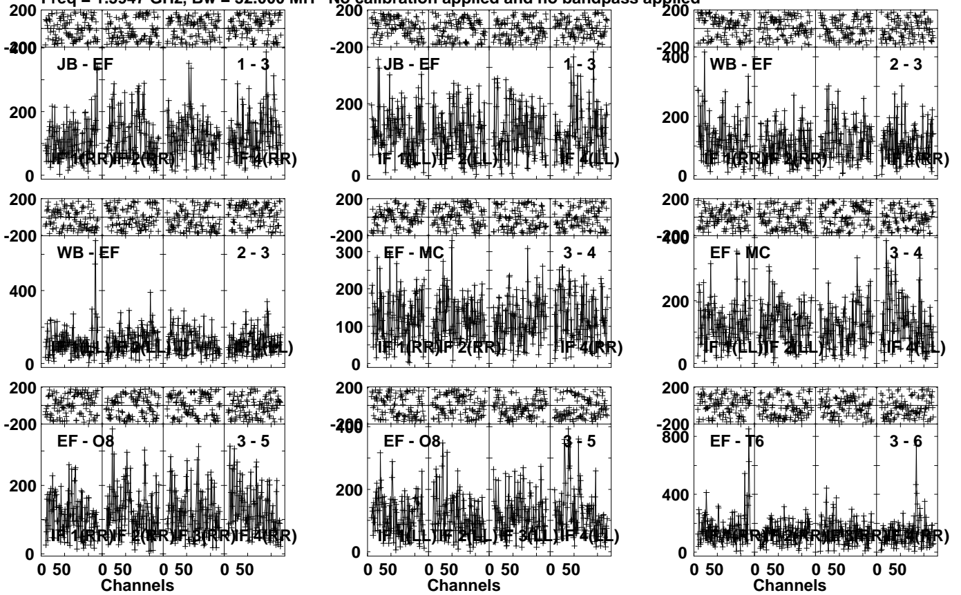
Lower frame: Micro Ampl Jy Top frame: Phas deg Vector averaged cross-power spectrum Several baselines displayed Timerange: 01/05:51:31 to 01/05:54:59
