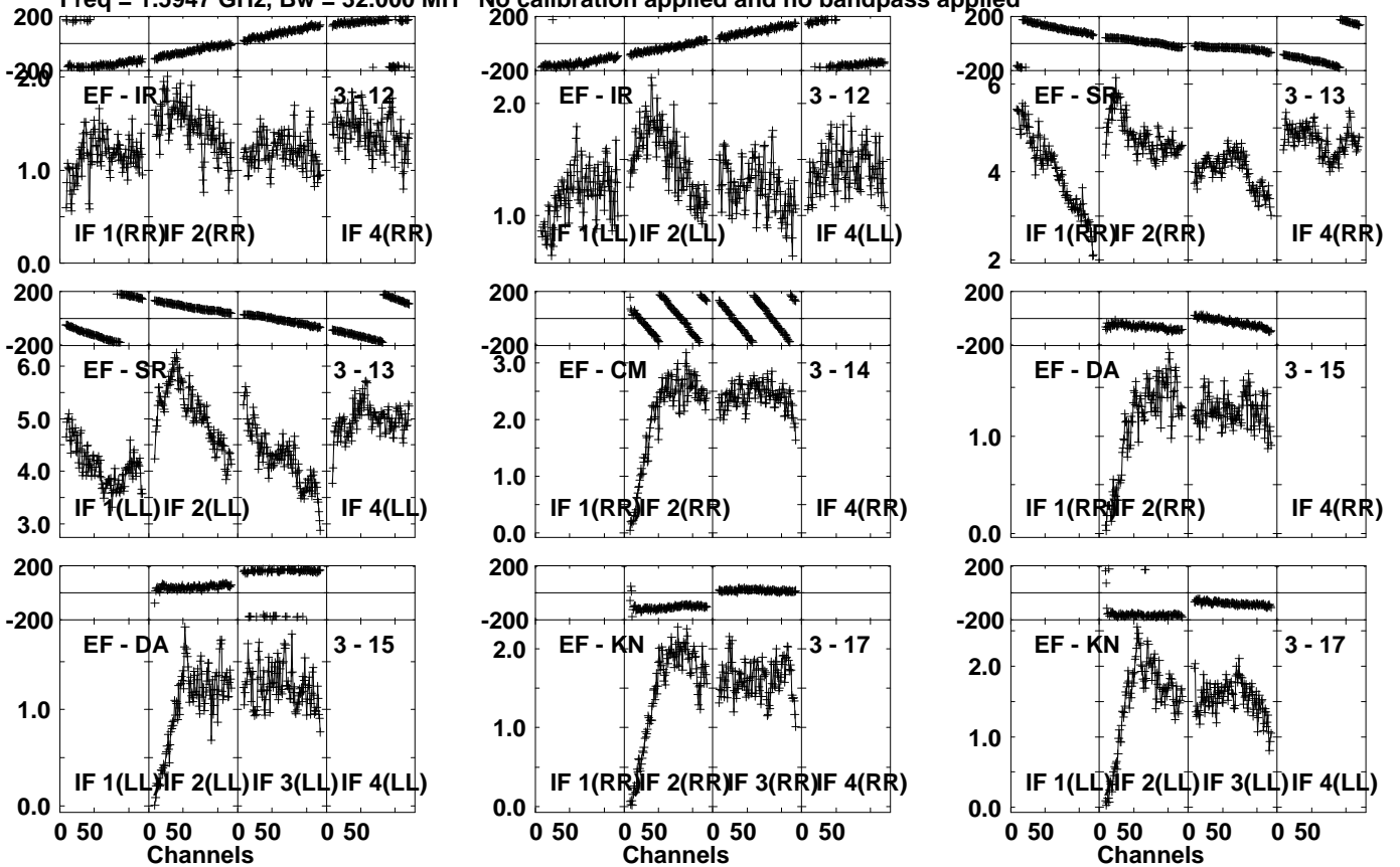
Lower frame: Milli Ampl Jy Top frame: Phas deg Vector averaged cross-power spectrum Several baselines displayed Timerange: 00/19:17:31 to 00/19:18:29
