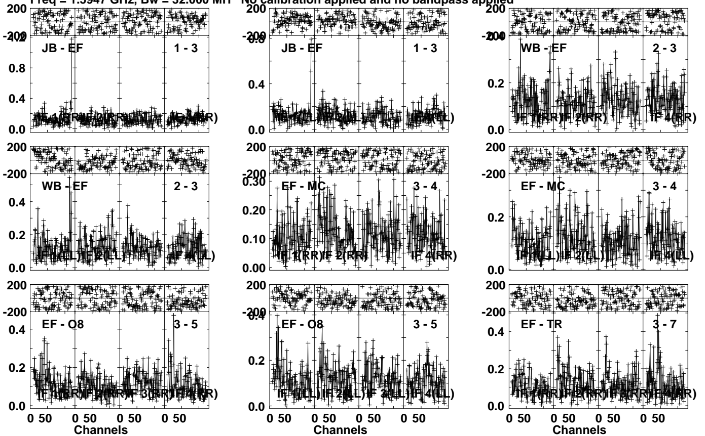
Lower frame: Milli Ampl Jy Top frame: Phas deg Vector averaged cross-power spectrum Several baselines displayed Timerange: 00/19:08:31 to 00/19:11:59
