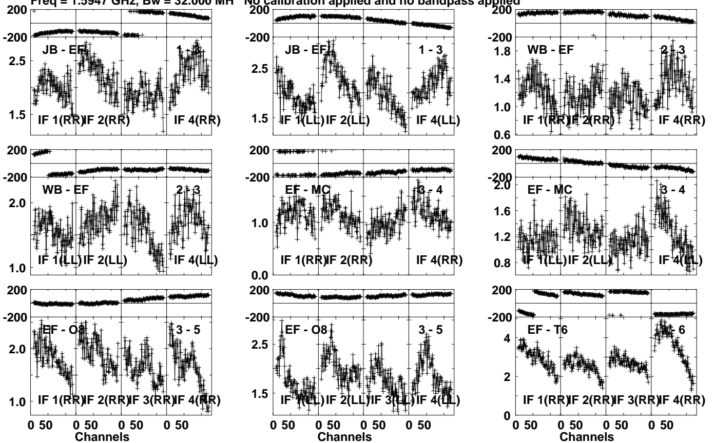
Lower frame: Milli Ampl Jy Top frame: Phas deg Vector averaged cross-power spectrum Several baselines displayed Timerange: 00/17:42:01 to 00/17:43:29
