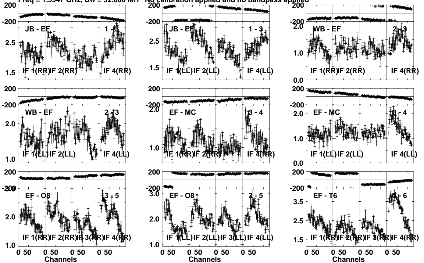
Lower frame: Milli Ampl Jy Top frame: Phas deg Vector averaged cross-power spectrum Several baselines displayed Timerange: 00:18:27:31 to 00:18:28:29
