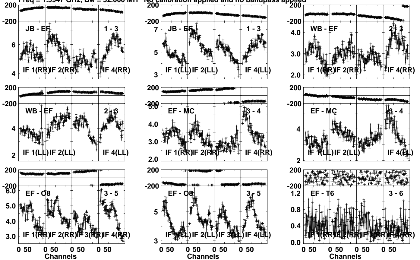
Lower frame: Milli Ampl Jy Top frame: Phas deg Vector averaged cross-power spectrum Several baselines displayed Timerange: 01/07:00:31 to 01/07:01:29
