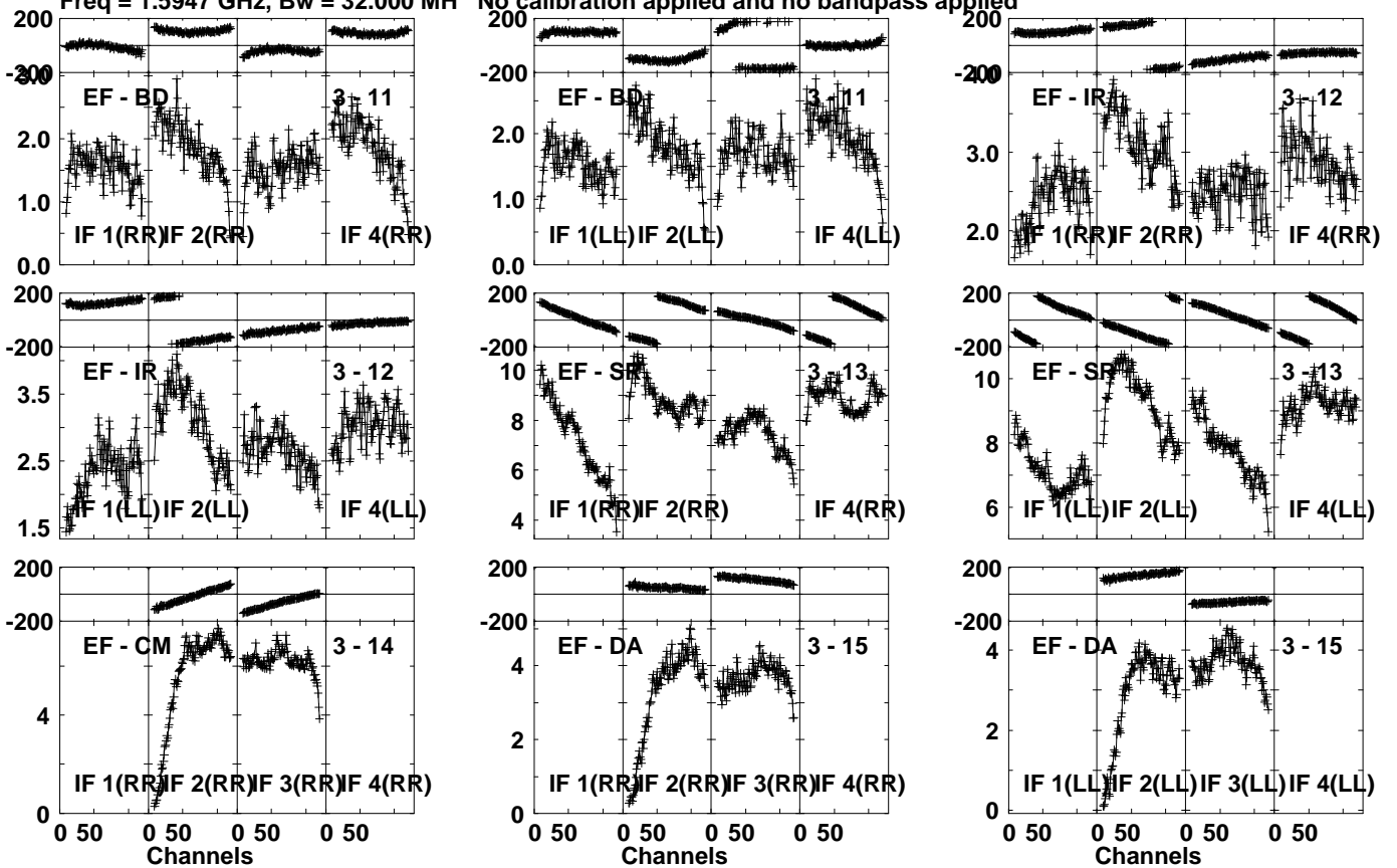
Lower frame: Milli Ampl Jy Top frame: Phas deg Vector averaged cross-power spectrum Several baselines displayed Timerange: 01/05:35:01 to 01/05:36:29
