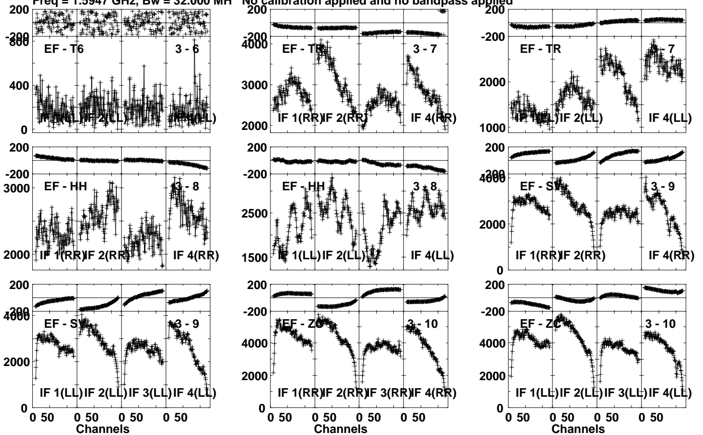
Lower frame: Micro Ampl Jy Top frame: Phas deg Vector averaged cross-power spectrum Several baselines displayed Timerange: 01/04:30:01 to 01/04:31:29
