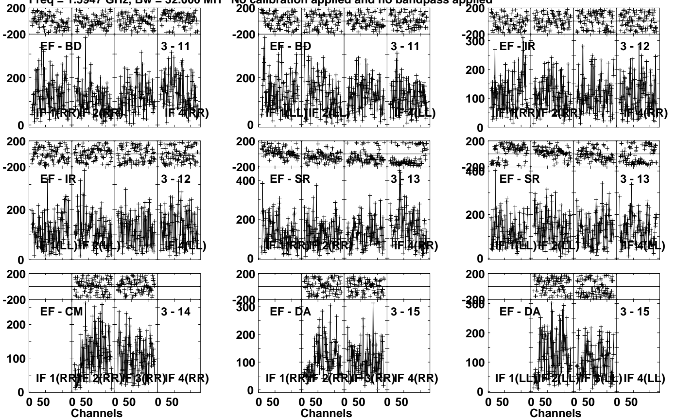
Lower frame: Micro Ampl Jy Top frame: Phas deg Vector averaged cross-power spectrum Several baselines displayed Timerange: 00/17:13:31 to 00/17:16:59
