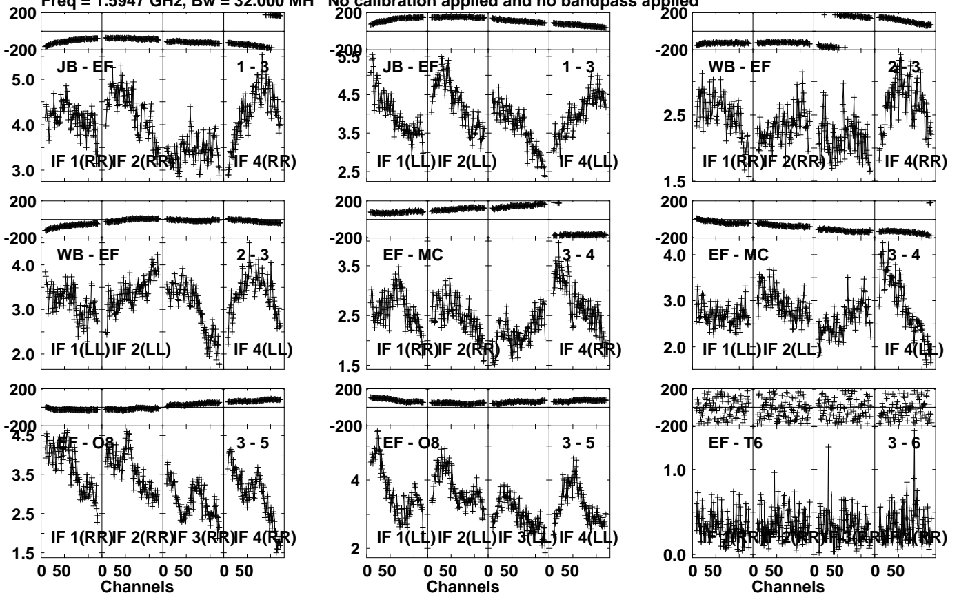
Lower frame: Milli Ampl Jy Top frame: Phas deg Vector averaged cross-power spectrum Several baselines displayed Timerange: 01/04:45:01 to 01/04:46:29
