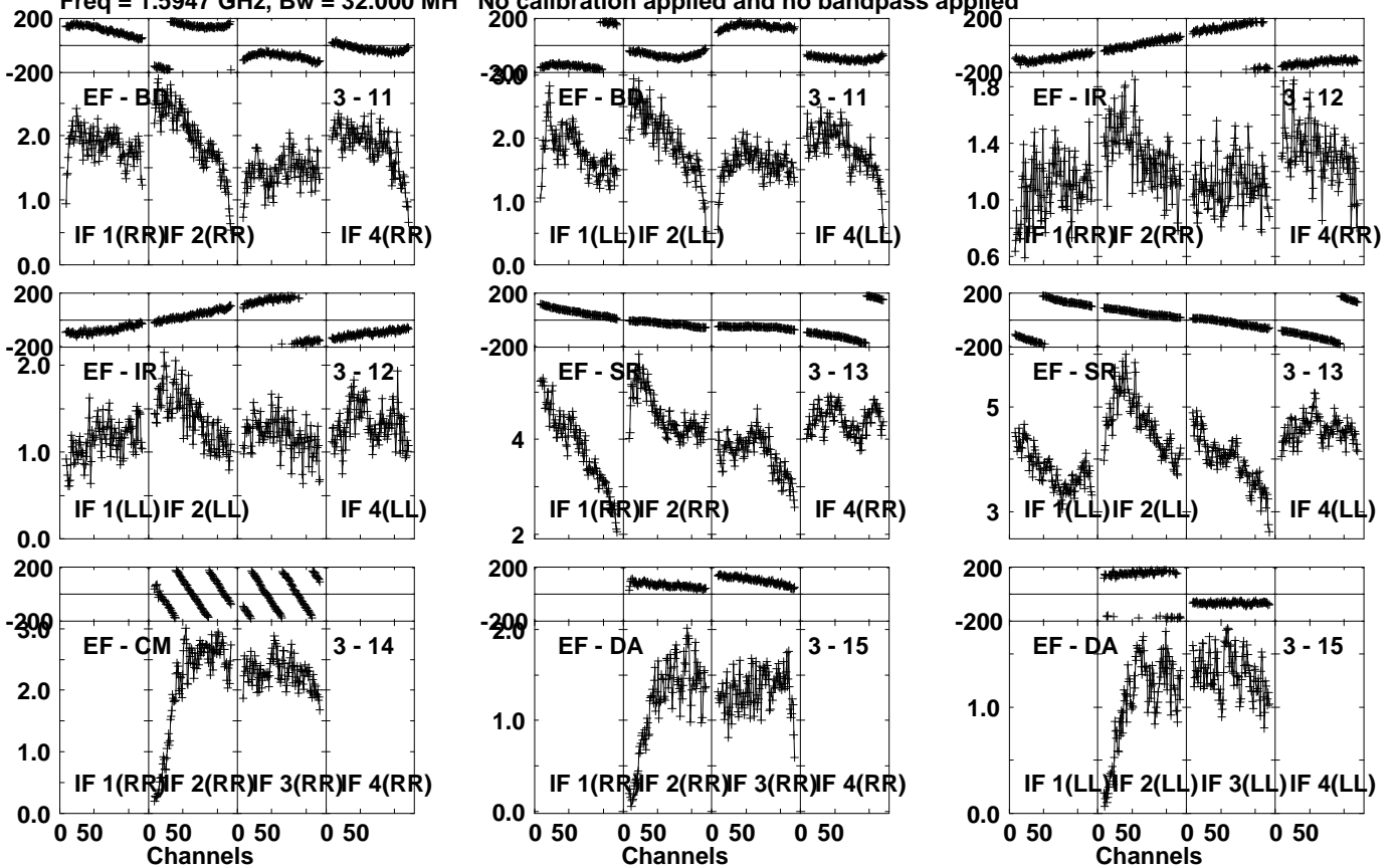
Lower frame: Milli Ampl Jy Top frame: Phas deg Vector averaged cross-power spectrum Several baselines displayed Timerange: 00/17:32:01 to 00/17:33:29
