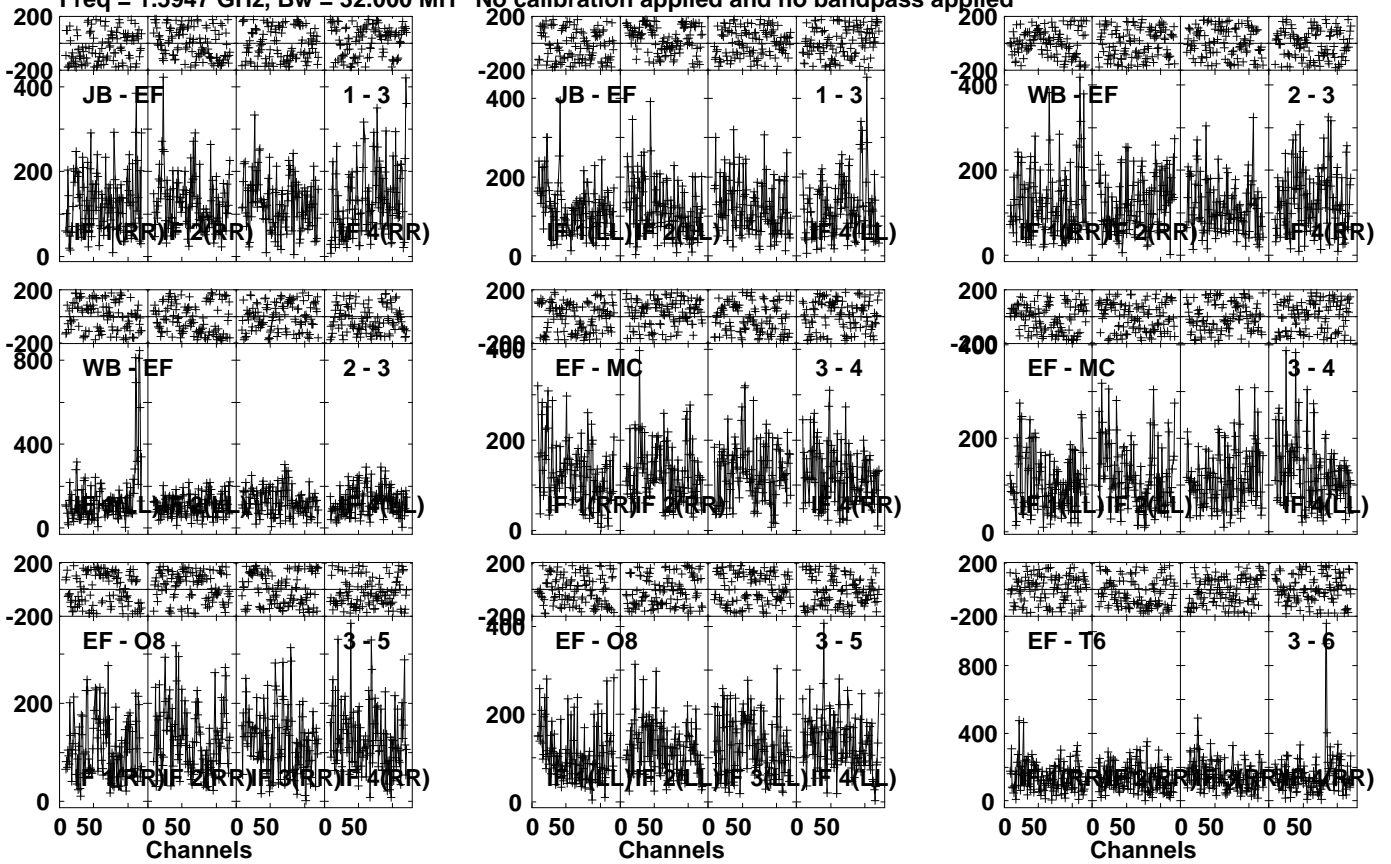
Lower frame: Micro Ampl Jy Top frame: Phas deg Vector averaged cross-power spectrum Several baselines displayed Timerange: 01/06:26:31 to 01/06:29:59
