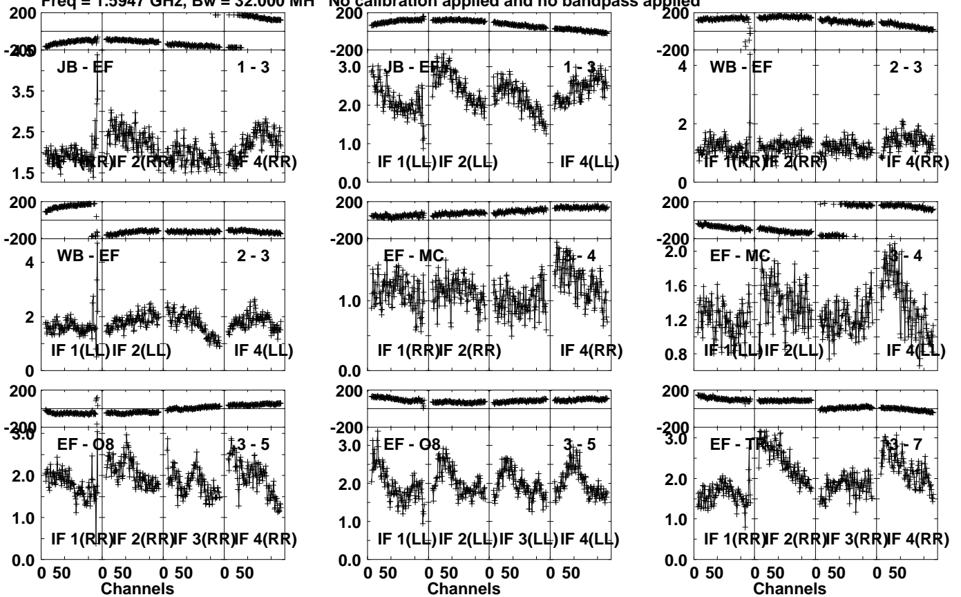
Lower frame: Milli Ampl Jy Top frame: Phas deg Vector averaged cross-power spectrum Several baselines displayed Timerange: 00/19:07:31 to 00/19:08:29
