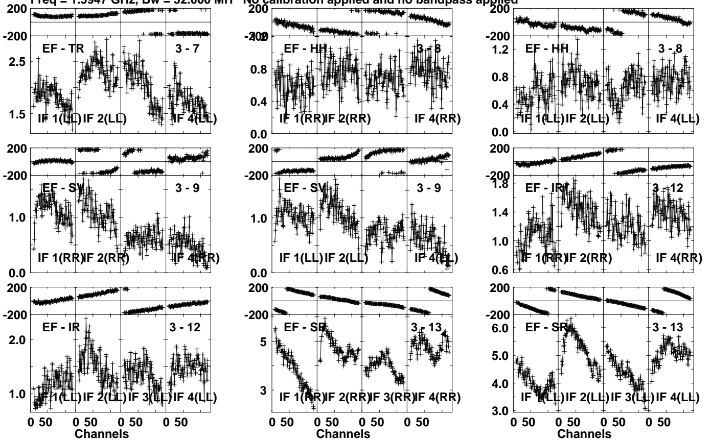
Lower frame: Milli Ampl Jy Top frame: Phas deg Vector averaged cross-power spectrum Several baselines displayed Timerange: 00/20:37:31 to 00/20:38:29
