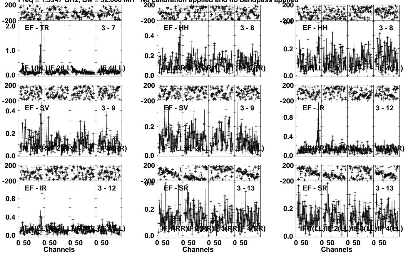
Lower frame: Milli Ampl Jy Top frame: Phas deg Vector averaged cross-power spectrum Several baselines displayed Timerange: 00/21:03:31 to 00/21:06:59
