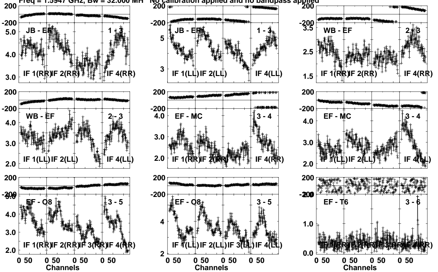
Lower frame: Milli Ampl Jy Top frame: Phas deg Vector averaged cross-power spectrum Several baselines displayed Timerange: 01/04:55:01 to 01/04:56:29
