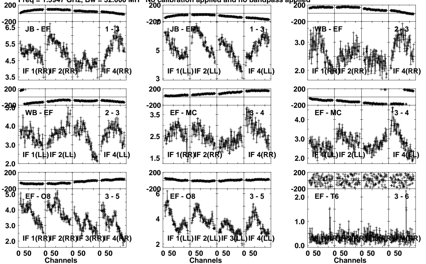
Lower frame: Milli Ampl Jy Top frame: Phas deg Vector averaged cross-power spectrum Several baselines displayed Timerange: 01/05:20:31 to 01/05:21:29
