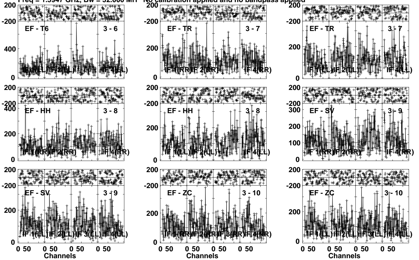
Lower frame: Micro Ampl Jy Top frame: Phas deg Vector averaged cross-power spectrum Several baselines displayed Timerange: 00/17:28:31 to 00/17:31:59
