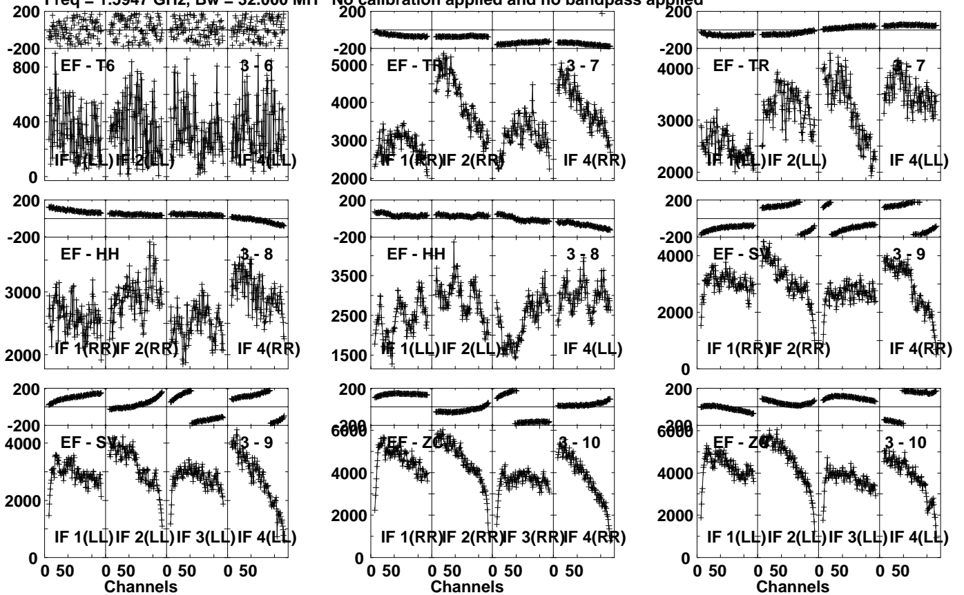
Lower frame: Micro Ampl Jy Top frame: Phas deg Vector averaged cross-power spectrum Several baselines displayed Timerange: 01/04:45:01 to 01/04:46:29
