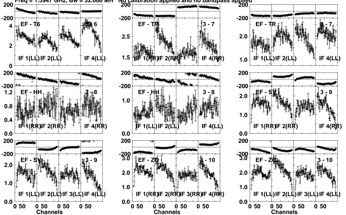
Lower frame: Milli Ampl Jy Top frame: Phas deg Vector averaged cross-power spectrum Several baselines displayed Timerange: 00/17:47:31 to 00/17:48:29
