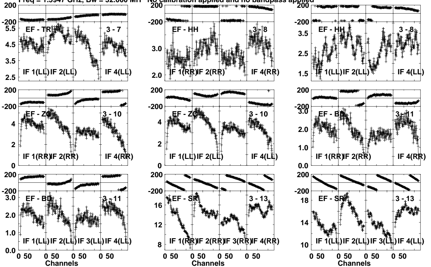
Lower frame: Milli Ampl Jy Top frame: Phas deg Vector averaged cross-power spectrum Several baselines displayed Timerange: 01/09:20:31 to 01/09:21:29
