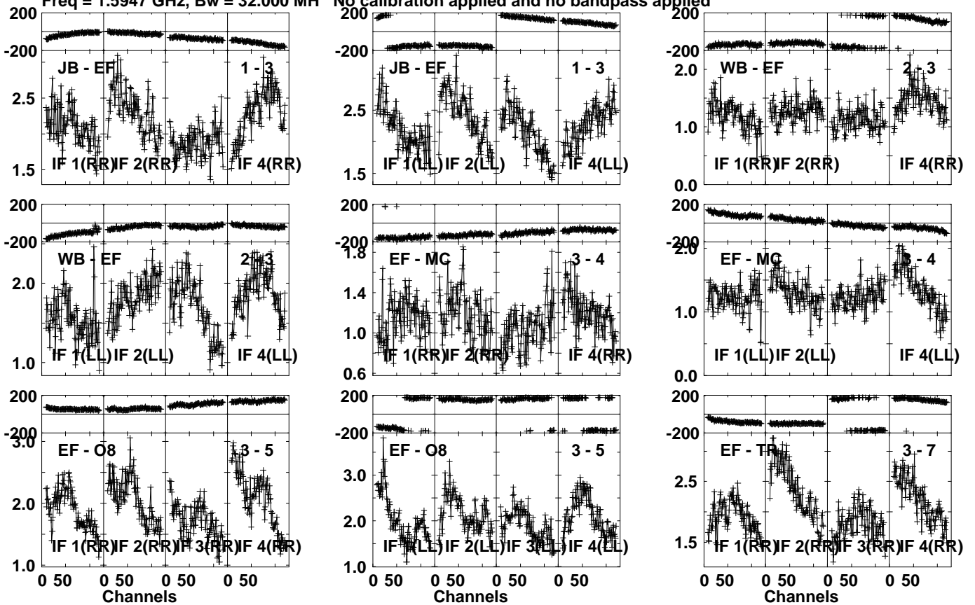
Lower frame: Milli Ampl Jy Top frame: Phas deg Vector averaged cross-power spectrum Several baselines displayed Timerange: 00:18:37:31 to 00:18:38:29
