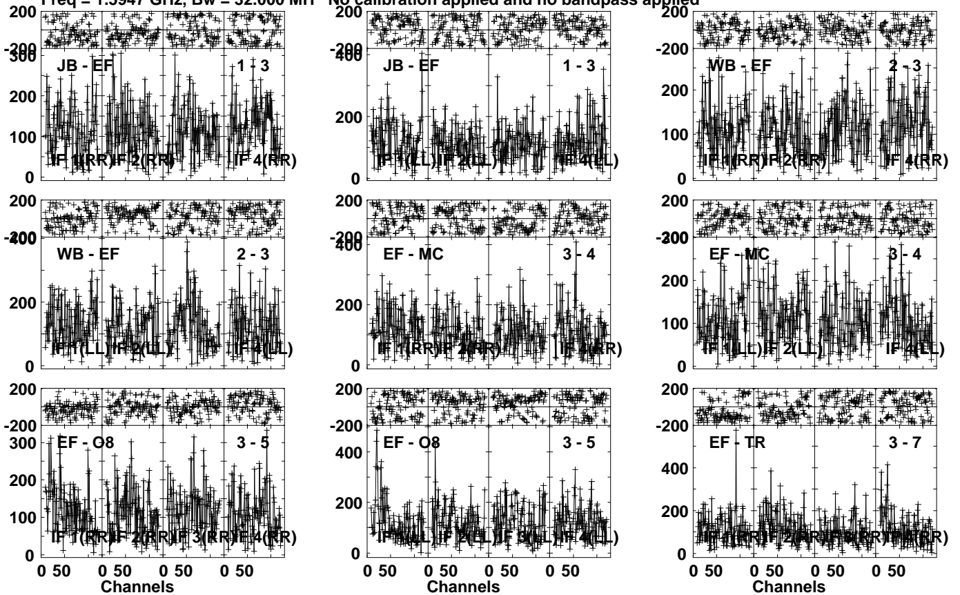
Lower frame: Micro Ampl Jy Top frame: Phas deg Vector averaged cross-power spectrum Several baselines displayed Timerange: 00/19:38:31 to 00/19:41:59
