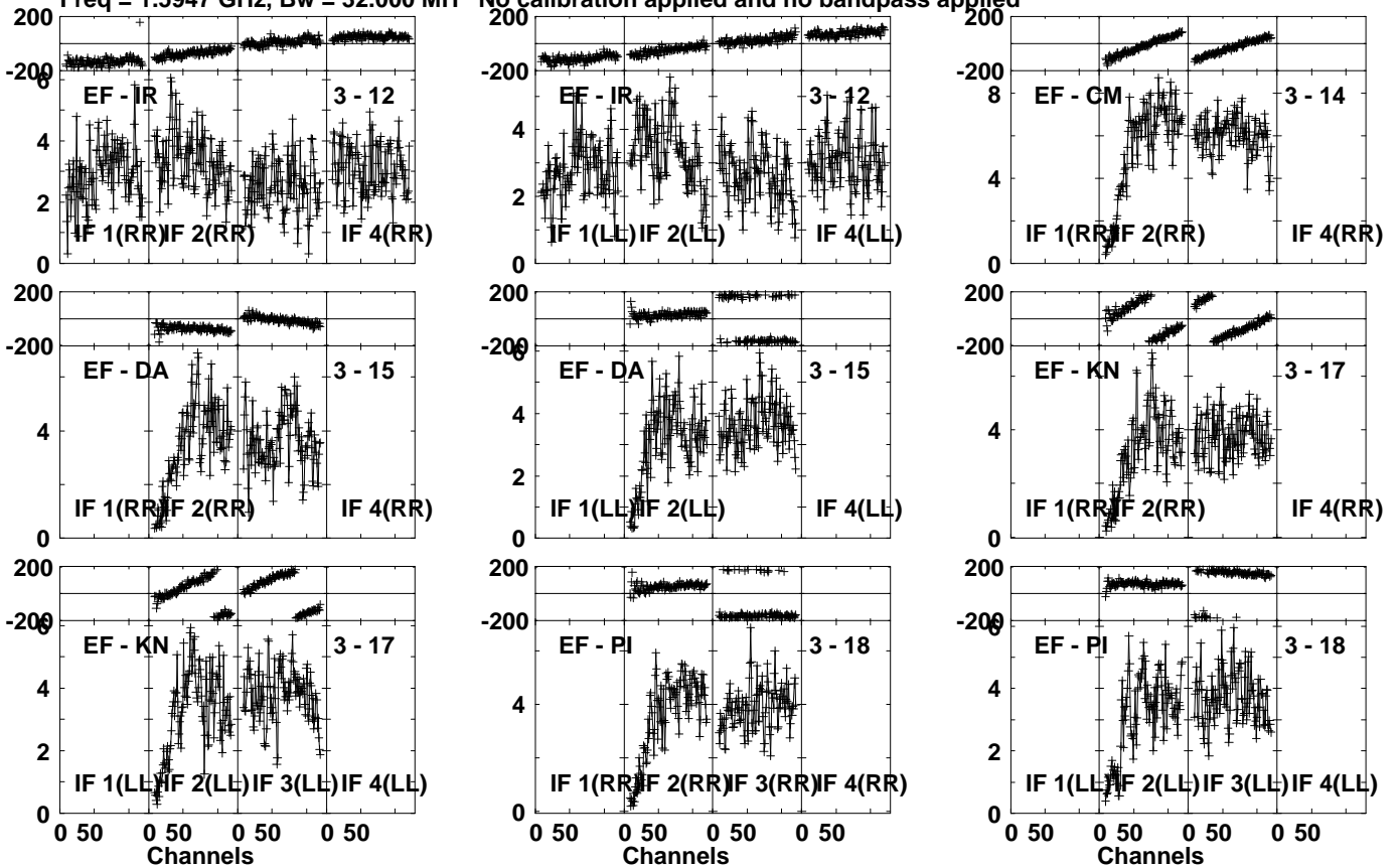
Lower frame: Milli Ampl Jy Top frame: Phas deg Vector averaged cross-power spectrum Several baselines displayed Timerange: 01/06:45:01 to 01/06:46:29
