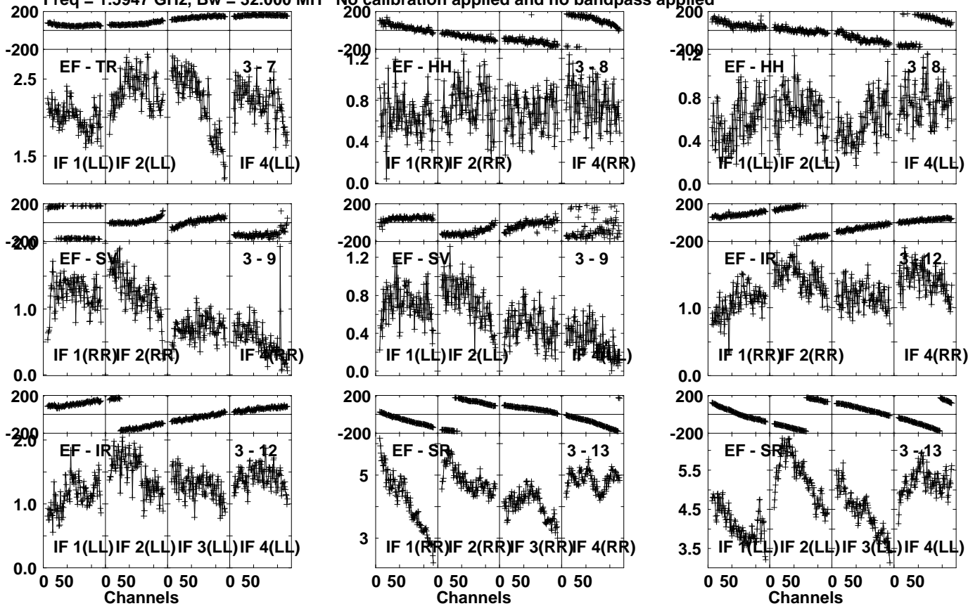
Lower frame: Milli Ampl Jy Top frame: Phas deg Vector averaged cross-power spectrum Several baselines displayed Timerange: 00/21:07:31 to 00/21:08:29
