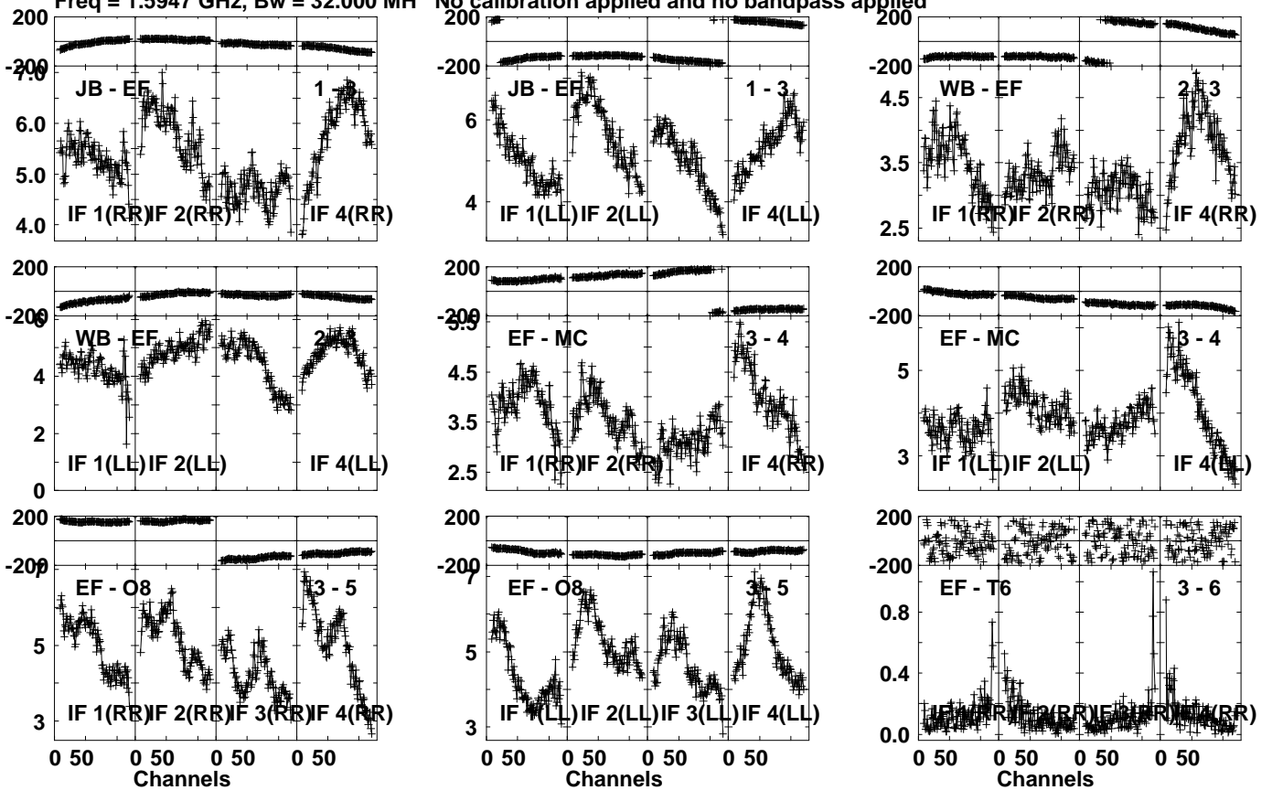
Lower frame: Milli Ampl Jy Top frame: Phas deg Vector averaged cross-power spectrum Several baselines displayed Timerange: 01/07:45:01 to 01/07:46:29
