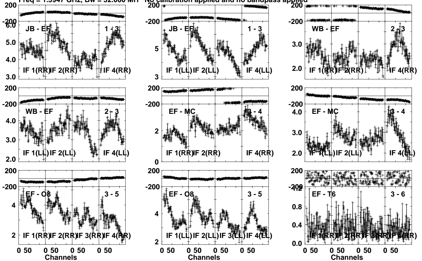
Lower frame: Milli Ampl Jy Top frame: Phas deg Vector averaged cross-power spectrum Several baselines displayed Timerange: 01/05:10:31 to 01/05:11:29
