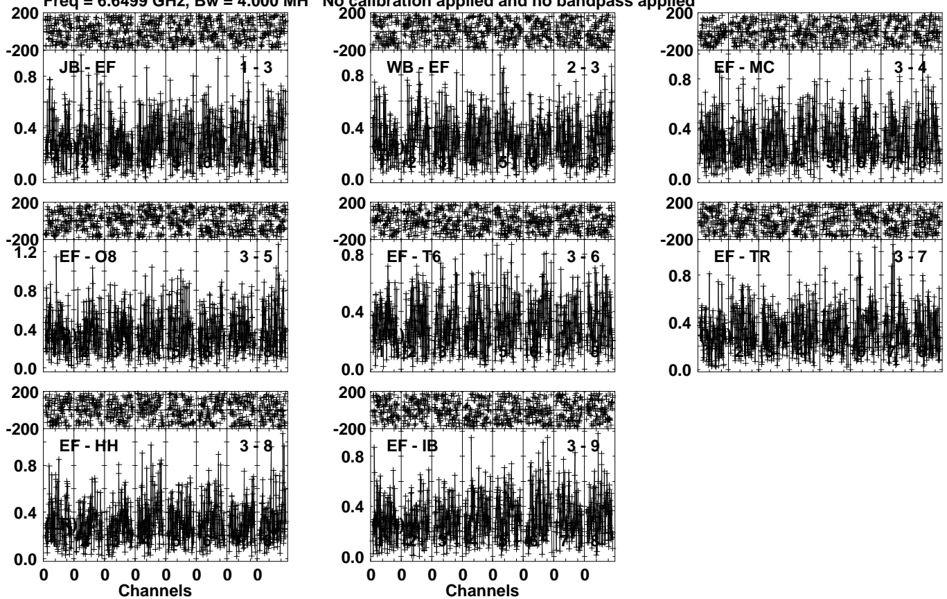
Lower frame: Milli Ampl Jy Top frame: Phas deg Vector averaged cross-power spectrum Several baselines displayed Timerange: 00/12:58:31 to 00/13:01:29
