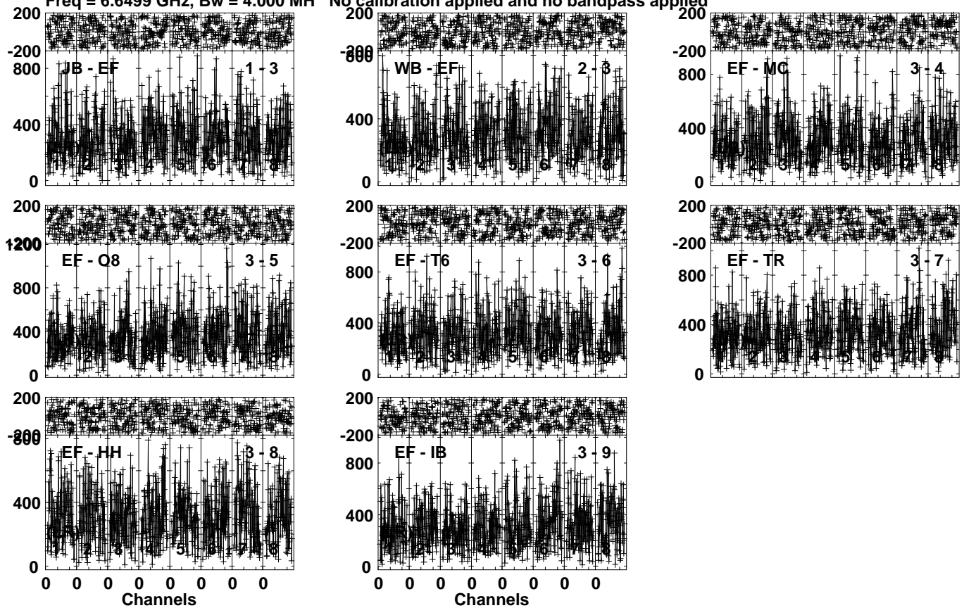
Lower frame: Micro Ampl Jy Top frame: Phas deg Vector averaged cross-power spectrum Several baselines displayed Timerange: 00/14:38:11 to 00/14:41:09
