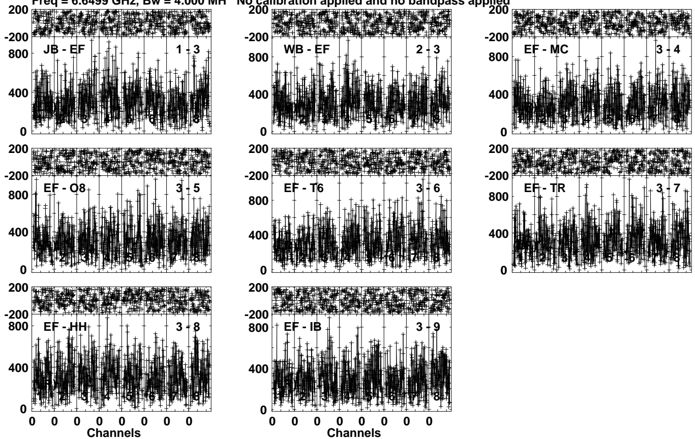
Lower frame: Micro Ampl Jy Top frame: Phas deg Vector averaged cross-power spectrum Several baselines displayed Timerange: 00/15:25:31 to 00/15:28:29
