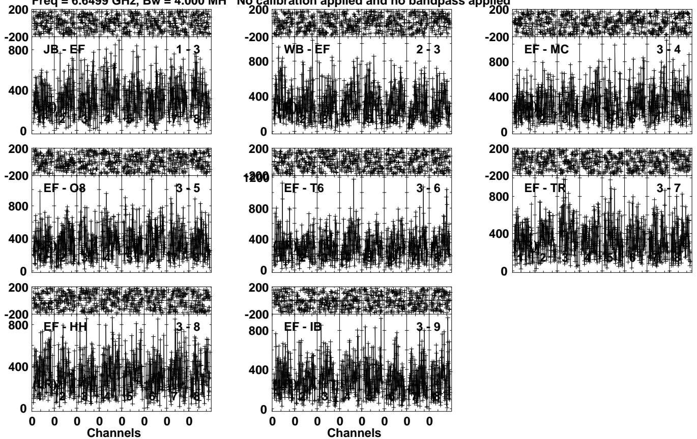
Lower frame: Micro Ampl Jy Top frame: Phas deg Vector averaged cross-power spectrum Several baselines displayed Timerange: 00/14:01:31 to 00/14:04:29
