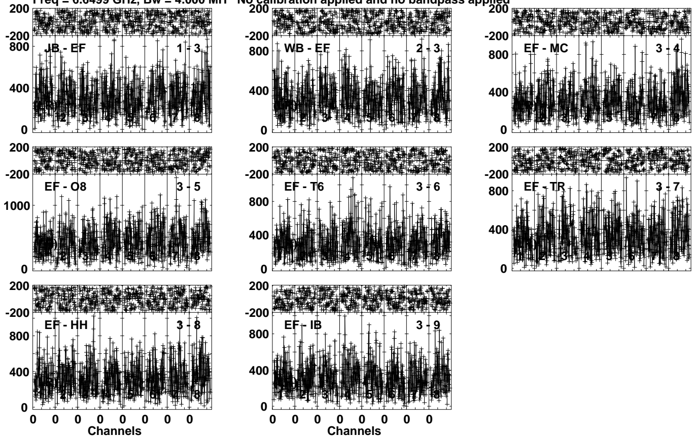
Lower frame: Micro Ampl Jy Top frame: Phas deg Vector averaged cross-power spectrum Several baselines displayed Timerange: 00/13:14:11 to 00/13:17:09
