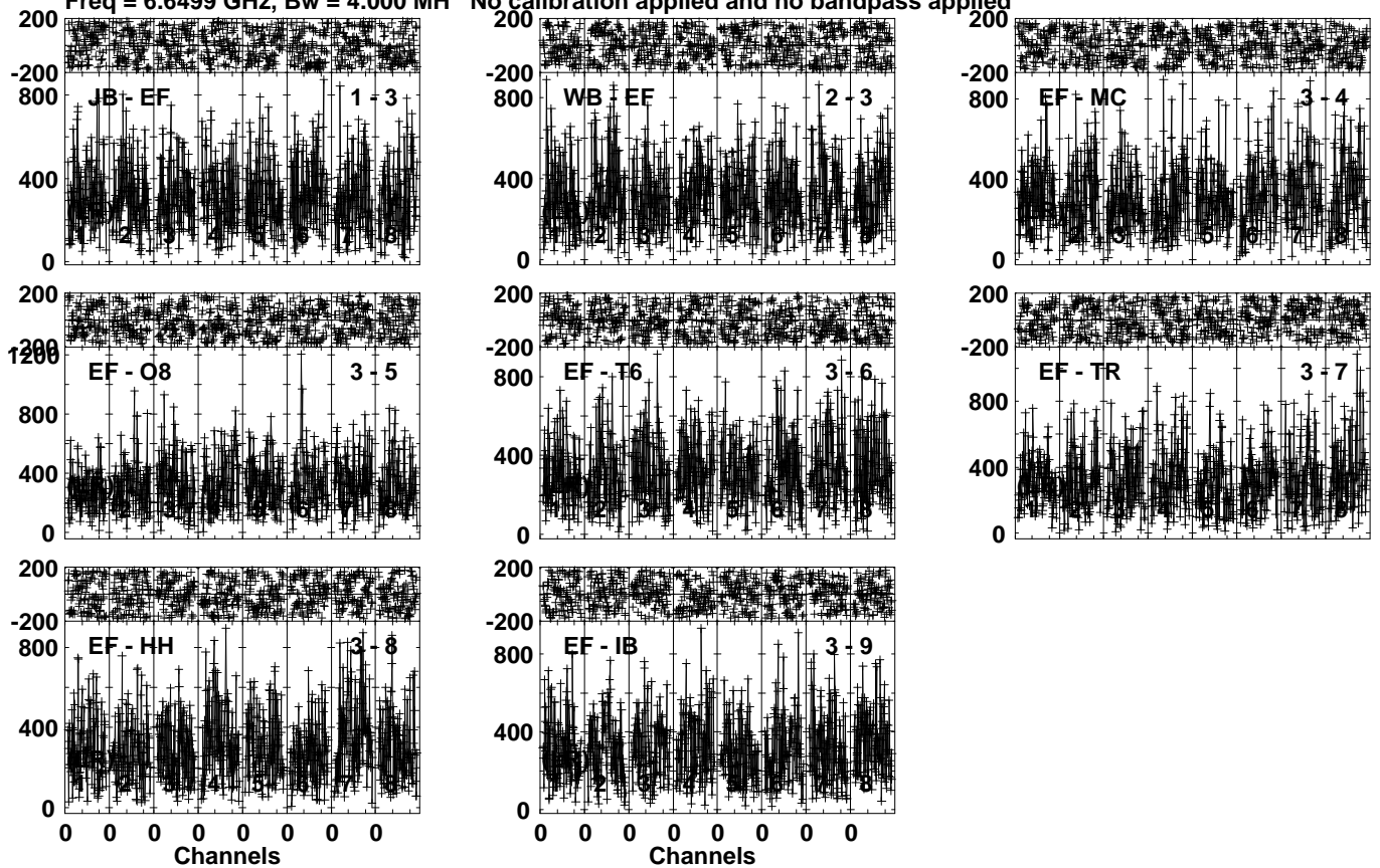
Lower frame: Micro Ampl Jy Top frame: Phas deg Vector averaged cross-power spectrum Several baselines displayed Timerange: 00/14:27:41 to 00/14:30:39
