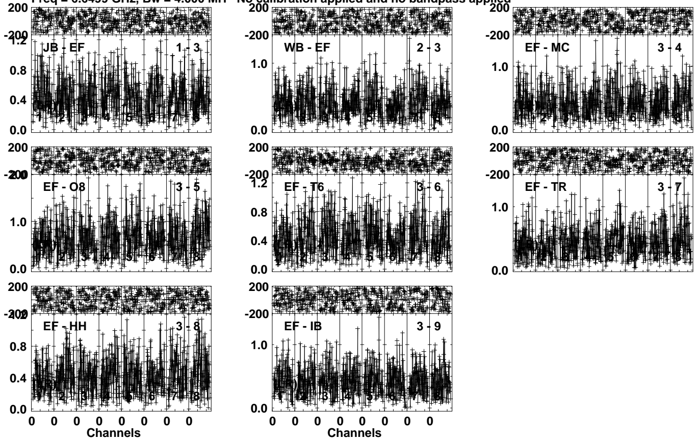
Lower frame: Milli Ampl Jy Top frame: Phas deg Vector averaged cross-power spectrum Several baselines displayed Timerange: 00/13:38:21 to 00/13:40:19
