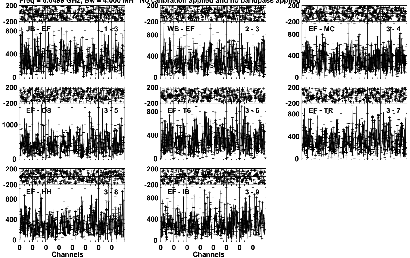
Lower frame: Micro Ampl Jy Top frame: Phas deg Vector averaged cross-power spectrum Several baselines displayed Timerange: 00/13:09:01 to 00/13:11:59
