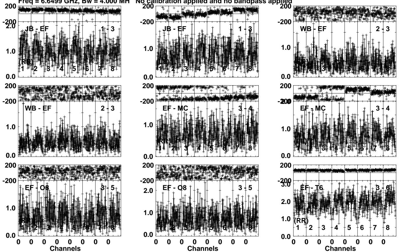
Lower frame: Milli Ampl Jy Top frame: Phas deg Vector averaged cross-power spectrum Several baselines displayed Timerange: 00/13:44:01 to 00/13:45:29
