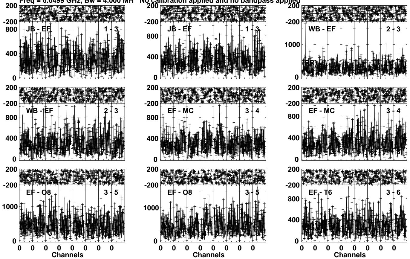
Lower frame: Micro Ampl Jy Top frame: Phas deg Vector averaged cross-power spectrum Several baselines displayed Timerange: 00/12:53:11 to 00/12:56:09
