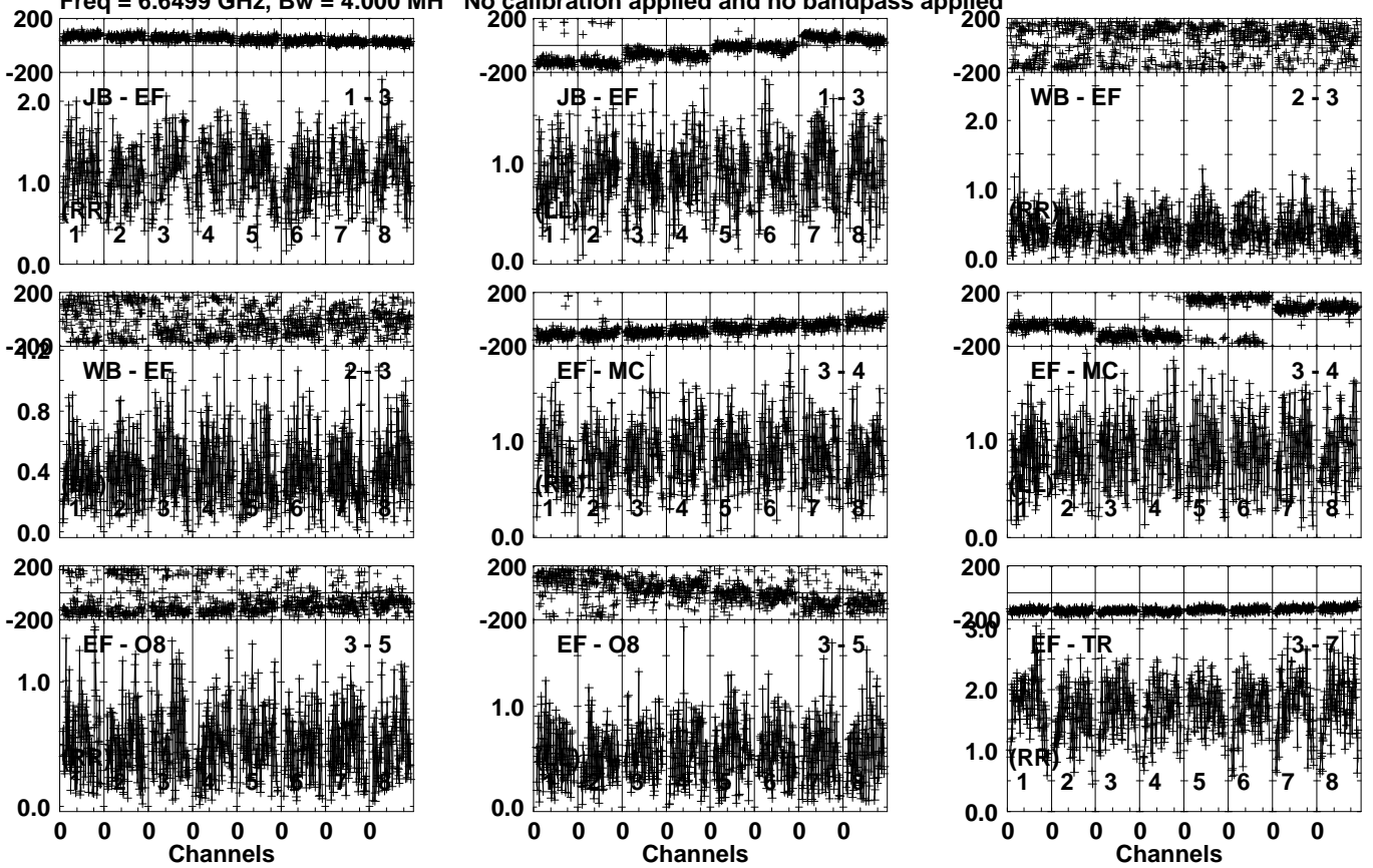
Lower frame: Milli Ampl Jy Top frame: Phas deg Vector averaged cross-power spectrum Several baselines displayed Timerange: 00/16:05:21 to 00/16:07:19
