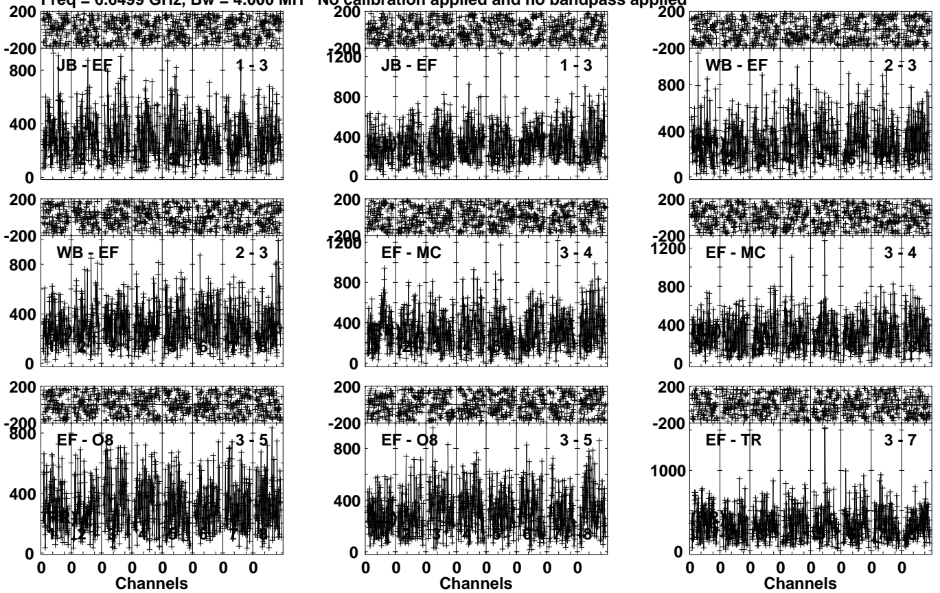
Lower frame: Micro Ampl Jy Top frame: Phas deg Vector averaged cross-power spectrum Several baselines displayed Timerange: 00/16:12:41 to 00/16:15:39
