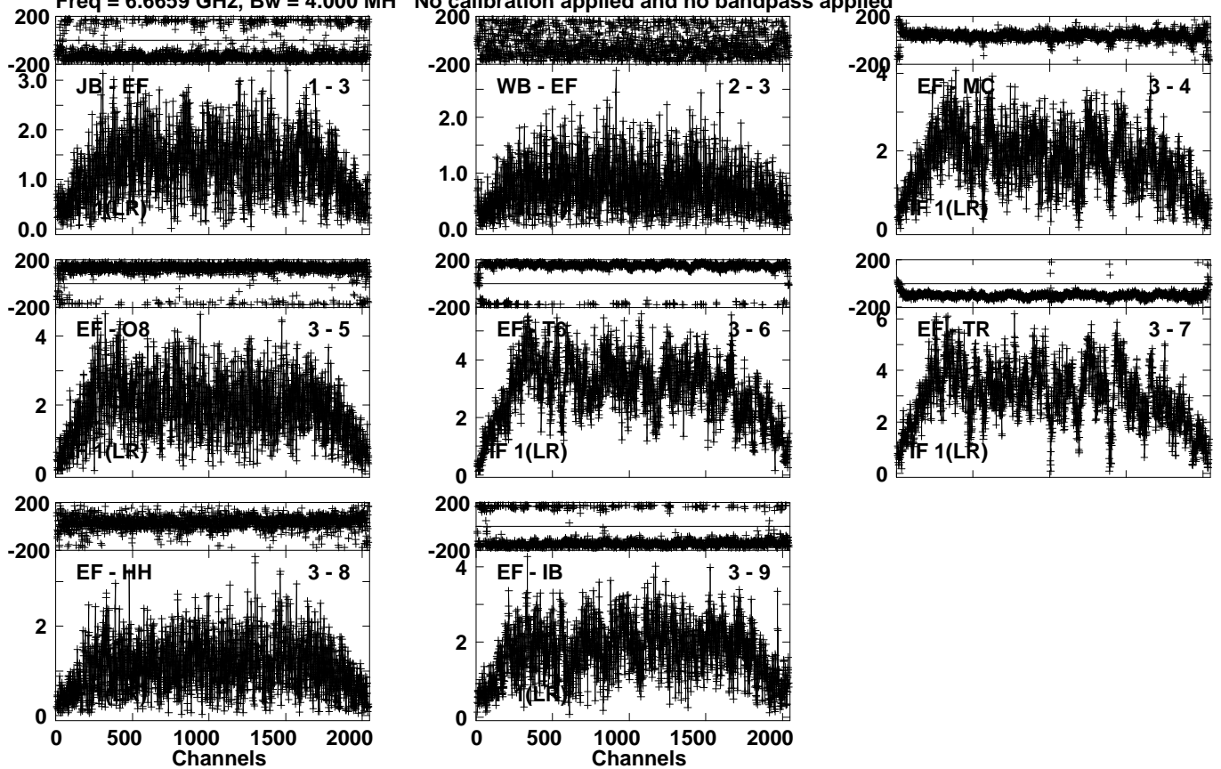
Lower frame: Milli Ampl Jy Top frame: Phas deg Vector averaged cross-power spectrum Several baselines displayed Timerange: 00/16:52:21 to 00/16:59:59
