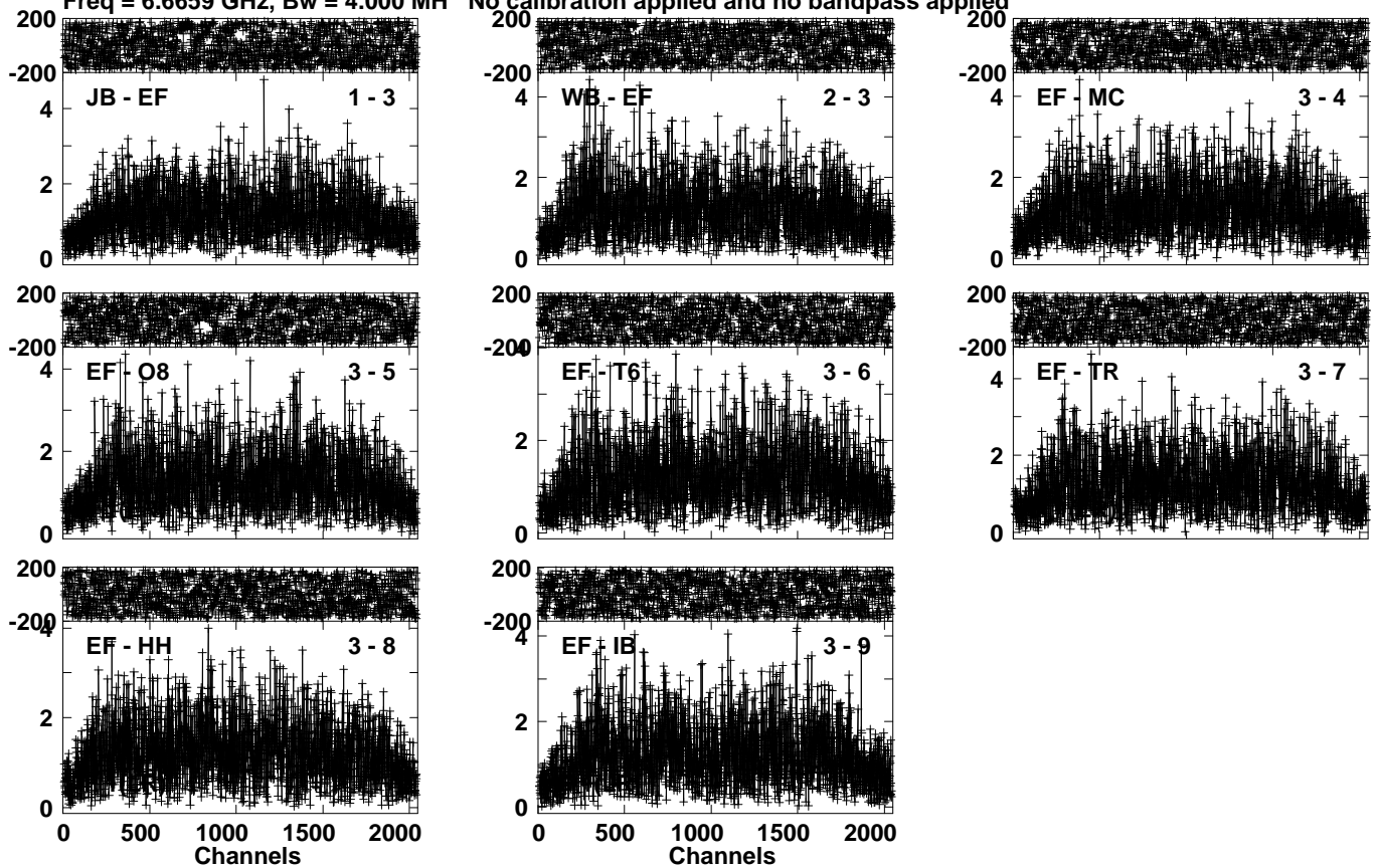
Lower frame: Milli Ampl Jy Top frame: Phas deg Vector averaged cross-power spectrum Several baselines displayed Timerange: 00/14:17:11 to 00/14:20:09
