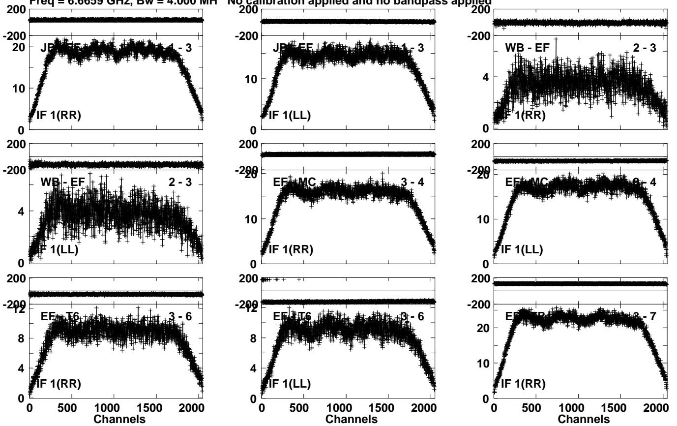
Lower frame: Milli Ampl Jy Top frame: Phas deg Vector averaged cross-power spectrum Several baselines displayed Timerange: 00/12:00:01 to 00/12:05:59
