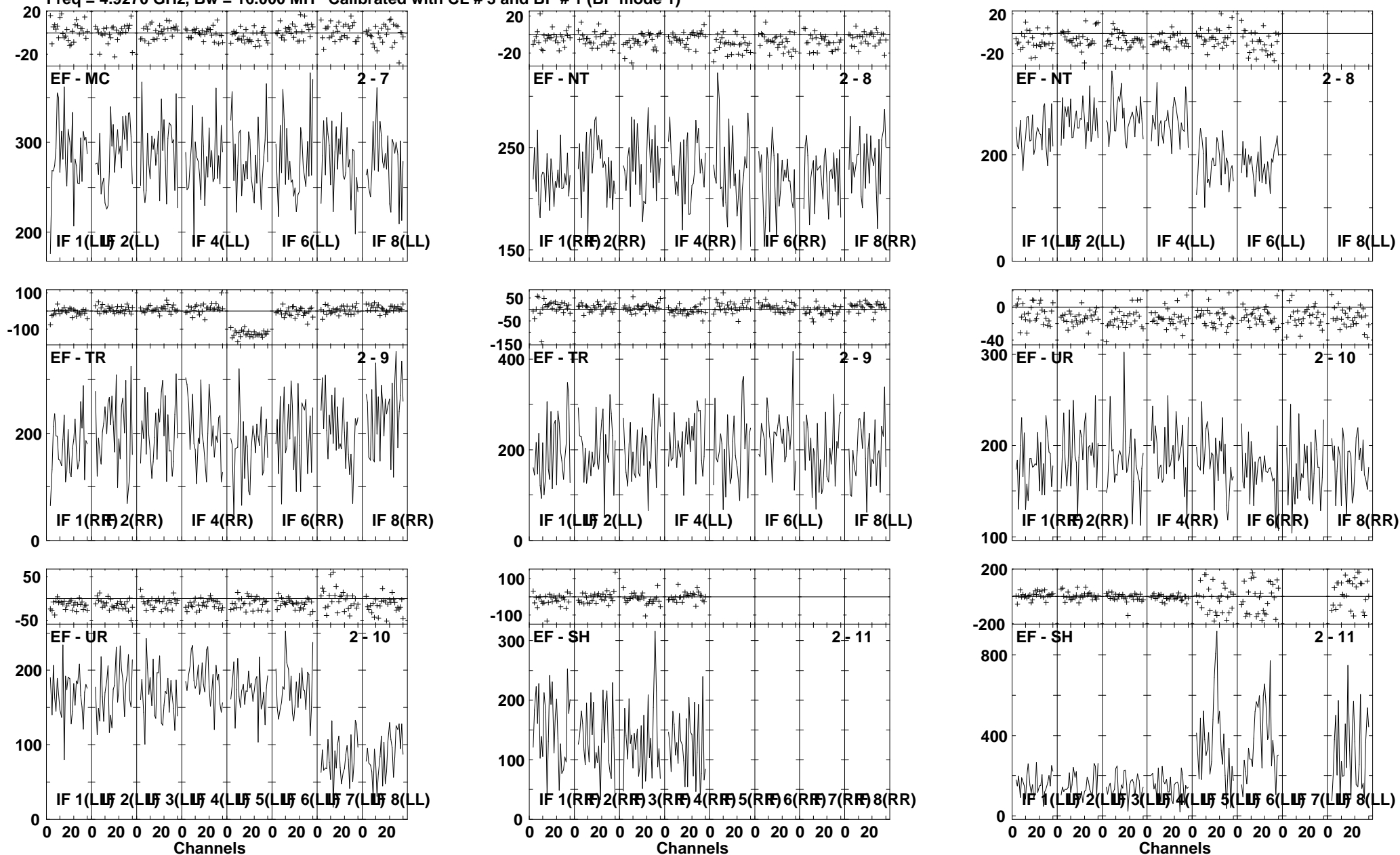
Lower frame: Milli Ampl Jy Top frame: Phas deg Vector averaged cross-power spectrum Several baselines displayed Timerange: 00/21:34:01 to 00/21:35:29
