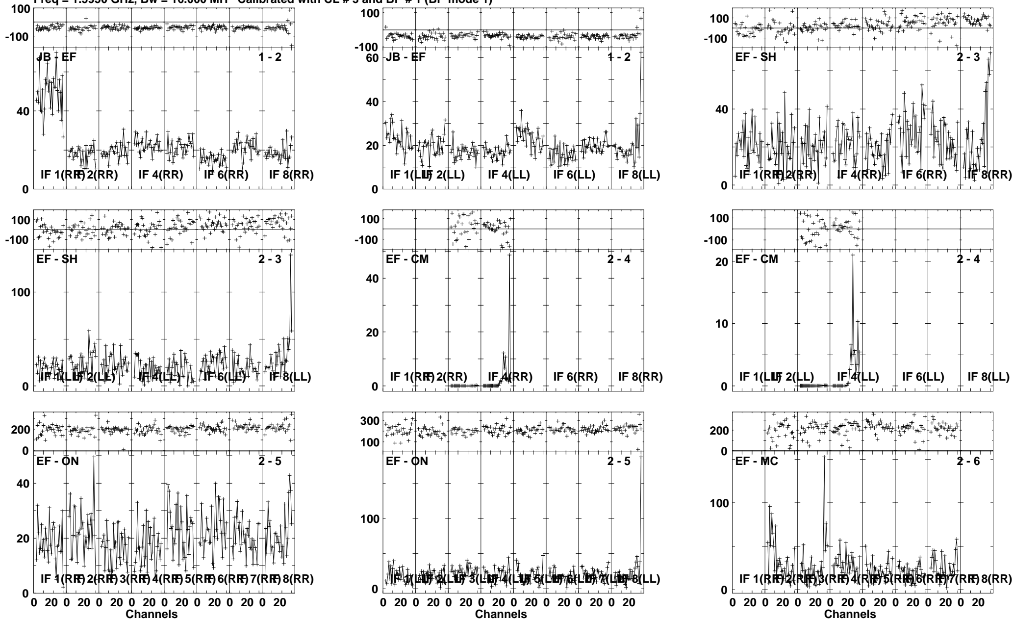
Lower frame: Milli Ampl Jy Top frame: Phas deg Vector averaged cross-power spectrum Several baselines displayed Timerange: 00/18:08:02 to 00/18:11:28
