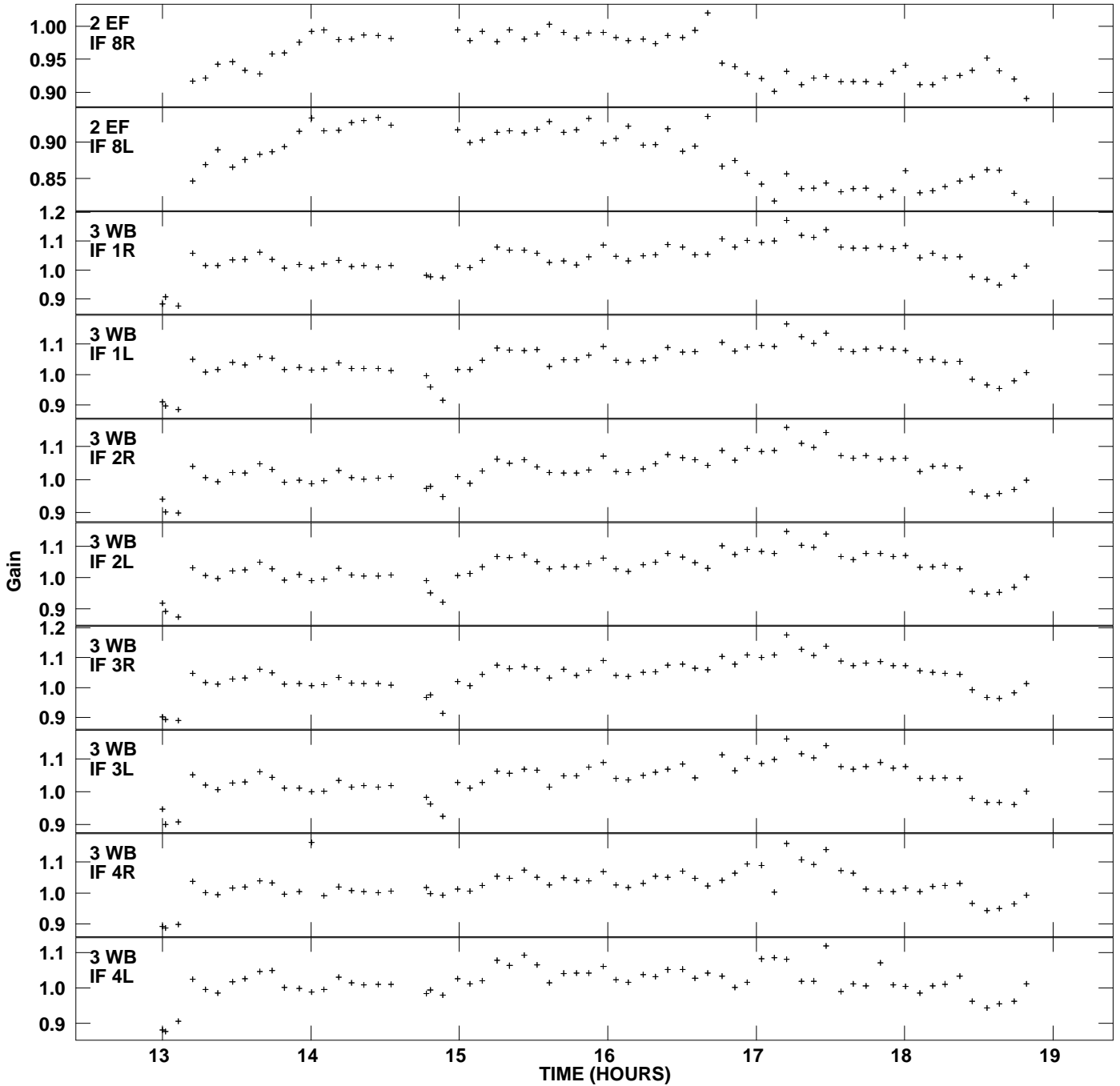
Plot file version 4 created 20-DEC-2011 15:26:06 Gain amp vs UTC time for J1128+5925.MULTI.1 SN 2 Rpol & Lpol IF 1 - 8
