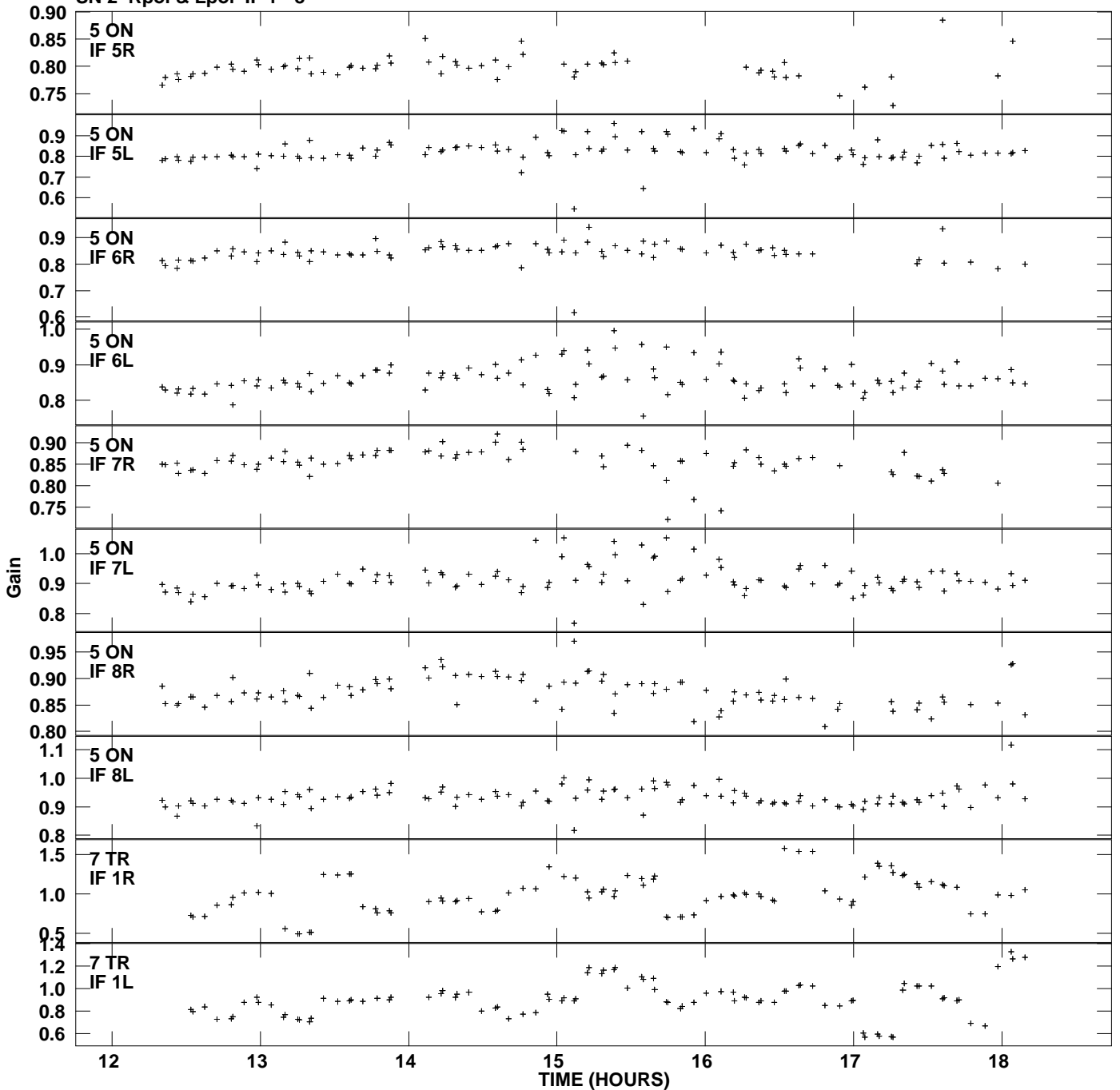
Plot file version 5 created 05-JAN-2012 19:17:12 Gain amp vs UTC time for J1128+5925.MULTI.1 SN 2 Rpol & Lpol IF 1 - 8
