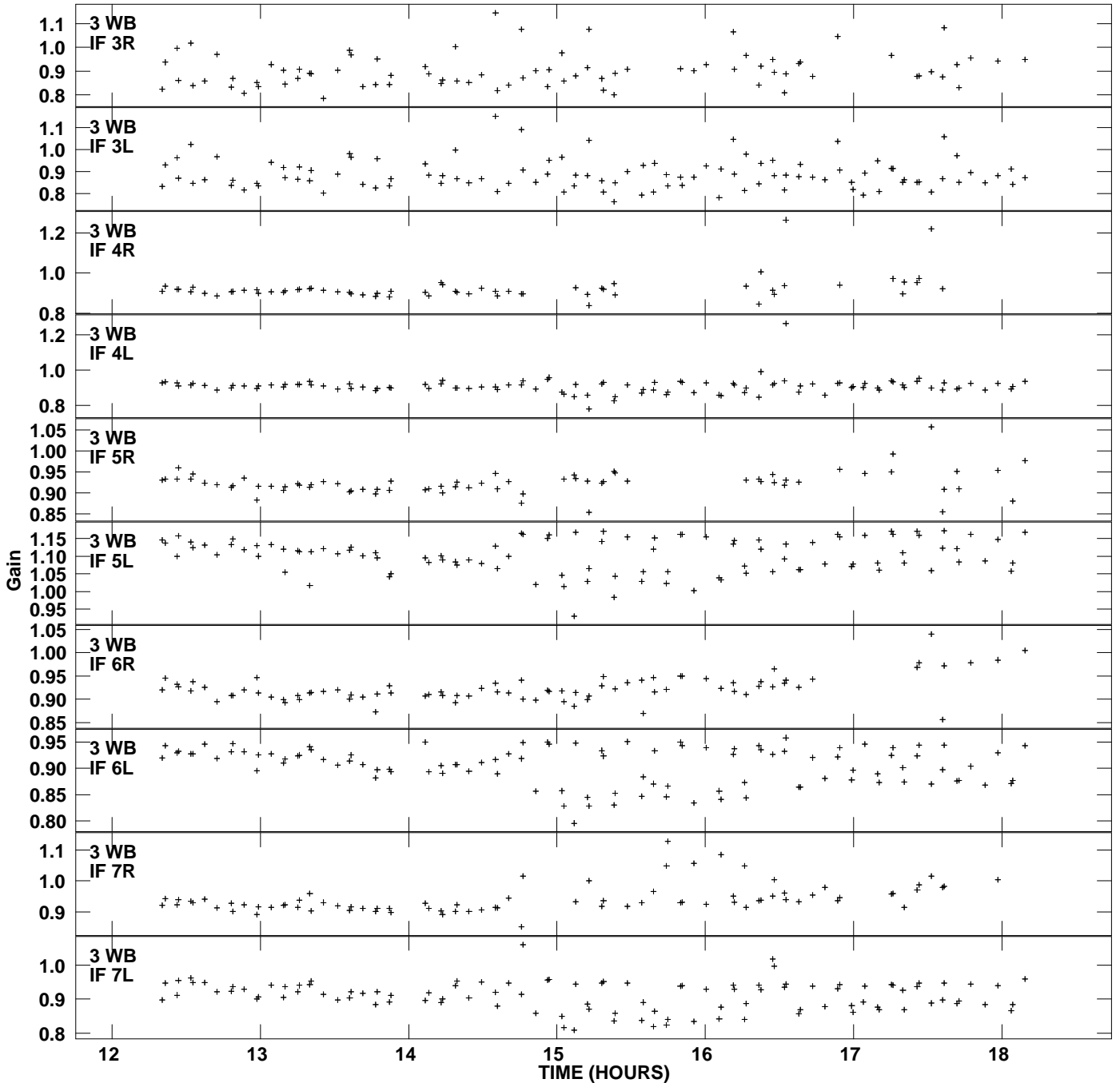
Plot file version 3 created 05-JAN-2012 19:17:12 Gain amp vs UTC time for J1128+5925.MULTI.1 SN 2 Rpol & Lpol IF 1 - 8
