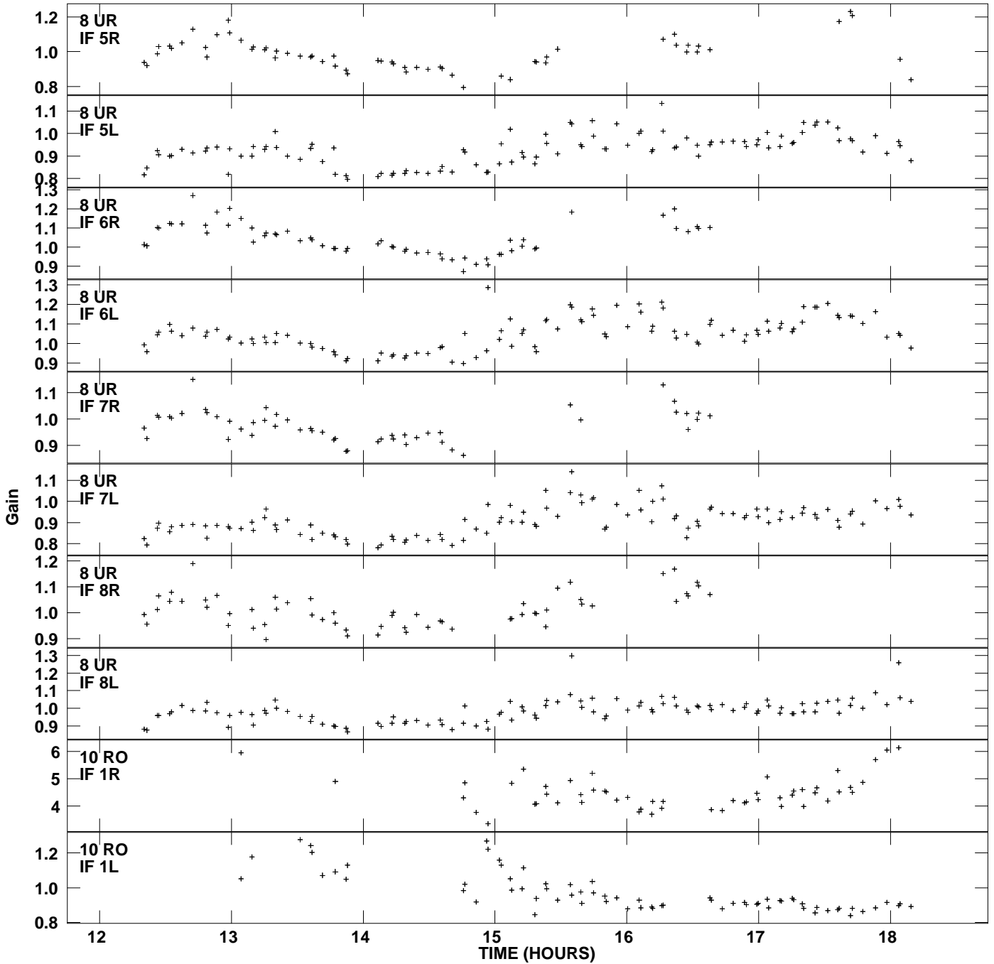
Plot file version 8 created 05-JAN-2012 19:17:12 Gain amp vs UTC time for J1128+5925.MULTI.1 SN 2 Rpol & Lpol IF 1 - 8
