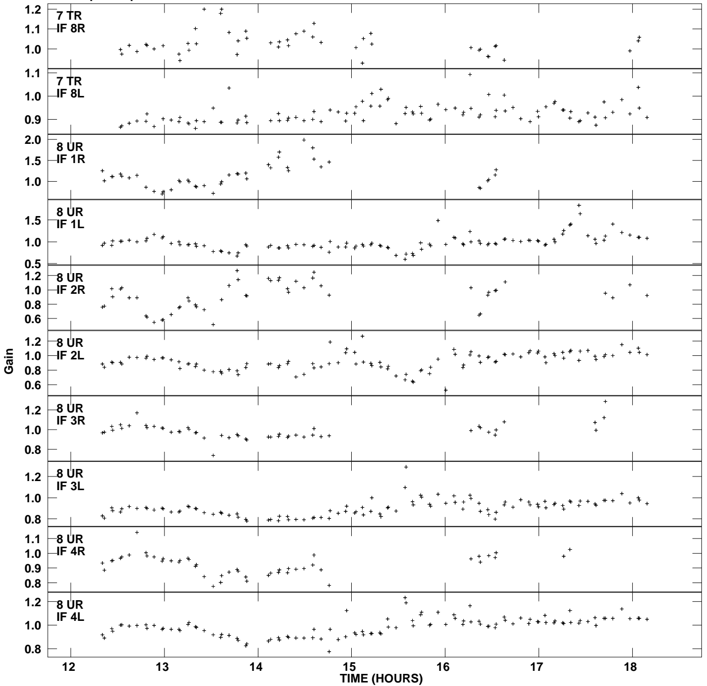
Plot file version 7 created 05-JAN-2012 19:17:12 Gain amp vs UTC time for J1128+5925.MULTI.1 SN 2 Rpol & Lpol IF 1 - 8
