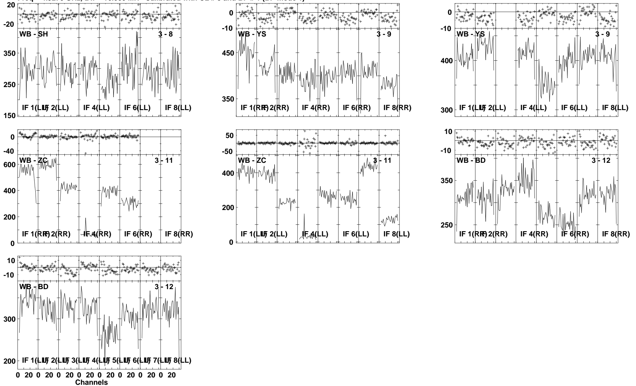
Lower frame: Milli Ampl Jy Top frame: Phas deg Vector averaged cross-power spectrum Several baselines displayed Timerange: 00/06:17:36 to 00/06:19:00
