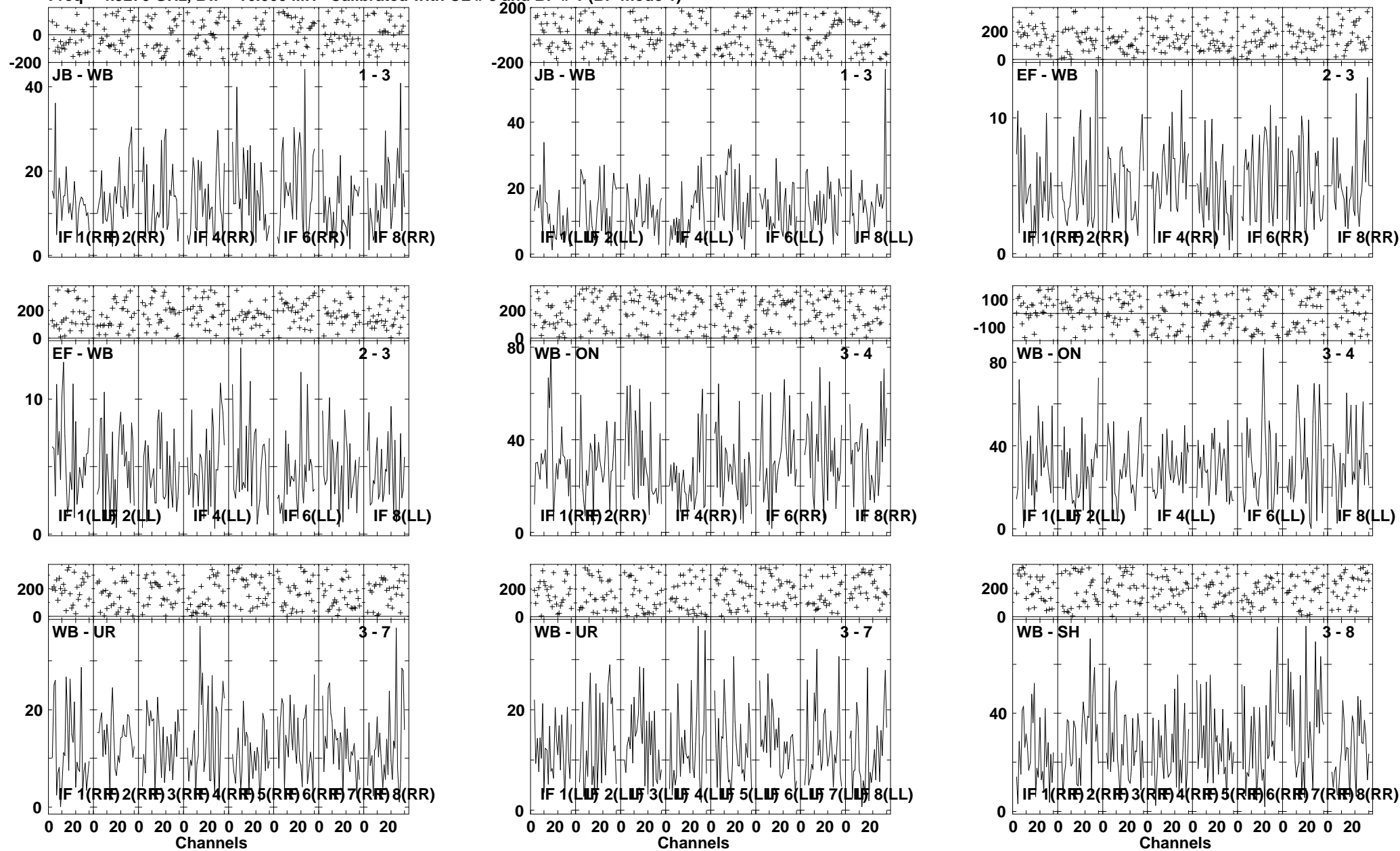
Lower frame: Milli Ampl Jy Top frame: Phas deg Vector averaged cross-power spectrum Several baselines displayed Timerange: 00/07:55:05 to 00/07:58:30
