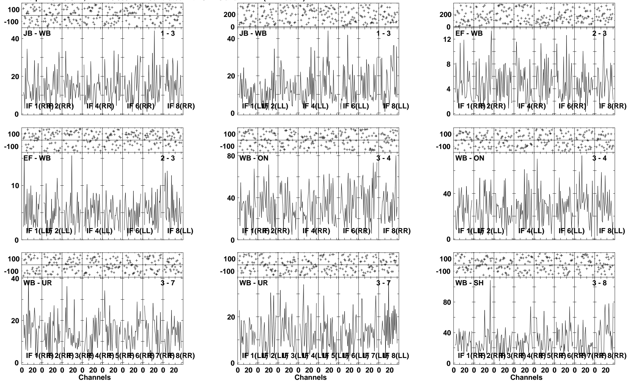
Lower frame: Milli Ampl Jy Top frame: Phas deg Vector averaged cross-power spectrum Several baselines displayed Timerange: 00/08:17:05 to 00/08:20:30
