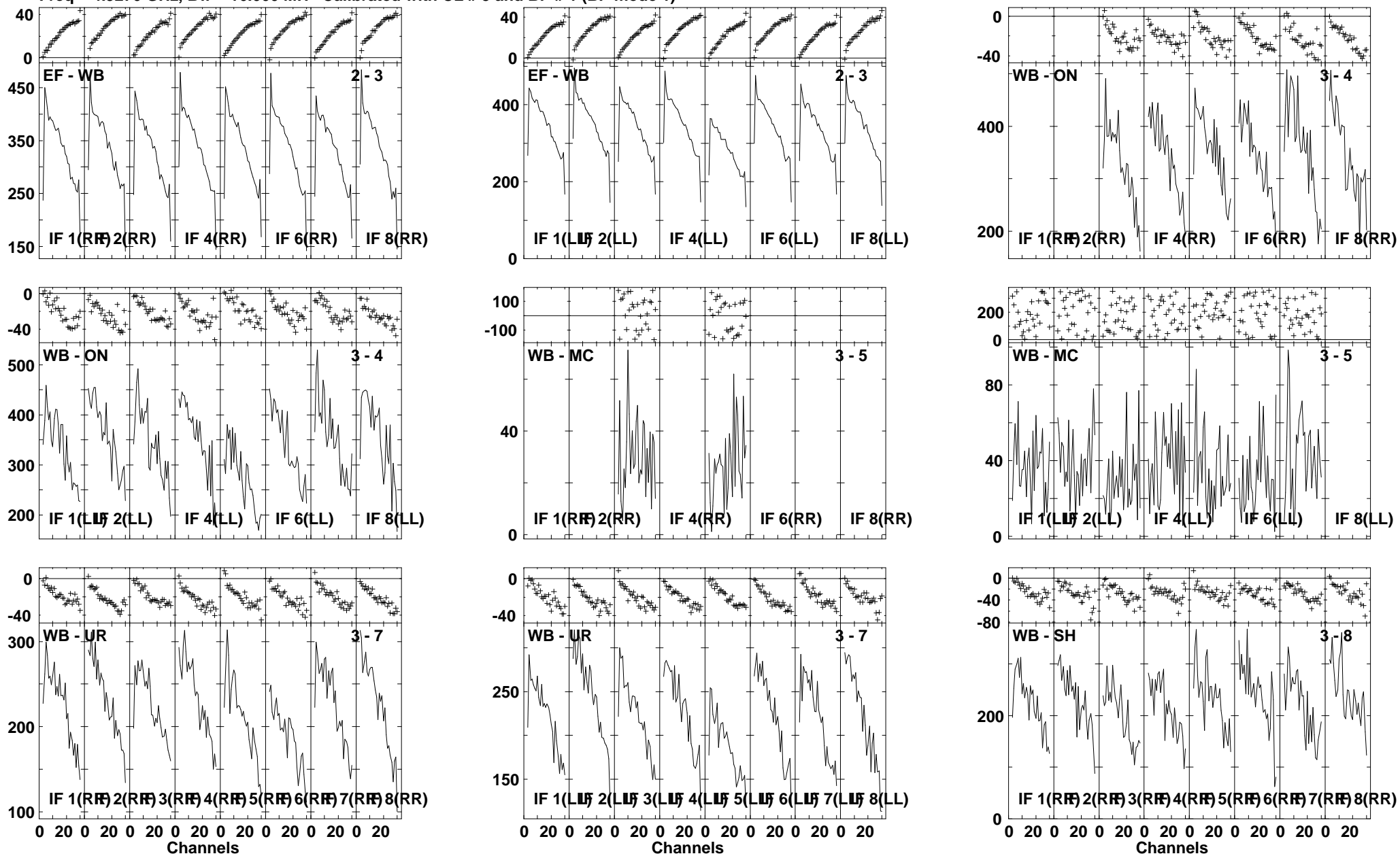
Lower frame: Milli Ampl Jy Top frame: Phas deg Vector averaged cross-power spectrum Several baselines displayed Timerange: 00/08:53:32 to 00/08:55:00
