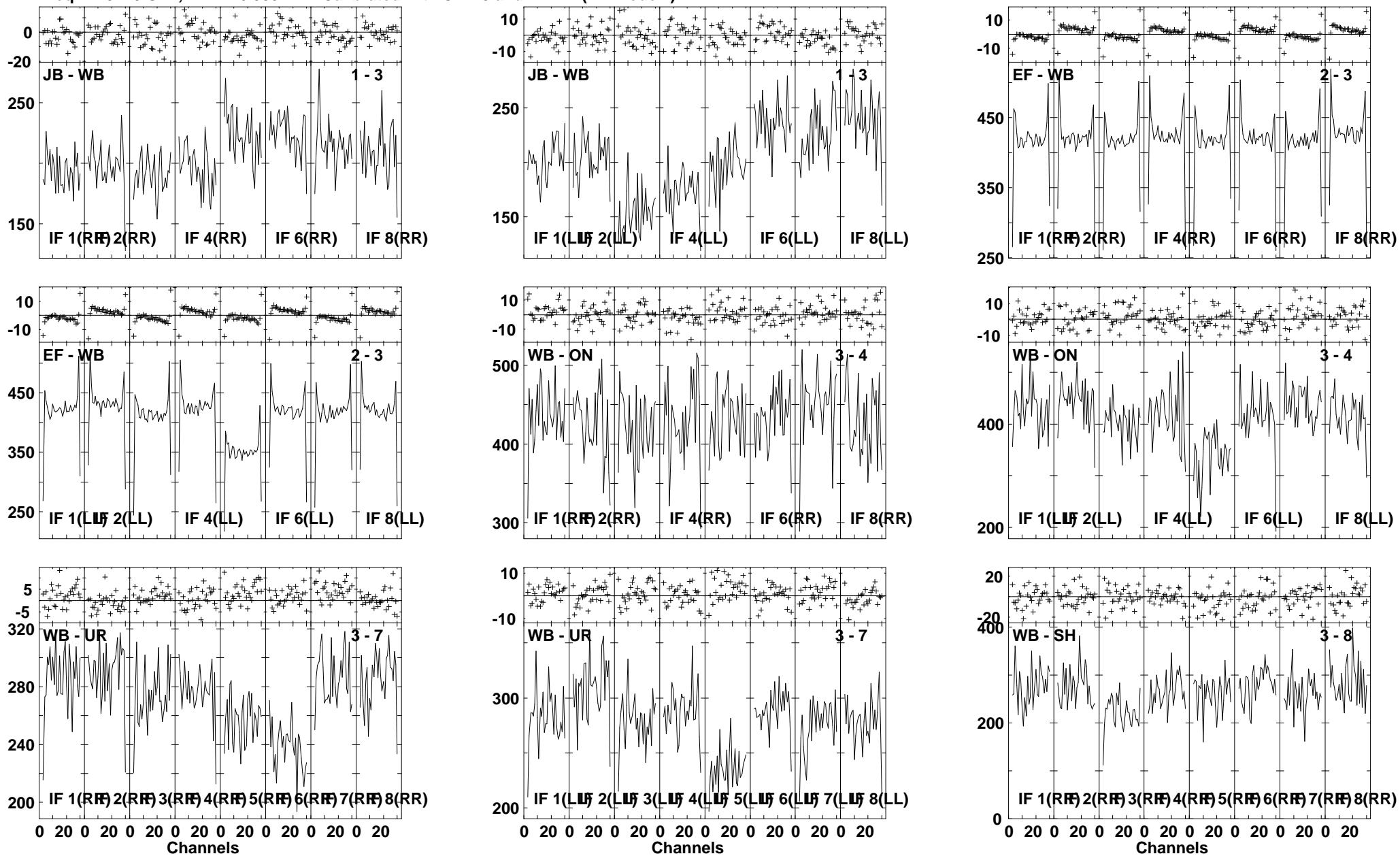
Lower frame: Milli Ampl Jy Top frame: Phas deg Vector averaged cross-power spectrum Several baselines displayed Timerange: 00/07:53:36 to 00/07:54:59
