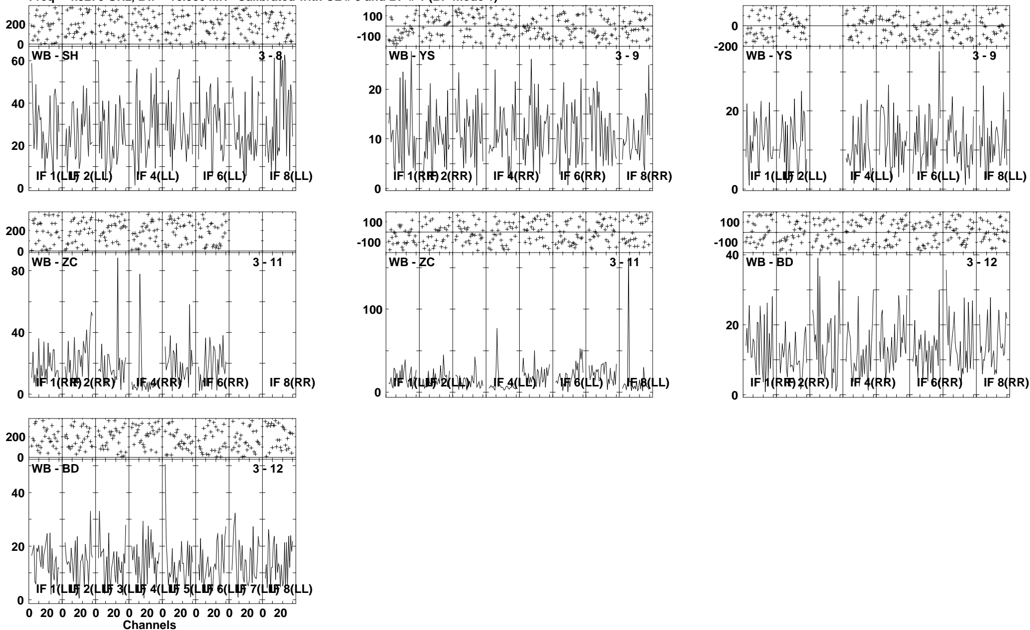
Lower frame: Milli Ampl Jy Top frame: Phas deg Vector averaged cross-power spectrum Several baselines displayed Timerange: 00/07:18:01 to 00/07:21:30
