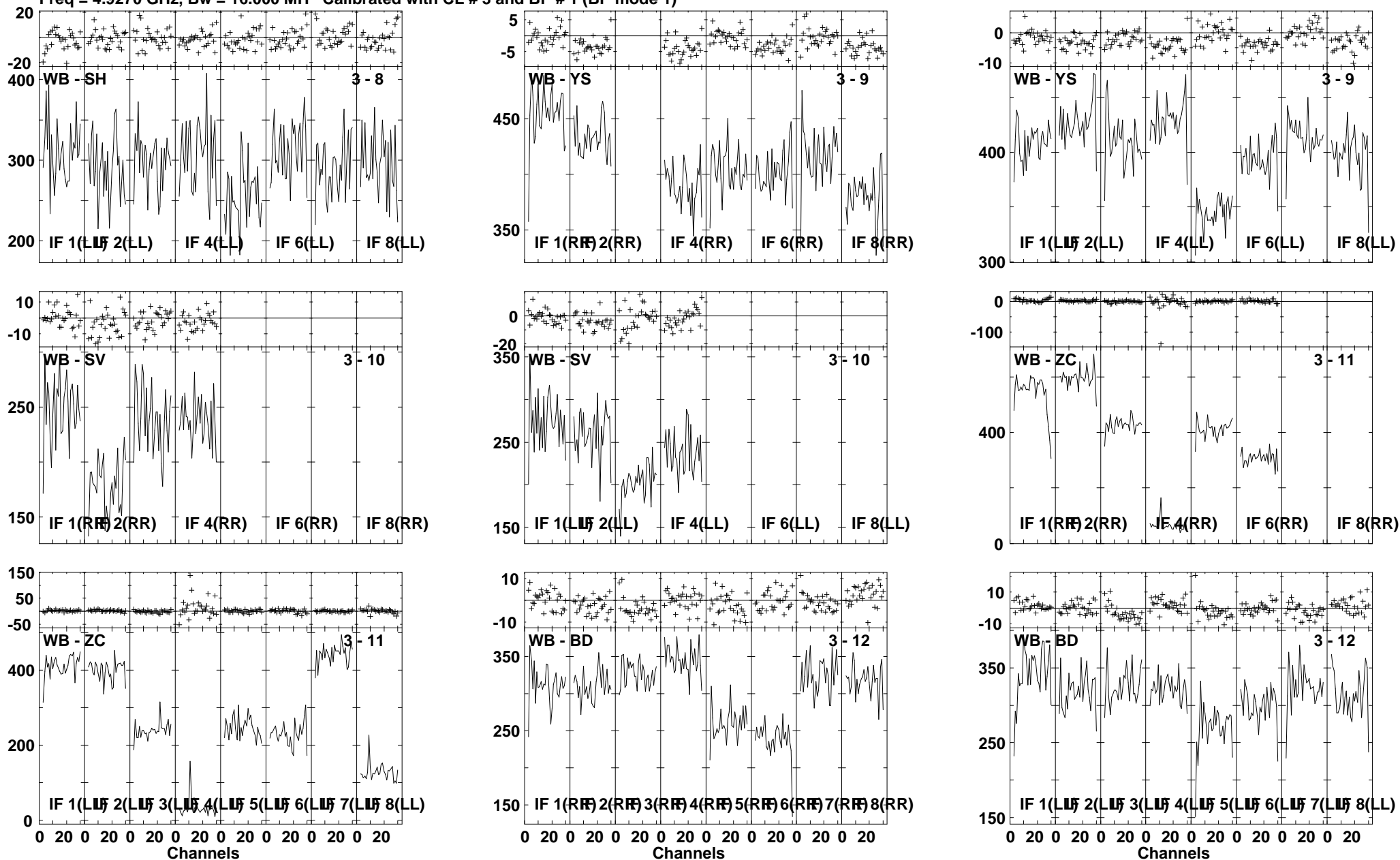
Lower frame: Milli Ampl Jy Top frame: Phas deg Vector averaged cross-power spectrum Several baselines displayed Timerange: 00/06:12:35 to 00/06:13:59
