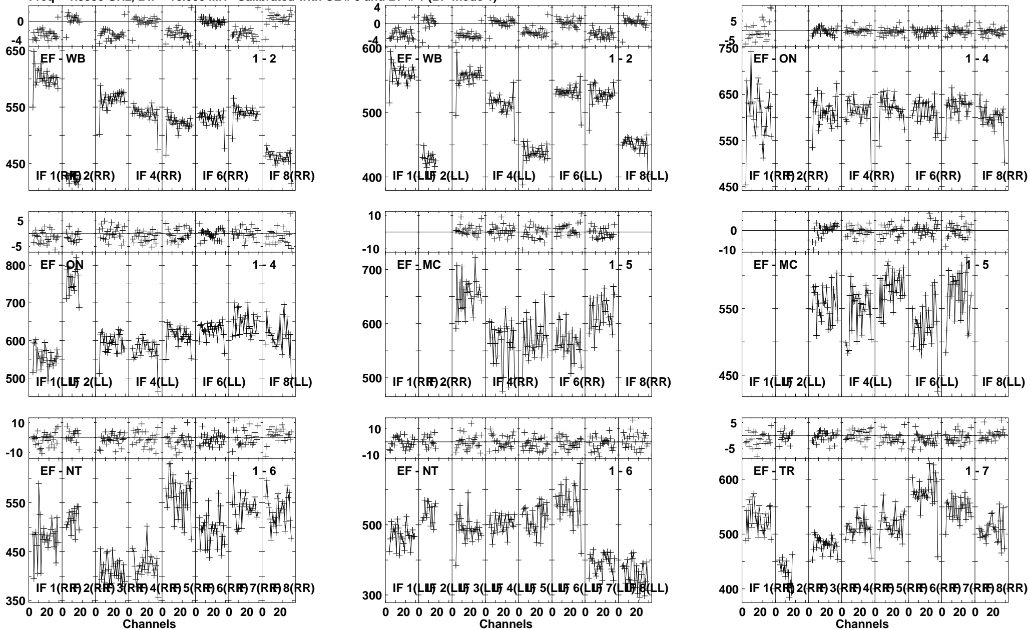
Lower frame: Milli Ampl Jy Top frame: Phas deg Vector averaged cross-power spectrum Several baselines displayed Timerange: 00/15:43:06 to 00/15:43:58
