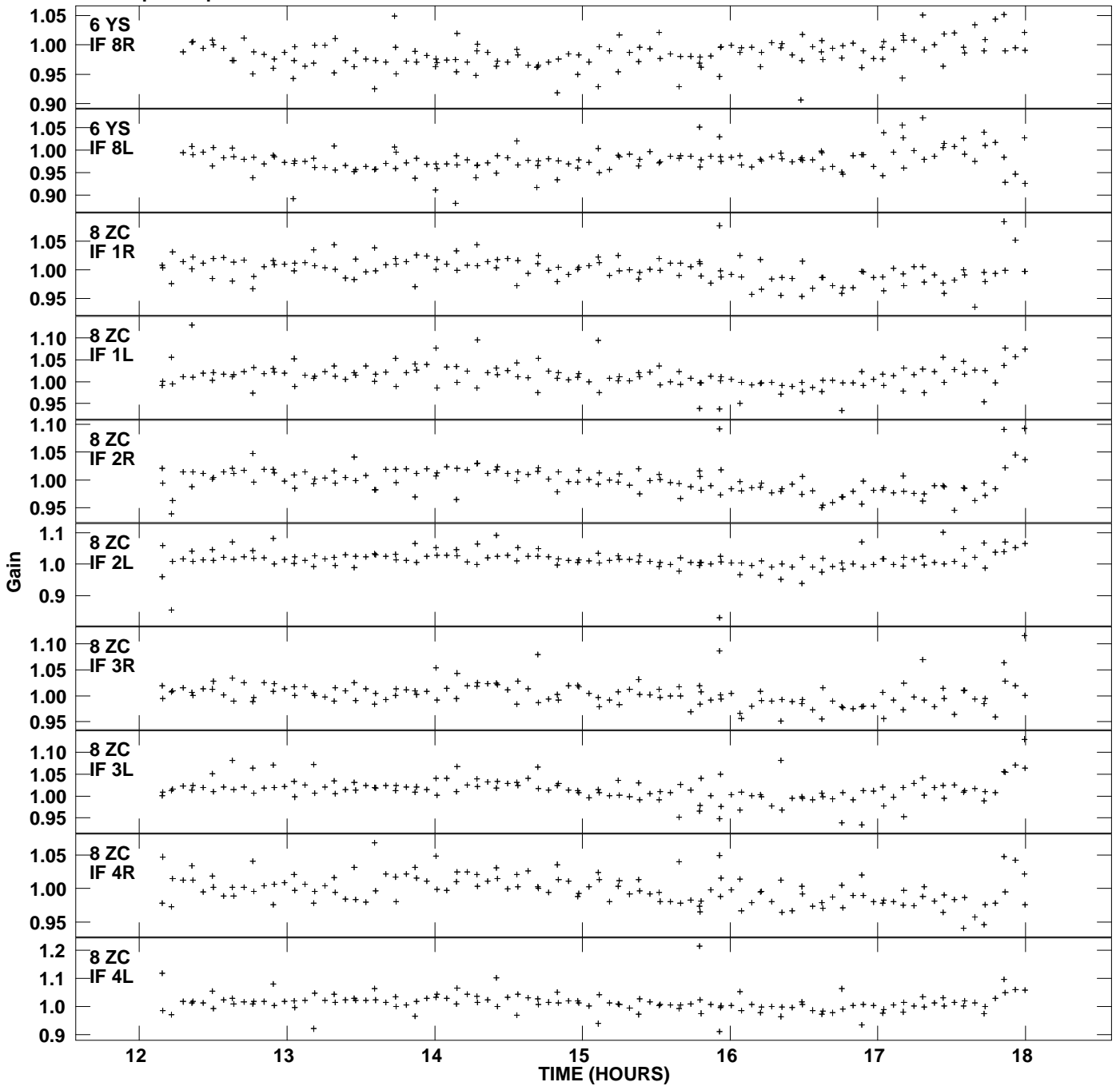
Plot file version 8 created 11-NOV-2013 20:57:20 Gain amp vs UTC time for J1128+5925.MULTI.1 SN 4 Rpol & Lpol IF 1 - 8
