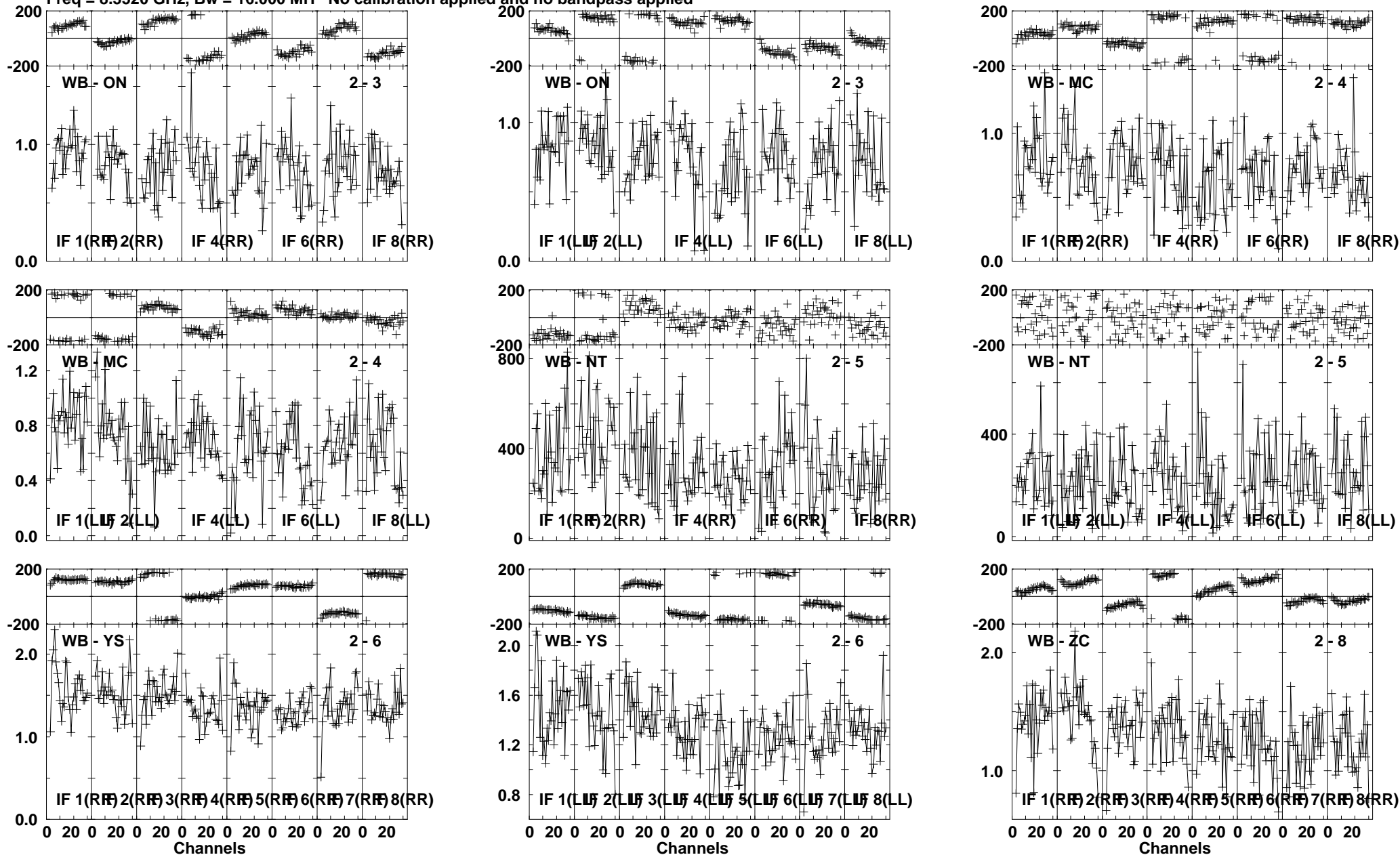
Lower frame: Milli Ampl Jy Top frame: Phas deg Vector averaged cross-power spectrum Several baselines displayed Timerange: 00/16:53:14 to 00/16:54:15
