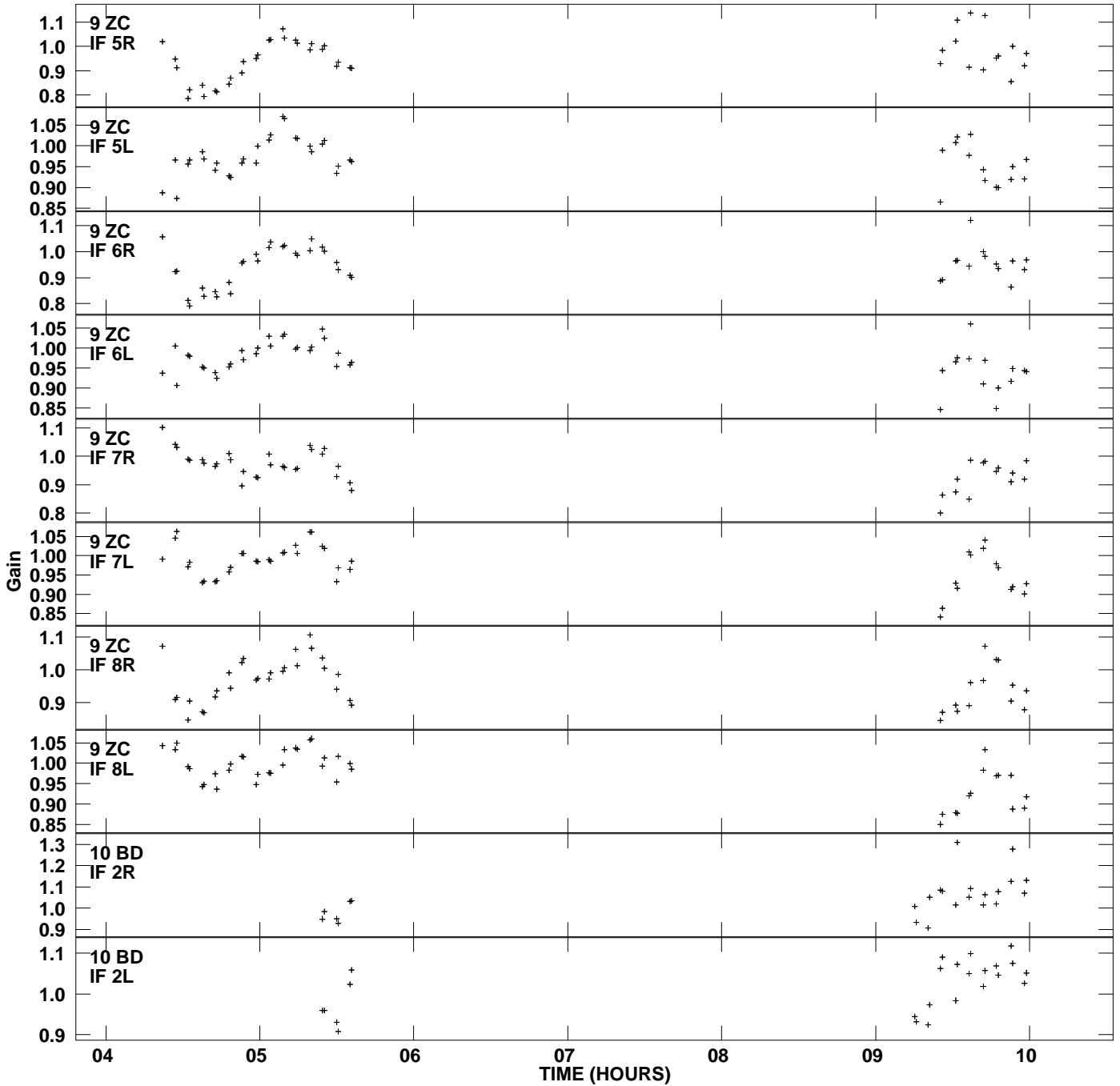
Plot file version 11 created 20-MAR-2013 15:31:52 Gain amp vs UTC time for J1332+4722.MULTI.1 SN 4 Rpol & Lpol IF 1 - 8
