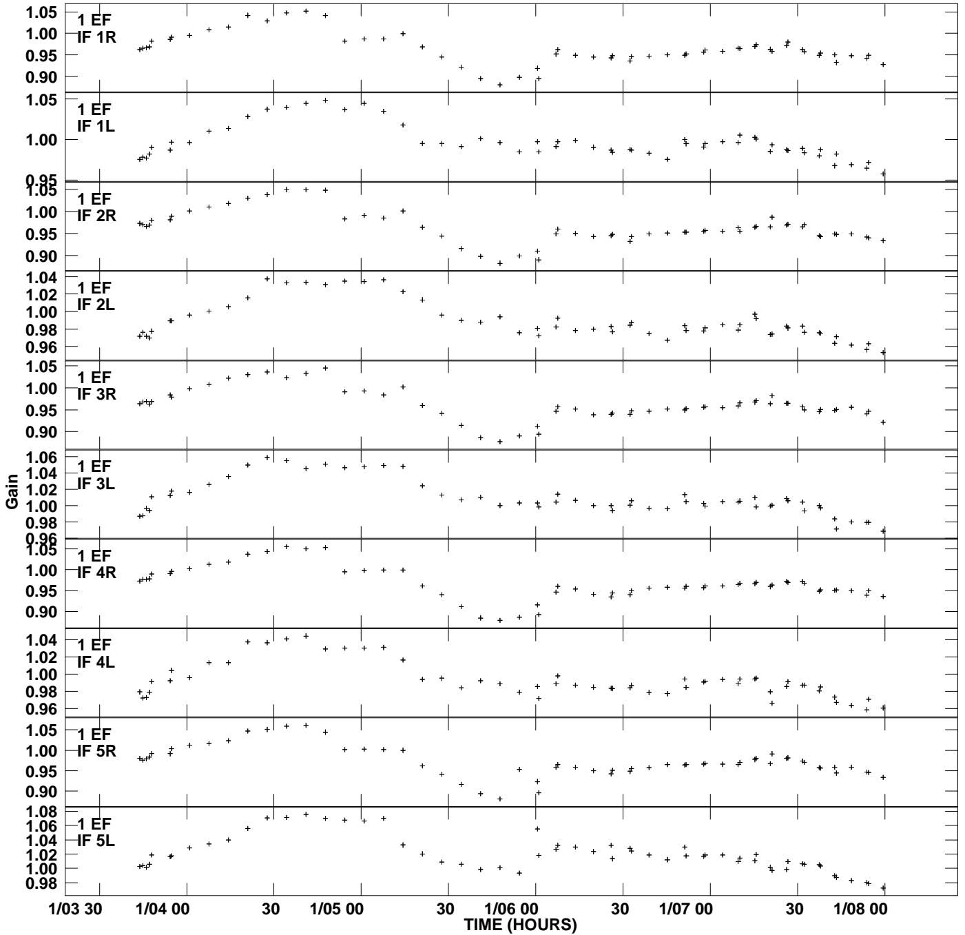
Plot file version 1 created 17-JUL-2012 18:52:48 Gain amp vs UTC time for B1637+57.MULTI.1 SN 2 Rpol & Lpol IF 1 - 8
