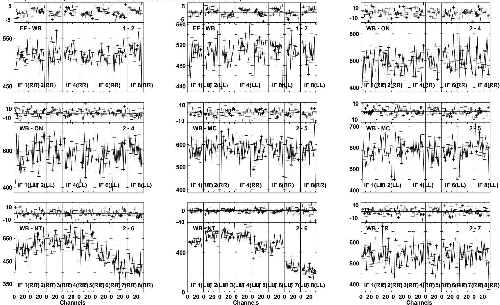
Lower frame: Milli Ampl Jy Top frame: Phas deg Vector averaged cross-power spectrum Several baselines displayed Timerange: 01/02:41:10 to 01/02:41:39
