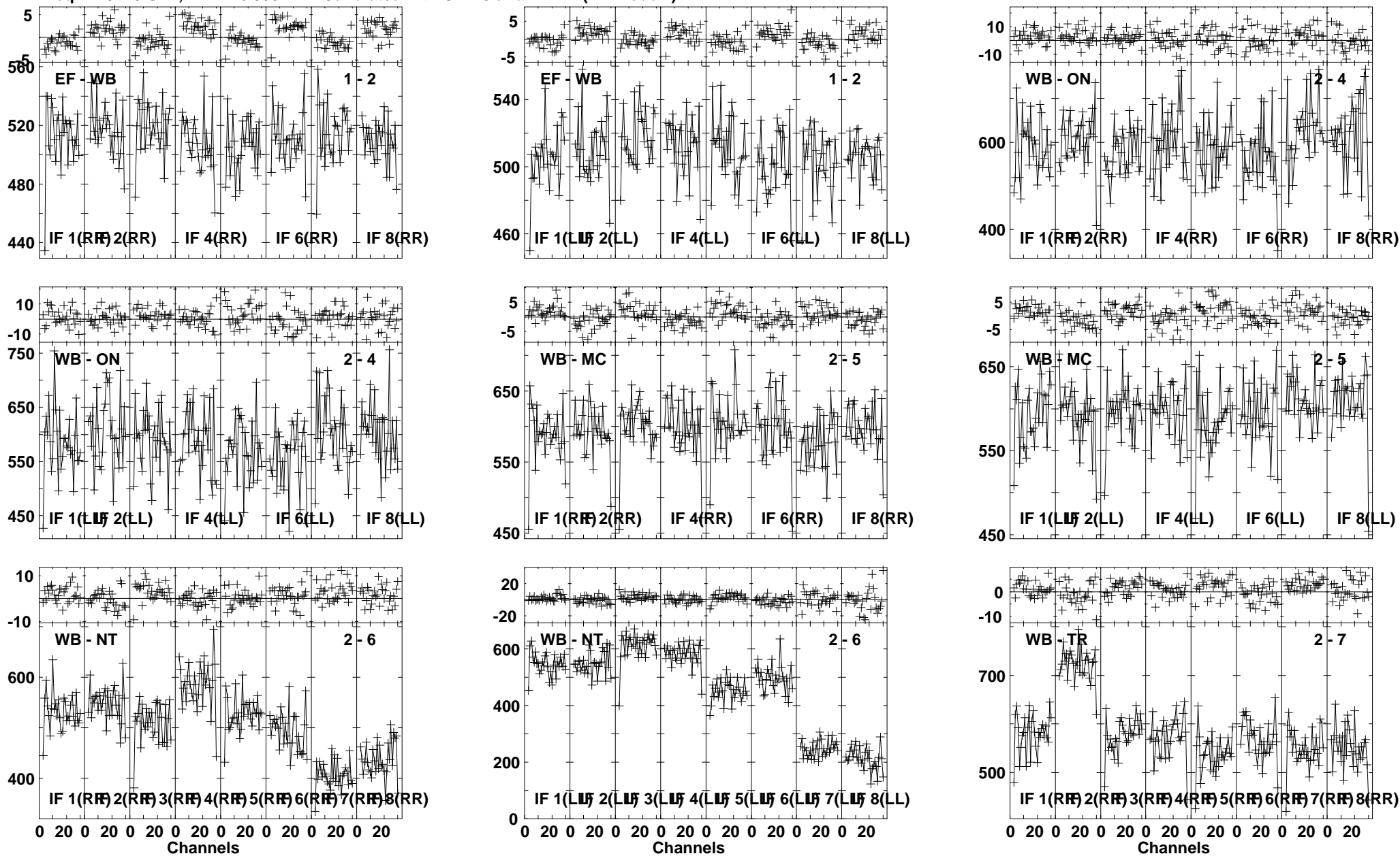
Lower frame: Milli Ampl Jy Top frame: Phas deg Vector averaged cross-power spectrum Several baselines displayed Timerange: 01/00:29:14 to 01/00:30:09
