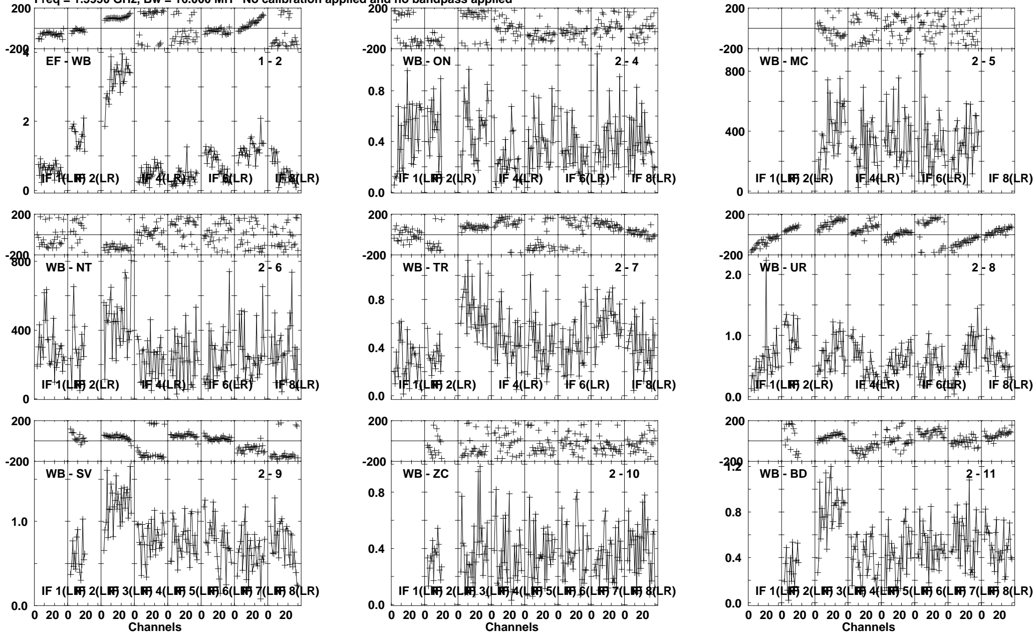
Lower frame: Milli Ampl Jy Top frame: Phas deg Vector averaged cross-power spectrum Several baselines displayed Timerange: 01/02:58:25 to 01/02:59:19
