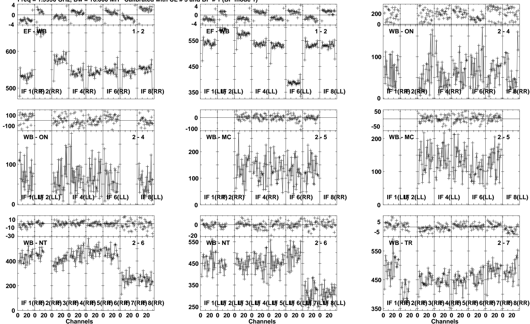
Lower frame: Milli Ampl Jy Top frame: Phas deg Vector averaged cross-power spectrum Several baselines displayed Timerange: 01/02:35:43 to 01/02:36:49
