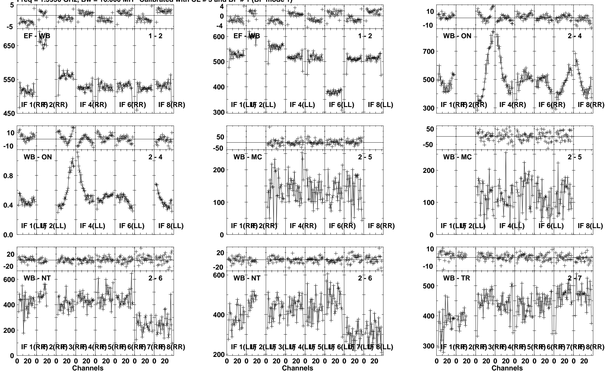
Lower frame: Milli Ampl Jy Top frame: Phas deg Vector averaged cross-power spectrum Several baselines displayed Timerange: 00/23:01:33 to 00/23:02:29
