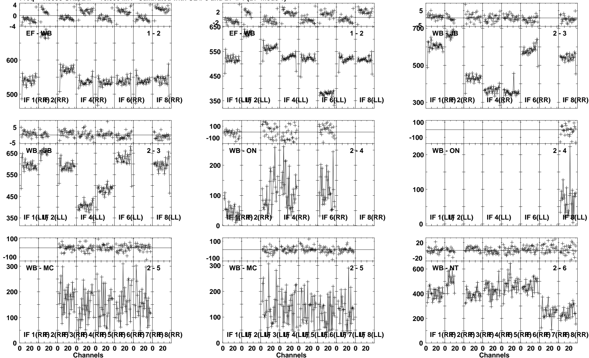
Lower frame: Milli Ampl Jy Top frame: Phas deg Vector averaged cross-power spectrum Several baselines displayed Timerange: 01/01:56:51 to 01/01:57:19
