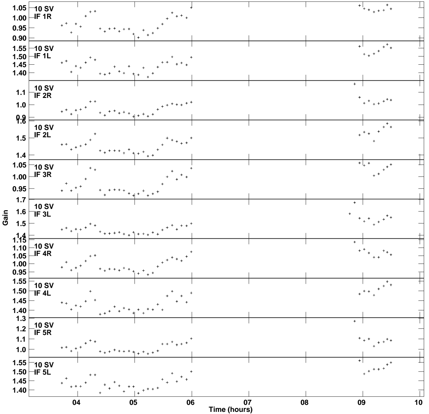
Plot file version 12 created 25-MAR-2014 11:08:37 Gain amp vs UTC time for J1128+5925.MULTI.1 SN 2 Rpol & Lpol IF 1 - 8
