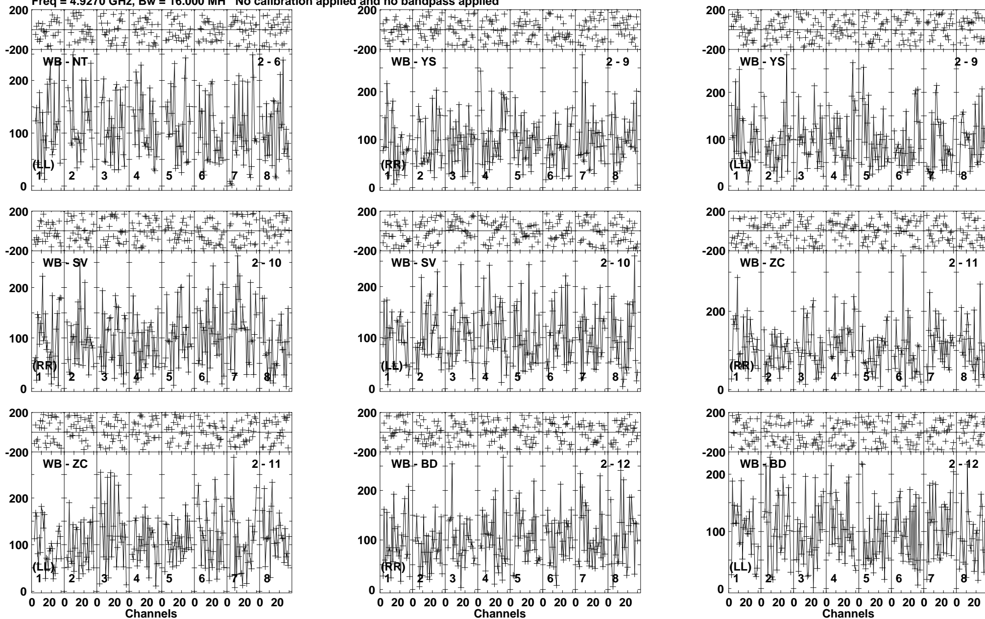
Lower frame: Micro Ampl Jy Top frame: Phas deg Vector averaged cross-power spectrum Baseline: WB (02) - NT (06) Timerange: 00/05:54:55 to 00/05:58:49
