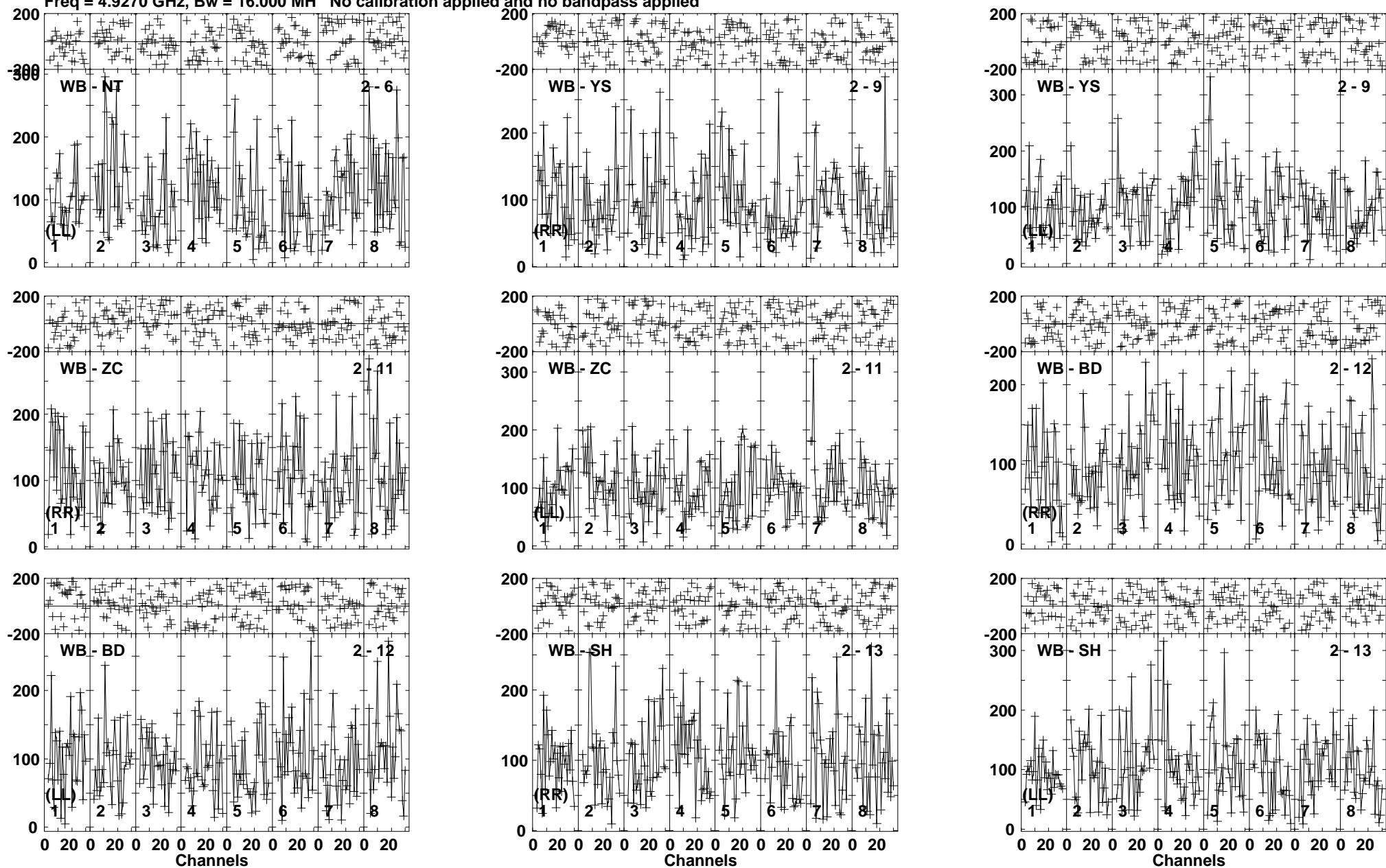
Lower frame: Micro Ampl Jy Top frame: Phas deg Vector averaged cross-power spectrum Baseline: WB (02) - NT (06) Timerange: 00/07:41:01 to 00/07:44:59
