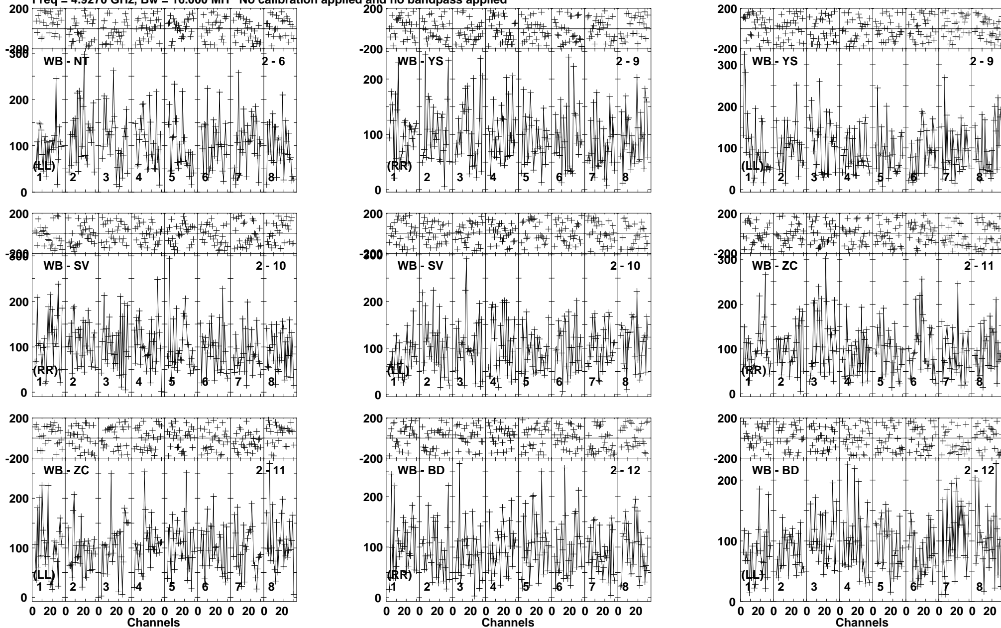
Lower frame: Micro Ampl Jy Top frame: Phas deg Vector averaged cross-power spectrum Baseline: WB (02) - NT (06) Timerange: 00/05:49:41 to 00/05:53:39
