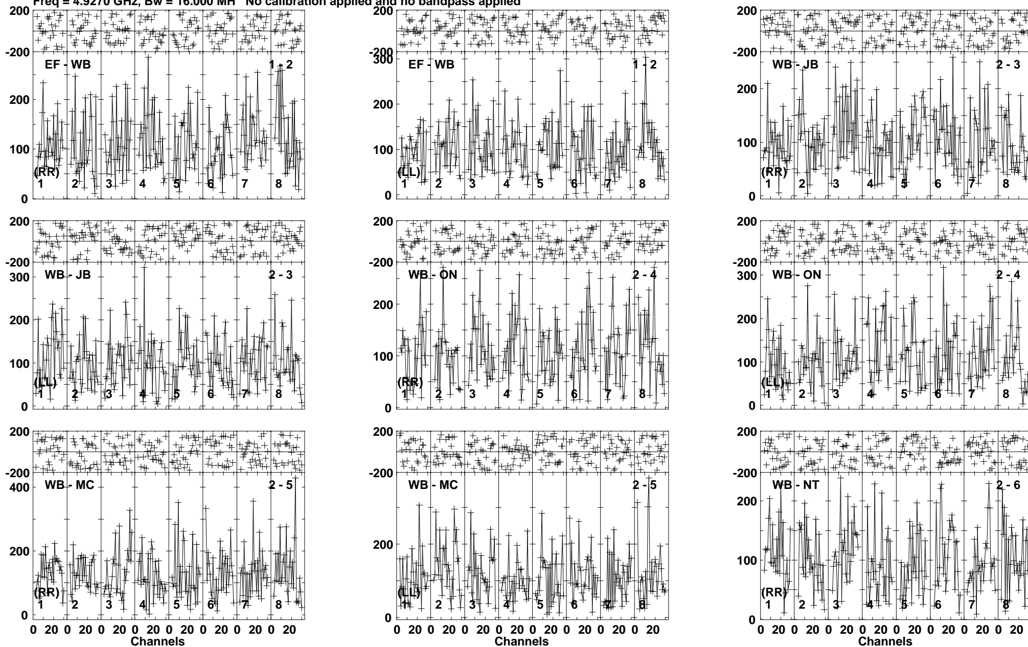
Lower frame: Micro Ampl Jy Top frame: Phas deg Vector averaged cross-power spectrum Baseline: EF (01) - WB (02) Timerange: 00/08:46:45 to 00/08:50:39
